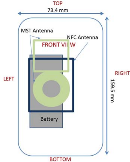
Figure F-2 MST and NFC Antenna Locations
