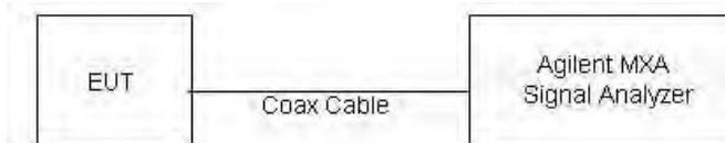
Figure 9-4 Power Measurement Setup for Bandwidths > 50 MHz
