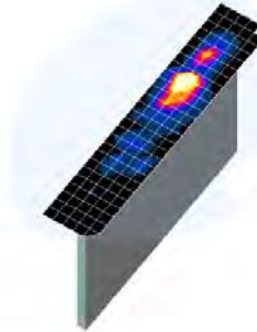
Figure 4-1 Sample SAR Area Scan
