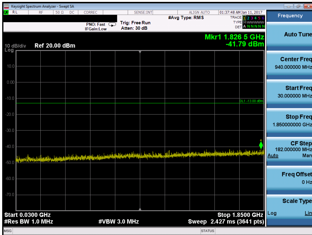
Plot 7-8. Conducted Spurious Plot (PCS GSM Mode – Ch. 661)
