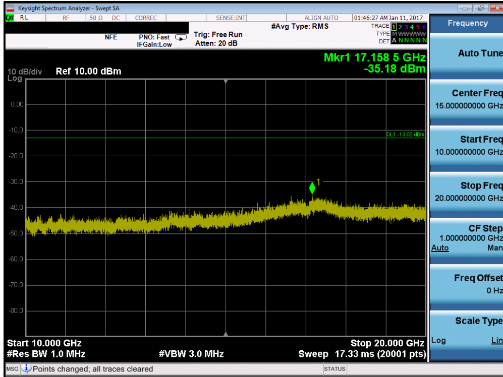
Plot 7-7. Conducted Spurious Plot (PCS GSM Mode – Ch. 512)
