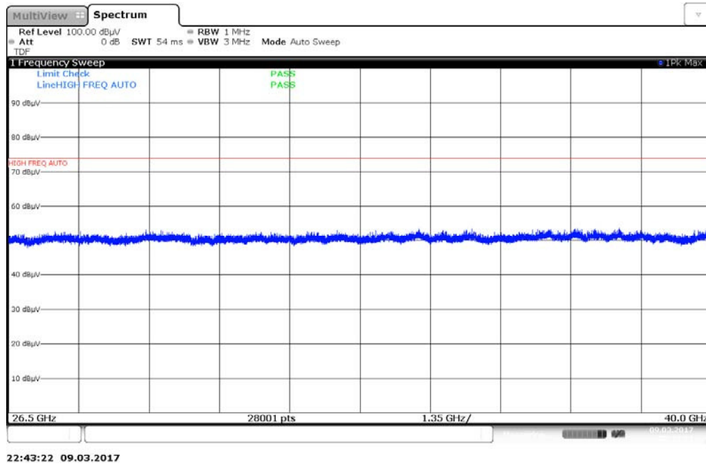
Plot 7-23. Radiated Spurious Plot 26.5GHz - 40GHz (802.11a – Ant. Pol. H)
