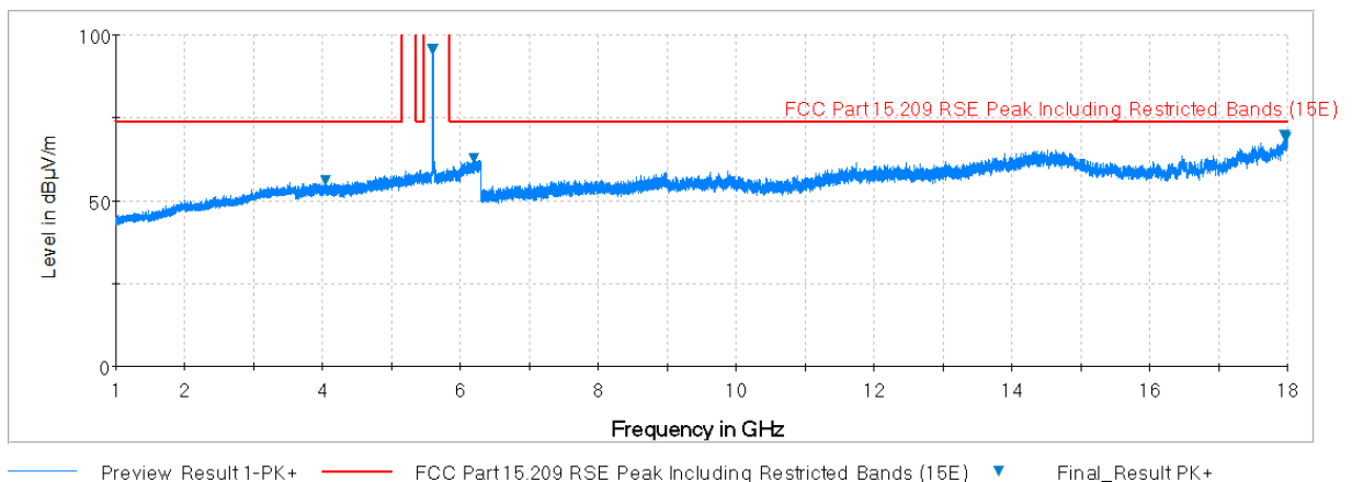
Plot 7-6. Radiated Spurious Plot above 1GHz (802.11a – U2C Ch. 120, Ant. Pol. V)
