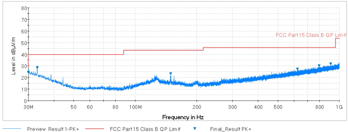
Plot 7-39. Radiated Spurious Plot below 1GHz (802.11a – U3 Ch. 157, Ant. Pol. V)
