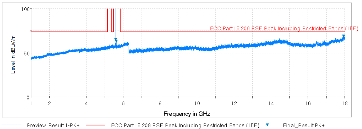
Plot 7-5. Radiated Spurious Plot above 1GHz (802.11a – U2C Ch. 120, Ant. Pol. H)
