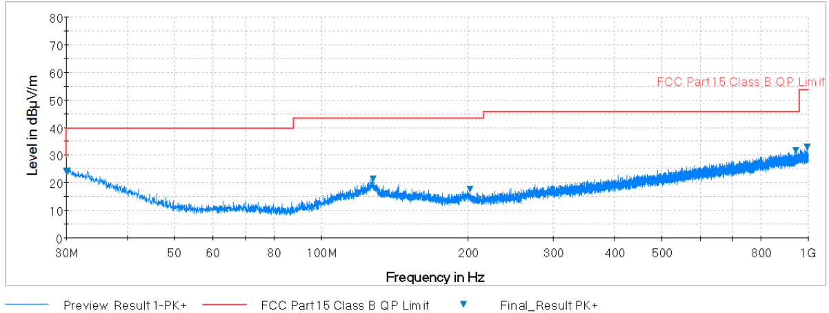
Plot 7-40. Radiated Spurious Plot below 1GHz (802.11a – U3 Ch. 157, Ant. Pol. H)
