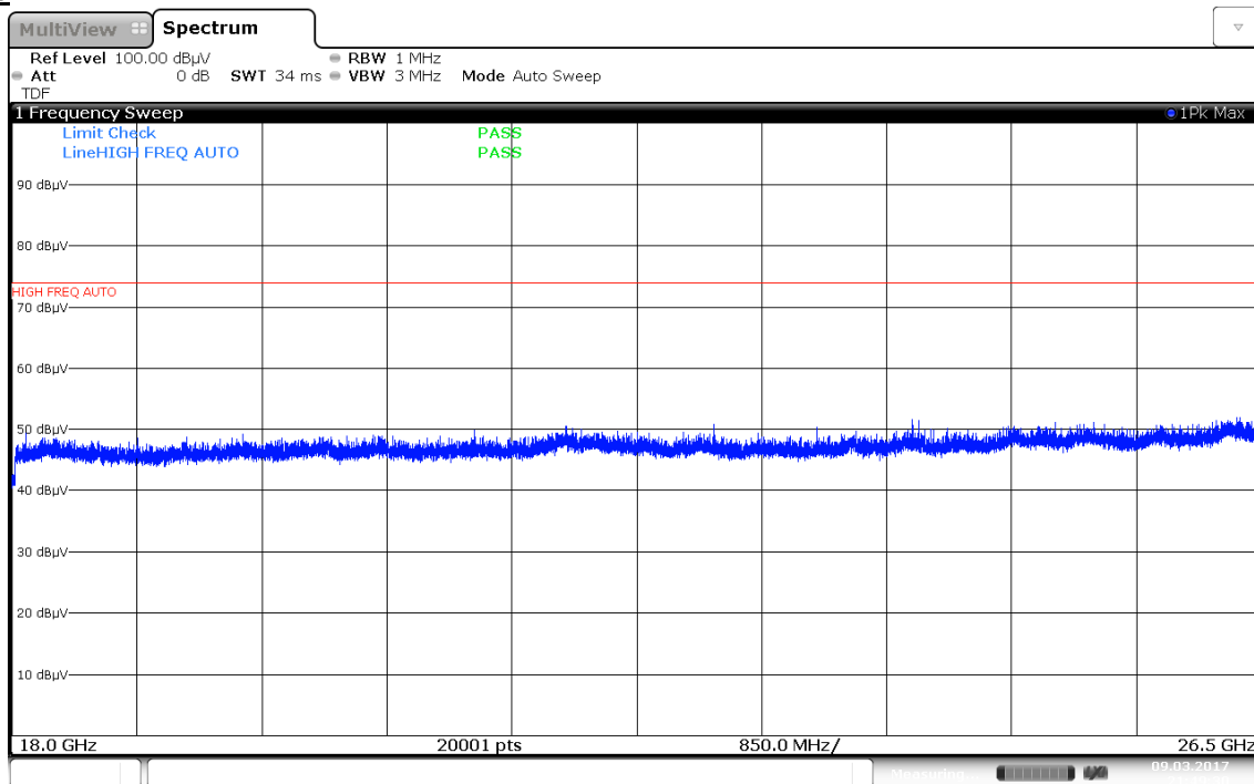
Plot 7-21. Radiated Spurious Plot above 18GHz - 26.5GHz (802.11a – Ant. Pol. H)
