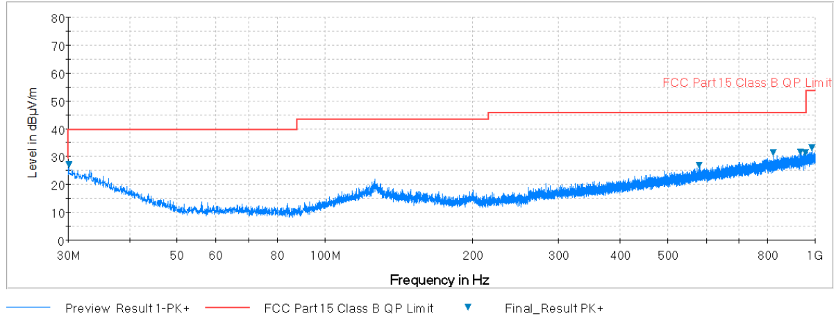
Plot 7-38. Radiated Spurious Plot below 1GHz (802.11a – U3 Ch. 157, Ant. Pol. H)
