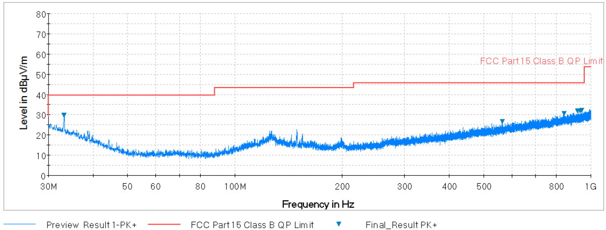
Plot 7-41. Radiated Spurious Plot below 1GHz (802.11a – U3 Ch. 157, Ant. Pol. V)
