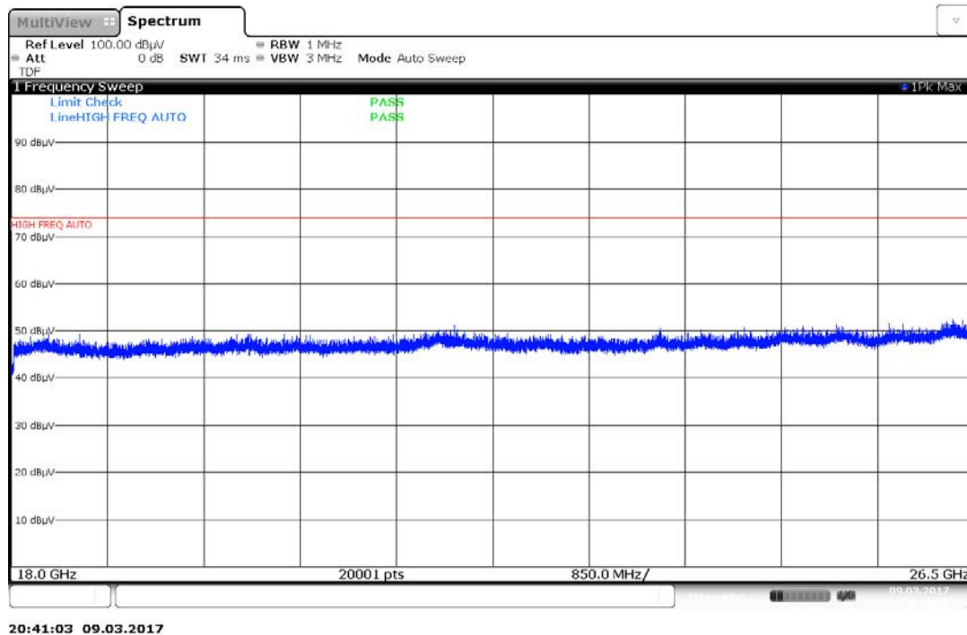
Plot 7-10. Radiated Spurious Plot above 18GHz - 26.5GHz (802.11a – Ant. Pol. V)
