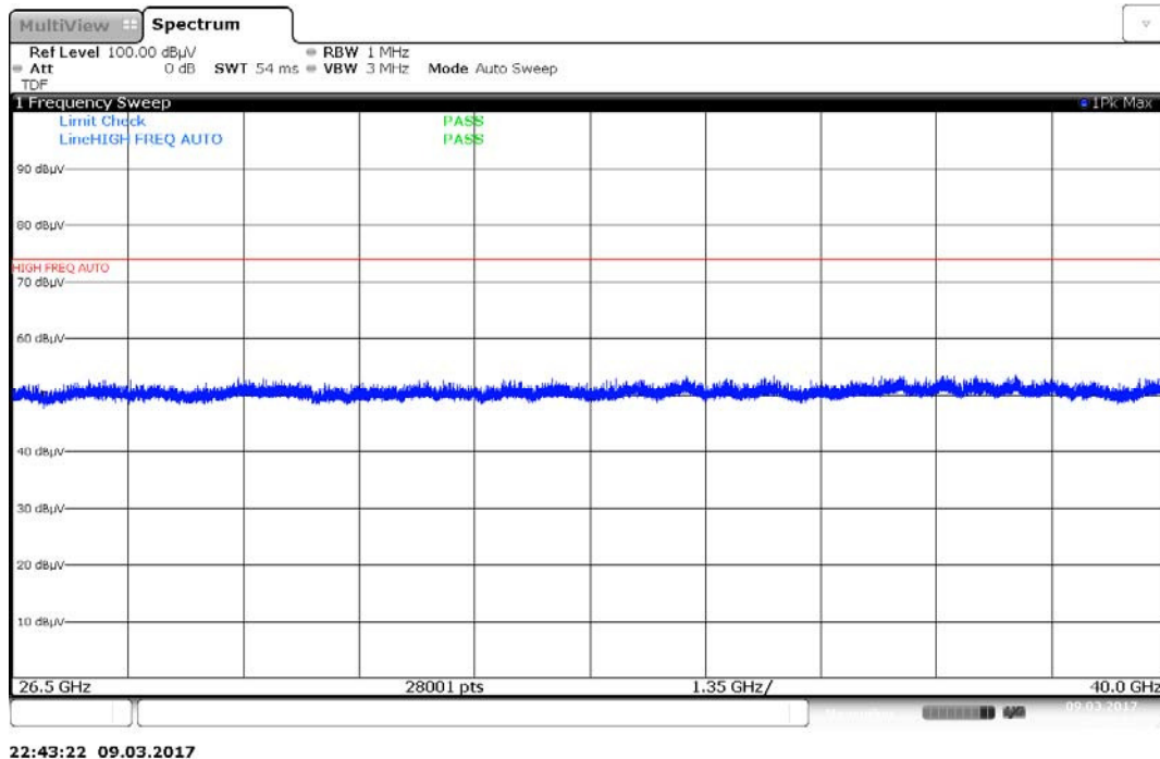
Plot 7-24. Radiated Spurious Plot above 26.5GHz - 40GHz (802.11a – Ant. Pol. V)
