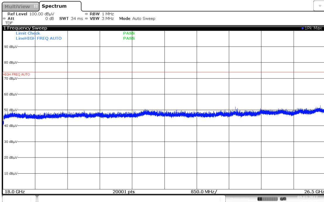
Plot 7-9. Radiated Spurious Plot 18GHz - 26.5GHz (802.11a – Ant. Pol. H)
