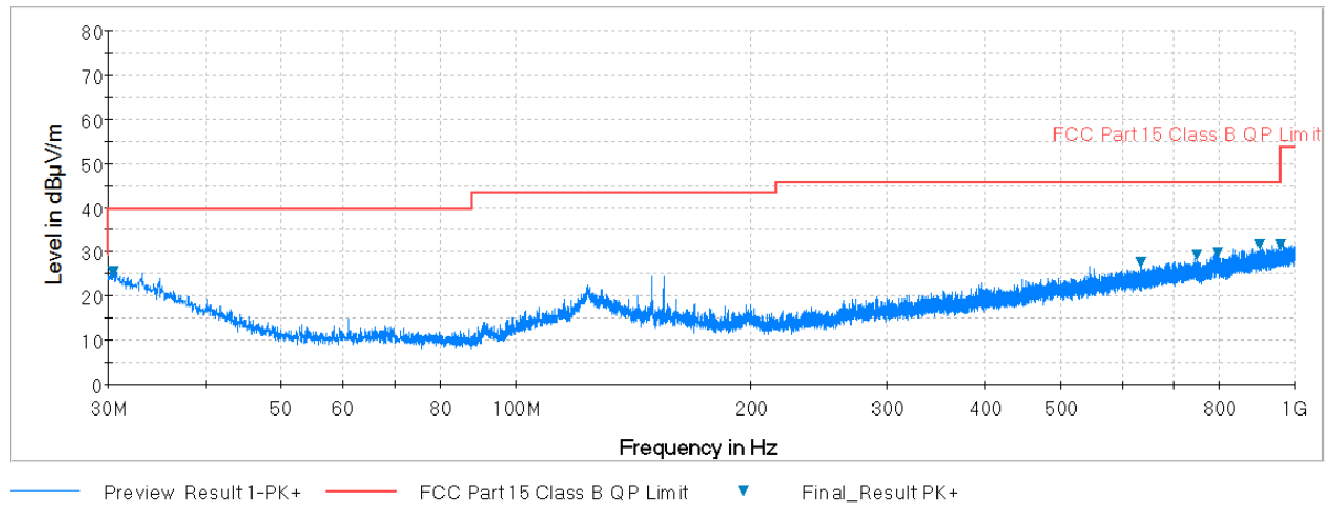
Plot 7-91. Radiated Spurious Plot below 1GHz (Pol. H)
