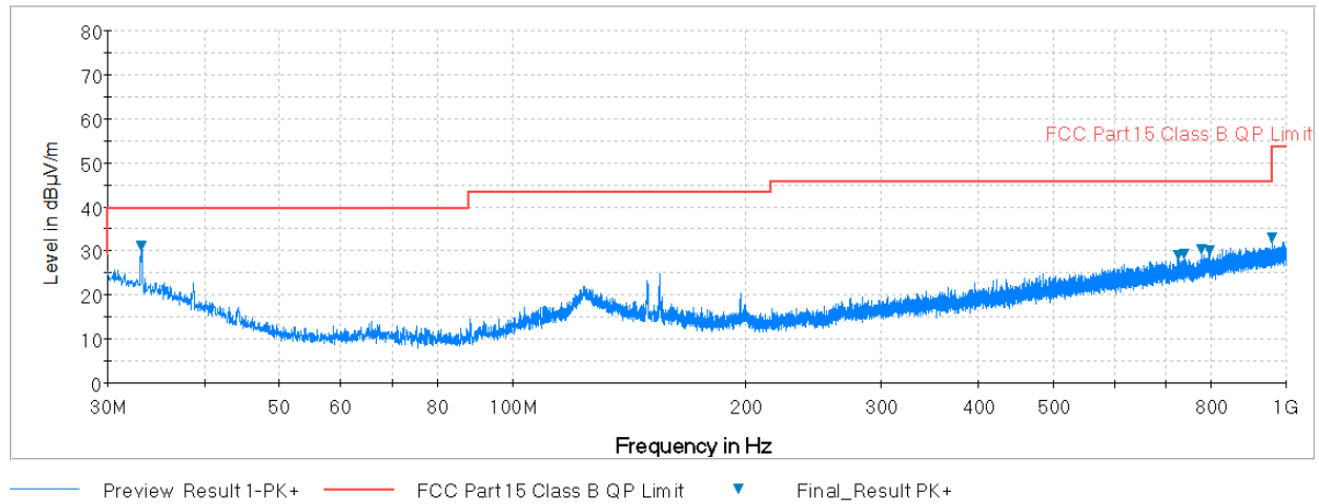
Plot 7-92. Radiated Spurious Plot below 1GHz (Pol. V)
