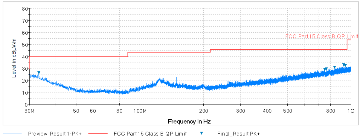
Plot 7-89. Radiated Spurious Plot below 1GHz (Pol. H)
