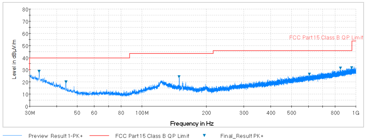
Plot 7-90. Radiated Spurious Plot below 1GHz (Pol. V)
