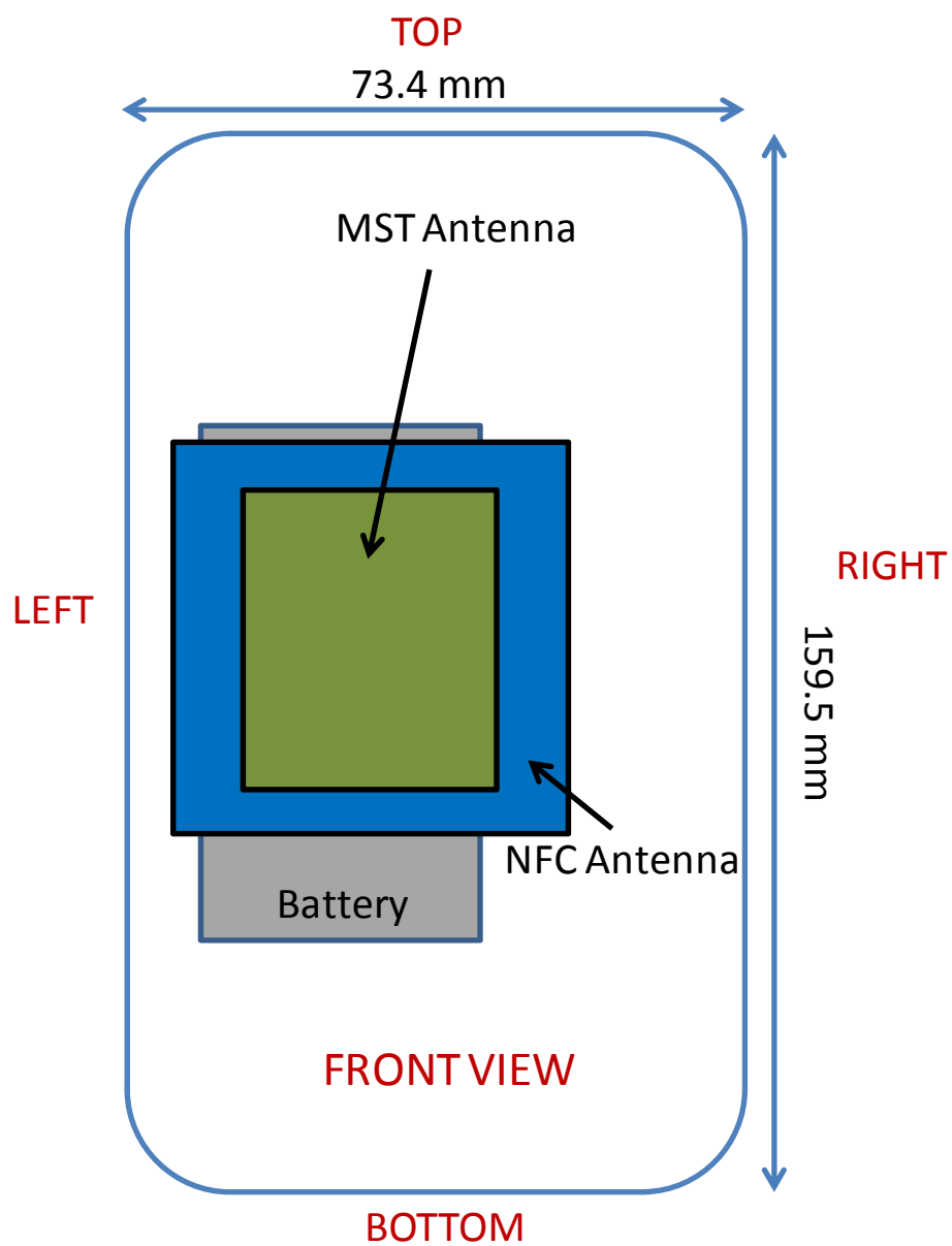
Figure F-2 MST and NFC Antenna Locations
