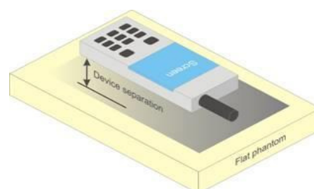
Figure 6-4 Sample Body-Worn Diagram
