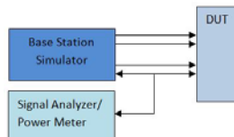
Figure 4-2 Power Measurement Setup
