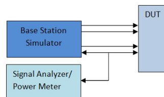
Figure 4-1 Power Measurement Setup
