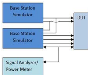
Figure 4-3 Power Measurement Setup
