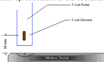
Figure 4-10 Measurement Distance
