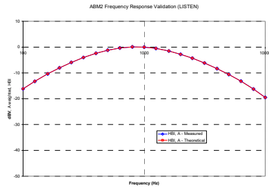
Figure 4-7 ABM2 Frequency Response Validation
