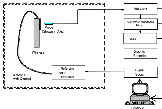
Figure 4-13 Audio Magnetic Field Test Setup
