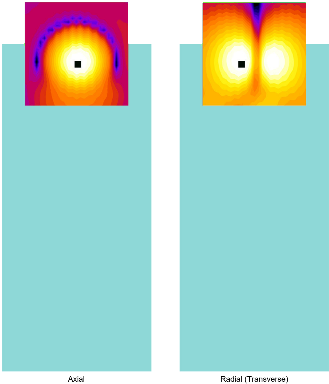
Figure 7-1 T-Coil Scan Overlay Magnetic Field Distributions
