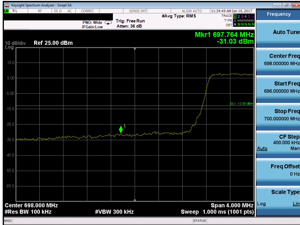
Plot 7-149. Lower Band Edge Plot (Band 12/17 - 5.0MHz QPSK - RB Size 25)
