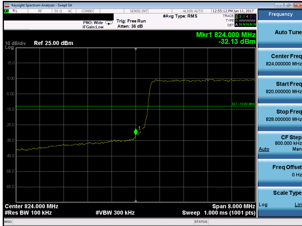
Plot 7-167. Lower Band Edge Plot (Band 5/26 - 10.0MHz QPSK - RB Size 50)
