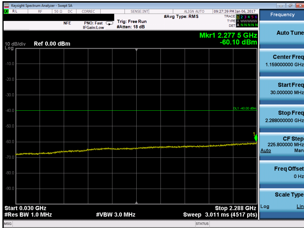
Plot 7-133. Conducted Spurious Plot (Band 30 – 5.0MHz QPSK – RB Size 1, RB Offset 0 – High Channel)
