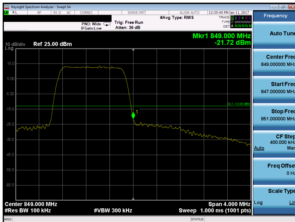
Plot 7-162. Upper Band Edge Plot (Band 5/26 – 1.4MHz QPSK – RB Size 6)
