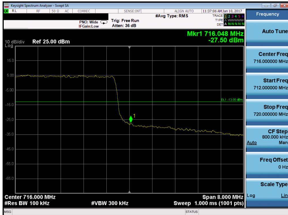
Plot 7-152. Upper Band Edge Plot (Band 12/17 - 10.0MHz QPSK - RB Size 50)
