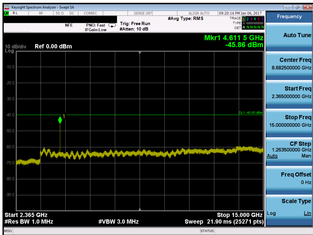
Plot 7-128. Conducted Spurious Plot (Band 30 – 5.0MHz QPSK – RB Size 1, RB Offset 0 – Low Channel)
