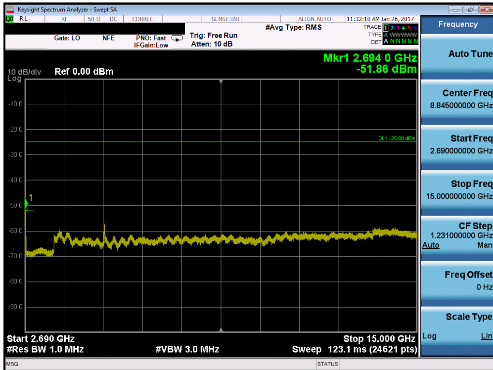
Plot 7-140. Conducted Spurious Plot (Band 41 – 20.0MHz QPSK – RB Size 1, RB Offset 0 – Mid Channel)
