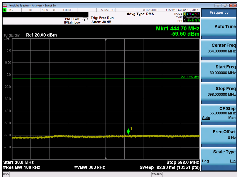
Plot 7-94. Conducted Spurious Plot (Band 12/17 – 5.0MHz QPSK – RB Size 1, RB Offset 0 – High Channel)
