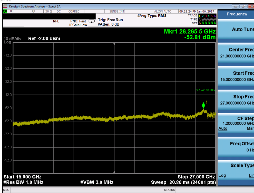
Plot 7-135. Conducted Spurious Plot (Band 30 – 5.0MHz QPSK – RB Size 1, RB Offset 0 – High Channel)
