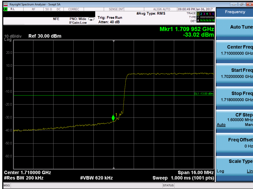
Plot 7-191. Lower Band Edge Plot (Band 4/66 – 20.0MHz QPSK – RB Size 100)
