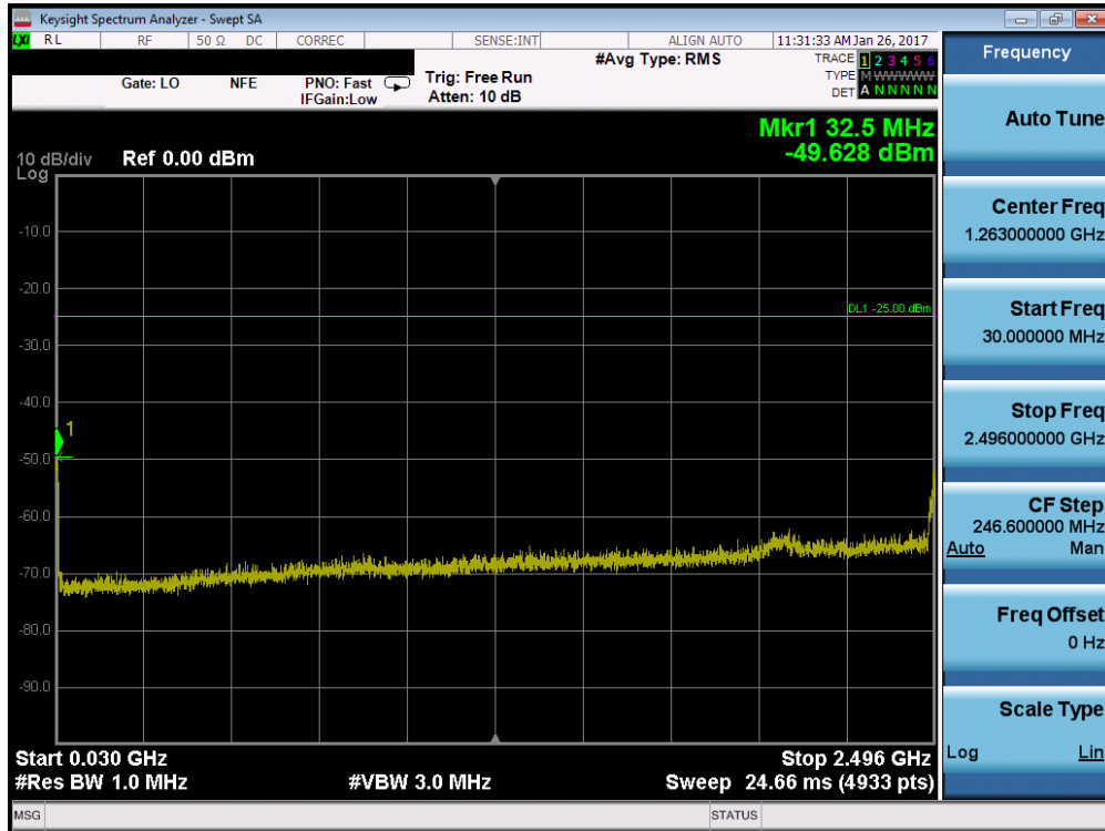
Plot 7-139. Conducted Spurious Plot (Band 41 – 20.0MHz QPSK – RB Size 1, RB Offset 0 – Mid Channel)
