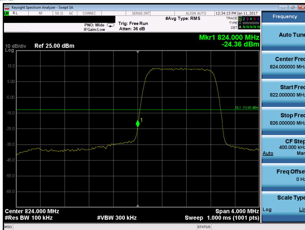
Plot 7-161. Lower Band Edge Plot (Band 5/26 – 1.4MHz QPSK – RB Size 6)
