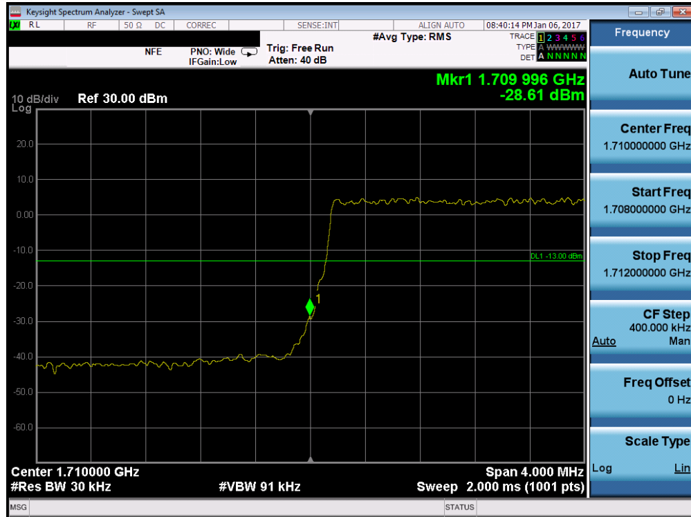
Plot 7-175. Lower Band Edge Plot (Band 4/66 – 3.0MHz QPSK – RB Size 15)
