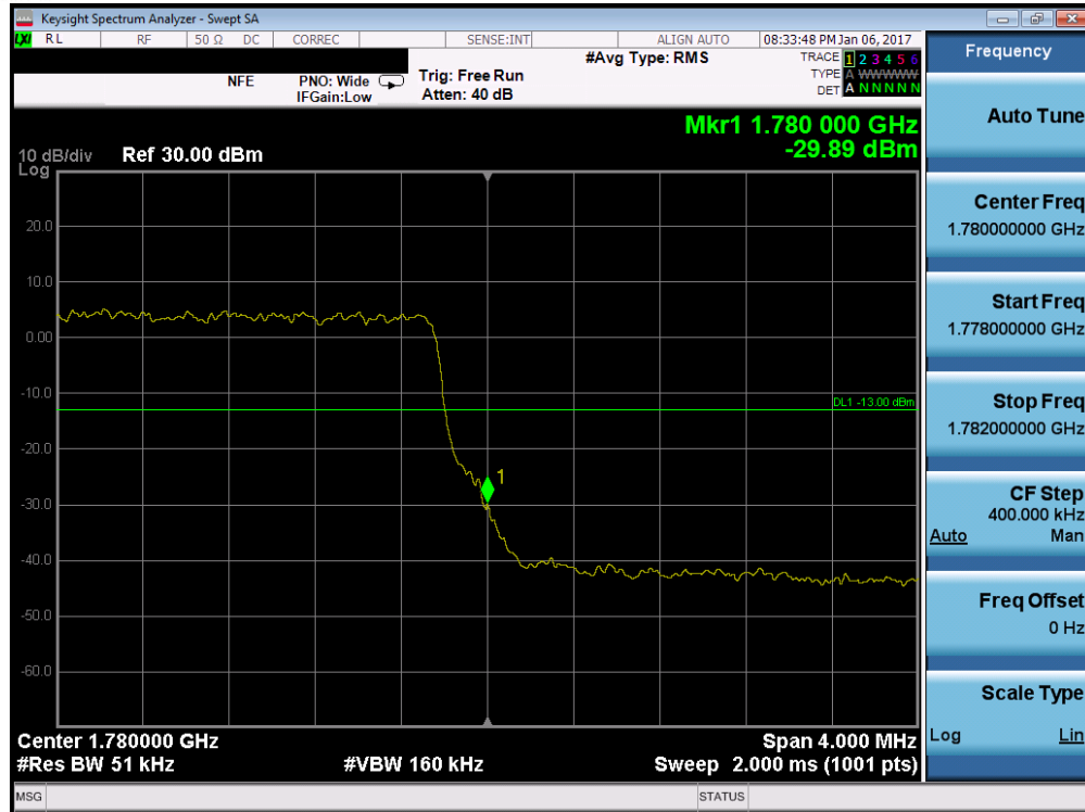
Plot 7-181. Upper Band Edge Plot (Band 4/66 – 5.0MHz QPSK – RB Size 25)
