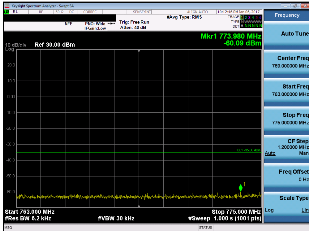
Plot 7-154. Lower Emission Mask Edge Plot (Band 13 – 5.0MHz QPSK – RB Size 25)
