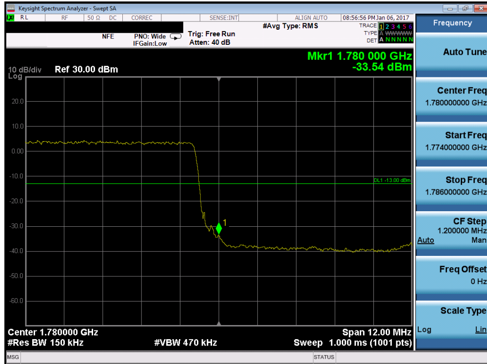
Plot 7-189. Upper Band Edge Plot (Band 4/66 – 15.0MHz QPSK – RB Size 75)
