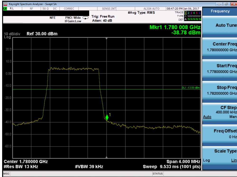
Plot 7-173. Upper Band Edge Plot (Band 4/66 – 1.4MHz QPSK – RB Size 6)
