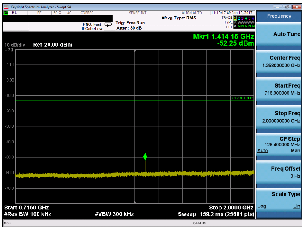
Plot 7-92. Conducted Spurious Plot (Band 12/17 – 5.0MHz QPSK – RB Size 1, RB Offset 0 – Mid Channel)
