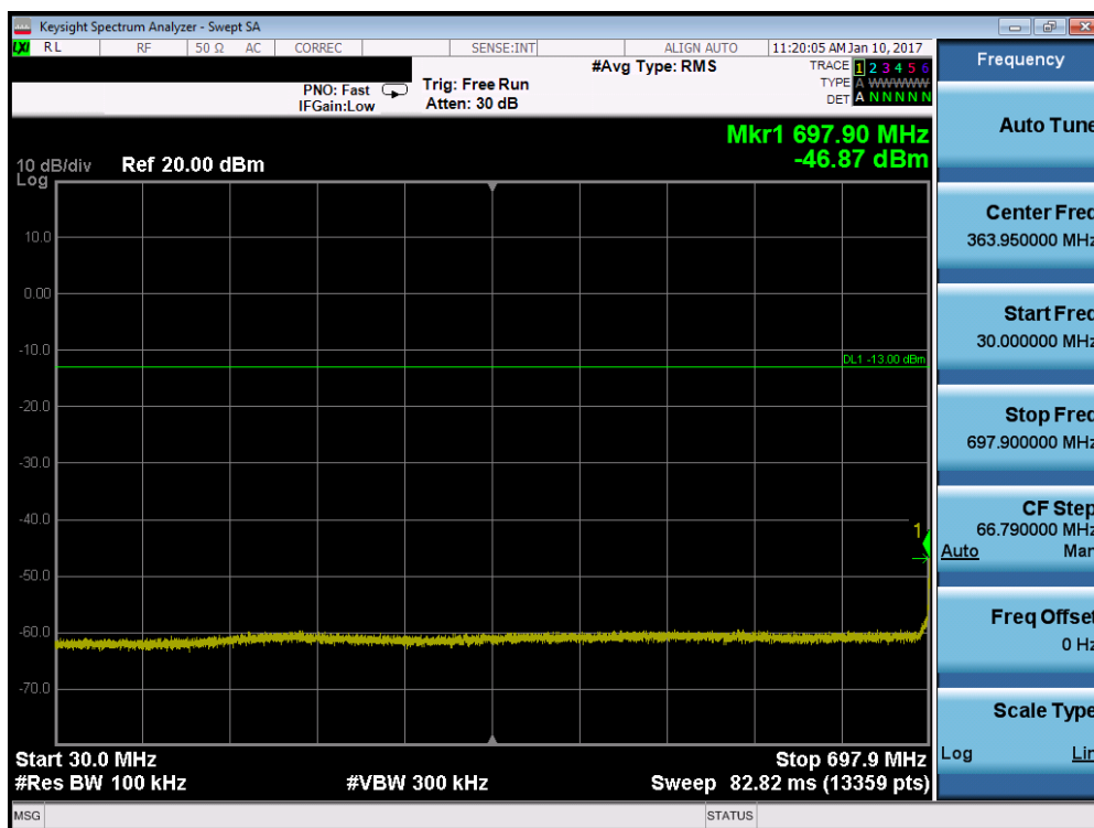
Plot 7-88. Conducted Spurious Plot (Band 12/17 – 1.4MHz QPSK – RB Size 1, RB Offset 0 – Low Channel)
