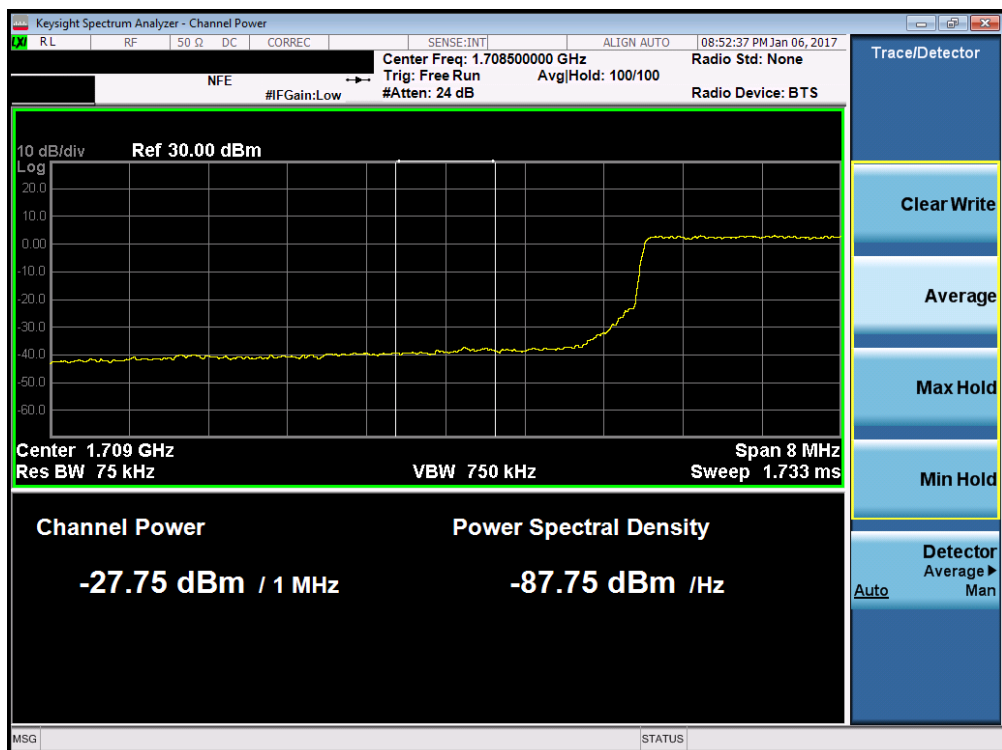
Plot 7-184. Lower Extended Band Edge Plot (Band 4/66 – 10.0MHz QPSK – RB Size 50)
