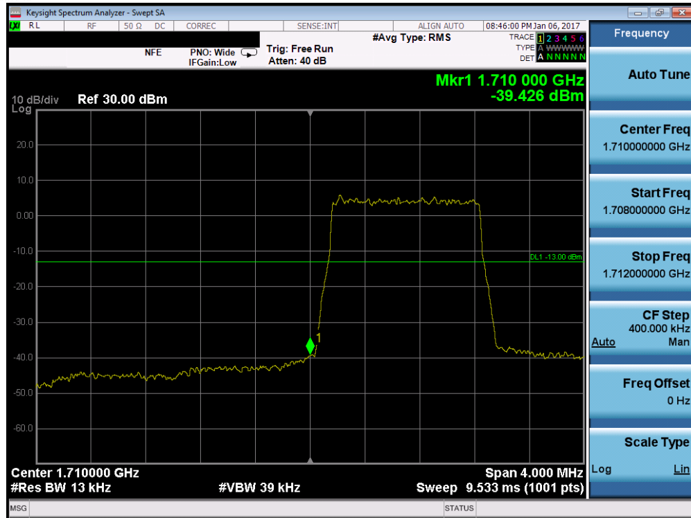
Plot 7-171. Lower Band Edge Plot (Band 4/66 – 1.4MHz QPSK – RB Size 6)
