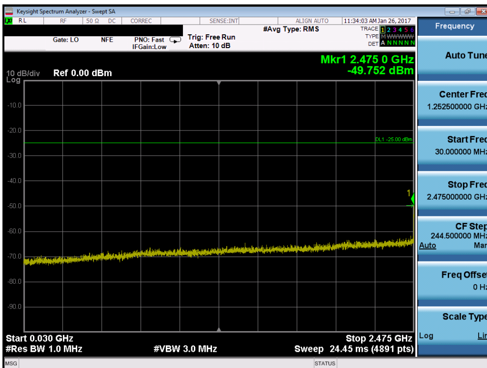
Plot 7-136. Conducted Spurious Plot (Band 41 – 20.0MHz QPSK – RB Size 1, RB Offset 0– Low Channel)
