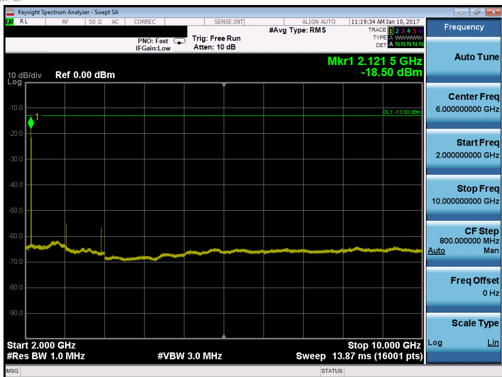
Plot 7-93. Conducted Spurious Plot (Band 12/17 – 5.0MHz QPSK – RB Size 1, RB Offset 0 – Mid Channel)
