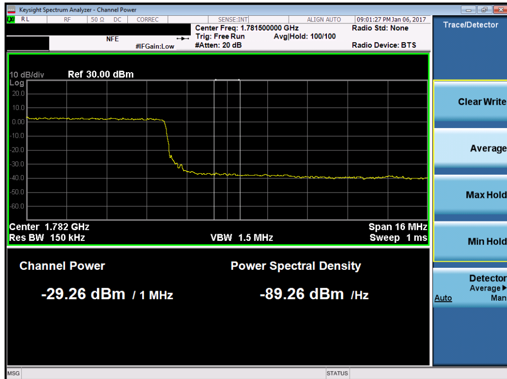
Plot 7-194. Upper Extended Band Edge Plot (Band 4/66 – 20.0MHz QPSK – RB Size 100)
