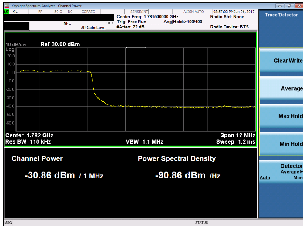
Plot 7-190. Upper Extended Band Edge Plot (Band 4/66 – 15.0MHz QPSK – RB Size 75)
