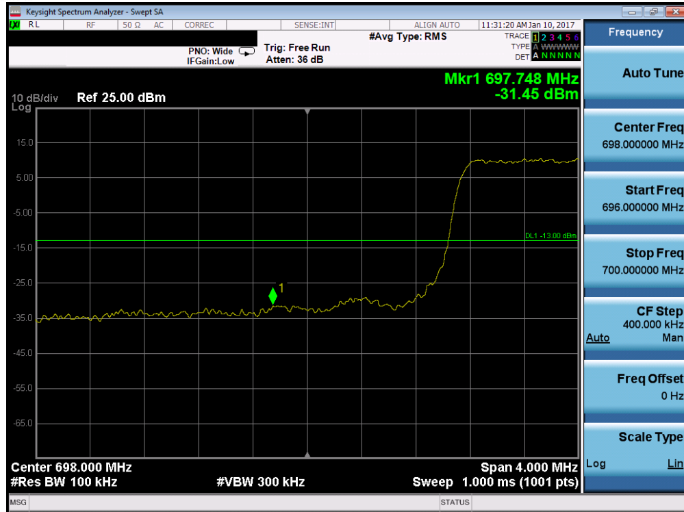
Plot 7-147. Lower Band Edge Plot (Band 12 – 3.0MHz QPSK – RB Size 15)
