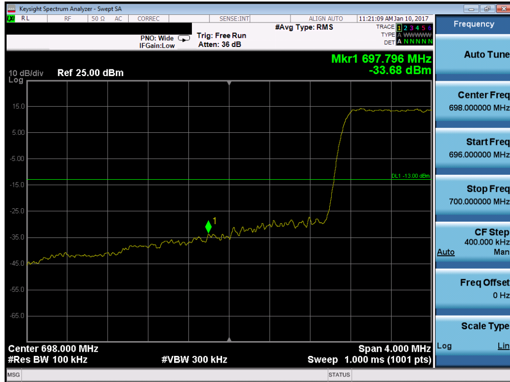
Plot 7-145. Lower Band Edge Plot (Band 12 – 1.4MHz QPSK – RB Size 6)
