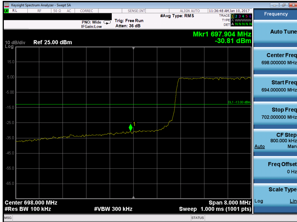
Plot 7-151. Lower Band Edge Plot (Band 12/17 - 10.0MHz QPSK - RB Size 50)
