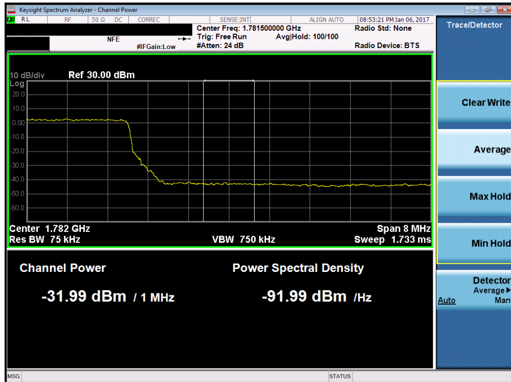
Plot 7-186. Upper Extended Band Edge Plot (Band 4/66 – 10.0MHz QPSK – RB Size 50)
