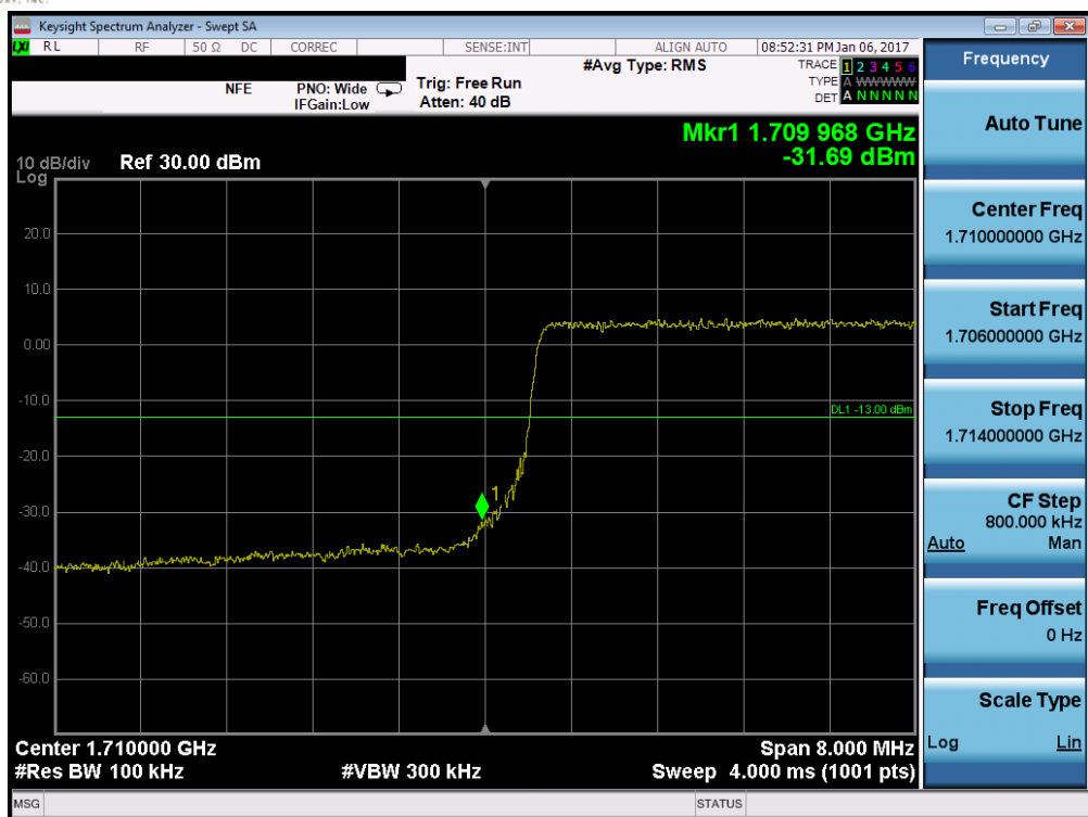
Plot 7-183. Lower Band Edge Plot (Band 4/66 – 10.0MHz QPSK – RB Size 50)
