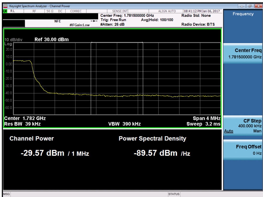
Plot 7-178. Upper Extended Band Edge Plot (Band 4/66 – 3.0MHz QPSK – RB Size 15)
