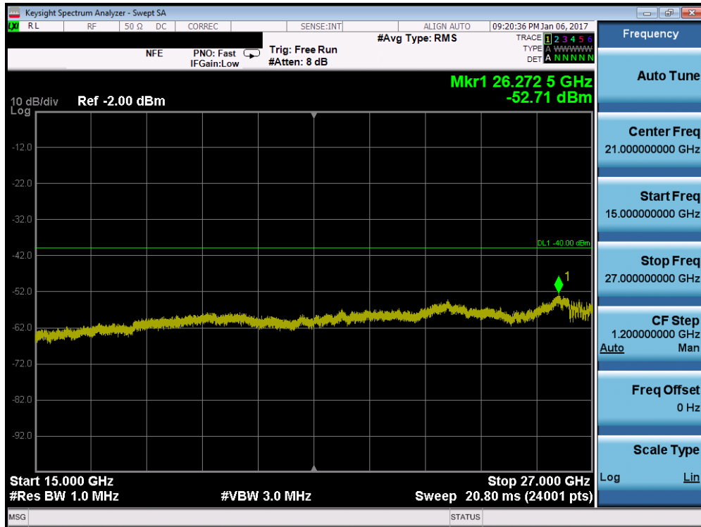
Plot 7-129. Conducted Spurious Plot (Band 30 – 5.0MHz QPSK – RB Size 1, RB Offset 0 – Low Channel)
