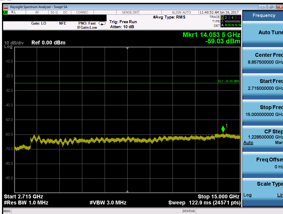
Plot 7-143. Conducted Spurious Plot (Band 41 – 20.0MHz QPSK – RB Size 1, RB Offset 0 – High Channel)
