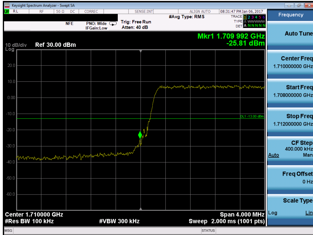
Plot 7-179. Lower Band Edge Plot (Band 4/66 – 5.0MHz QPSK – RB Size 25)
