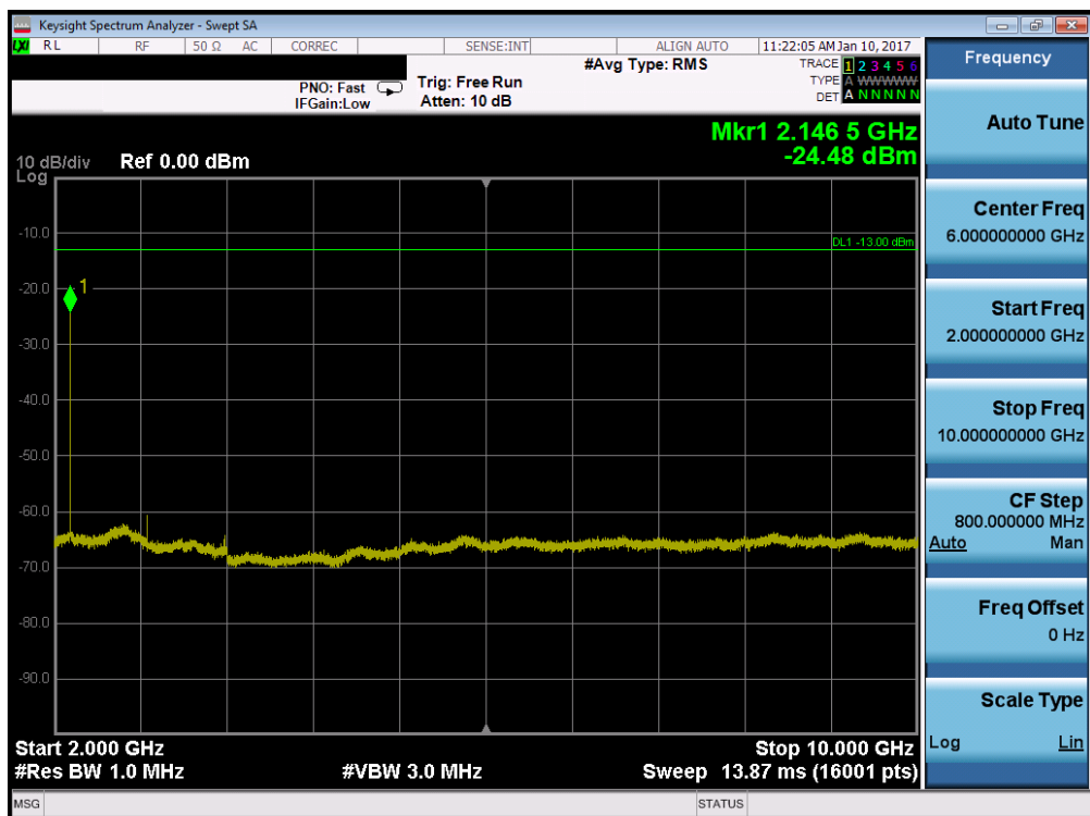
Plot 7-96. Conducted Spurious Plot (Band 12/17 – 5.0MHz QPSK – RB Size 1, RB Offset 0 – High Channel)
