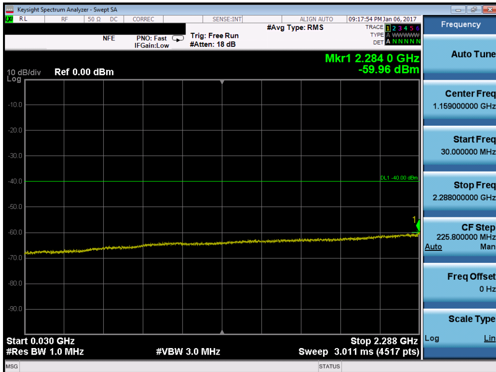
Plot 7-130. Conducted Spurious Plot (Band 30 – 5.0MHz QPSK – RB Size 1, RB Offset 0 – Mid Channel)
