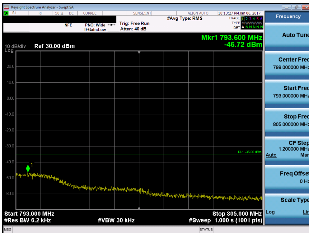
Plot 7-156. Upper Emission Mask Edge Plot (Band 13 – 5.0MHz QPSK – RB Size 25)
