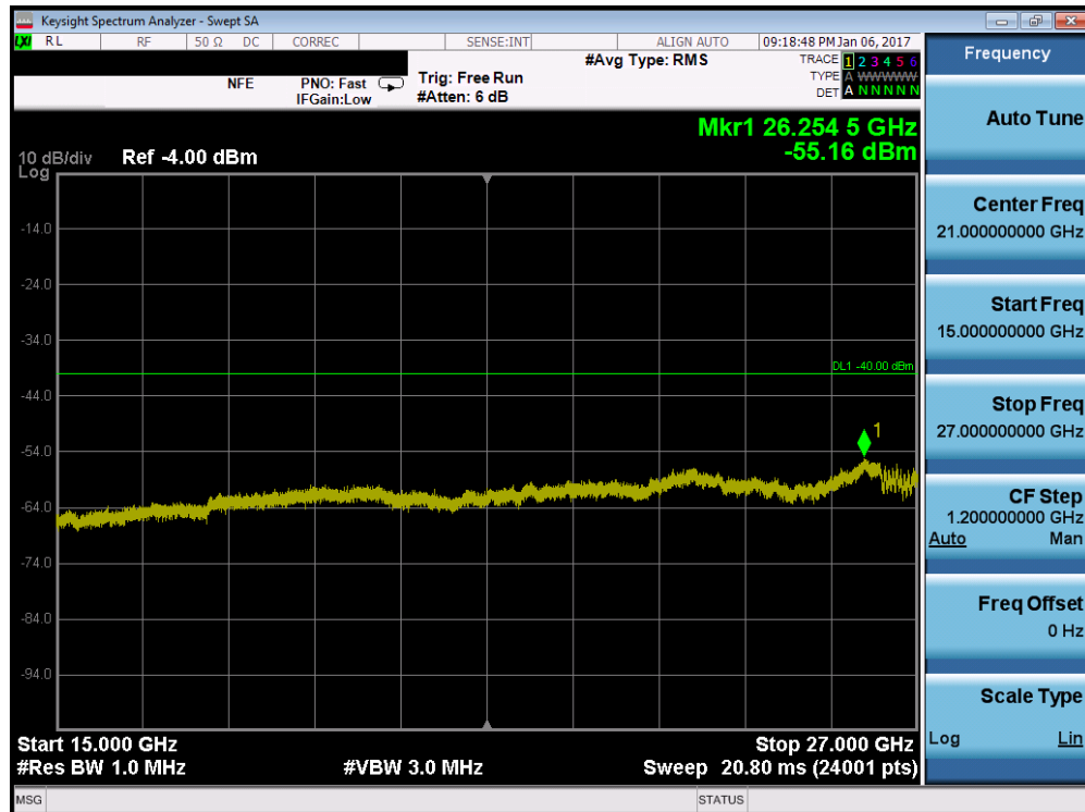
Plot 7-132. Conducted Spurious Plot (Band 30 – 5.0MHz QPSK – RB Size 1, RB Offset 0 – Mid Channel)
