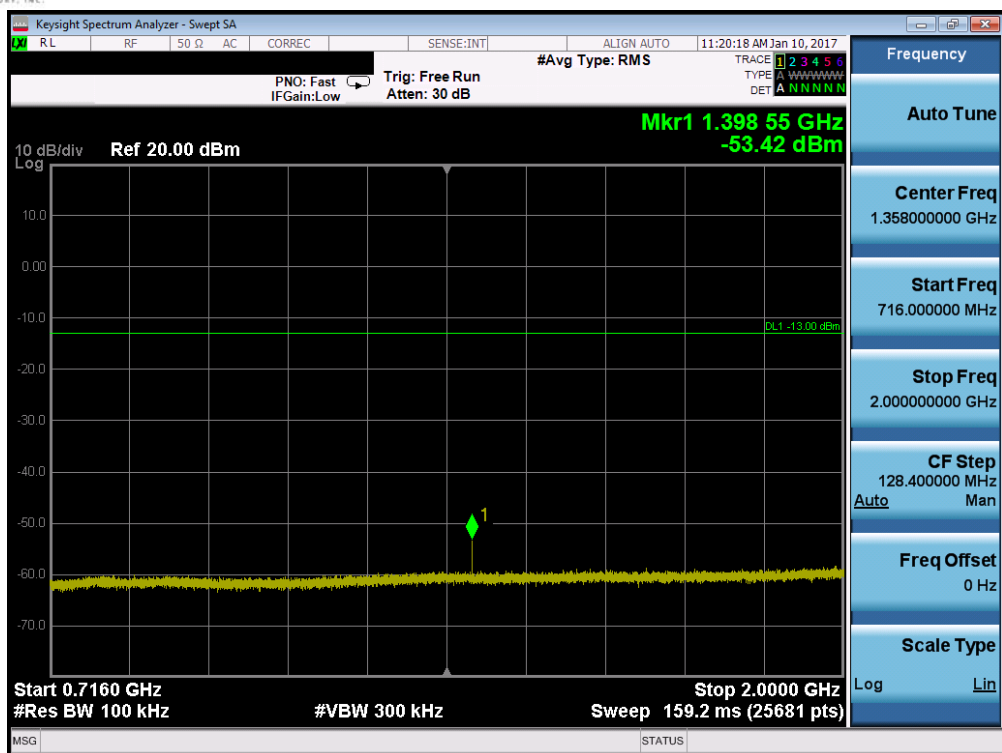
Plot 7-89. Conducted Spurious Plot (Band 12/17 – 5.0MHz QPSK – RB Size 1, RB Offset 0 – Low Channel)
