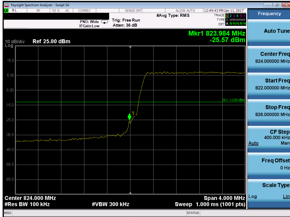
Plot 7-165. Lower Band Edge Plot (Band 5/26 - 5.0MHz QPSK - RB Size 25)
