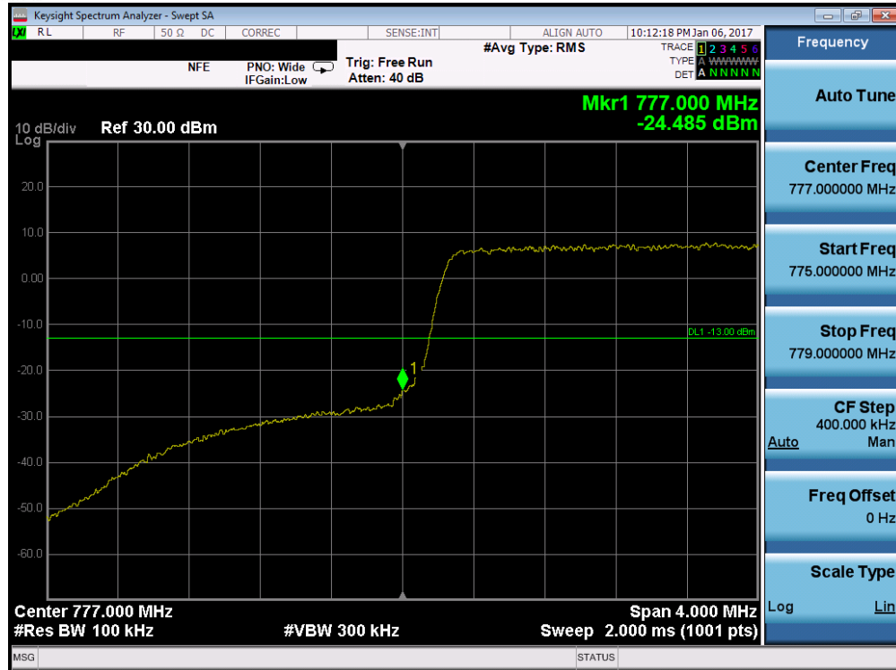
Plot 7-153. Lower Band Edge Plot (Band 13 – 5.0MHz QPSK – RB Size 25)
