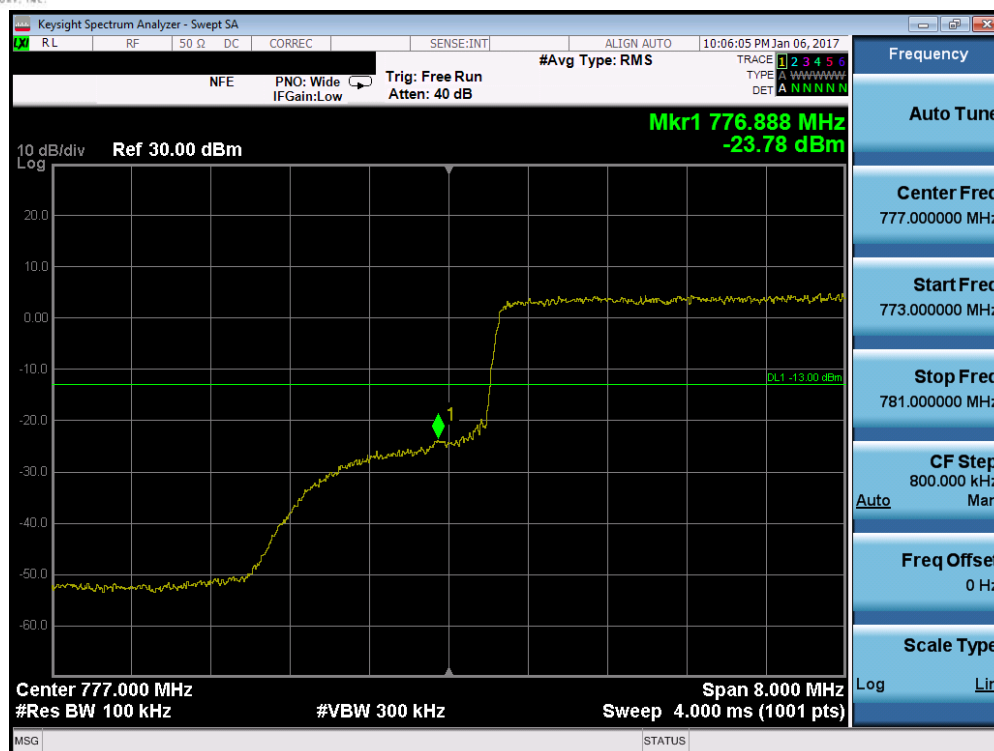
Plot 7-157. Lower Band Edge Plot (Band 13 – 10.0MHz QPSK – RB Size 50)
