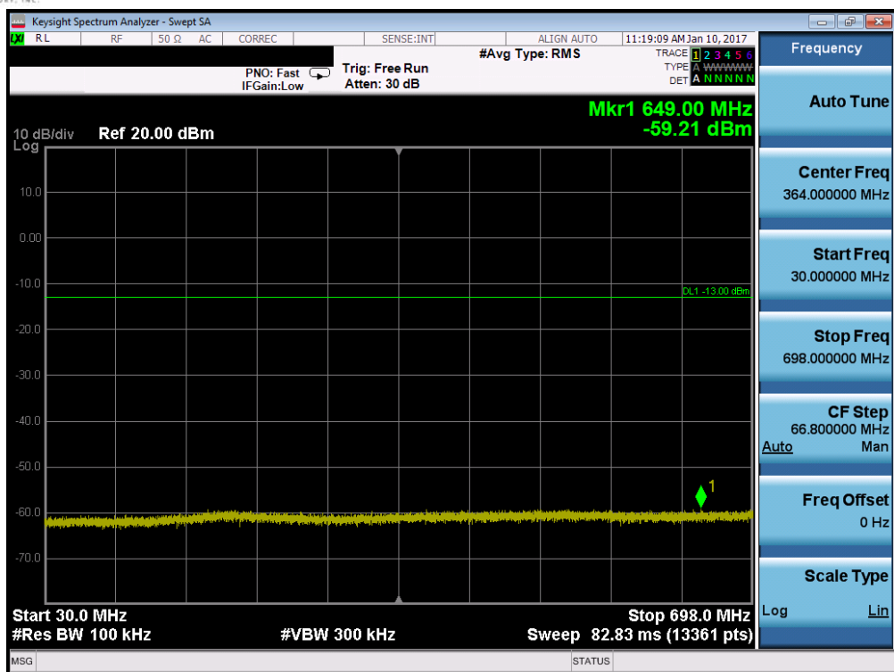
Plot 7-91. Conducted Spurious Plot (Band 12/17 – 5.0MHz QPSK – RB Size 1, RB Offset 0 – Mid Channel)
