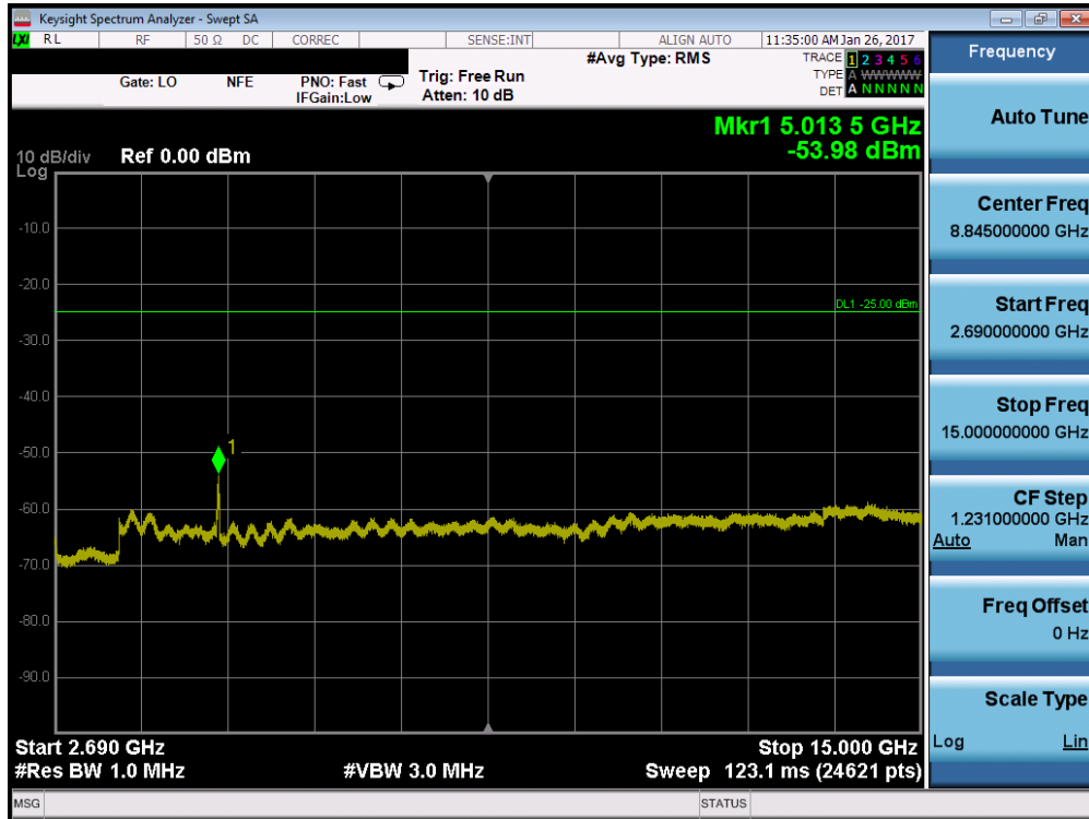
Plot 7-137. Conducted Spurious Plot (Band 41 – 20.0MHz QPSK – RB Size 1, RB Offset 0 – Low Channel)
