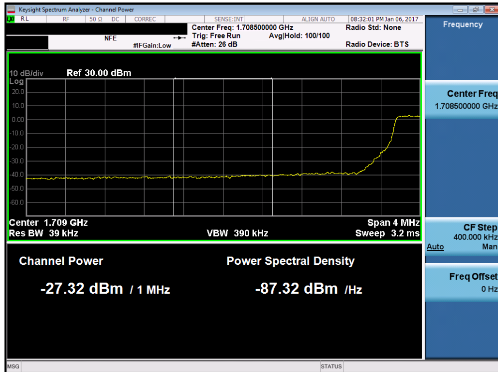
Plot 7-180. Lower Extended Band Edge Plot (Band 4/66 – 5.0MHz QPSK – RB Size 25)
