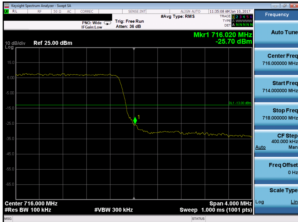
Plot 7-150. Upper Band Edge Plot (Band 12/17 - 5.0MHz QPSK - RB Size 25)
