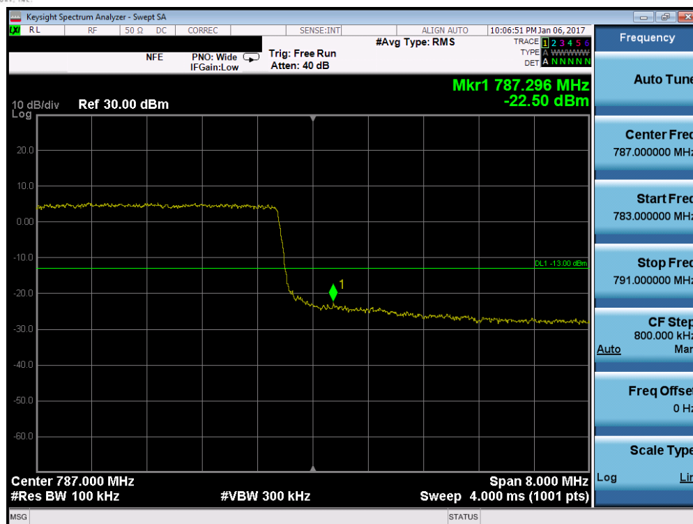
Plot 7-159. Upper Band Edge Plot (Band 13 – 10.0MHz QPSK – RB Size 50)
