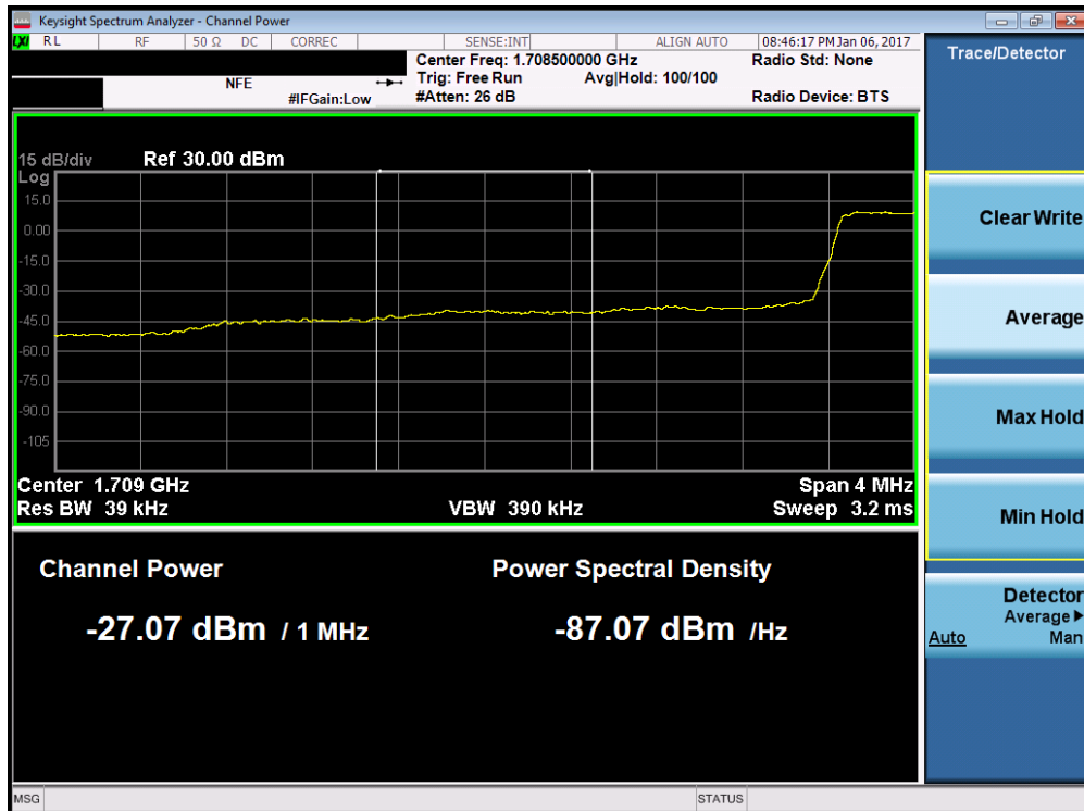
Plot 7-172. Lower Extended Band Edge Plot (Band 4/66 – 1.4MHz QPSK – RB Size 6)
