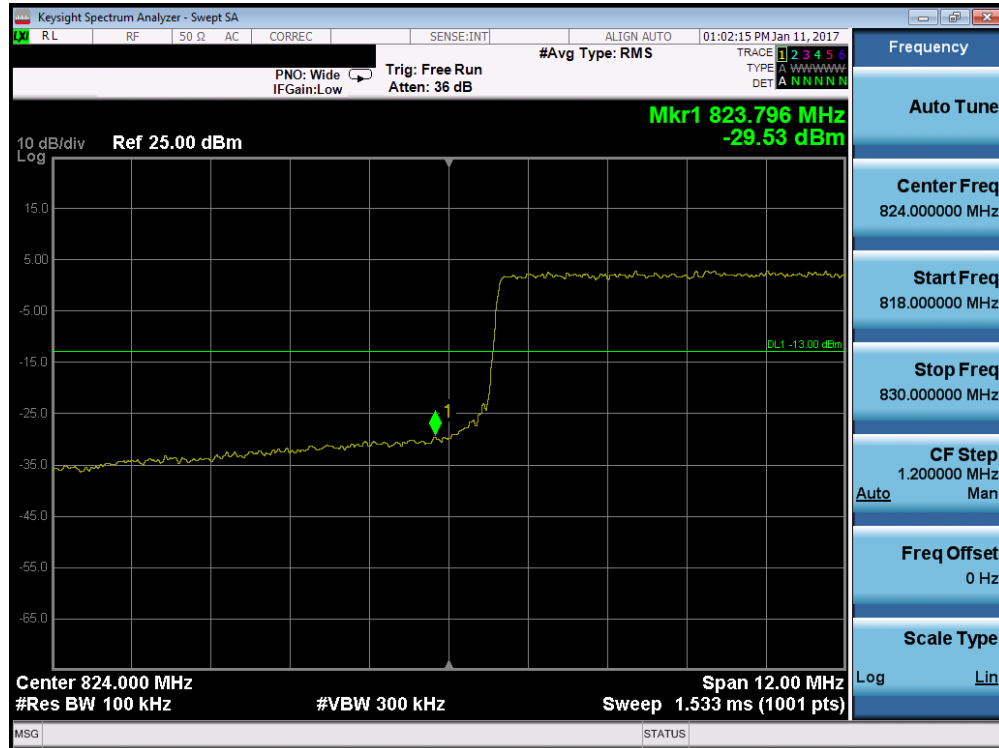
Plot 7-169. Lower Band Edge Plot (Band 26 – 15.0MHz QPSK – RB Size 75)
