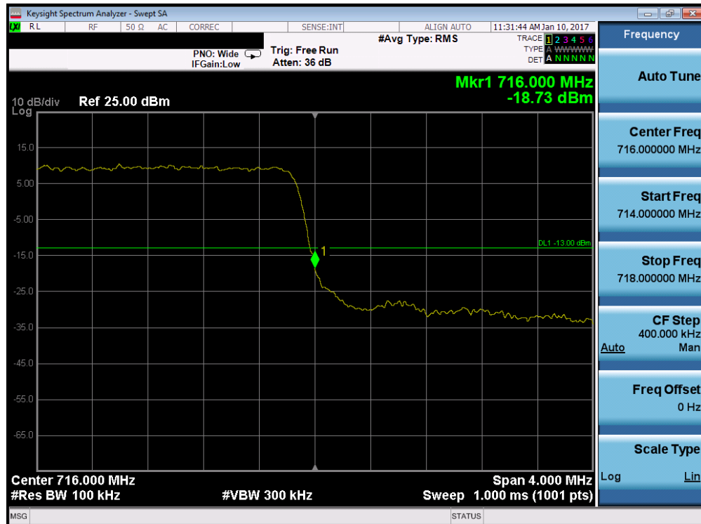
Plot 7-148. Upper Band Edge Plot (Band 12 – 3.0MHz QPSK – RB Size 15)
