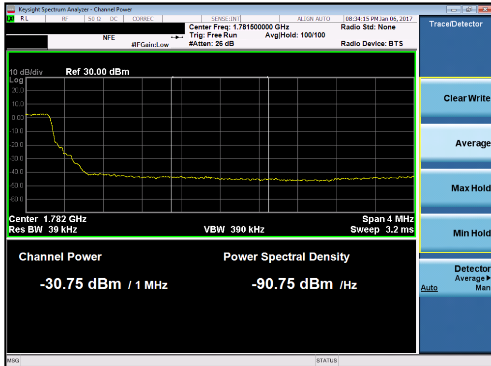
Plot 7-182. Upper Extended Band Edge Plot (Band 4/66 – 5.0MHz QPSK – RB Size 25)
