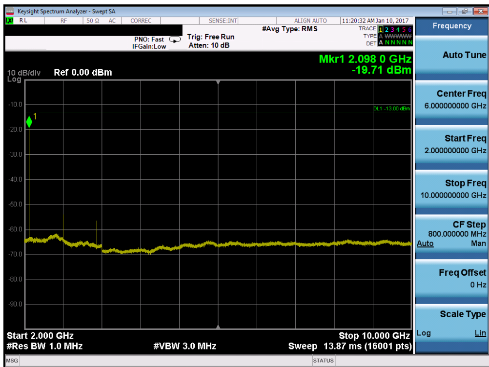
Plot 7-90. Conducted Spurious Plot (Band 12/17 – 5.0MHz QPSK – RB Size 1, RB Offset 0 – Low Channel)
