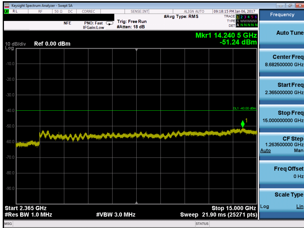
Plot 7-131. Conducted Spurious Plot (Band 30 – 5.0MHz QPSK – RB Size 1, RB Offset 0 – Mid Channel)
