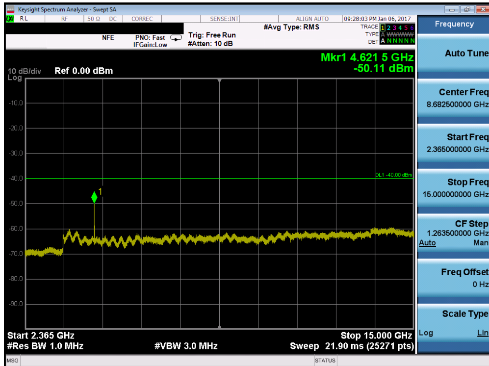
Plot 7-134. Conducted Spurious Plot (Band 30 – 5.0MHz QPSK – RB Size 1, RB Offset 0 – High Channel)
