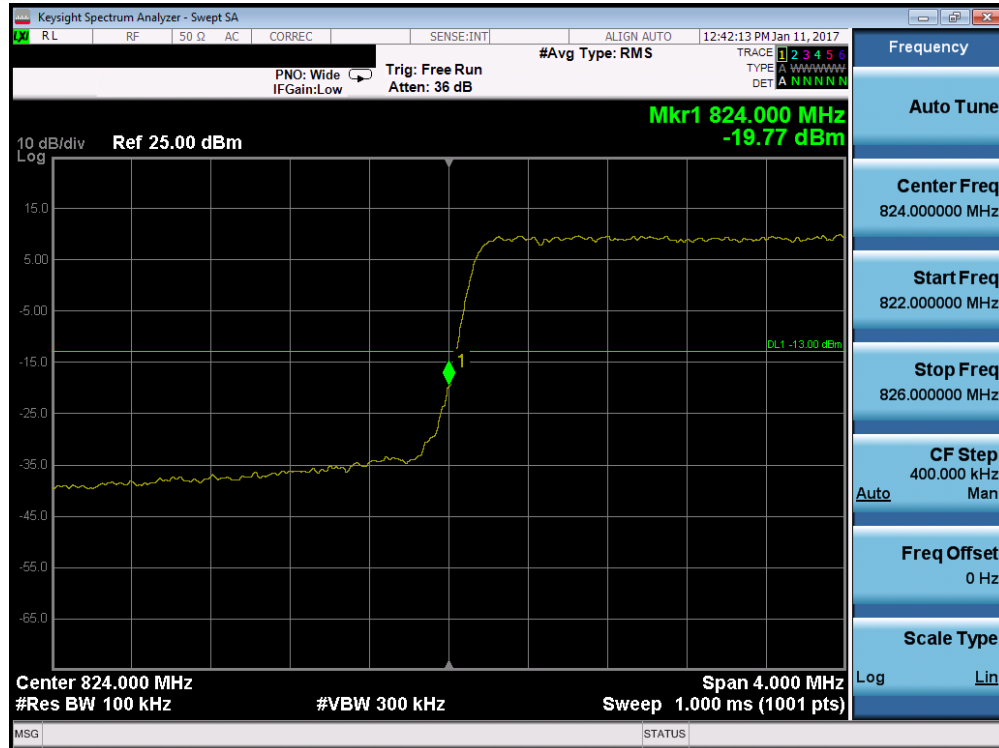
Plot 7-163. Lower Band Edge Plot (Band 5/26 - 3.0MHz QPSK - RB Size 15)
