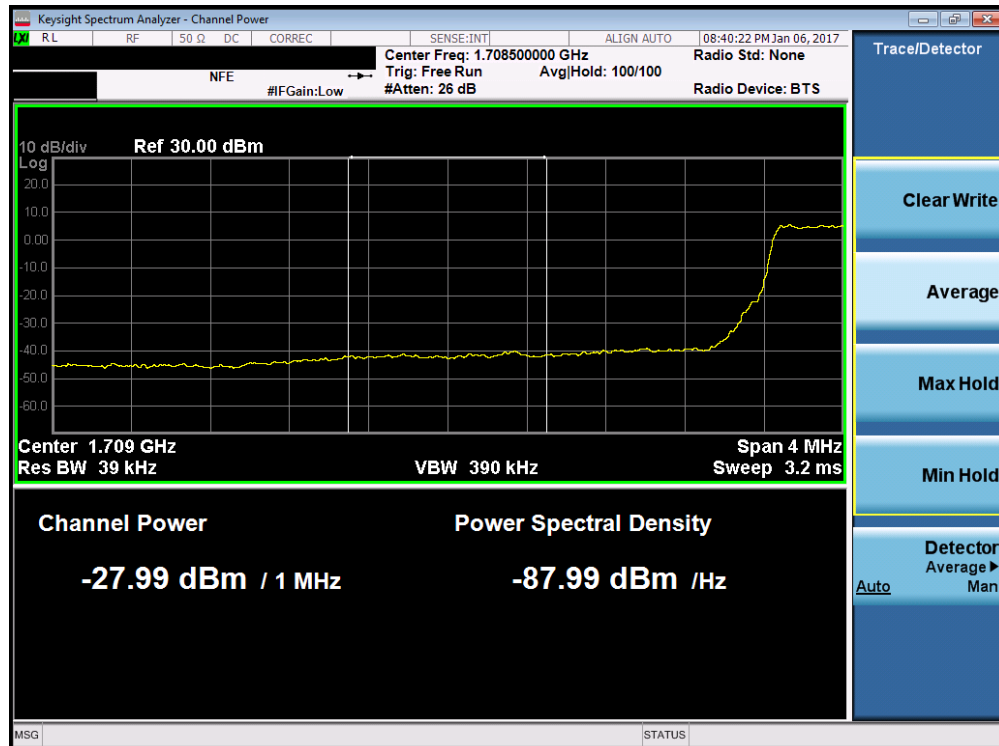
Plot 7-176. Lower Extended Band Edge Plot (Band 4/66 – 3.0MHz QPSK – RB Size 15)
