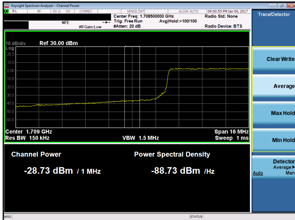
Plot 7-192. Lower Extended Band Edge Plot (Band 4/66 – 20.0MHz QPSK – RB Size 100)
