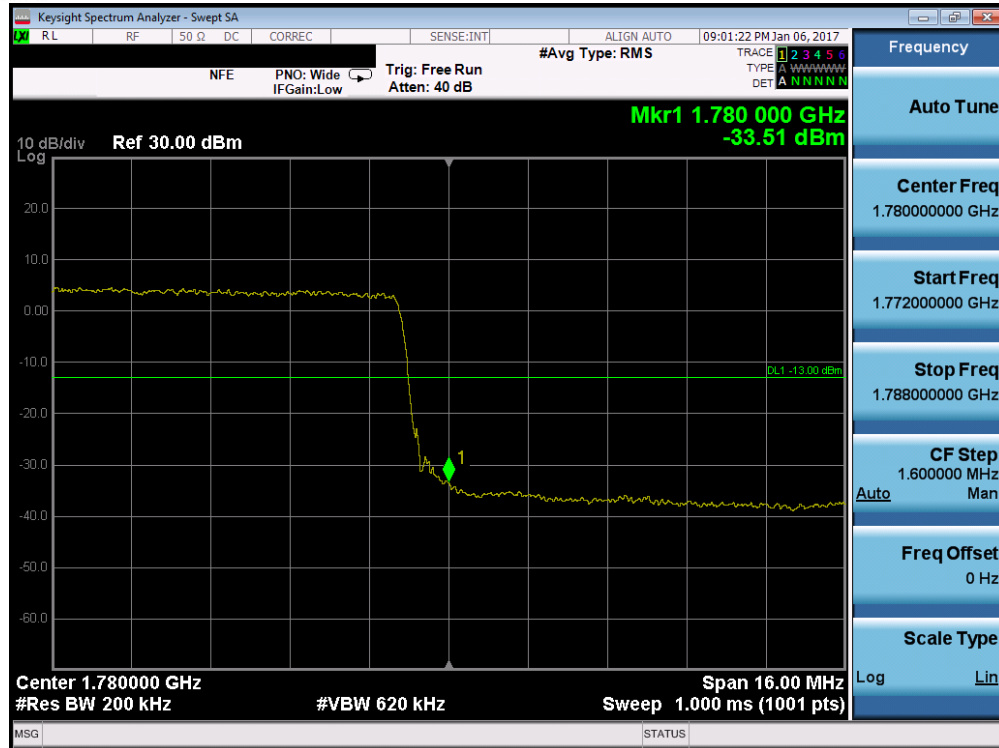
Plot 7-193. Upper Band Edge Plot (Band 4/66 – 20.0MHz QPSK – RB Size 100)
