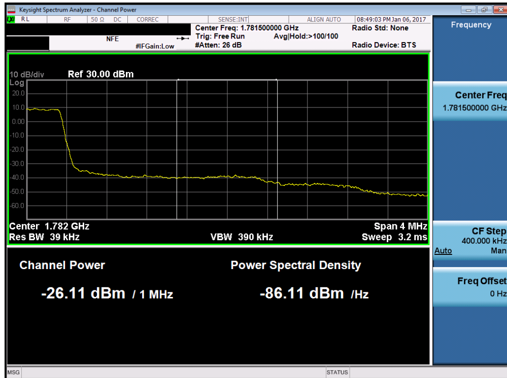
Plot 7-174. Upper Extended Band Edge Plot (Band 4/66 – 1.4MHz QPSK – RB Size 6)
