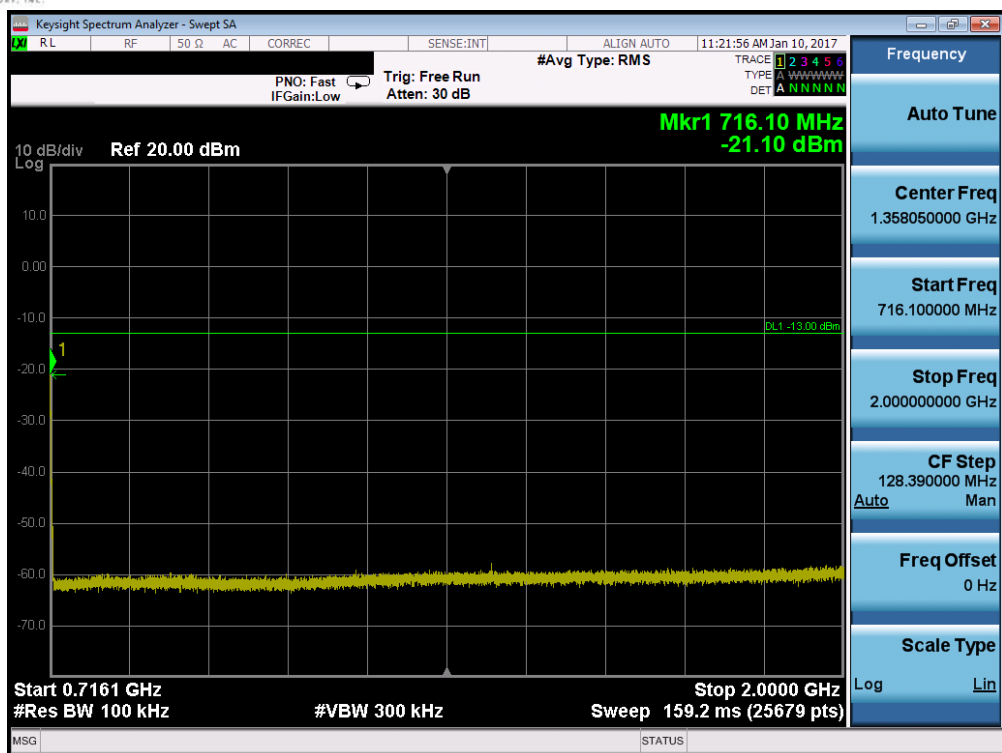
Plot 7-95. Conducted Spurious Plot (Band 12/17 – 5.0MHz QPSK – RB Size 1, RB Offset 0 – High Channel)
