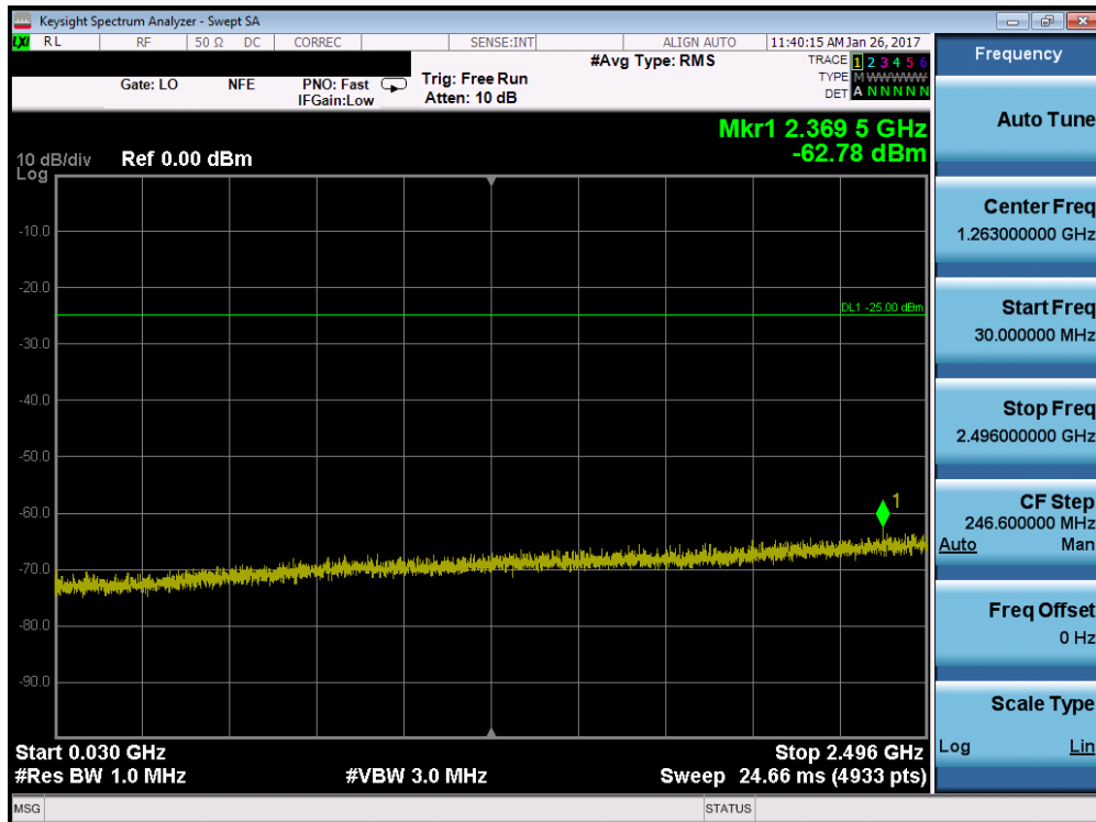
Plot 7-142. Conducted Spurious Plot (Band 41 – 20.0MHz QPSK – RB Size 1, RB Offset 0 – High Channel)
