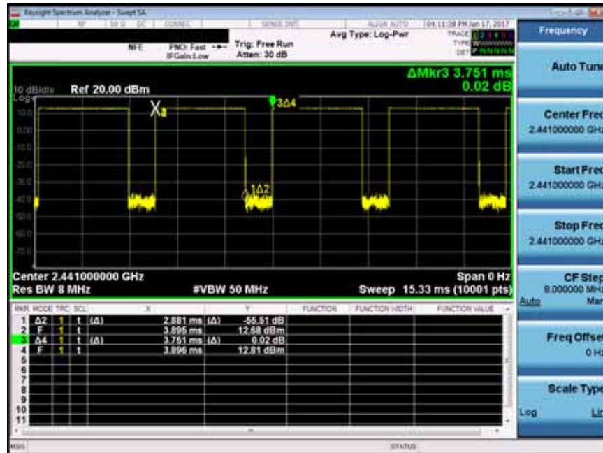
Figure 8-3 Bluetooth Transmission Plot
