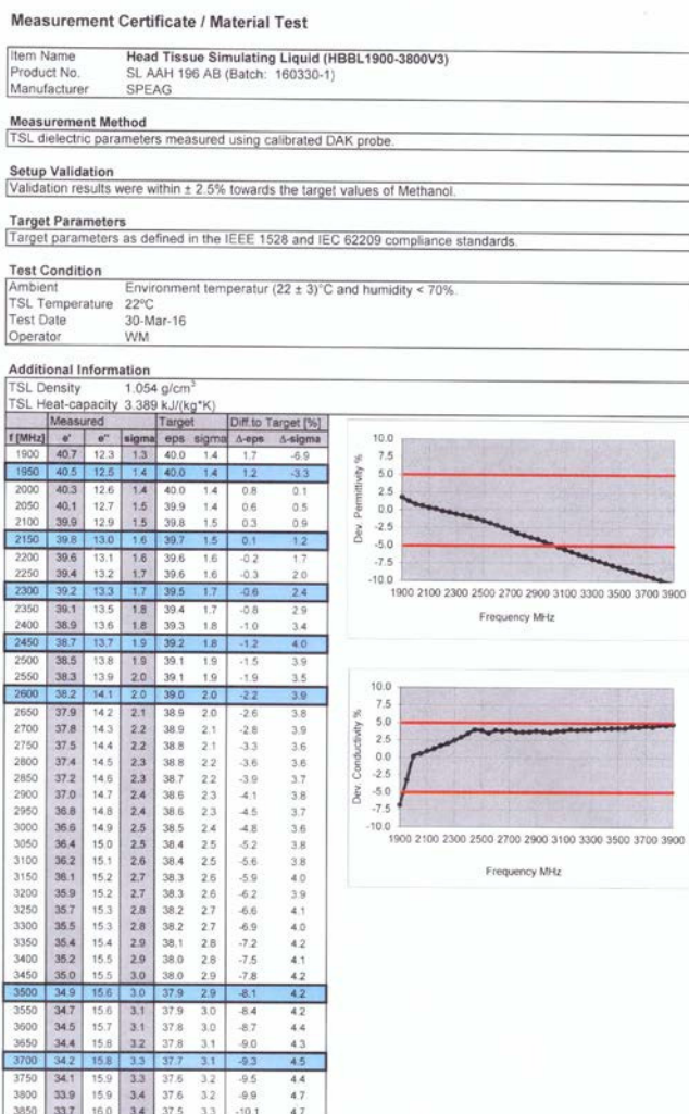
Figure D-2 2.4 GHz Head Tissue Equivalent Matter
