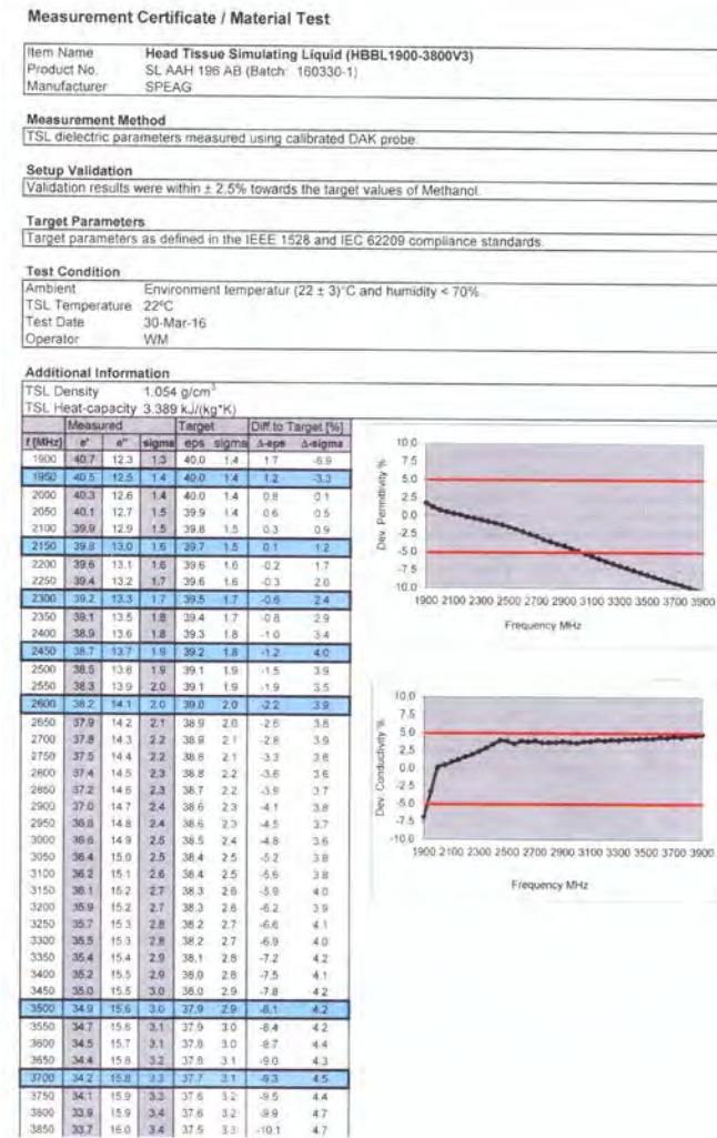
Figure D-5 2.4 GHz Head Tissue Equivalent Matter
