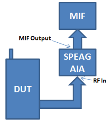
Figure 7-2 MIF Measurement Setup for unlicensed modes
