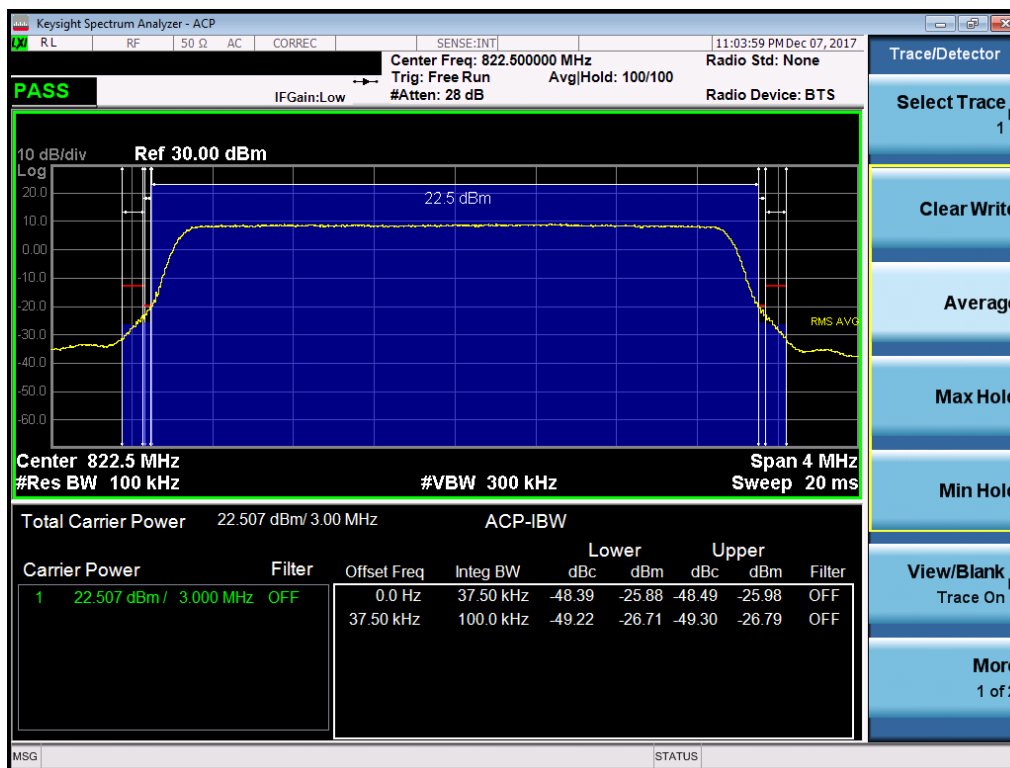
Plot 7-32. Channel Edge Plot (3MHz QPSK – RB Size 15 – High Channel)
