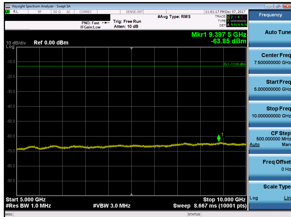
Plot 7-26. Conducted Spurious Plot (3MHz QPSK – RB Size 1, RB Offset 0 – Low Channel)
