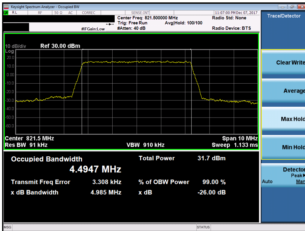
Plot 7-16. Occupied Bandwidth Plot (5MHz QPSK – RB Size 25– High Channel)
