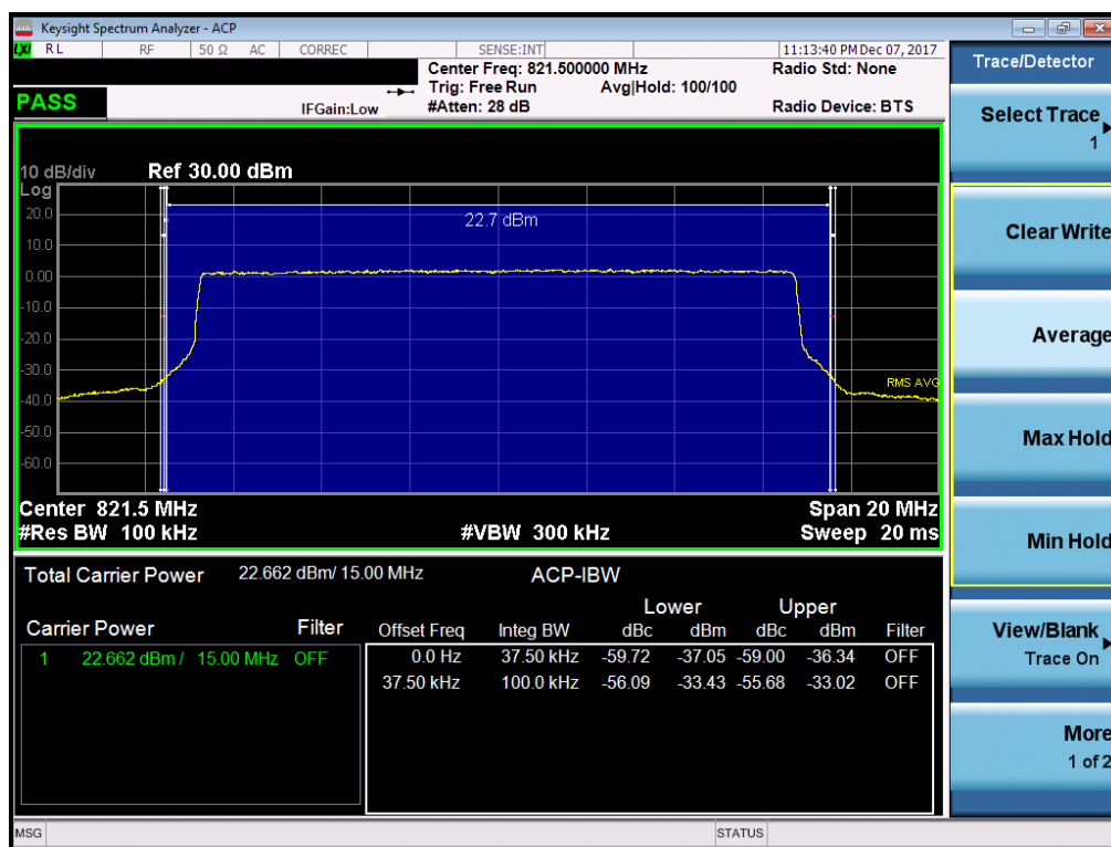
Plot 7-36. Channel Edge Plot (15MHz QPSK – RB Size 75)
