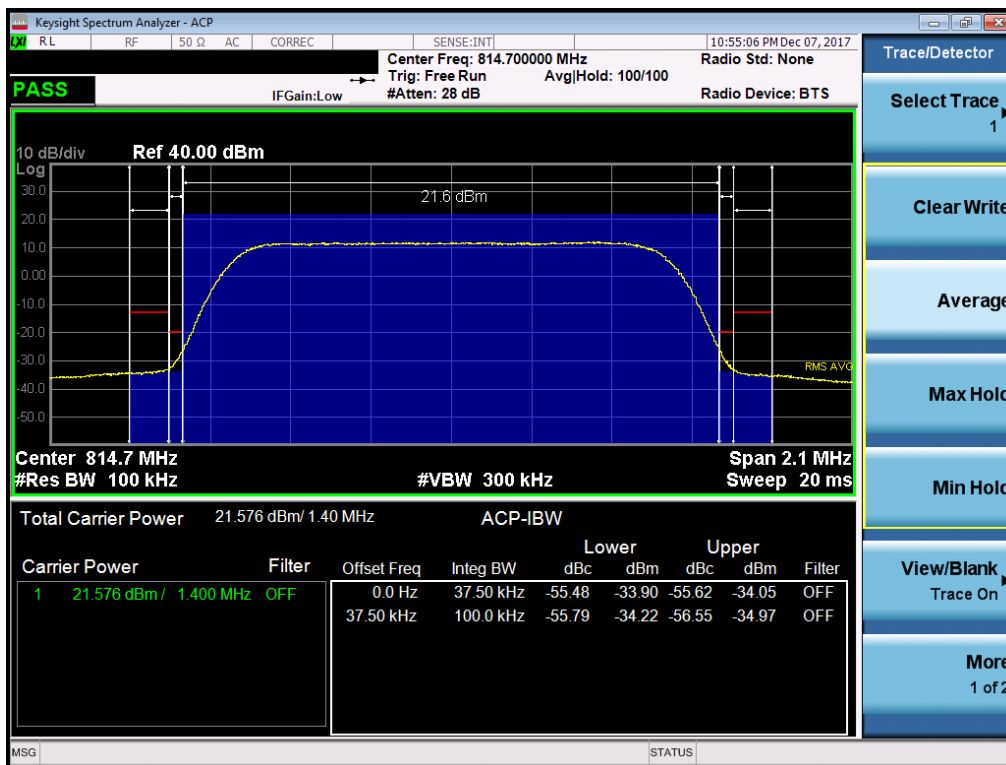
Plot 7-29. Channel Edge Plot (1.4MHz QPSK – RB Size 6– Low Channel)
