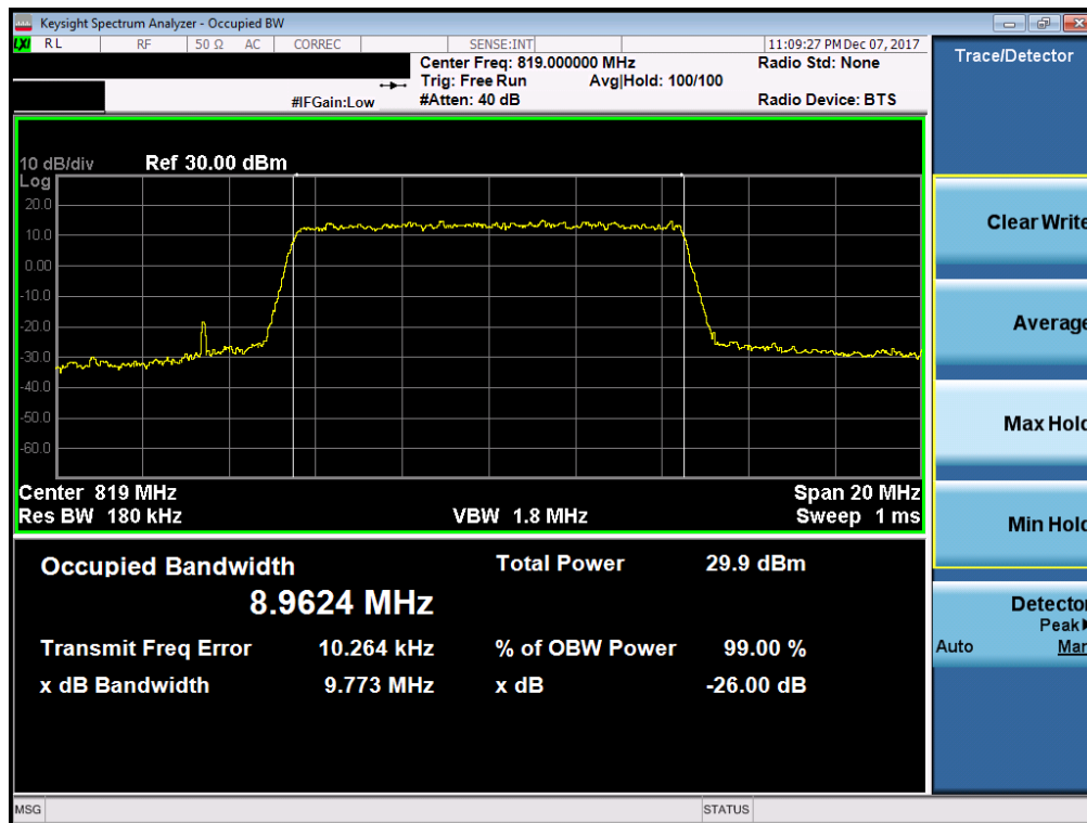
Plot 7-21. Occupied Bandwidth Plot (10MHz 64-QAM – RB Size 50)
