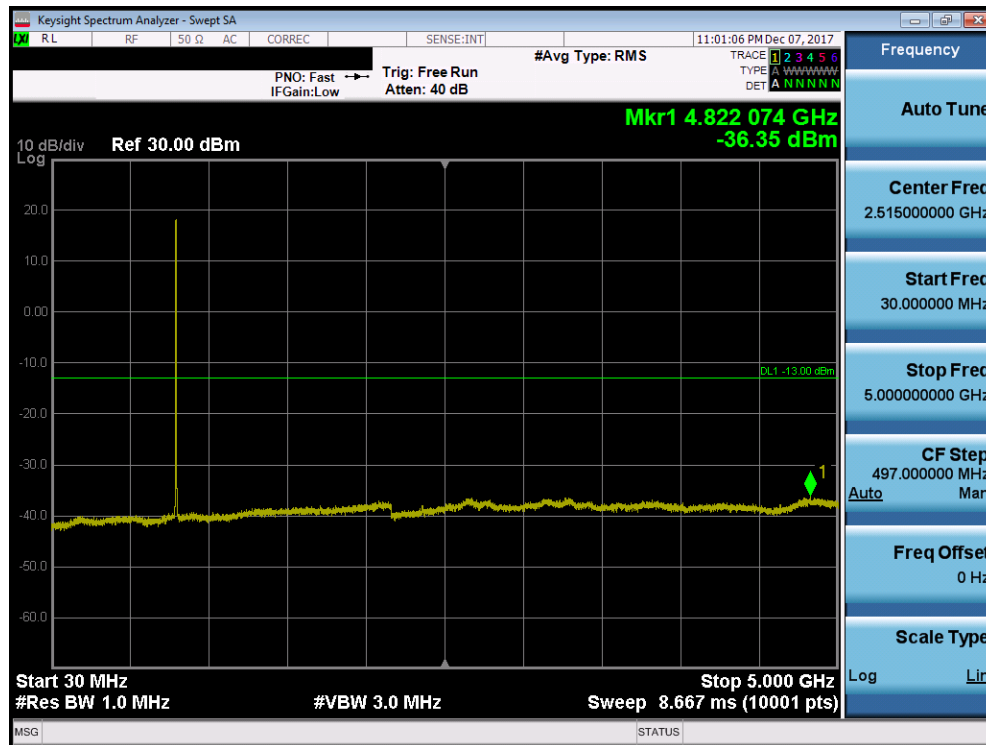
Plot 7-25. Conducted Spurious Plot (3MHz QPSK – RB Size 1, RB Offset 0 – Low Channel)
