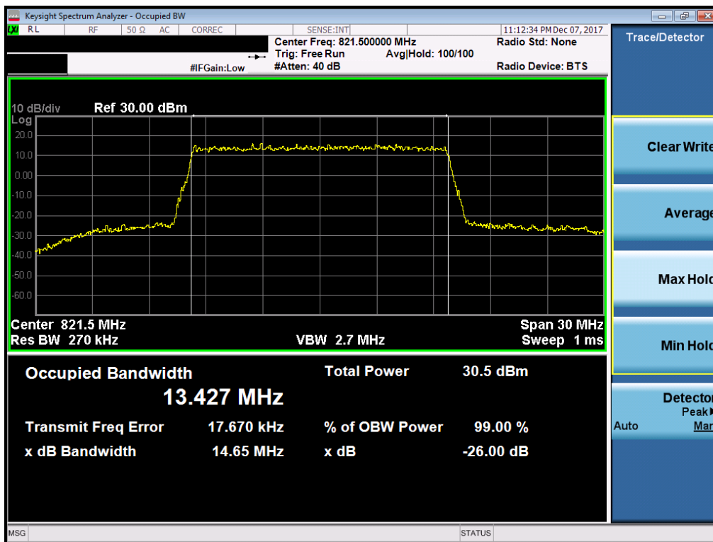
Plot 7-23. Occupied Bandwidth Plot (15MHz 16-QAM – RB Size 75)
