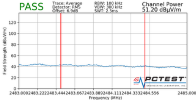
Plot 7-97. Radiated Restricted Band Edge Measurement (Average)
