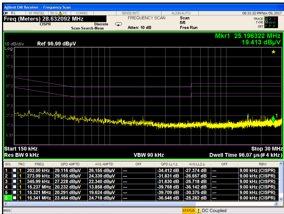
Plot 7-108. Line Conducted Plot with WCP 802.11b (N)
