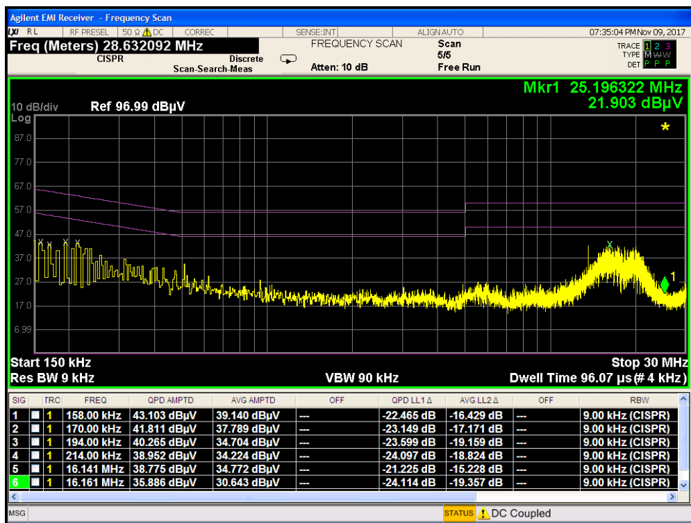
Plot 7-106. Line Conducted Plot 802.11b (N)
