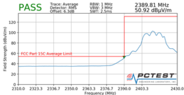
Plot 7-95. Radiated Restricted Band Edge Measurement (Average)
