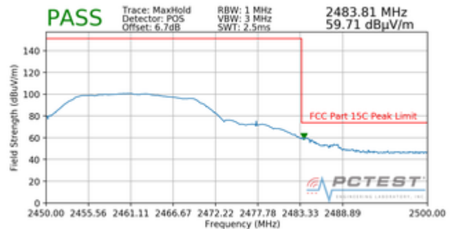
Plot 7-80. Radiated Restricted Upper Band Edge Measurement (Peak)
