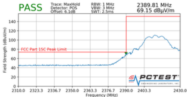
Plot 7-96. Radiated Restricted Band Edge Measurement (Peak)
