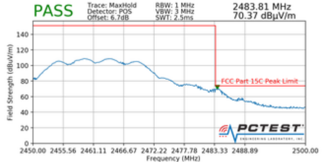
Plot 7-98. Radiated Restricted Band Edge Measurement (Peak)
