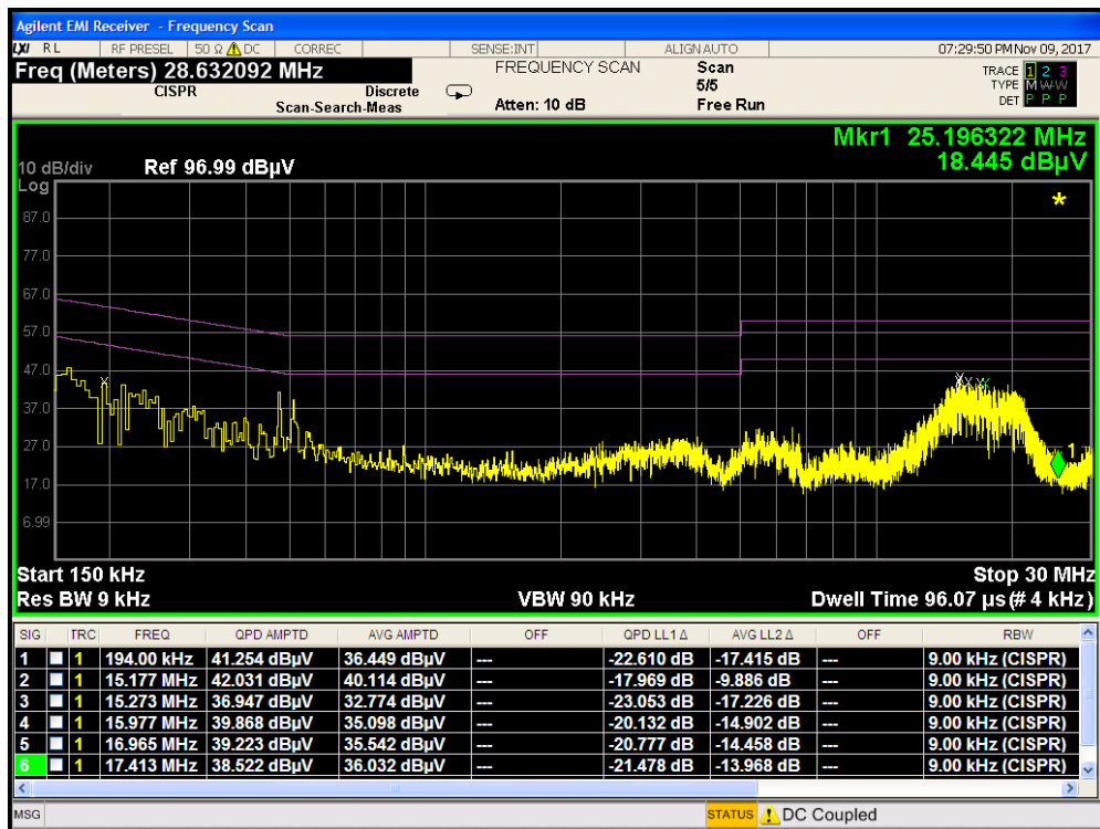
Plot 7-105. Line Conducted Plot 802.11b (L1)
