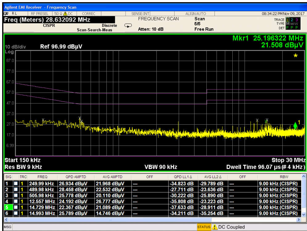
Plot 7-107. Line Conducted Plot with WCP 802.11b (L1)
