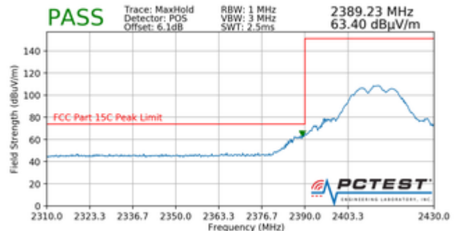
Plot 7-100. Radiated Restricted Band Edge Measurement with WCP (Peak)
