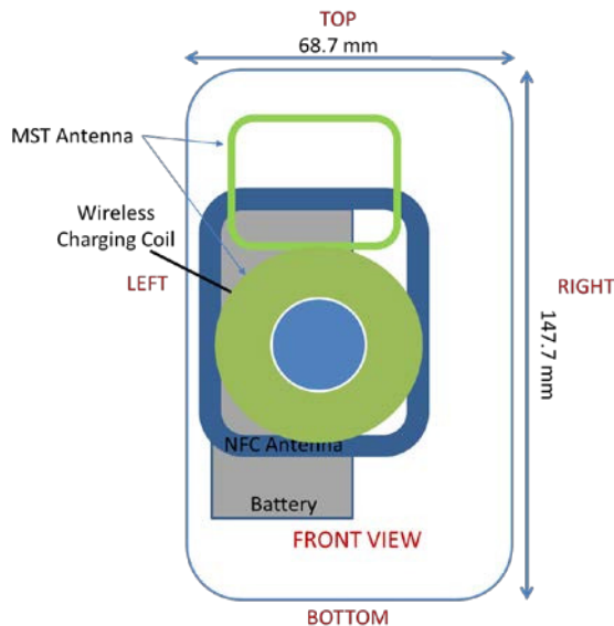
Figure F-2 NFC Antenna Locations
