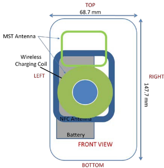
Figure F-2 NFC Antenna Locations
