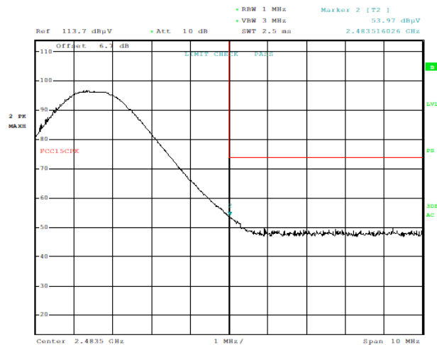
Plot 7-5. Radiated Restricted Upper Band Edge Measurement (Peak)
