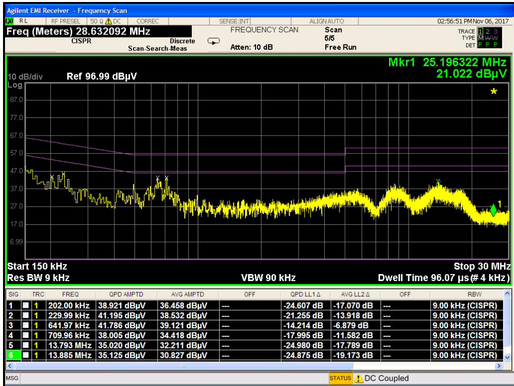
Plot 7-8. Line-Conducted Test Plot (L1)
