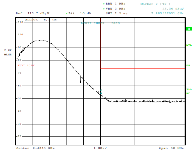
Plot 7-7. Radiated Restricted Upper Band Edge Measurement with WCP (Peak)
