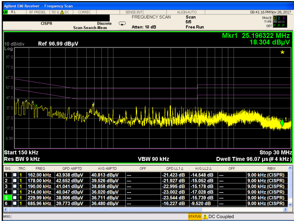
Plot 7-10. Line-Conducted Test Plot with WCP (L1)
