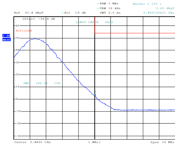
Plot 7-6. Radiated Restricted Upper Band Edge Measurement with WCP (Average)
