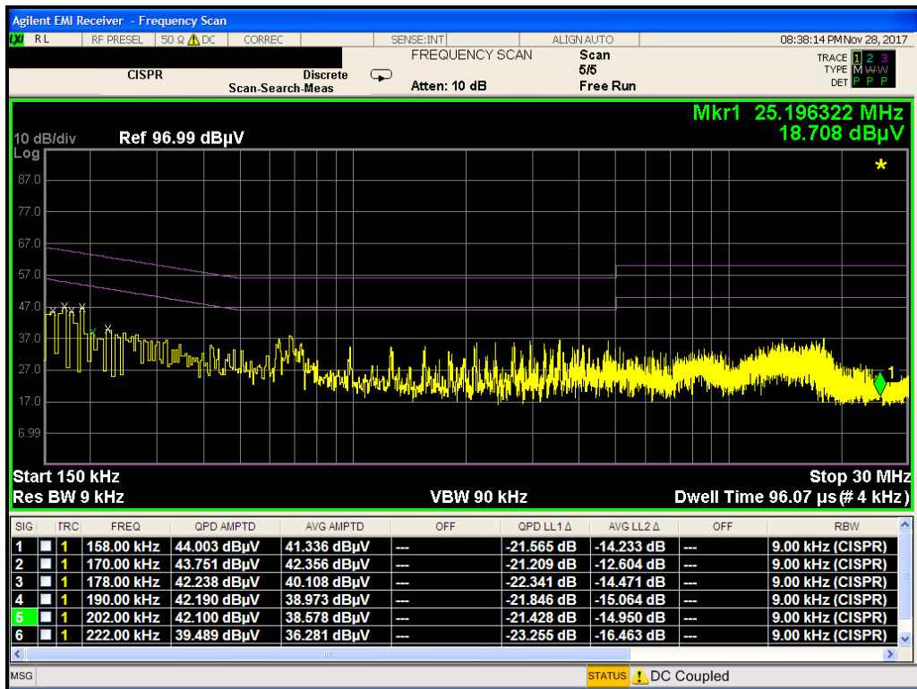
Plot 7-11. Line-Conducted Test Plot with WCP (N)
