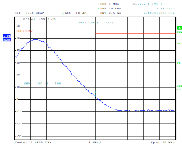
Plot 7-4. Radiated Restricted Upper Band Edge Measurement (Average)
