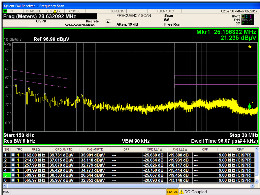
Plot 7-9. Line-Conducted Test Plot (N)
