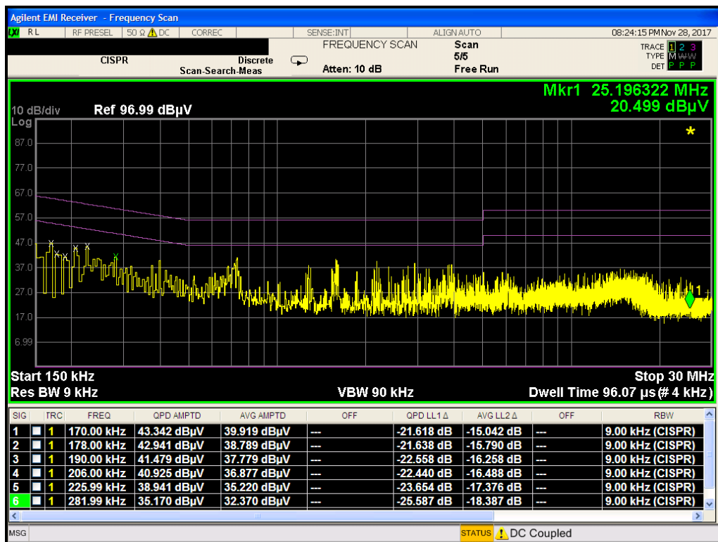
Plot 7-42. Line Conducted Plot with Bluetooth LE (N)
