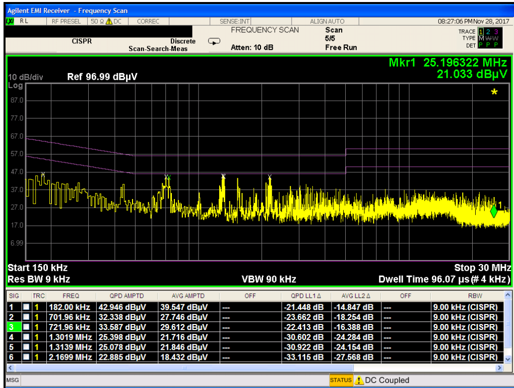
Plot 7-41. Line Conducted Plot with Bluetooth LE (L1)
