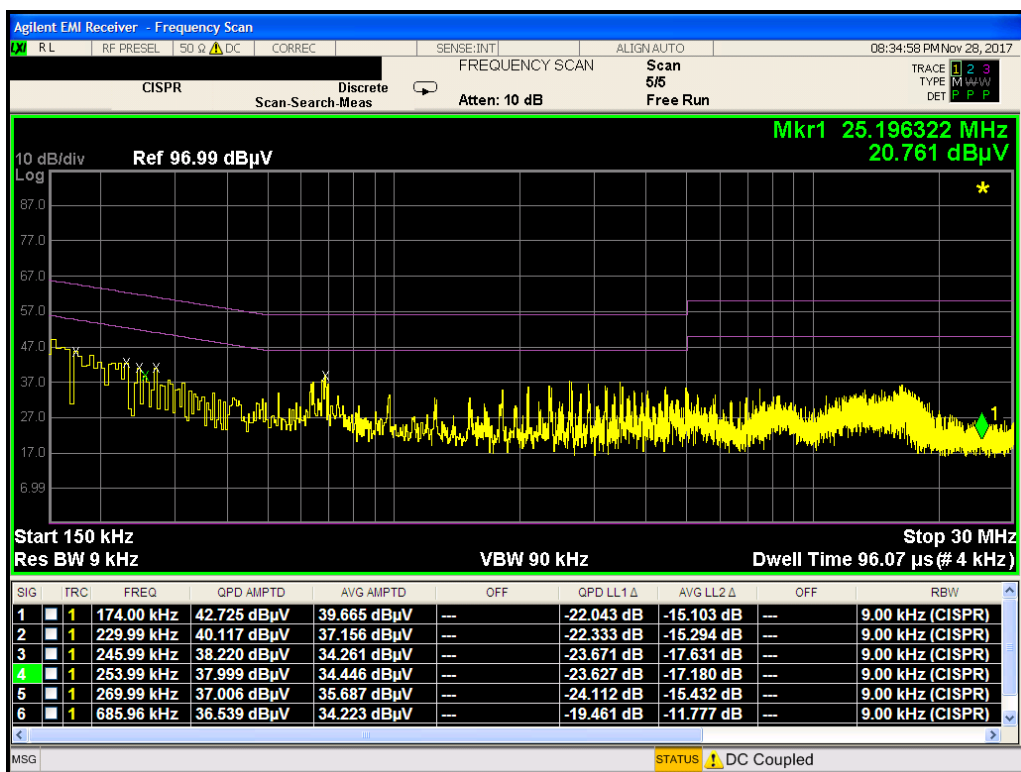
Plot 7-59. Line-Conducted Test Plot with WCP (N)
