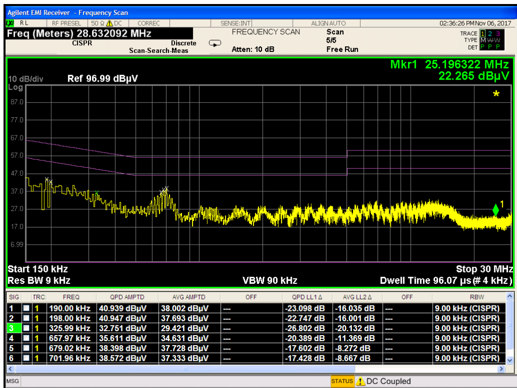
Plot 7-56. Line-Conducted Test Plot (L1)
