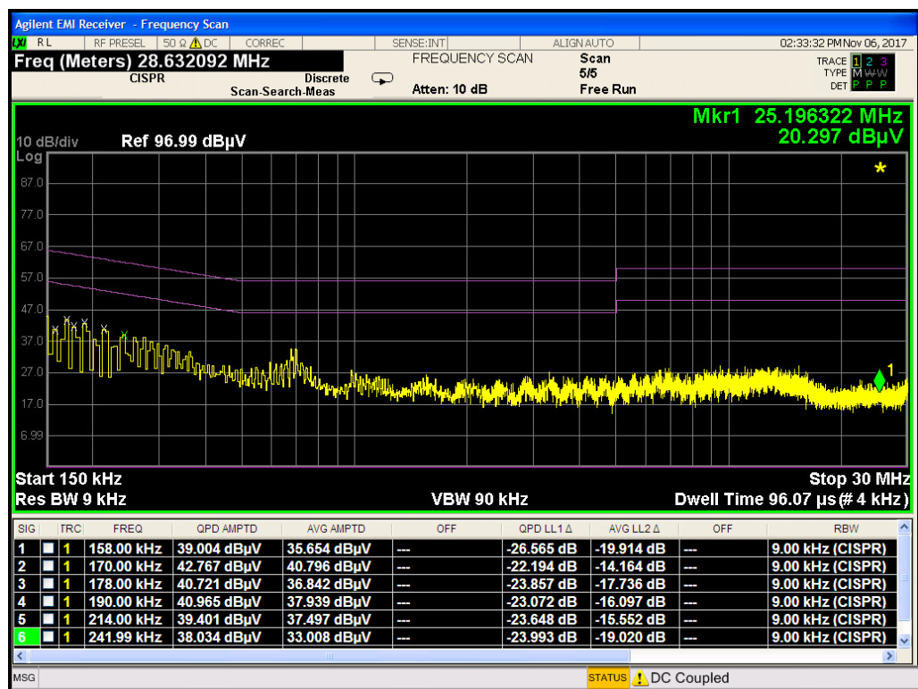
Plot 7-57. Line-Conducted Test Plot (N)
