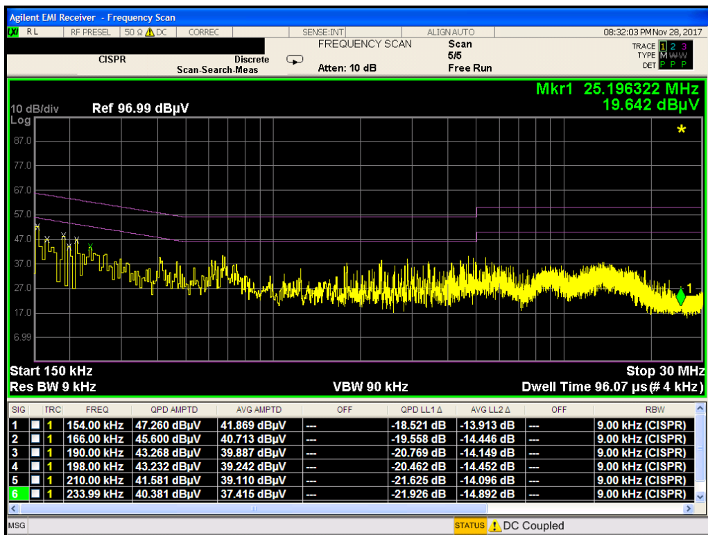
Plot 7-58. Line-Conducted Test Plot with WCP (L1)
