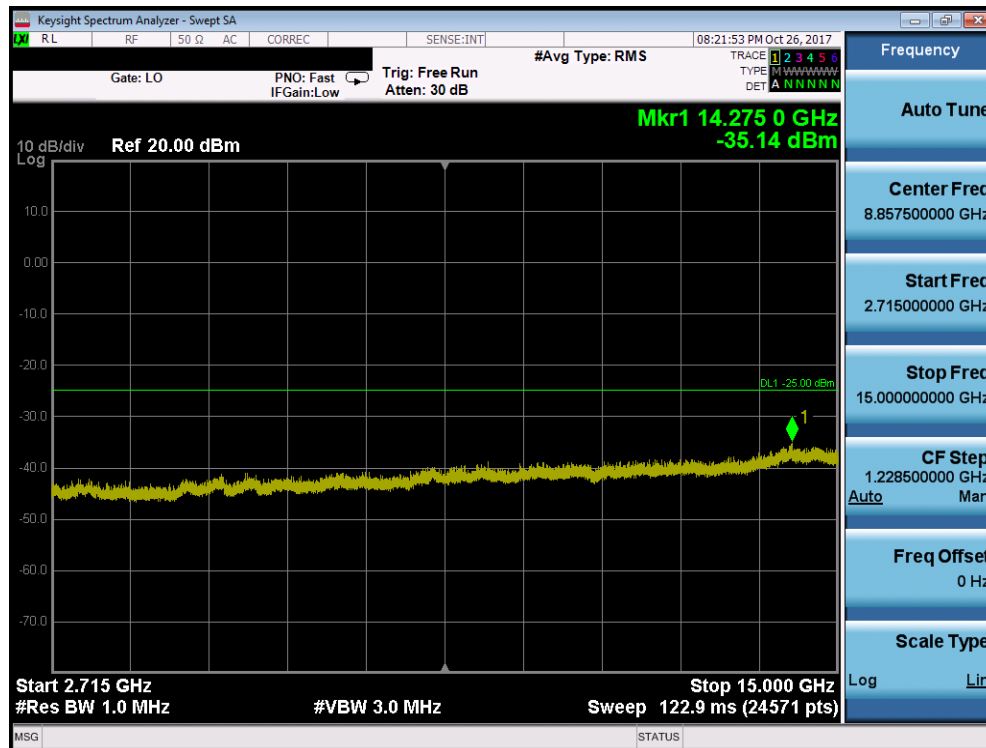
Plot 7-155. Conducted Spurious Plot (Band 38/41 - 20.0MHz QPSK - RB Size 1, RB Offset 0 - High Channel)
