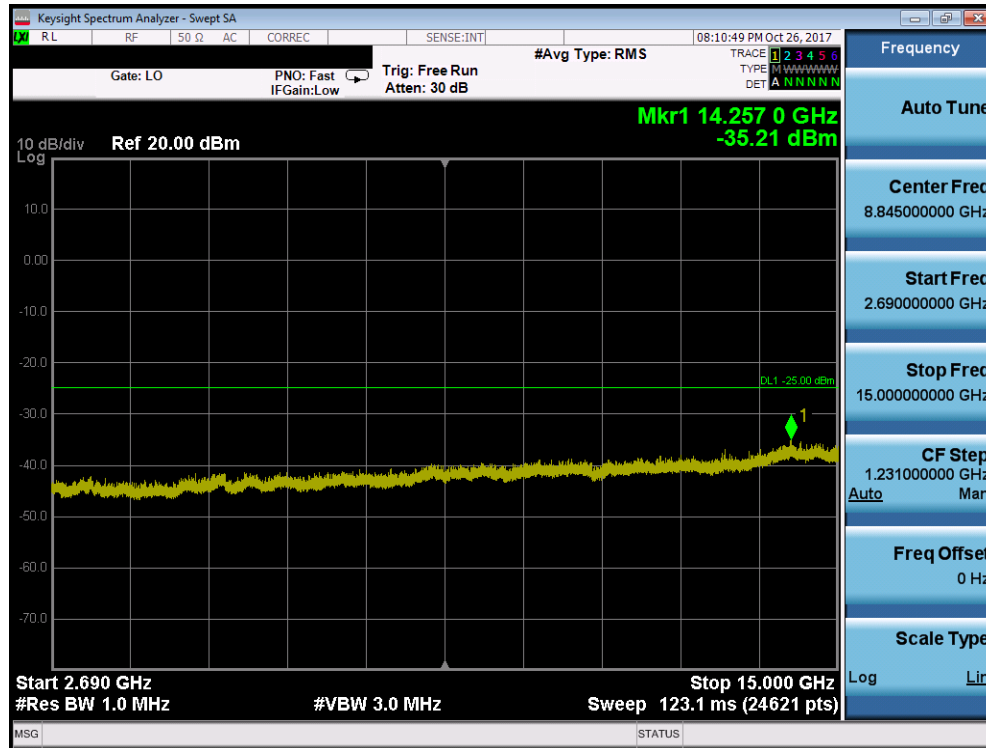
Plot 7-152. Conducted Spurious Plot (Band 38/41 - 20.0MHz QPSK - RB Size 1, RB Offset 0 - Mid Channel)
