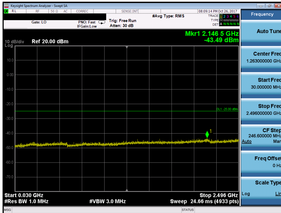
Plot 7-151. Conducted Spurious Plot (Band 38/41 - 20.0MHz QPSK - RB Size 1, RB Offset 0 - Mid Channel)
