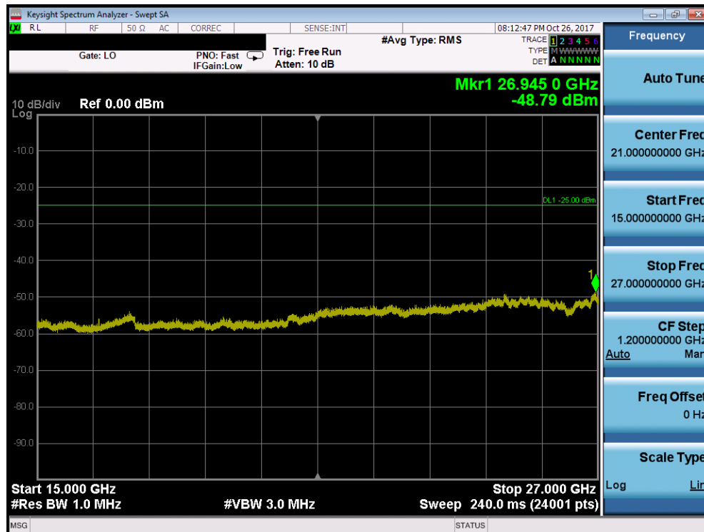
Plot 7-153. Conducted Spurious Plot (Band 38/41 - 20.0MHz QPSK - RB Size 1, RB Offset 0 - Mid Channel)
