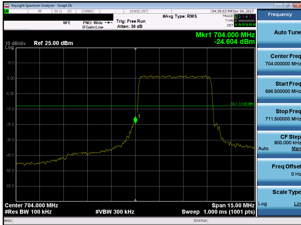
Plot 7-165. Lower Band Edge Plot (Band 17 - 5.0MHz QPSK - Full RB Configuration)
