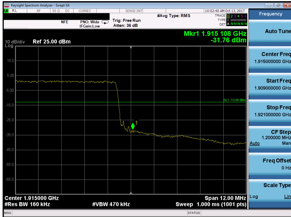
Plot 7-247. Upper Band Edge Plot (Band 25 - 15.0MHz QPSK - Full RB Configuration)
