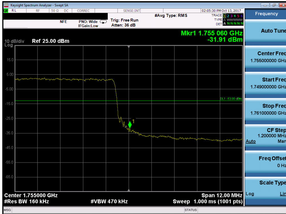
Plot 7-213. Upper Band Edge Plot (Band 4 – 15.0MHz QPSK - Full RB Configuration)
