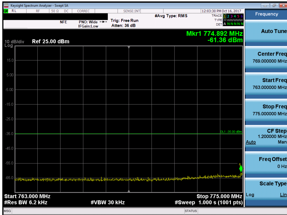
Plot 7-171. Lower Emission Mask Edge Plot (Band 13 – 10.0MHz QPSK – Full RB Configuration)
