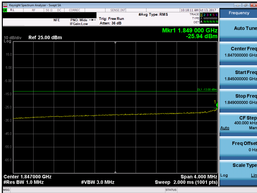
Plot 7-240. Lower Extended Band Edge Plot (Band 2/25 - 10.0MHz QPSK - Full RB Configuration)
