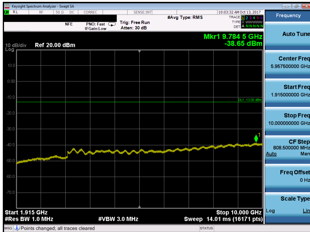
Plot 7-131. Conducted Spurious Plot (Band 2/25 - 15.0MHz QPSK - RB Size 1, RB Offset 0 - Low Channel)
