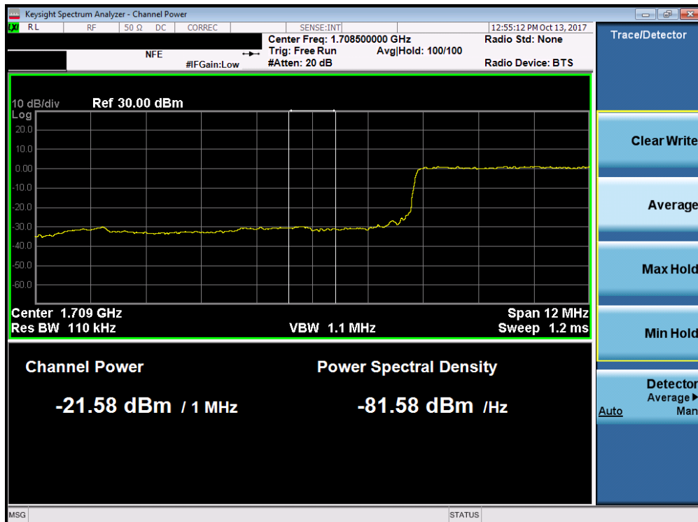
Plot 7-210. Lower Extended Band Edge Plot (Band 4/66 - 15.0MHz QPSK - Full RB Configuration)
