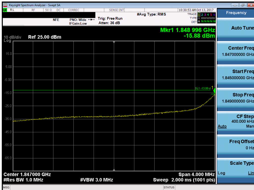
Plot 7-234. Lower Extended Band Edge Plot (Band 2/25 - 5.0MHz QPSK - Full RB Configuration)
