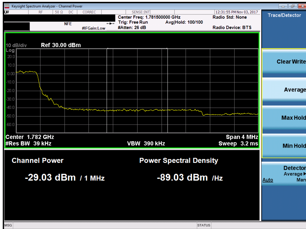
Plot 7-194. Upper Extended Band Edge Plot (Band 66 - 3.0MHz QPSK - Full RB Configuration)
