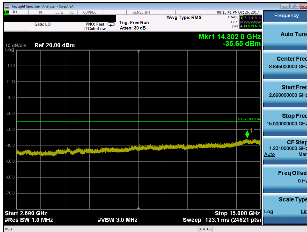
Plot 7-149. Conducted Spurious Plot (Band 38/41 - 20.0MHz QPSK - RB Size 1, RB Offset 0 - Low Channel)
