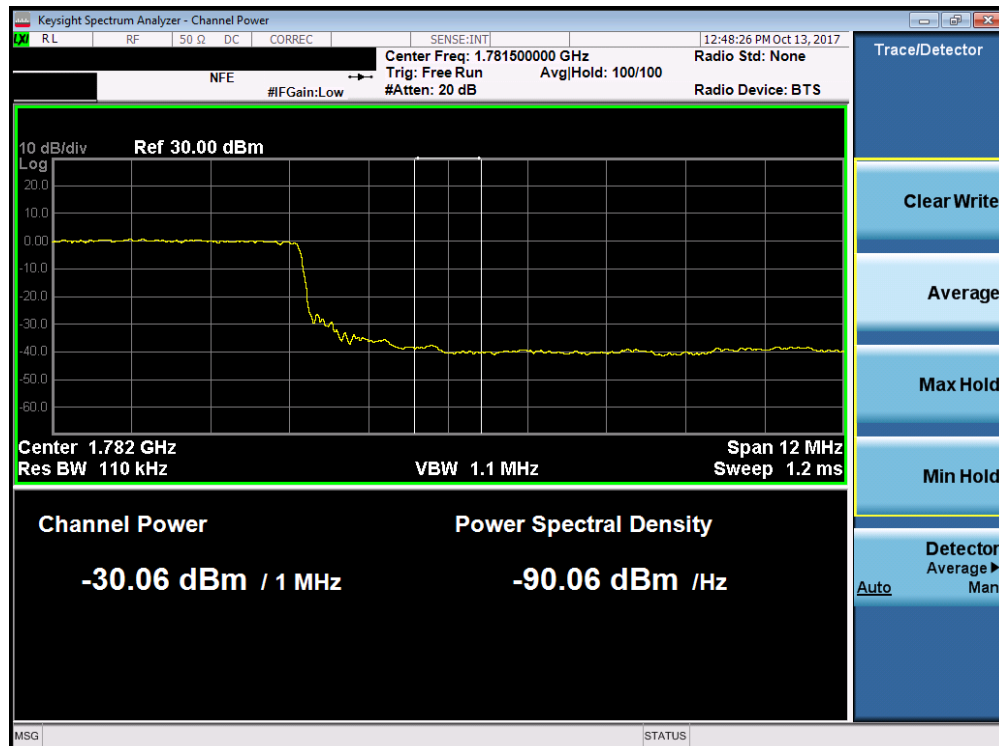
Plot 7-212. Upper Extended Band Edge Plot (Band 66 - 15.0MHz QPSK - Full RB Configuration)
