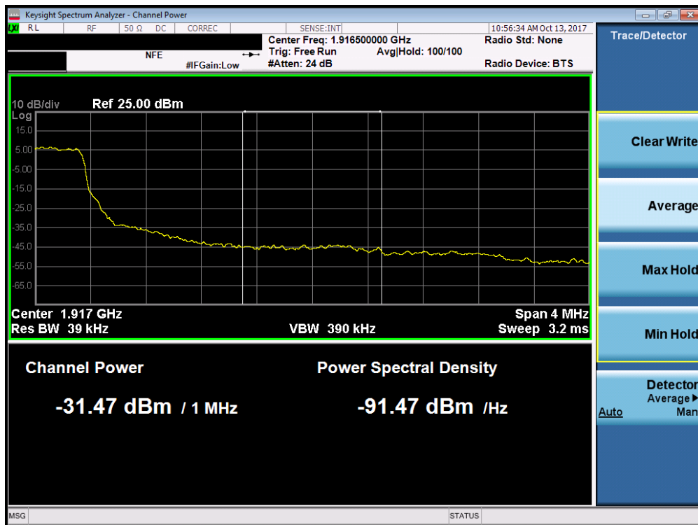
Plot 7-224. Upper Extended Band Edge Plot (Band 25 - 1.4MHz QPSK - Full RB Configuration)
