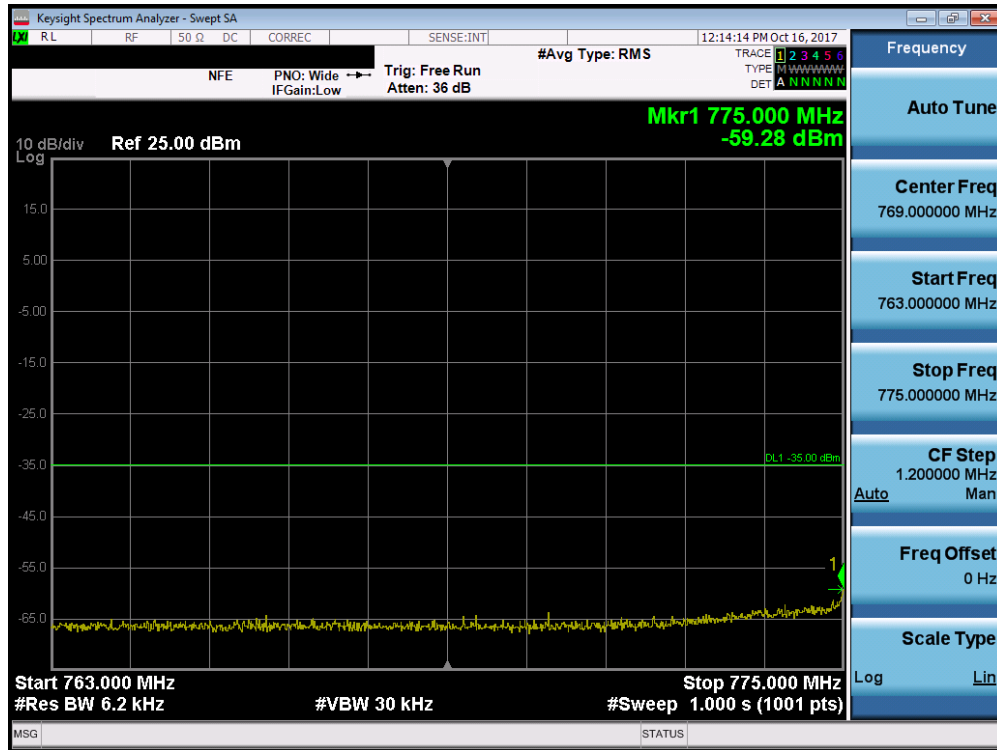
Plot 7-167. Lower Emission Mask Edge Plot (Band 13 – 5.0MHz QPSK – Full RB Configuration)
