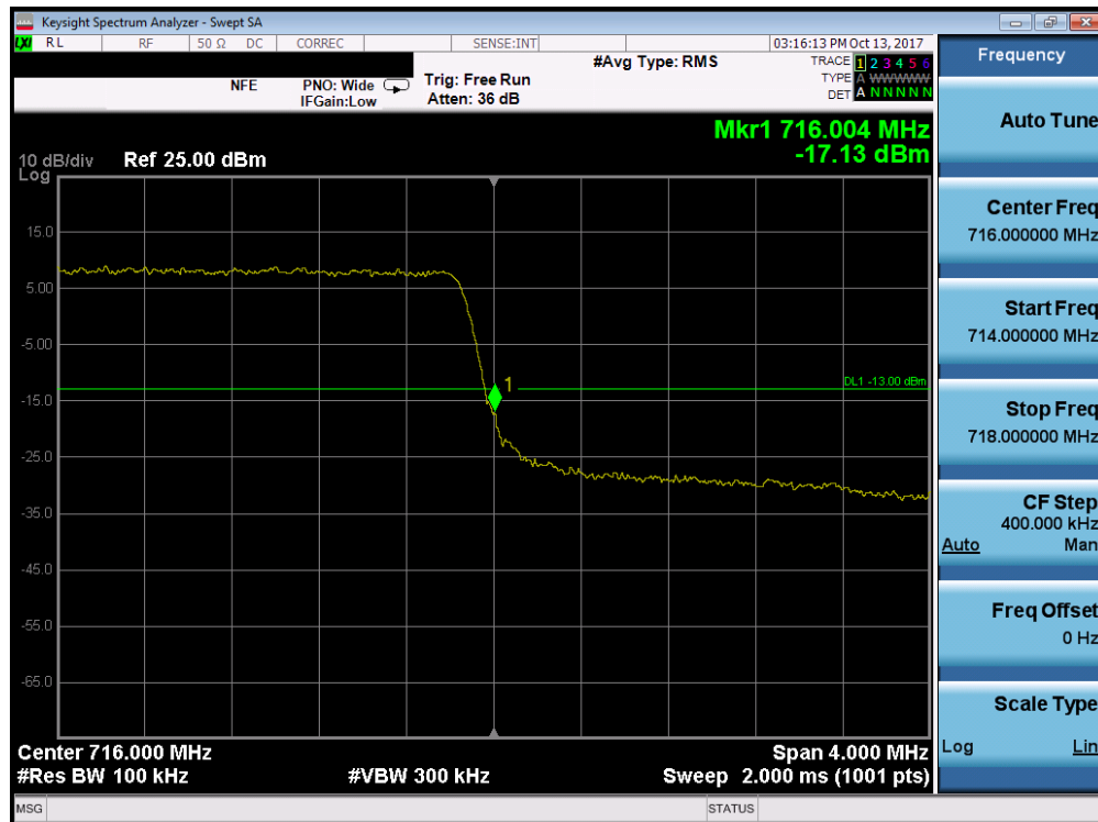
Plot 7-160. Upper Band Edge Plot (Band 12 - 3.0MHz QPSK - Full RB Configuration)
