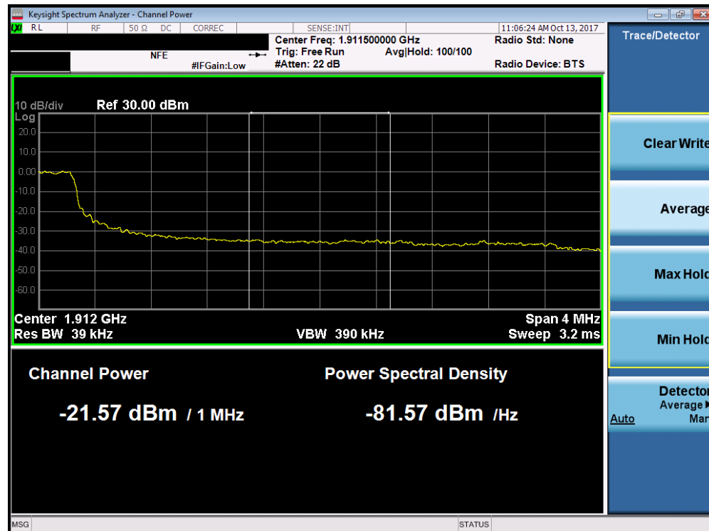
Plot 7-238. Upper Extended Band Edge Plot (Band 2 - 5.0MHz QPSK - Full RB Configuration)
