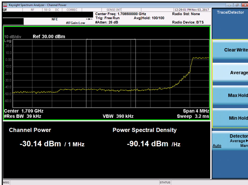
Plot 7-192. Lower Extended Band Edge Plot (Band 4/66 - 3.0MHz QPSK - Full RB Configuration)
