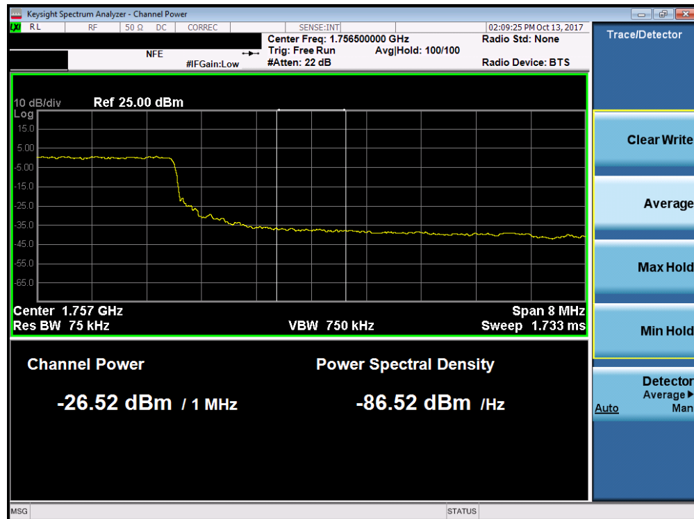
Plot 7-208. Upper Extended Band Edge Plot (Band 4 – 10.0MHz QPSK - Full RB Configuration)
