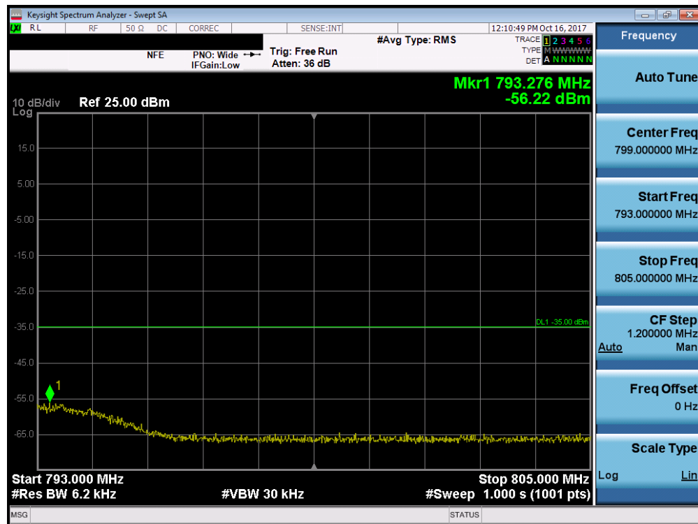
Plot 7-170. Upper Emission Mask Edge Plot (Band 13 - 5.0MHz QPSK - Full RB Configuration)
