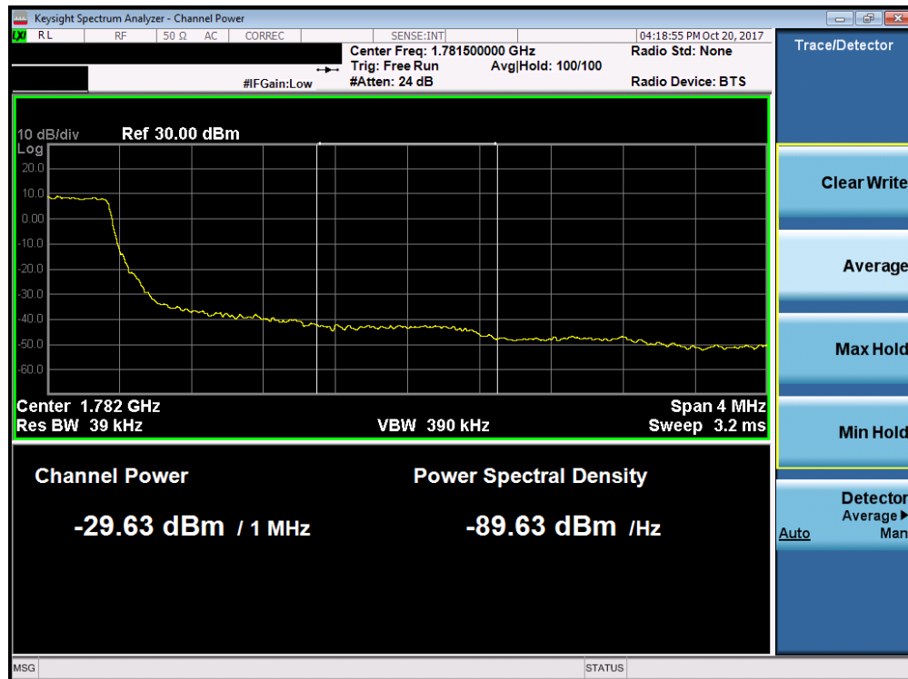
Plot 7-188. Upper Extended Band Edge Plot (Band 66 - 1.4MHz QPSK - Full RB Configuration)
