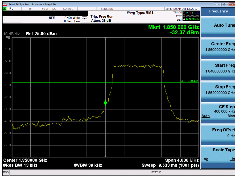
Plot 7-221. Lower Band Edge Plot (Band 2/25 - 1.4MHz QPSK - Full RB Configuration)
