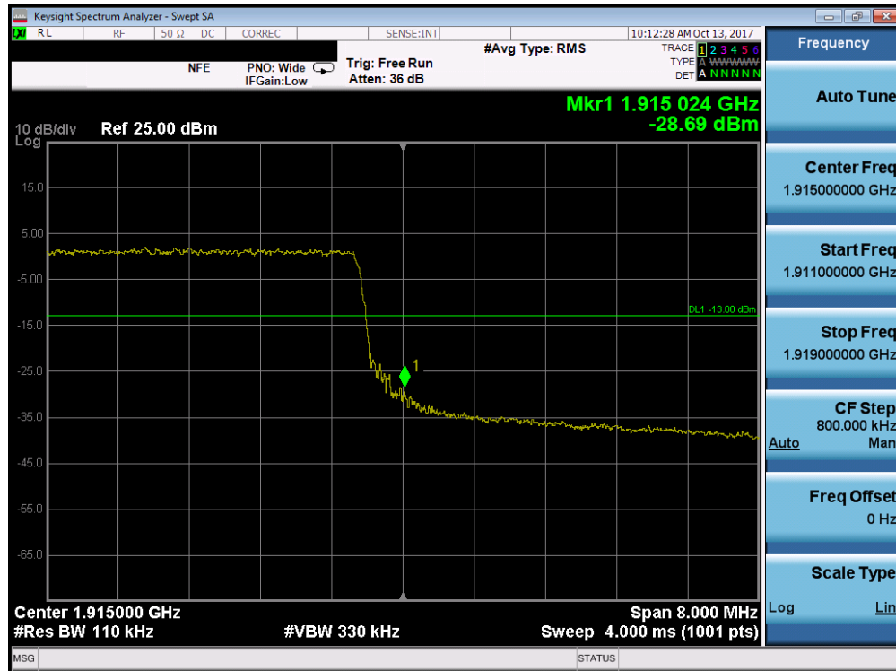
Plot 7-241. Upper Band Edge Plot (Band 25 - 10.0MHz QPSK - Full RB Configuration)
