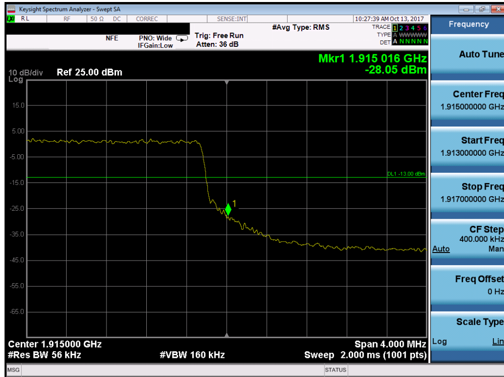
Plot 7-235. Upper Band Edge Plot (Band 25 - 5.0MHz QPSK - Full RB Configuration)
