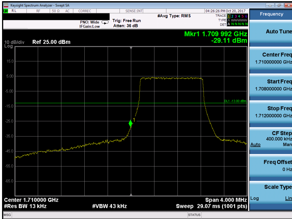
Plot 7-185. Lower Band Edge Plot (Band 4/66 - 1.4MHz QPSK - Full RB Configuration)
