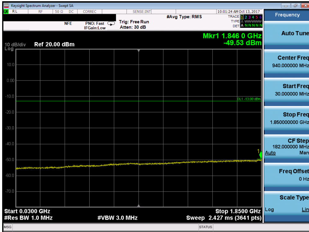
Plot 7-136. Conducted Spurious Plot (Band 2/25 - 15.0MHz QPSK - RB Size 1, RB Offset 0 - High Channel)
