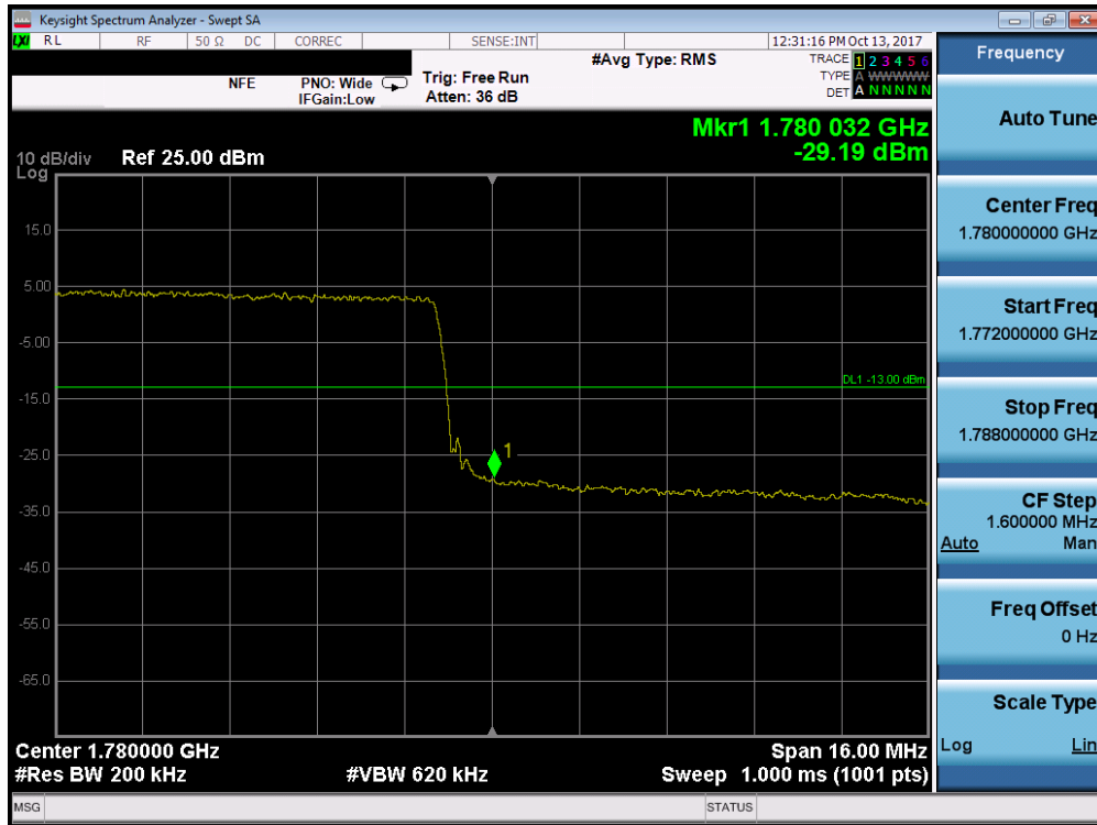
Plot 7-217. Upper Band Edge Plot (Band 66 - 20.0MHz QPSK - Full RB Configuration)
