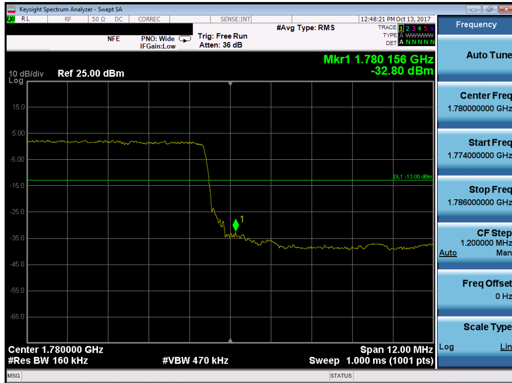
Plot 7-211. Upper Band Edge Plot (Band 66 - 15.0MHz QPSK - Full RB Configuration)
