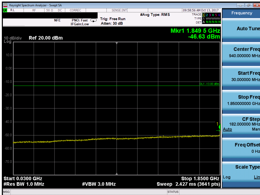
Plot 7-133. Conducted Spurious Plot (Band 2/25 - 15.0MHz QPSK - RB Size 1, RB Offset 0 - Mid Channel)
