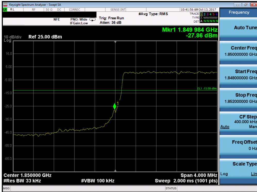
Plot 7-227. Lower Band Edge Plot (Band 2/25 - 3.0MHz QPSK - Full RB Configuration)
