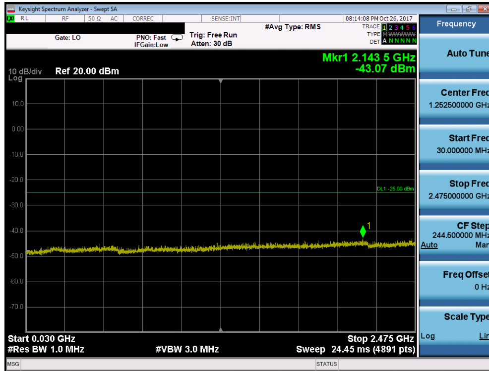
Plot 7-148. Conducted Spurious Plot (Band 38/41 - 20.0MHz QPSK - RB Size 1, RB Offset 0 - Low Channel)
