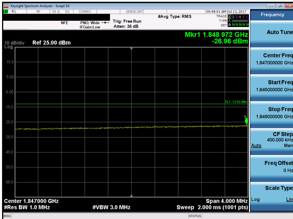
Plot 7-252. Lower Extended Band Edge Plot (Band 2/25 - 20.0MHz QPSK - Full RB Configuration)
