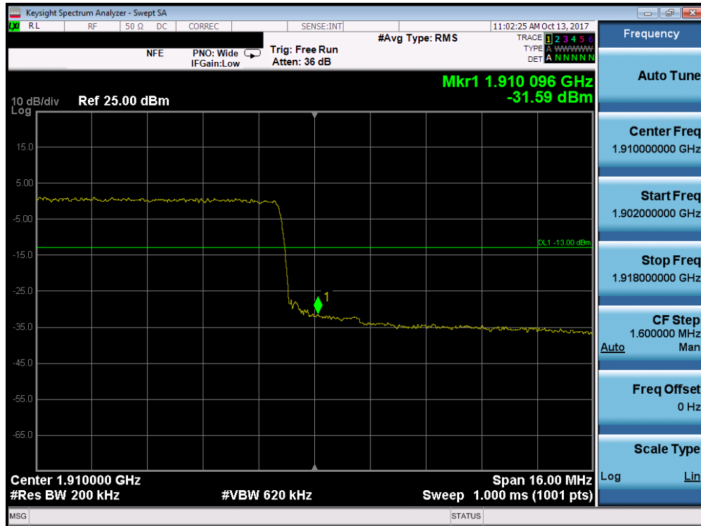
Plot 7-255. Upper Band Edge Plot (Band 2 – 20.0MHz QPSK - Full RB Configuration)
