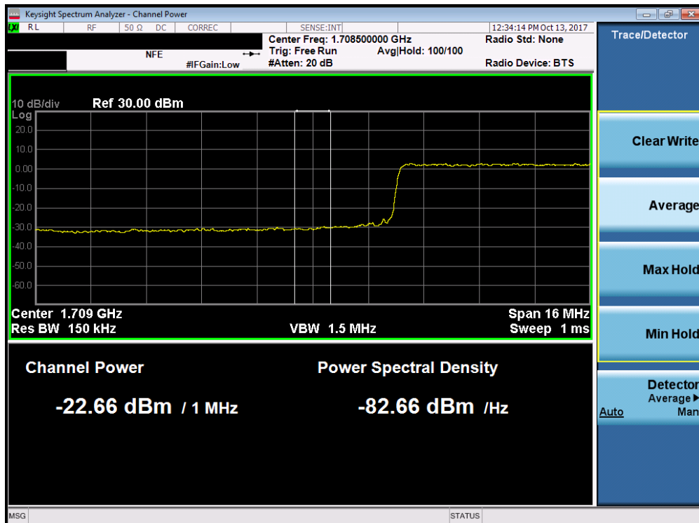
Plot 7-216. Lower Extended Band Edge Plot (Band 4/66 - 20.0MHz QPSK - Full RB Configuration)
