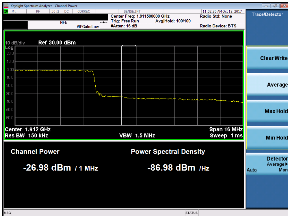
Plot 7-256. Upper Extended Band Edge Plot (Band 2 - 20.0MHz QPSK - Full RB Configuration)
