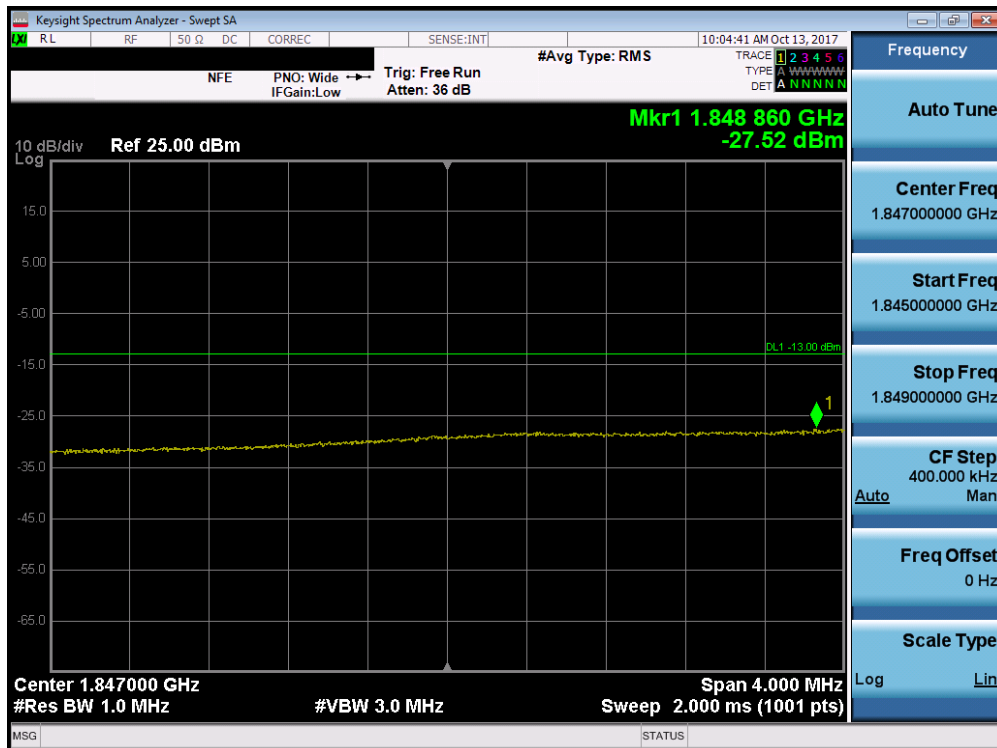
Plot 7-246. Lower Extended Band Edge Plot (Band 2/25 - 15.0MHz QPSK - Full RB Configuration)
