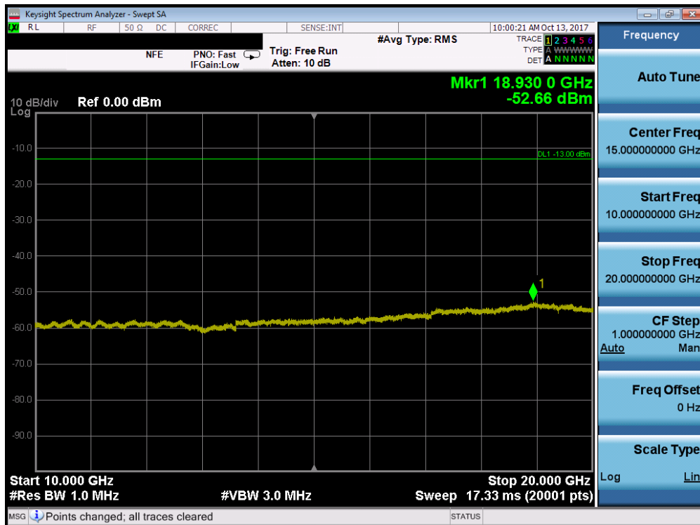
Plot 7-135. Conducted Spurious Plot (Band 2/25 - 15.0MHz QPSK - RB Size 1, RB Offset 0 - Mid Channel)
