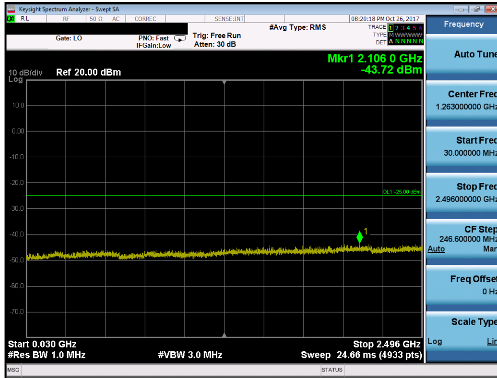
Plot 7-154. Conducted Spurious Plot (Band 38/41 - 20.0MHz QPSK - RB Size 1, RB Offset 0 - High Channel)
