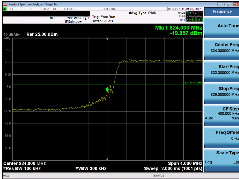
Plot 7-179. Lower Band Edge Plot (Band 5/26 - 5.0MHz QPSK - Full RB Configuration)
