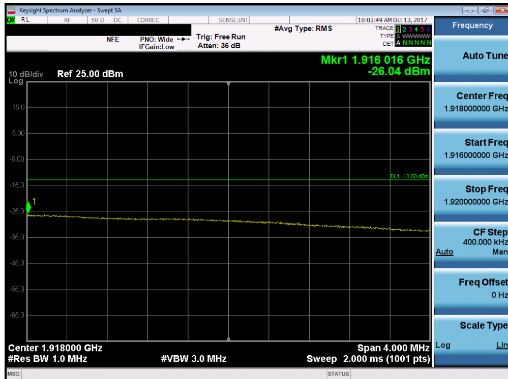
Plot 7-248. Upper Extended Band Edge Plot (Band 25 - 15.0MHz QPSK - Full RB Configuration)
