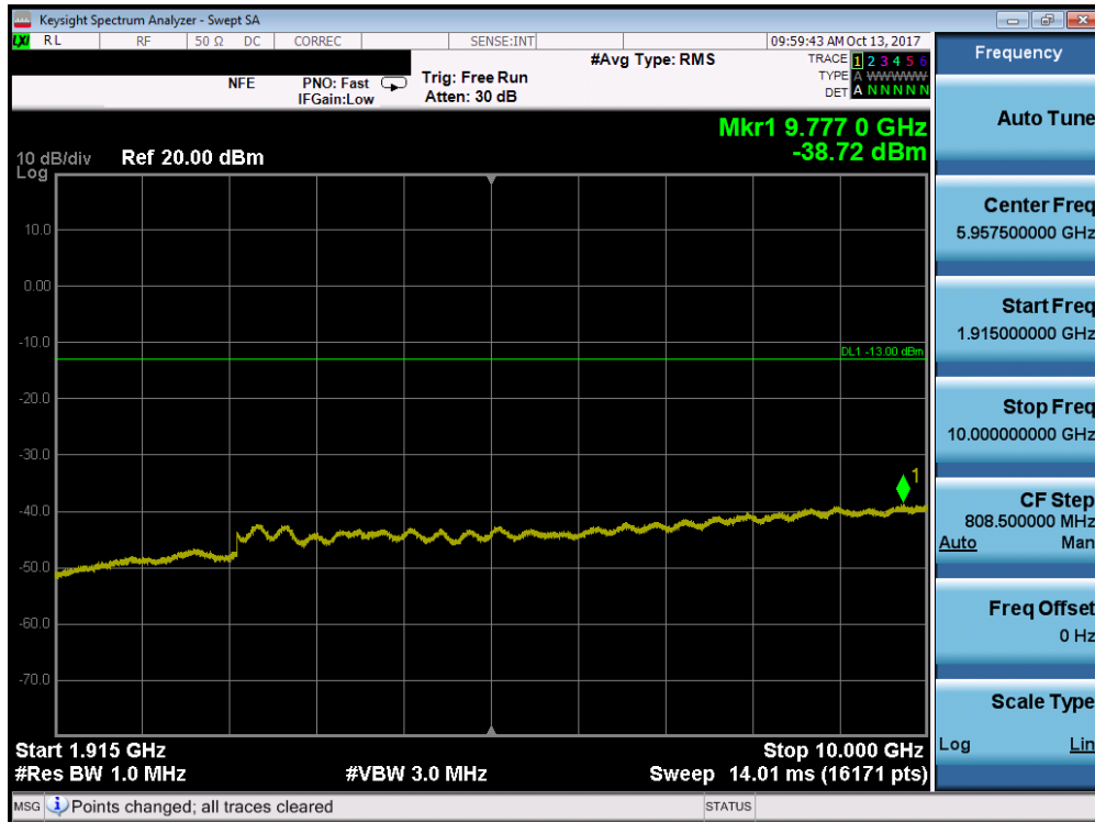
Plot 7-134. Conducted Spurious Plot (Band 2/25 - 15.0MHz QPSK - RB Size 1, RB Offset 0 - Mid Channel)
