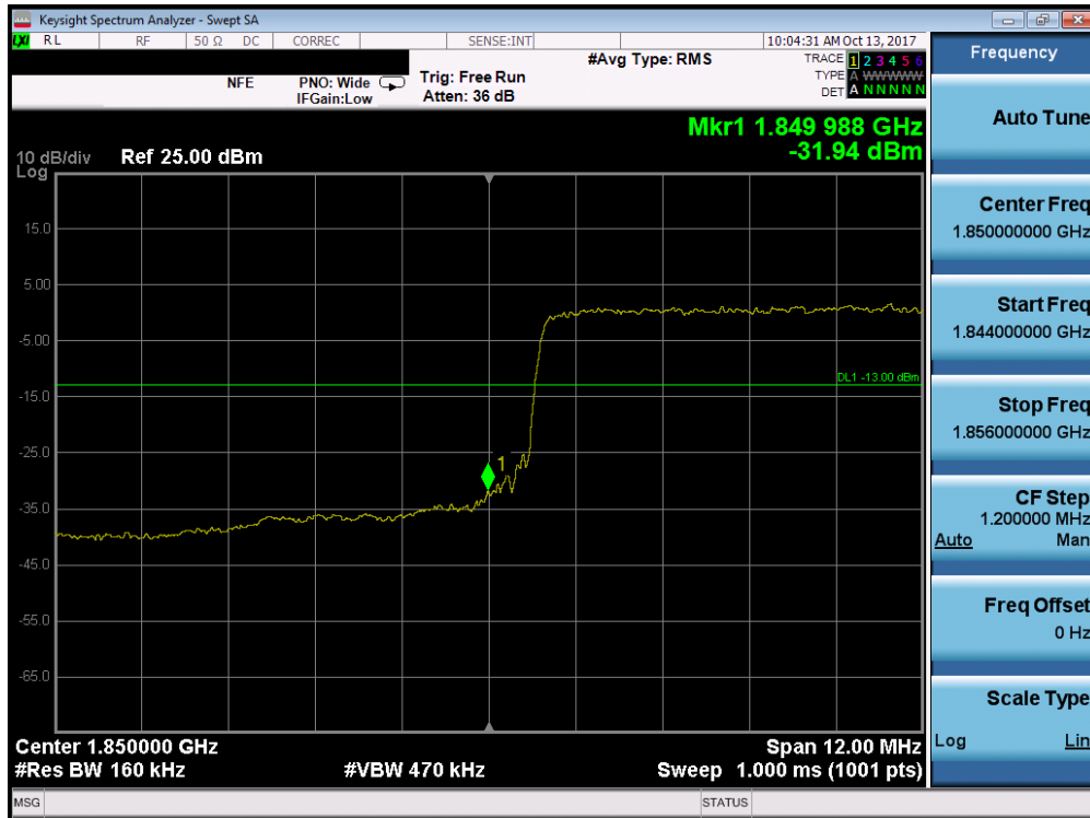
Plot 7-245. Lower Band Edge Plot (Band 2/25 - 15.0MHz QPSK - Full RB Configuration)
