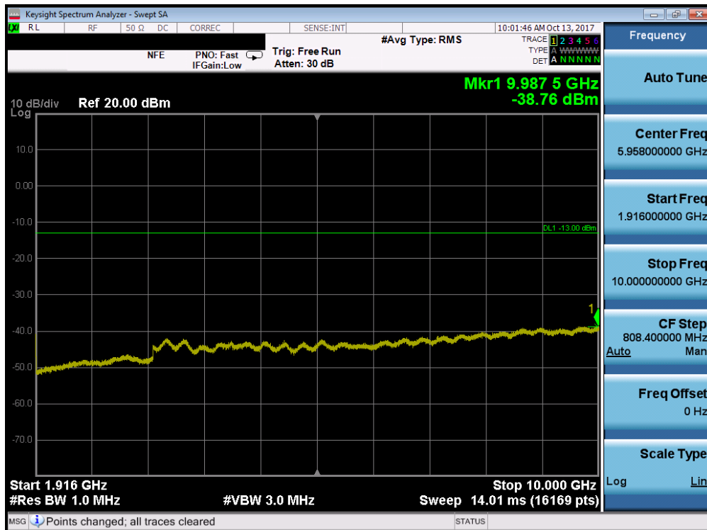
Plot 7-137. Conducted Spurious Plot (Band 2/25 - 15.0MHz QPSK - RB Size 1, RB Offset 0 - High Channel)
