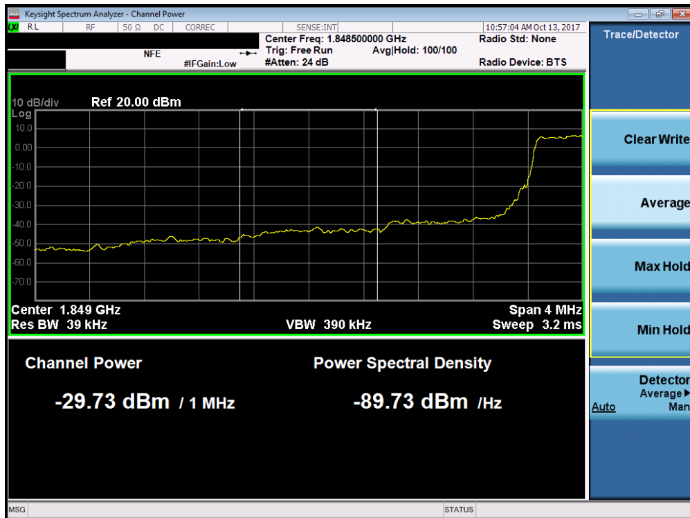
Plot 7-222. Lower Extended Band Edge Plot (Band 2/25 - 1.4MHz QPSK - Full RB Configuration)
