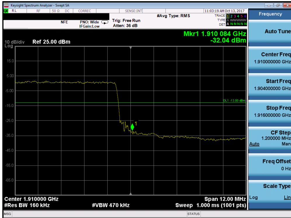
Plot 7-249. Upper Band Edge Plot (Band 2 – 15.0MHz QPSK - Full RB Configuration)
