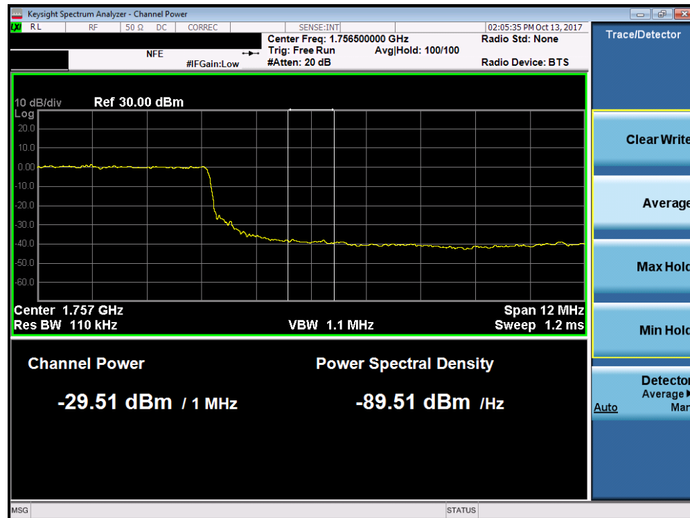
Plot 7-214. Upper Extended Band Edge Plot (Band 4 – 15.0MHz QPSK - Full RB Configuration)
