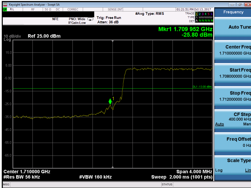
Plot 7-197. Lower Band Edge Plot (Band 4/66 - 5.0MHz QPSK - Full RB Configuration)
