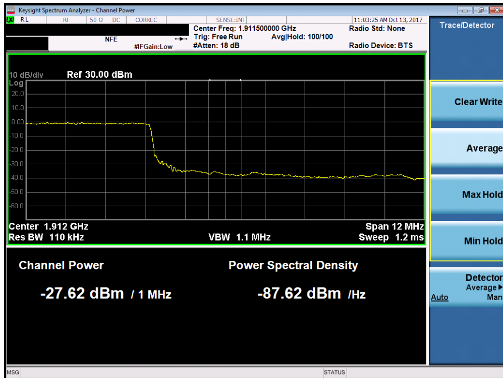
Plot 7-250. Upper Extended Band Edge Plot (Band 2 - 15.0MHz QPSK - Full RB Configuration)
