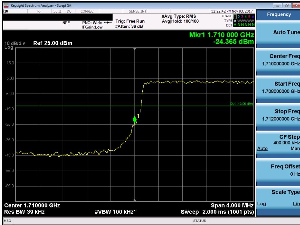
Plot 7-191. Lower Band Edge Plot (Band 4/66 - 3.0MHz QPSK - Full RB Configuration)
