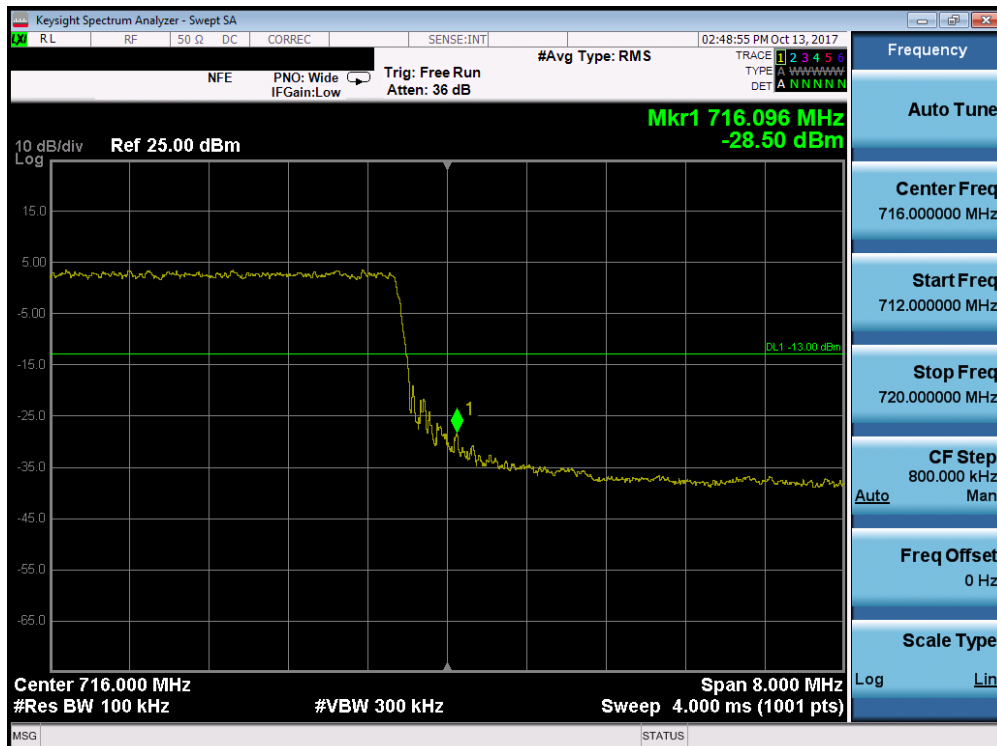
Plot 7-164. Upper Band Edge Plot (Band 12/17 - 10.0MHz QPSK - Full RB Configuration)
