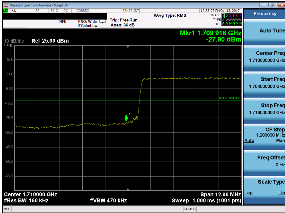
Plot 7-209. Lower Band Edge Plot (Band 4/66 - 15.0MHz QPSK - Full RB Configuration)
