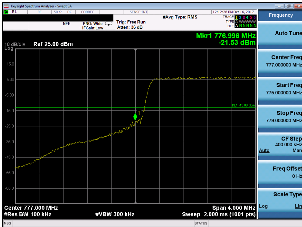
Plot 7-168. Lower Band Edge Plot (Band 13 - 5.0MHz QPSK - Full RB Configuration)
