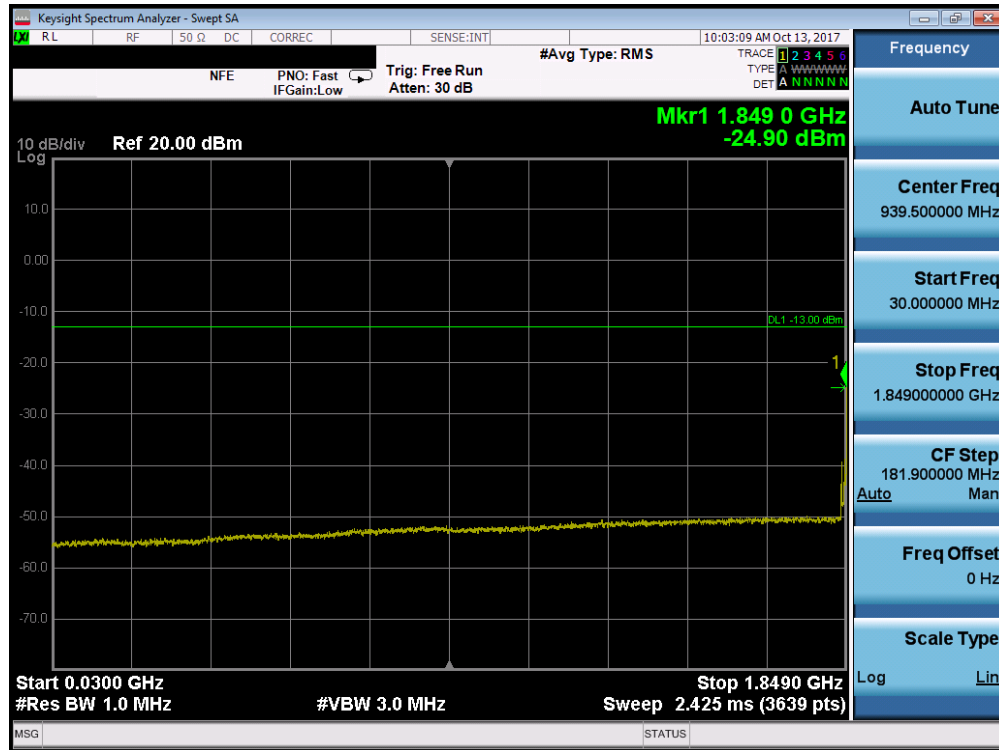
Plot 7-130. Conducted Spurious Plot (Band 2/25 - 15.0MHz QPSK - RB Size 1, RB Offset 0 - Low Channel)
