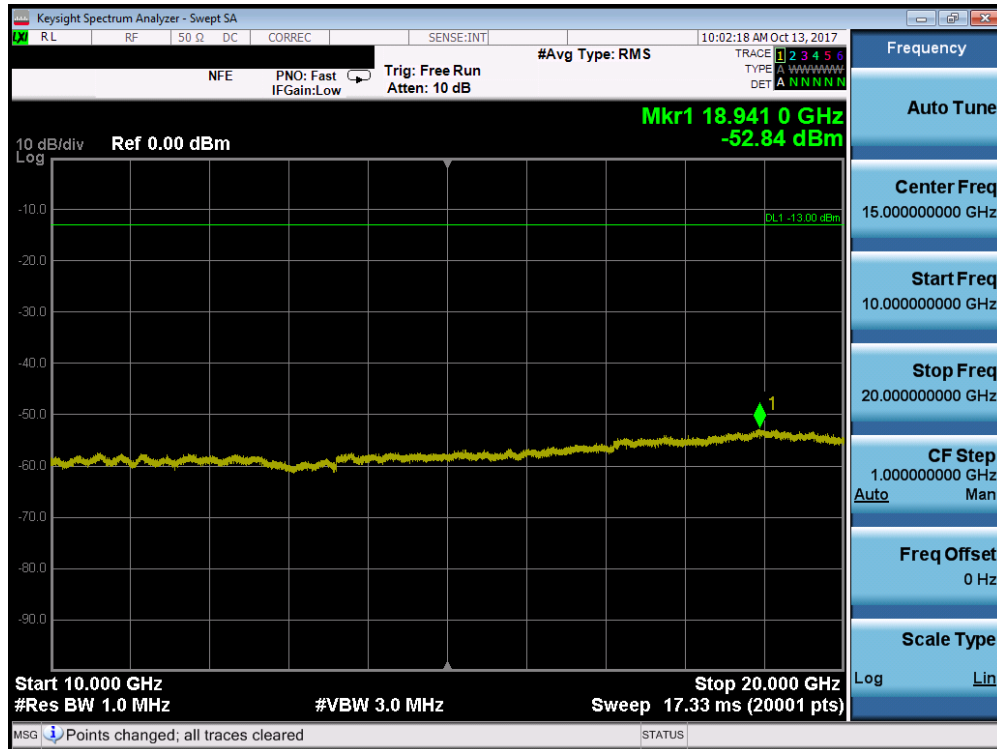
Plot 7-138. Conducted Spurious Plot (Band 2/25 - 15.0MHz QPSK - RB Size 1, RB Offset 0 - High Channel)
