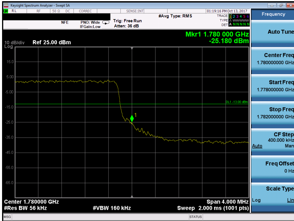
Plot 7-199. Upper Band Edge Plot (Band 66 - 5.0MHz QPSK - Full RB Configuration)
