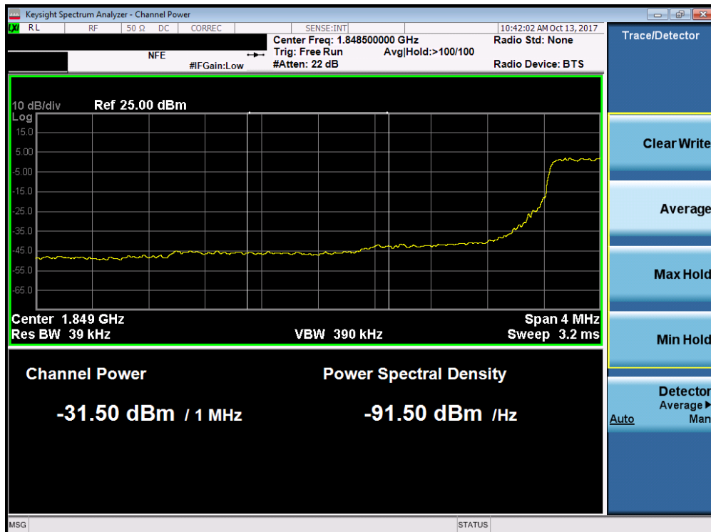
Plot 7-228. Lower Extended Band Edge Plot (Band 2/25 - 3.0MHz QPSK - Full RB Configuration)
