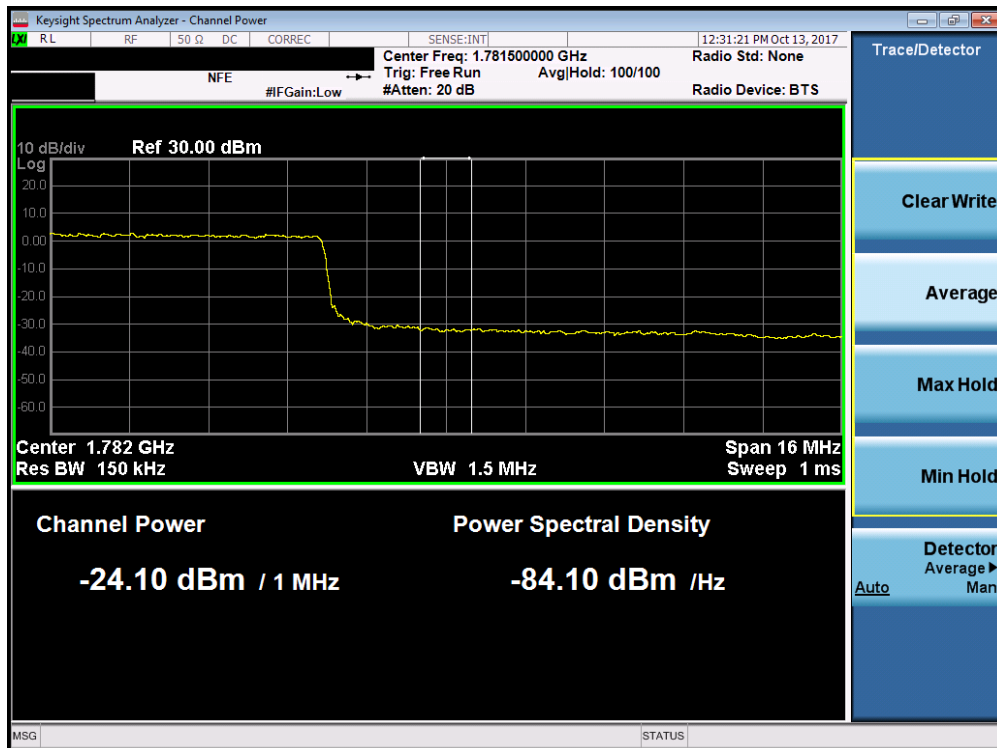
Plot 7-218. Upper Extended Band Edge Plot (Band 66 - 20.0MHz QPSK - Full RB Configuration)
