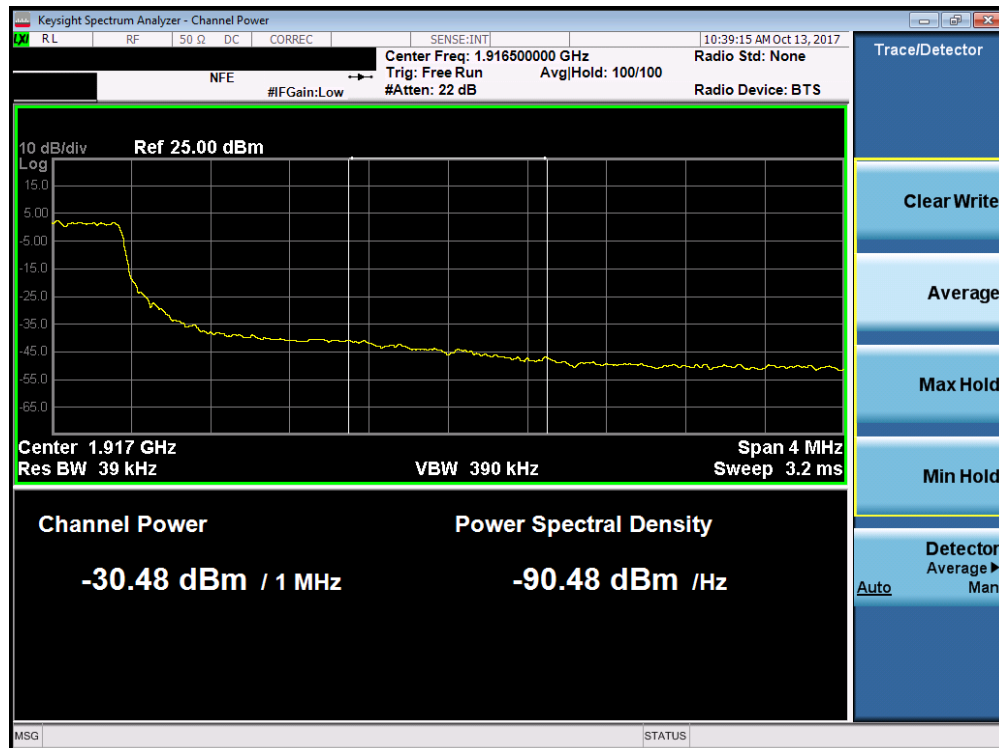
Plot 7-230. Upper Extended Band Edge Plot (Band 25 - 3.0MHz QPSK - Full RB Configuration)
