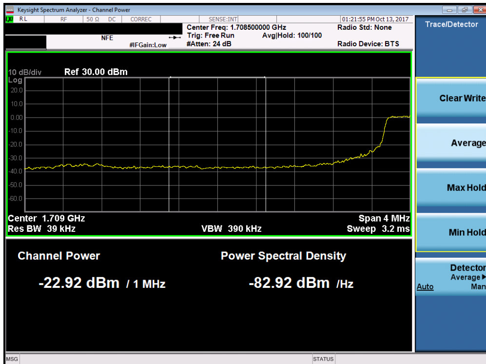
Plot 7-198. Lower Extended Band Edge Plot (Band 4/66 - 5.0MHz QPSK - Full RB Configuration)
