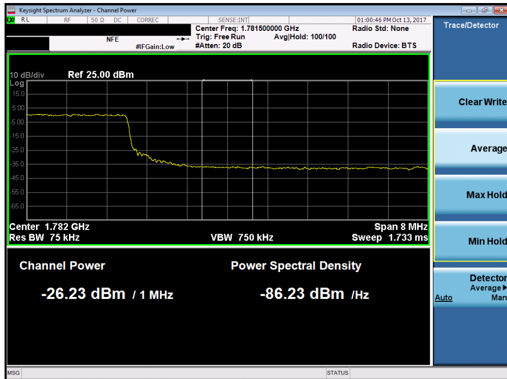
Plot 7-206. Upper Extended Band Edge Plot (Band 66 - 10.0MHz QPSK - Full RB Configuration)
