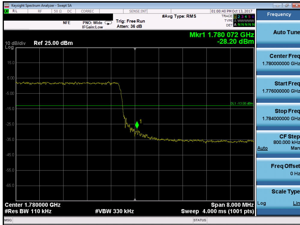
Plot 7-205. Upper Band Edge Plot (Band 66 - 10.0MHz QPSK - Full RB Configuration)
