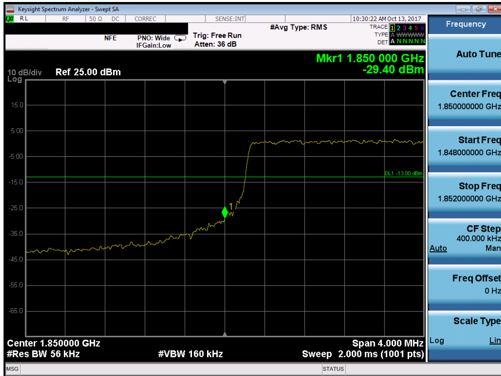
Plot 7-233. Lower Band Edge Plot (Band 2/25 - 5.0MHz QPSK - Full RB Configuration)
