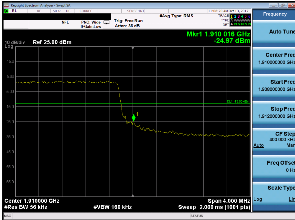
Plot 7-237. Upper Band Edge Plot (Band 2 – 5.0MHz QPSK - Full RB Configuration)
