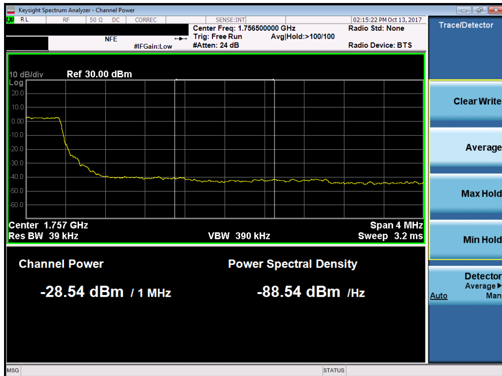
Plot 7-196. Upper Extended Band Edge Plot (Band 4 - 3.0MHz QPSK - Full RB Configuration)
