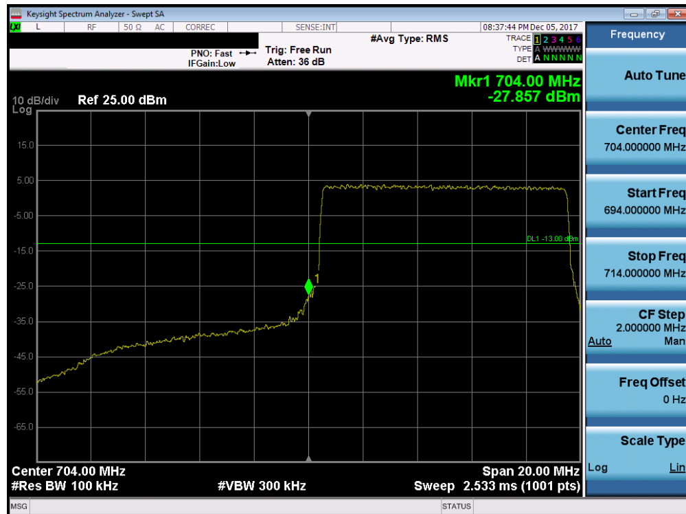
Plot 7-166. Lower Band Edge Plot (Band 17 - 10.0MHz QPSK - Full RB Configuration)
