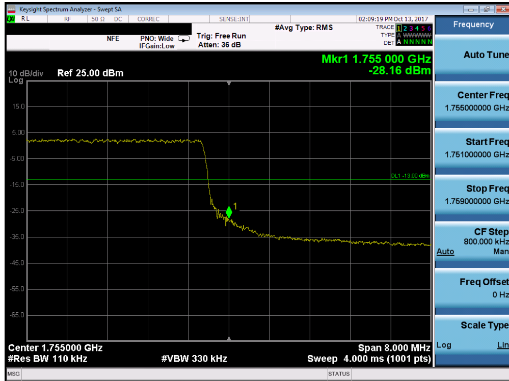
Plot 7-207. Upper Band Edge Plot (Band 4 – 10.0MHz QPSK - Full RB Configuration)
