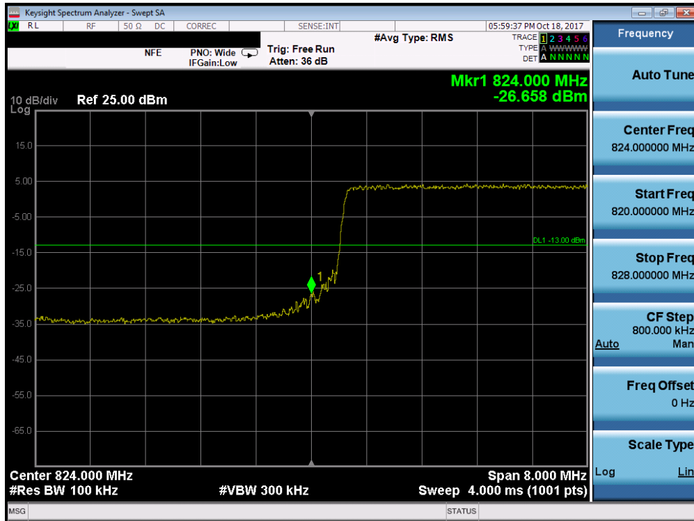
Plot 7-181. Lower Band Edge Plot (Band 5/26 - 10.0MHz QPSK - Full RB Configuration)
