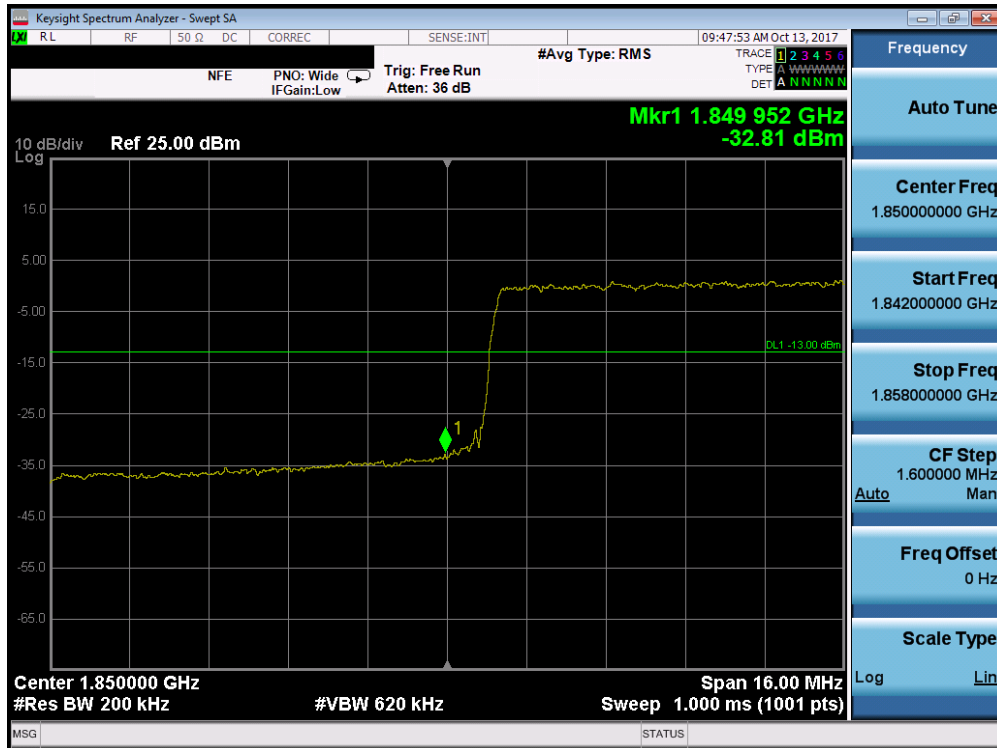
Plot 7-251. Lower Band Edge Plot (Band 2/25 - 20.0MHz QPSK - Full RB Configuration)
