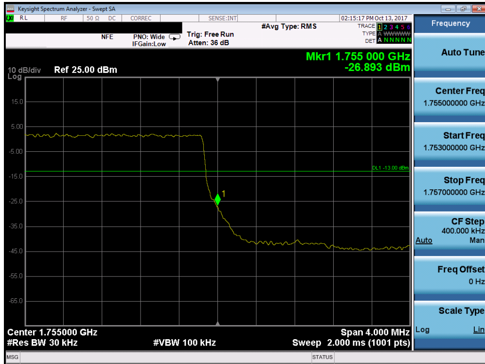
Plot 7-195. Upper Band Edge Plot (Band 4 – 3.0MHz QPSK - Full RB Configuration)
