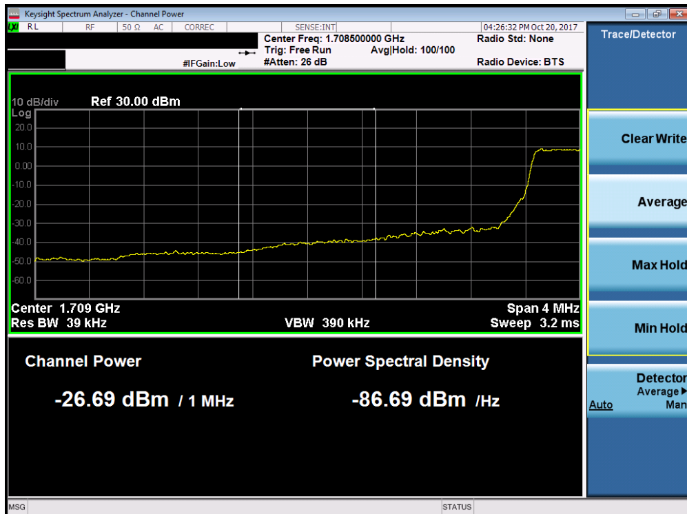
Plot 7-186. Lower Extended Band Edge Plot (Band 4/66 - 1.4MHz QPSK - Full RB Configuration)
