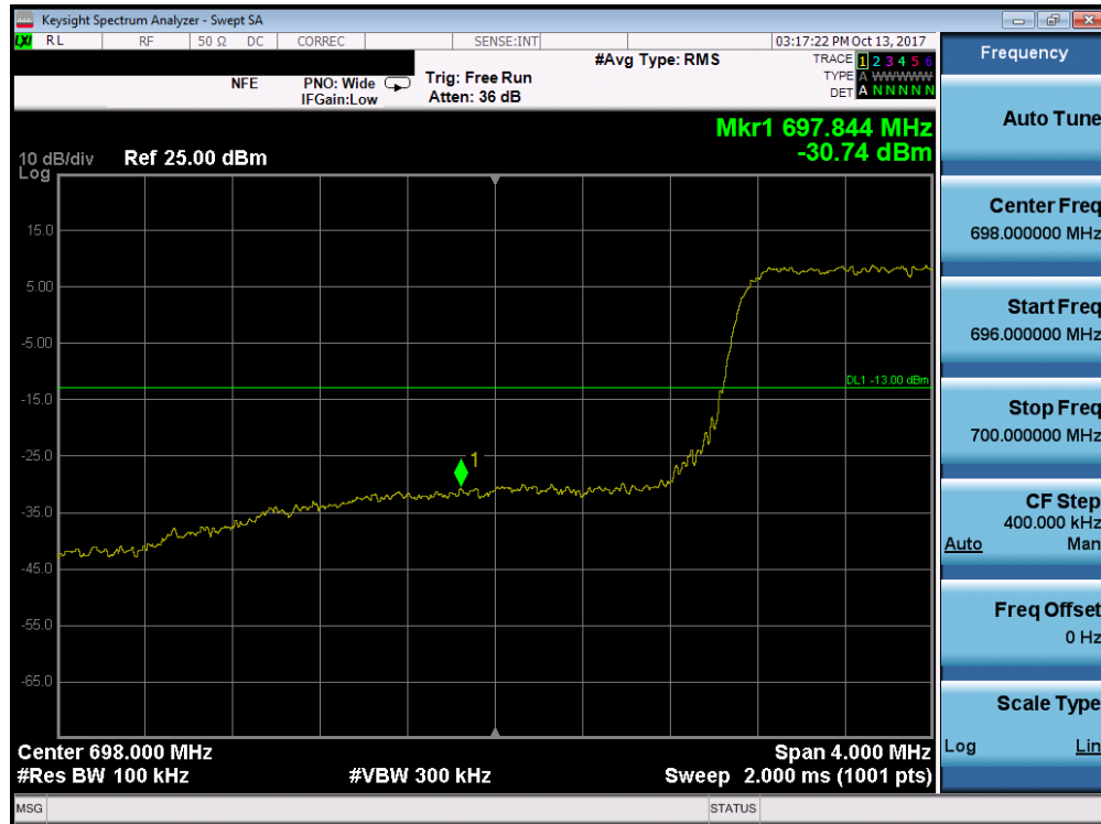
Plot 7-159. Lower Band Edge Plot (Band 12 - 3.0MHz QPSK - Full RB Configuration)
