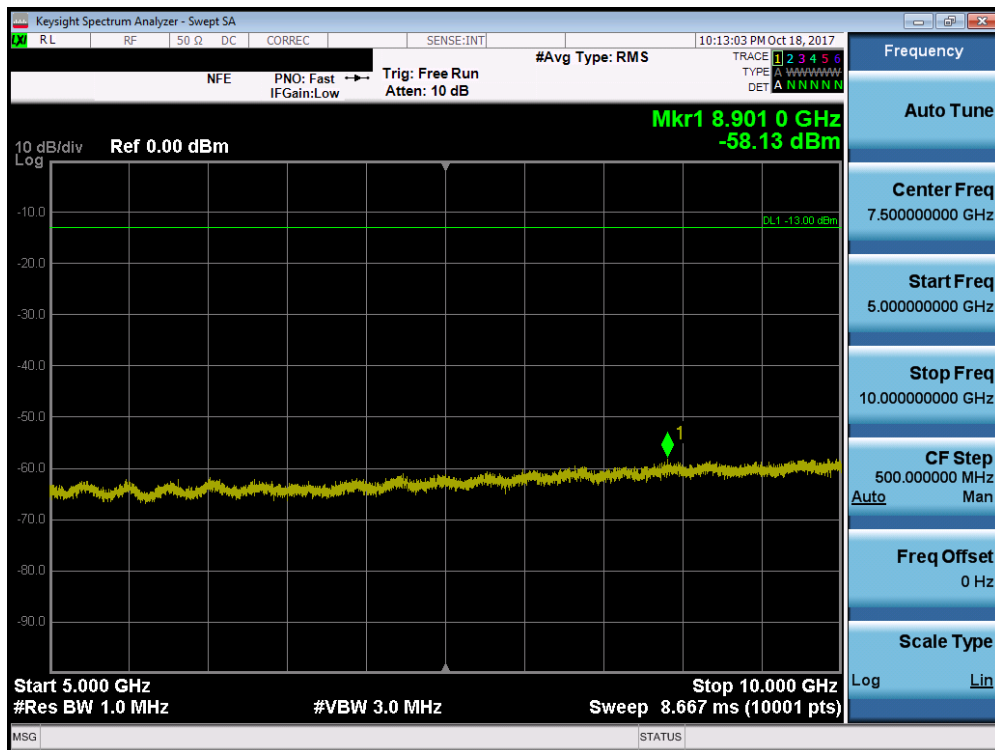
Plot 7-19. Conducted Spurious Plot (5.0MHz QPSK – RB Size 1, RB Offset 0 – High Channel)
