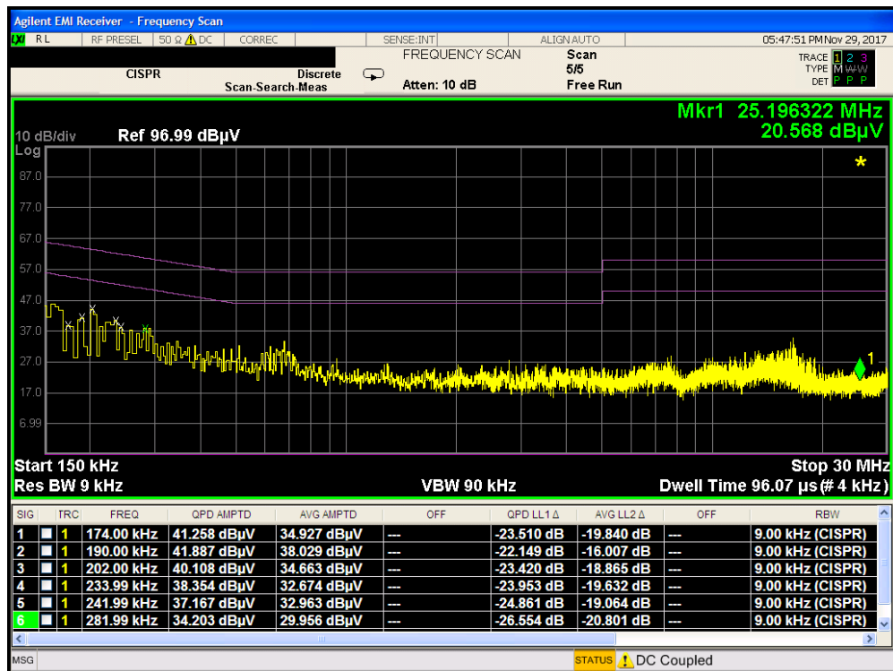
Plot 7-7. Line-Conducted Test Plot (N) RFID Antenna Terminated in 50Ω
