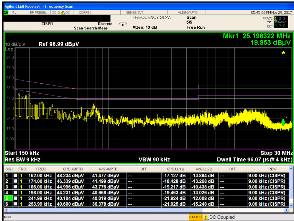
Plot 7-6. Line-Conducted Test Plot (L1) RFID Antenna Terminated in 50Ω
