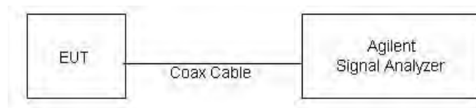
Figure 7-2. Test Instrument & Measurement Setup
