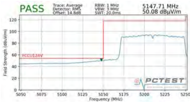
Plot 7-280. Radiated Lower Band Edge Plot (Average – UNII Band 1)
