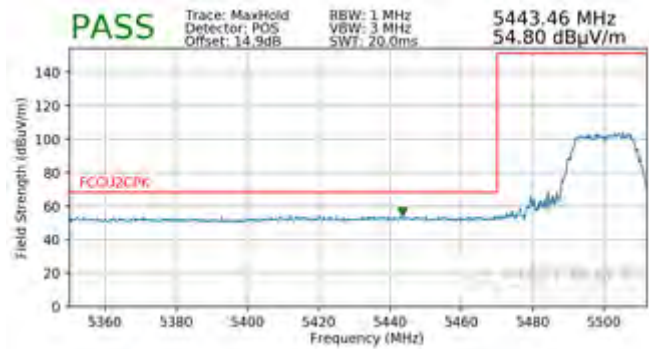
Plot 7-231. Radiated Lower Band Edge Plot (Peak – UNII Band 2C)
