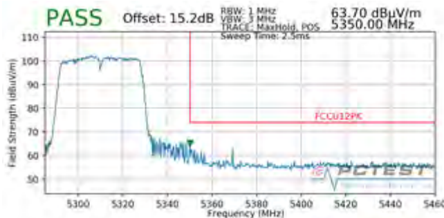
Plot 7-211. Radiated Upper Band Edge Plot (Peak - UNII Band 2A)
