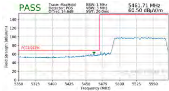
Plot 7-285. Radiated Lower Band Edge Plot (Peak – UNII Band 2C)
