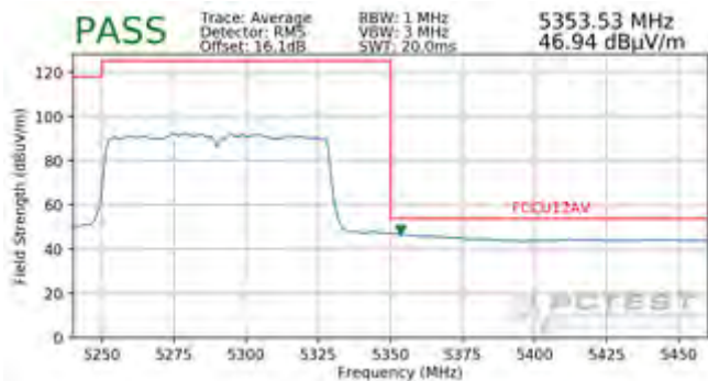
Plot 7-282. Radiated Upper Band Edge Plot (Average – UNII Band 2A)
