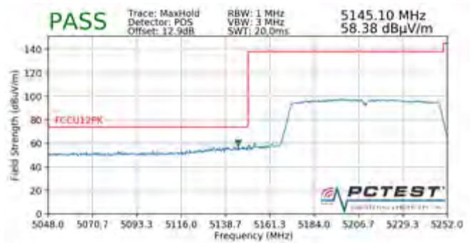
Plot 7-252. Radiated Band Edge Plot (Peak – WCP)
