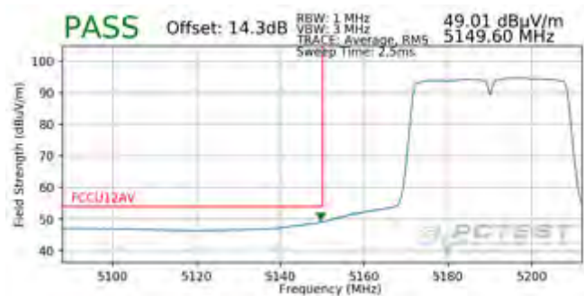
Plot 7-208. Radiated Lower Band Edge Plot (Average - UNII Band 1)
