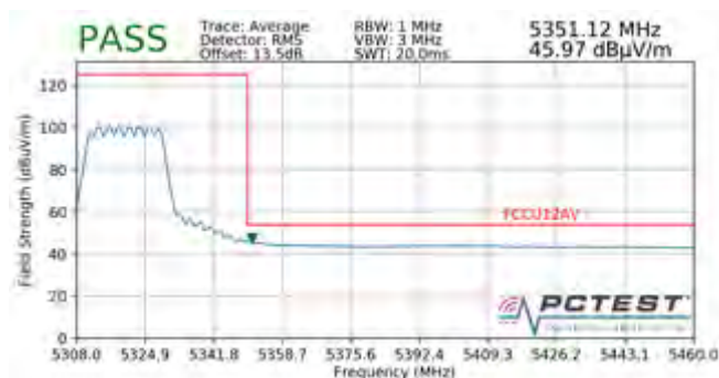
Plot 7-269. Radiated Band Edge Plot (Average – WCP)
