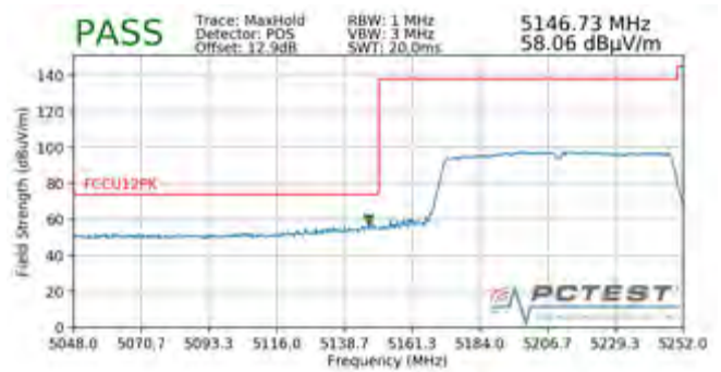
Plot 7-225. Radiated Band Edge Plot (Peak – WCP)
