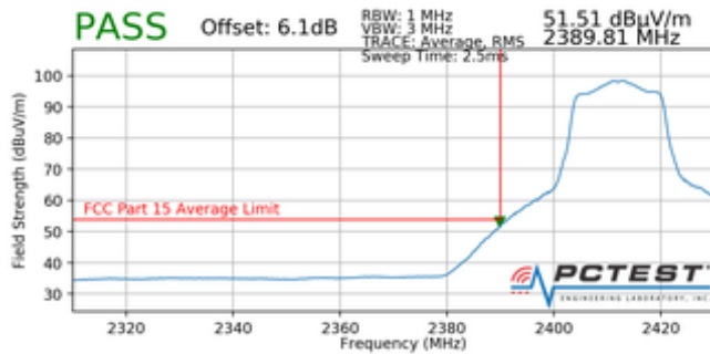
Plot 7-99. Radiated Restricted Lower Band Edge Measurement (Average)
