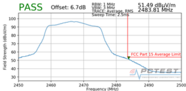
Plot 7-103. Radiated Restricted Upper Band Edge Measurement (Average)
