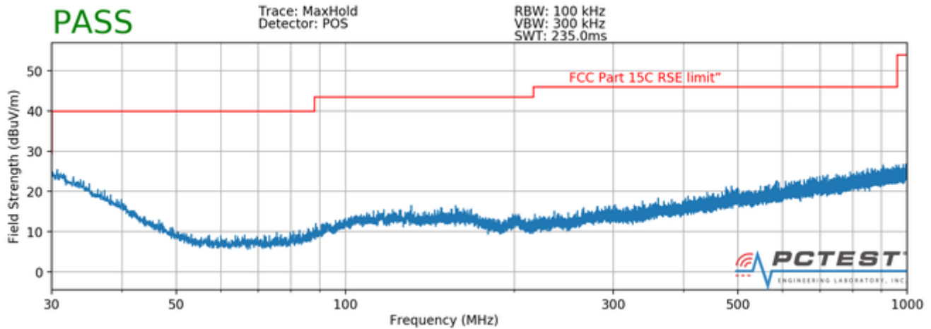
Plot 7-128. Radiated Spurious Plot below 1GHz (Pol. V)
