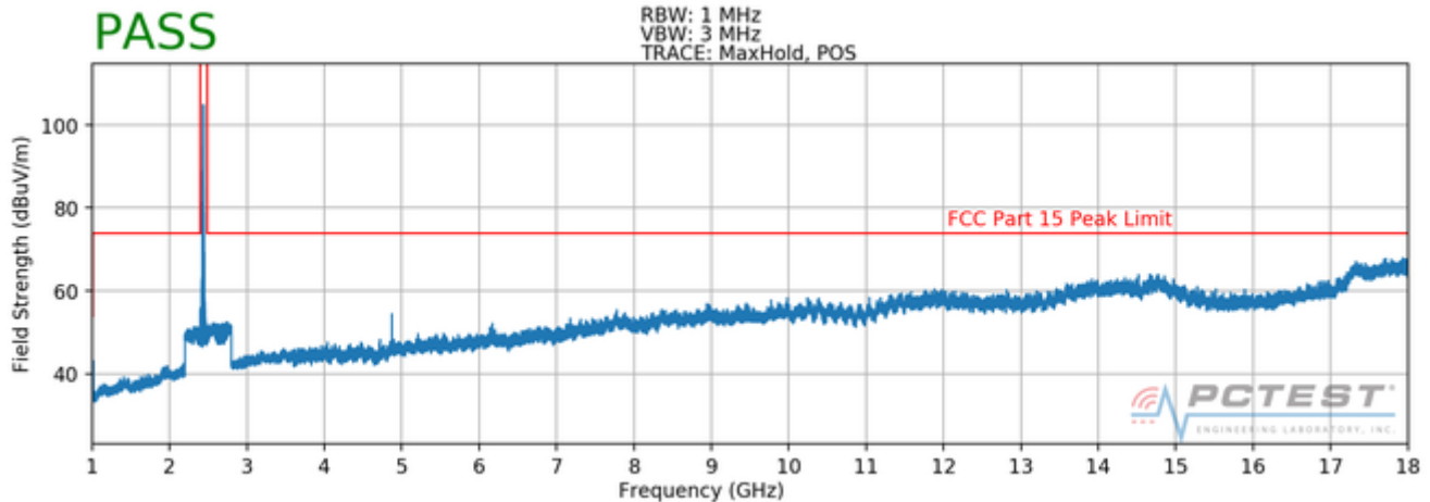
Plot 7-83. Radiated Spurious Plot above 1GHz (802.11b – Ch. 6, Ant. Pol. H)
