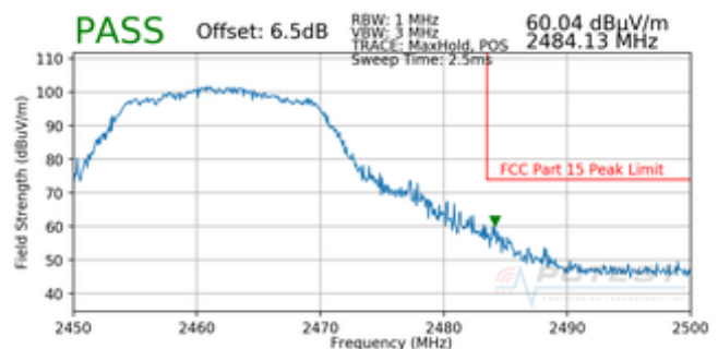
Plot 7-92. Radiated Restricted Upper Band Edge Measurement (Peak)
