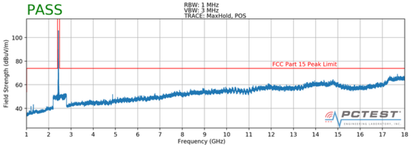
Plot 7-84. Radiated Spurious Plot above 1GHz (802.11b – Ch. 6, Ant. Pol. V)
