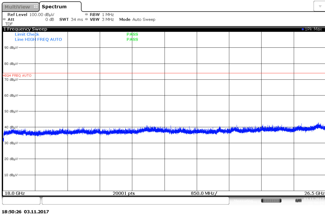
Plot 7-88. Radiated Spurious Plot above 18GHz (Pol. V)
