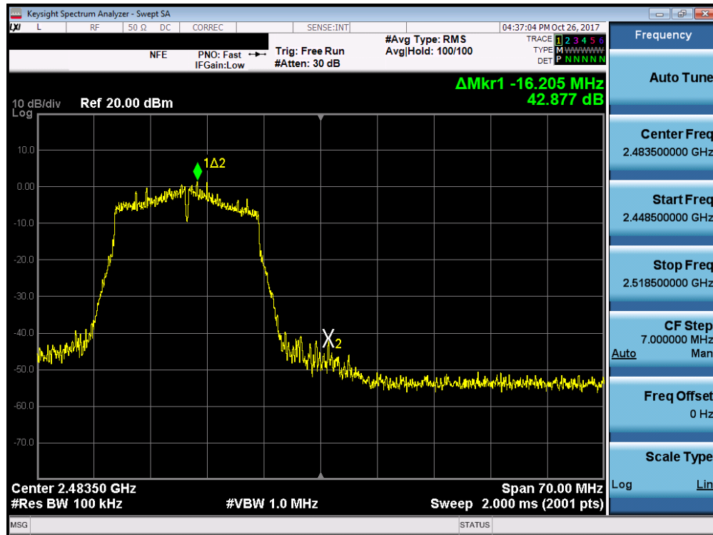
Plot 7-47. Band Edge Plot (802.11n – Ch. 12)
