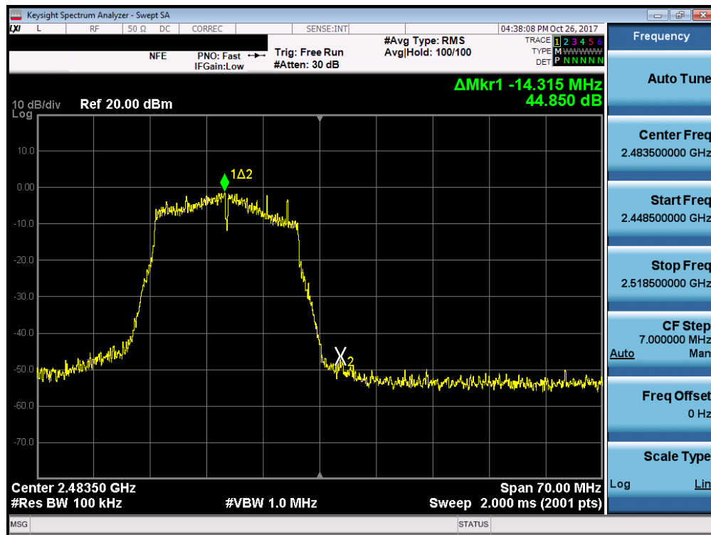
Plot 7-48. Band Edge Plot (802.11n – Ch. 13)
