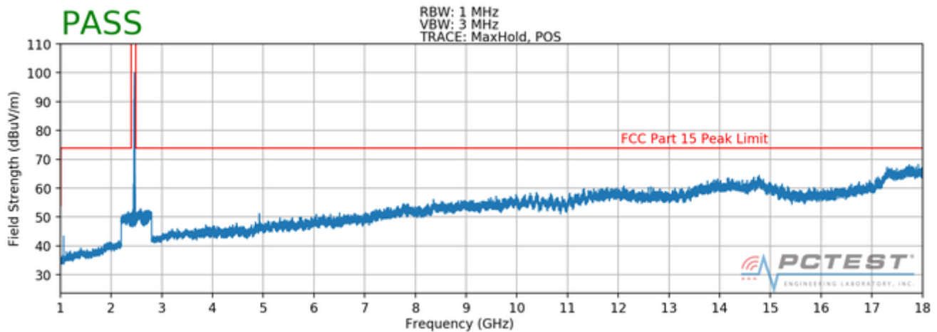
Plot 7-78. Radiated Spurious Plot above 1GHz (802.11b – Ch. 11, Ant. Pol. V)
