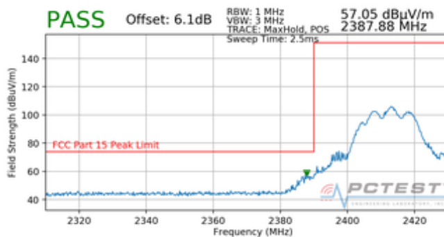
Plot 7-110. Radiated Restricted Lower Band Edge Measurement (Peak)
