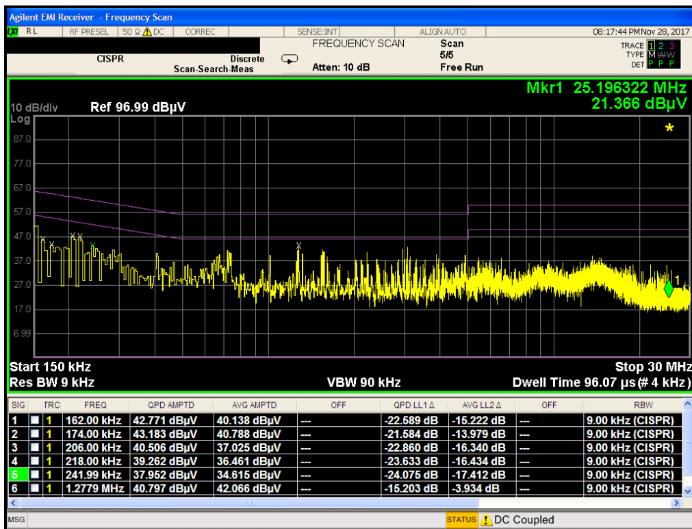
Plot 7-133. Line Conducted Plot with 802.11b (L1) (with WCP)
