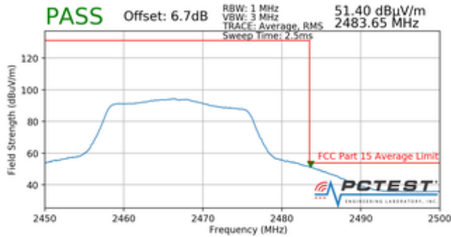
Plot 7-125. Radiated Restricted Band Edge Measurement with WCP (Average)
