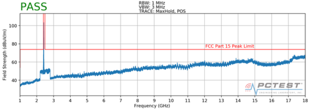
Plot 7-81. Radiated Spurious Plot above 1GHz (802.11b – Ch. 1, Ant. Pol. H)
