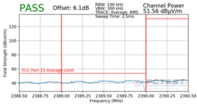
Plot 7-117. Radiated Restricted Lower Band Edge Measurement (Average)
