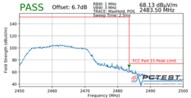
Plot 7-120. Radiated Restricted Upper Band Edge Measurement (Peak)
