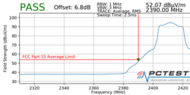
Plot 7-97. Radiated Restricted Band Edge Measurement with WCP (Average)
