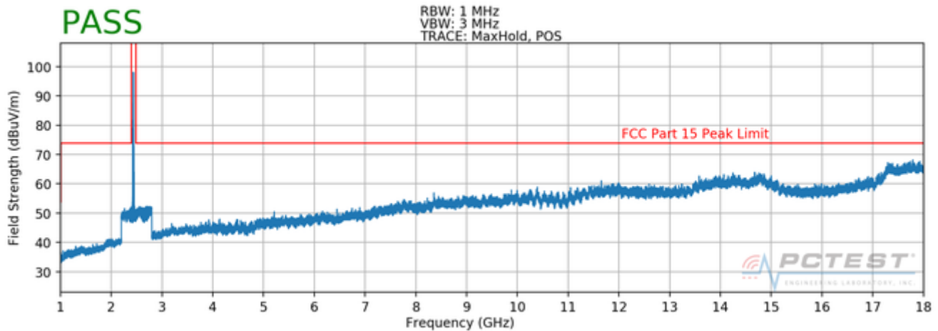
Plot 7-76. Radiated Spurious Plot above 1GHz (802.11b – Ch. 6, Ant. Pol. V)
