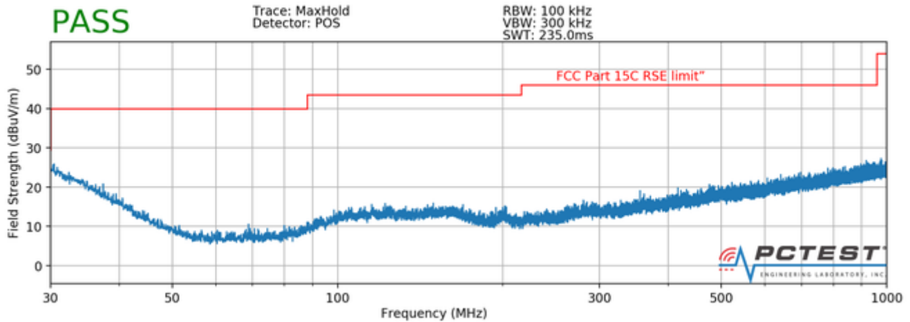
Plot 7-129. Radiated Spurious Plot below 1GHz (Pol. H)
