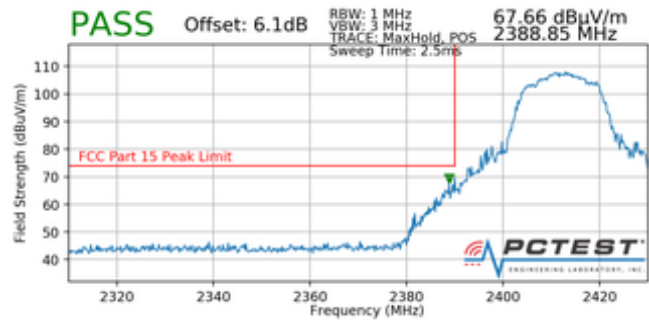
Plot 7-108. Radiated Restricted Band Edge Measurement with WCP (Peak)
