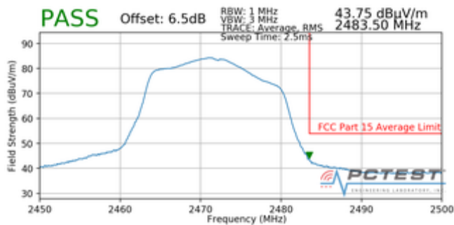
Plot 7-95. Radiated Restricted Upper Band Edge Measurement (Average)
