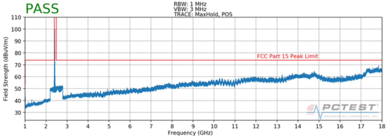
Plot 7-74. Radiated Spurious Plot above 1GHz (802.11b – Ch. 1, Ant. Pol. V)
