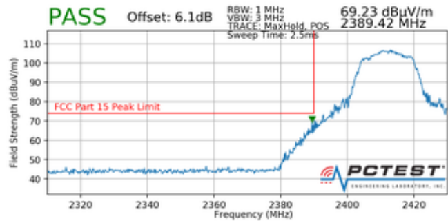
Plot 7-100. Radiated Restricted Lower Band Edge Measurement (Peak)
