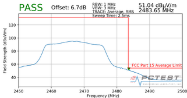
Plot 7-121. Radiated Restricted Upper Band Edge Measurement (Average)
