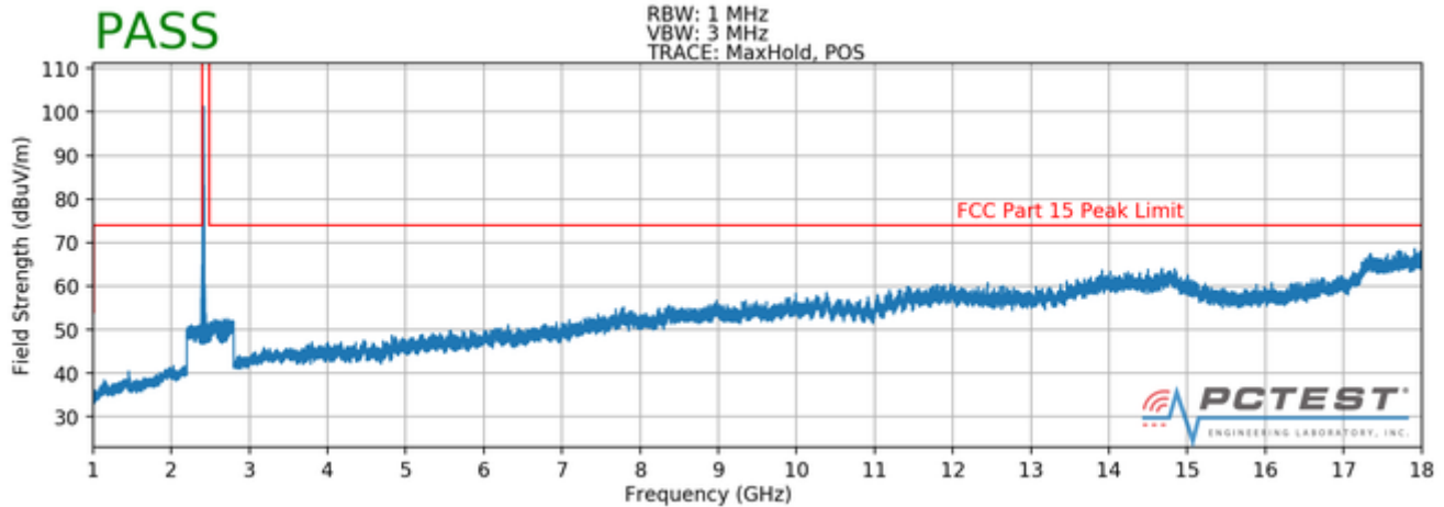
Plot 7-73. Radiated Spurious Plot above 1GHz (802.11b – Ch. 1, Ant. Pol. H)
