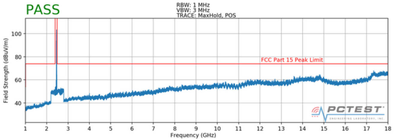
Plot 7-85. Radiated Spurious Plot above 1GHz (802.11b – Ch. 11, Ant. Pol. H)
