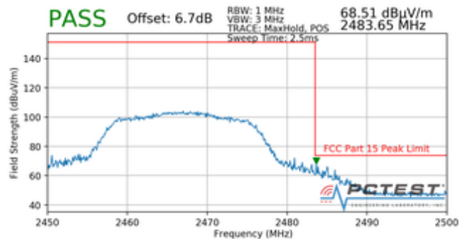
Plot 7-122. Radiated Restricted Upper Band Edge Measurement (Peak)
