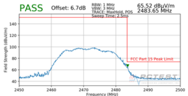
Plot 7-116. Radiated Restricted Upper Band Edge Measurement (Peak)
