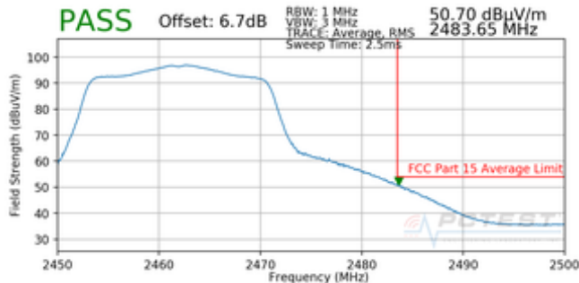
Plot 7-101. Radiated Restricted Upper Band Edge Measurement (Average)
