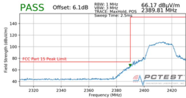
Plot 7-118. Radiated Restricted Lower Band Edge Measurement (Peak)
