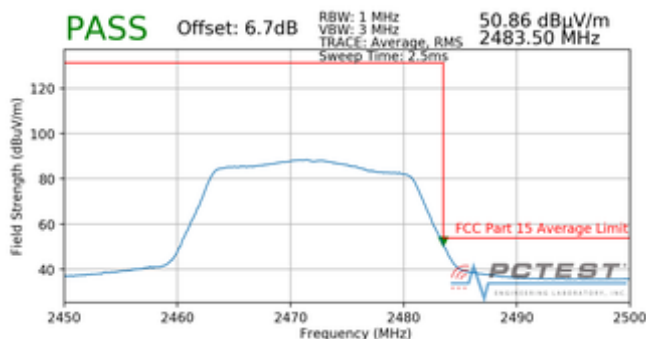
Plot 7-123. Radiated Restricted Upper Band Edge Measurement (Average)
