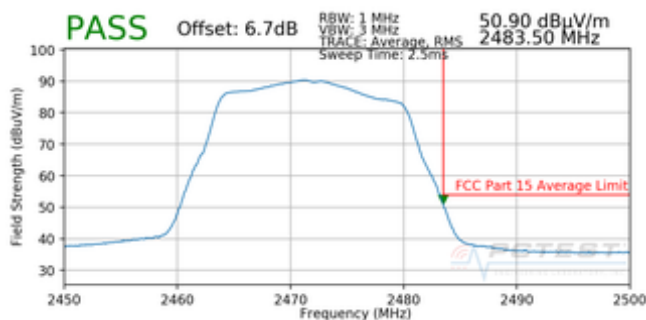
Plot 7-105. Radiated Restricted Upper Band Edge Measurement (Average)
