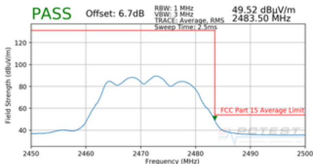
Plot 7-115. Radiated Restricted Upper Band Edge Measurement (Average)
