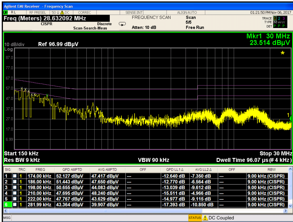
Plot 7-131. Line Conducted Plot with 802.11b (L1)
