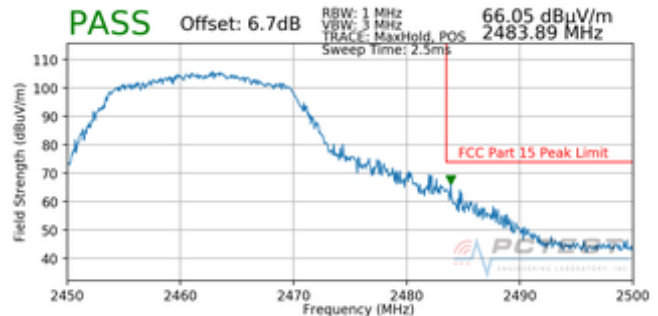
Plot 7-102. Radiated Restricted Upper Band Edge Measurement (Peak)
