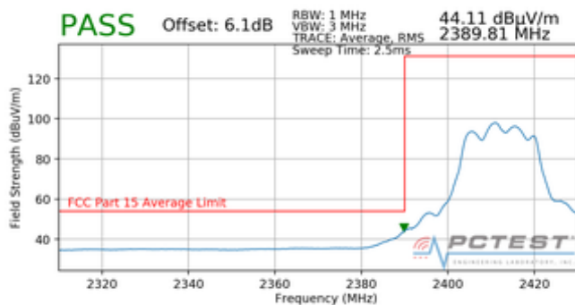
Plot 7-109. Radiated Restricted Lower Band Edge Measurement (Average)
