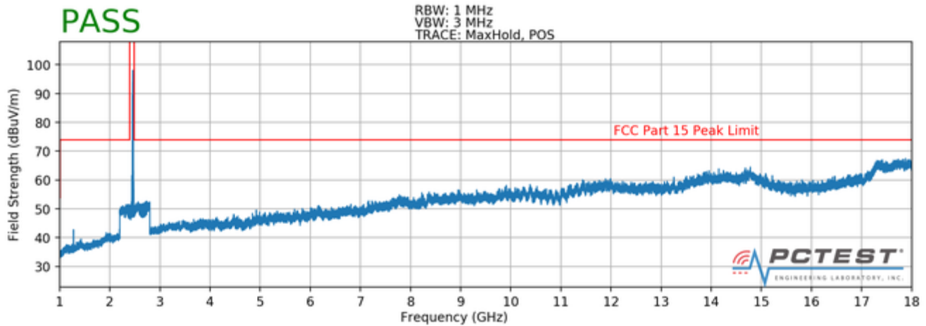
Plot 7-77. Radiated Spurious Plot above 1GHz (802.11b – Ch. 11, Ant. Pol. H)
