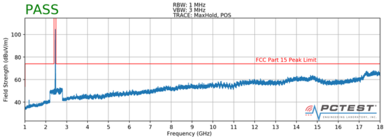
Plot 7-86. Radiated Spurious Plot above 1GHz (802.11b – Ch. 11, Ant. Pol. V)
