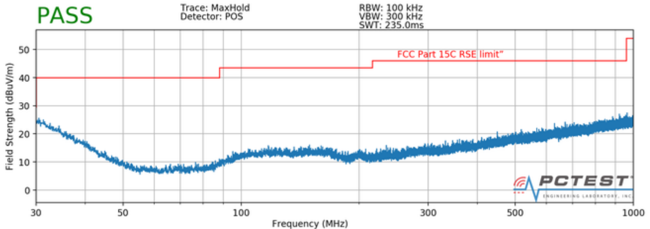
Plot 7-130. Radiated Spurious Plot below 1GHz (Pol. V)
