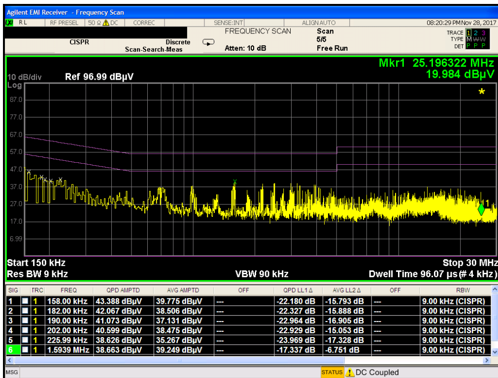
Plot 7-134. Line Conducted Plot with 802.11b (N) (with WCP)
