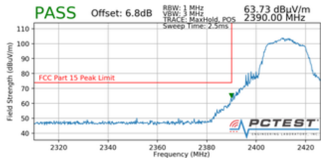
Plot 7-90. Radiated Restricted Lower Band Edge Measurement (Peak)
