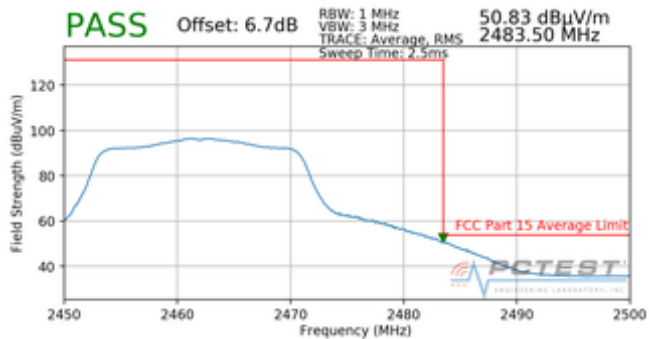
Plot 7-119. Radiated Restricted Upper Band Edge Measurement (Average)
