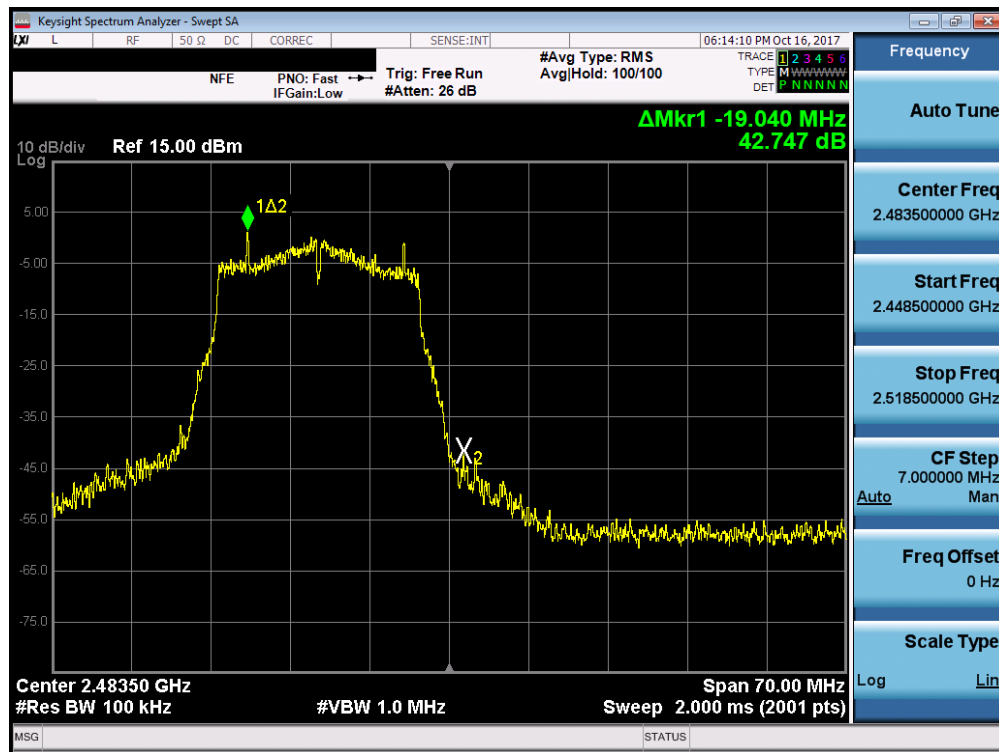
Plot 7-60. Band Edge Plot (802.11n – Ch. 13)
