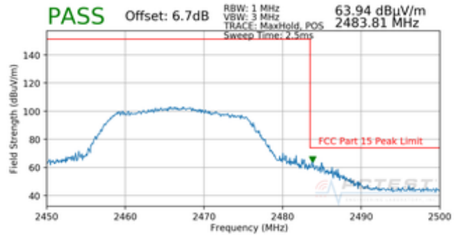
Plot 7-126. Radiated Restricted Band Edge Measurement with WCP (Peak)
