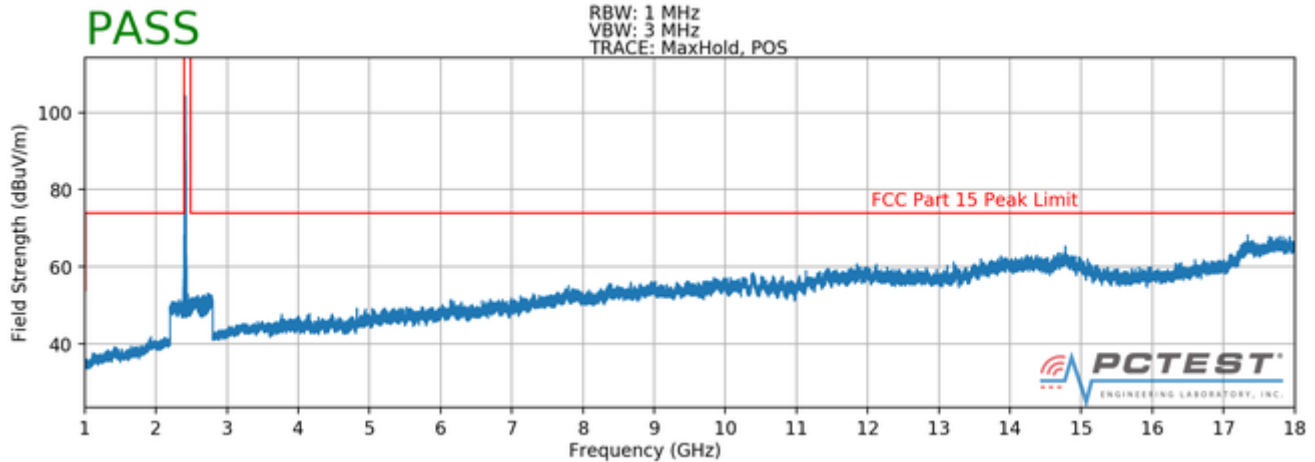
Plot 7-82. Radiated Spurious Plot above 1GHz (802.11b – Ch. 1, Ant. Pol. V)
