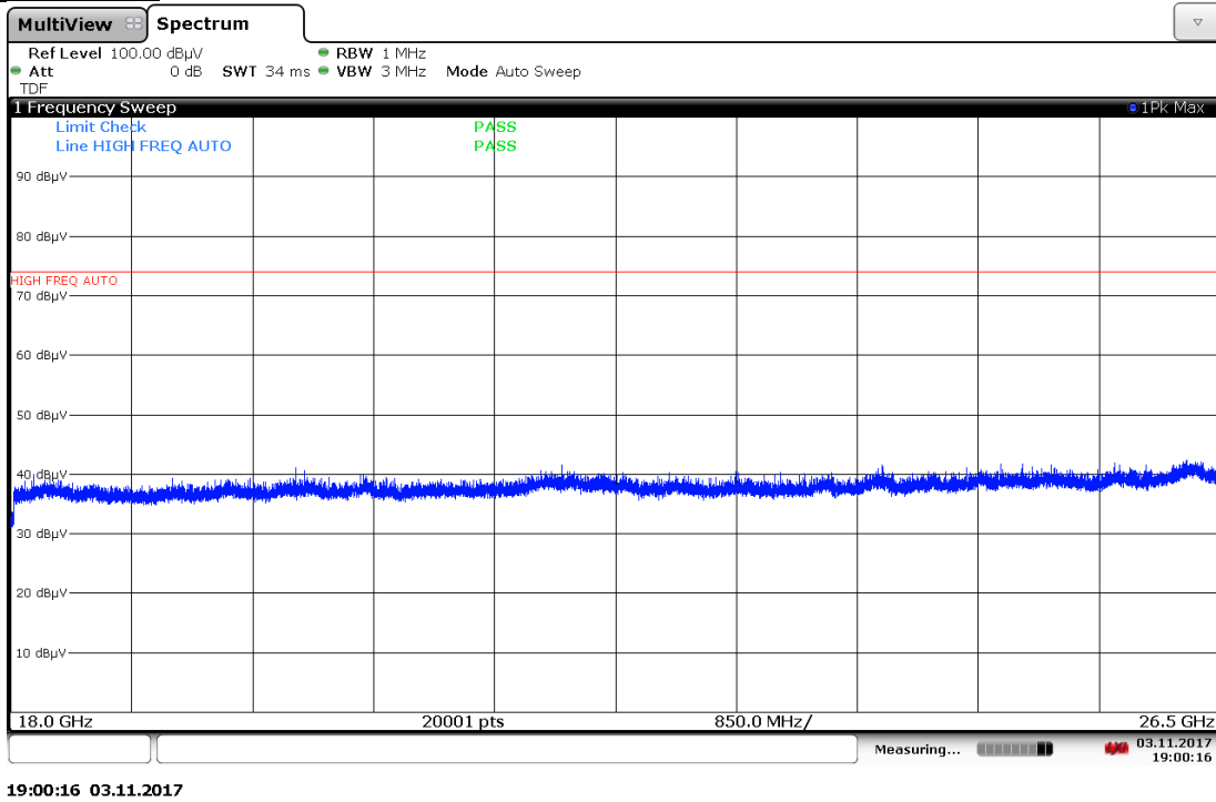
Plot 7-87. Radiated Spurious Plot above 18GHz (Pol. H)
