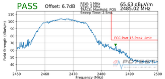
Plot 7-104. Radiated Restricted Upper Band Edge Measurement (Peak)
