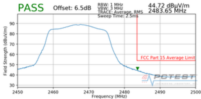
Plot 7-93. Radiated Restricted Upper Band Edge Measurement (Average)
