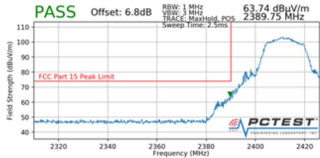
Plot 7-98. Radiated Restricted Band Edge Measurement with WCP (Peak)
