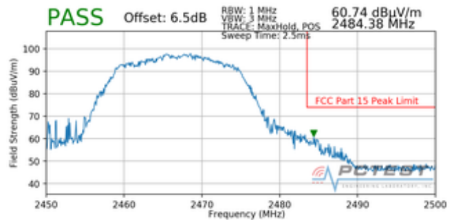
Plot 7-94. Radiated Restricted Upper Band Edge Measurement (Peak)
