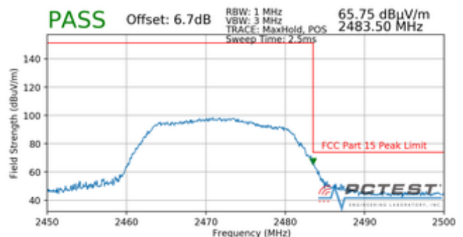
Plot 7-124. Radiated Restricted Upper Band Edge Measurement (Peak)
