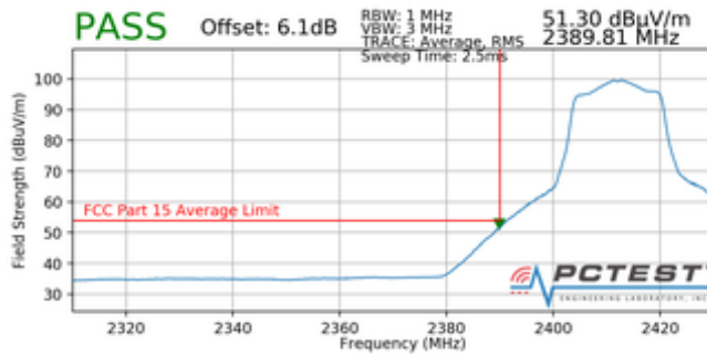
Plot 7-107. Radiated Restricted Band Edge Measurement with WCP (Average)
