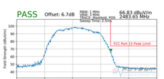
Plot 7-106. Radiated Restricted Upper Band Edge Measurement (Peak)
