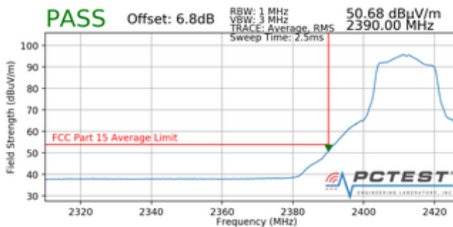
Plot 7-89. Radiated Restricted Lower Band Edge Measurement (Average)
