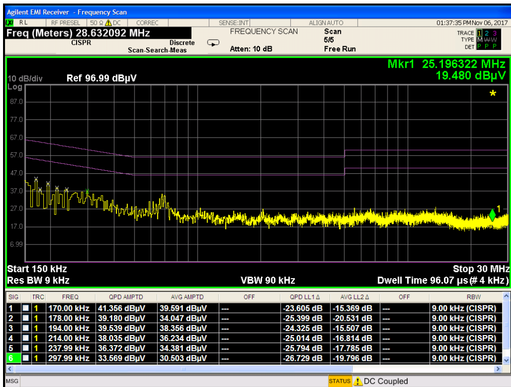
Plot 7-132. Line Conducted Plot with 802.11b (N)
