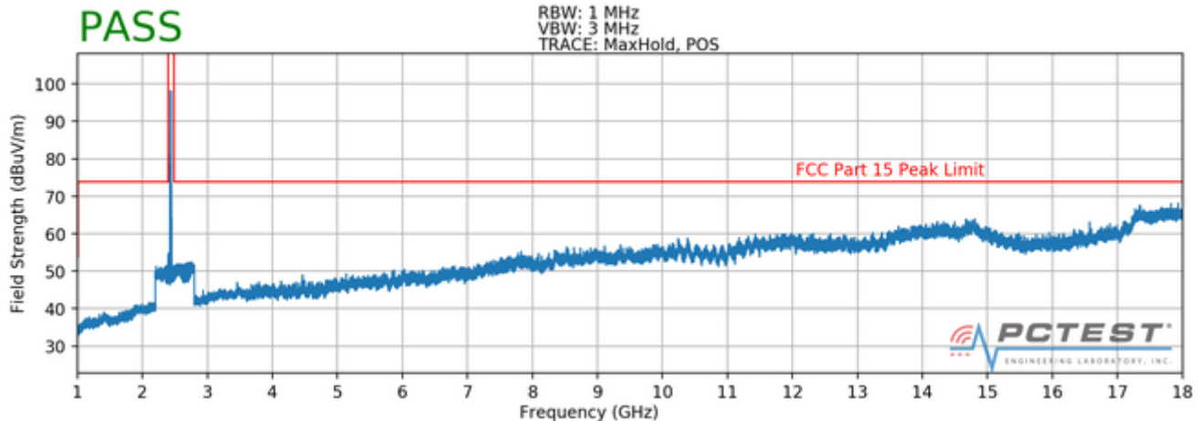
Plot 7-75. Radiated Spurious Plot above 1GHz (802.11b – Ch. 6, Ant. Pol. H)
