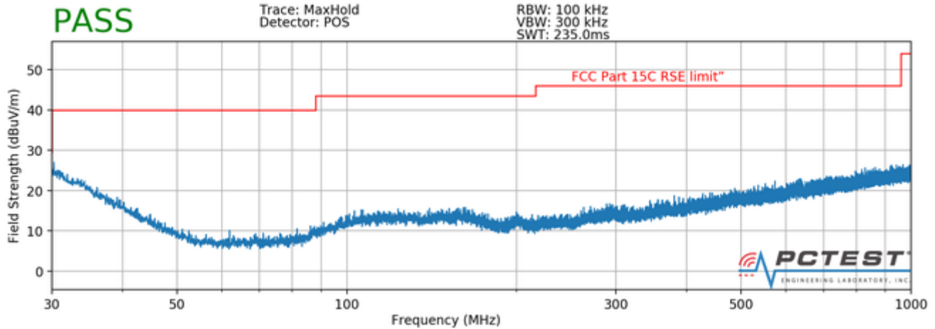
Plot 7-127. Radiated Spurious Plot below 1GHz (Pol. H)
