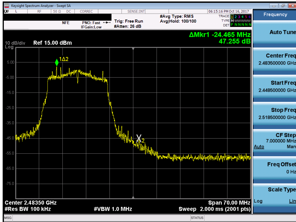
Plot 7-59. Band Edge Plot (802.11n – Ch. 12)
