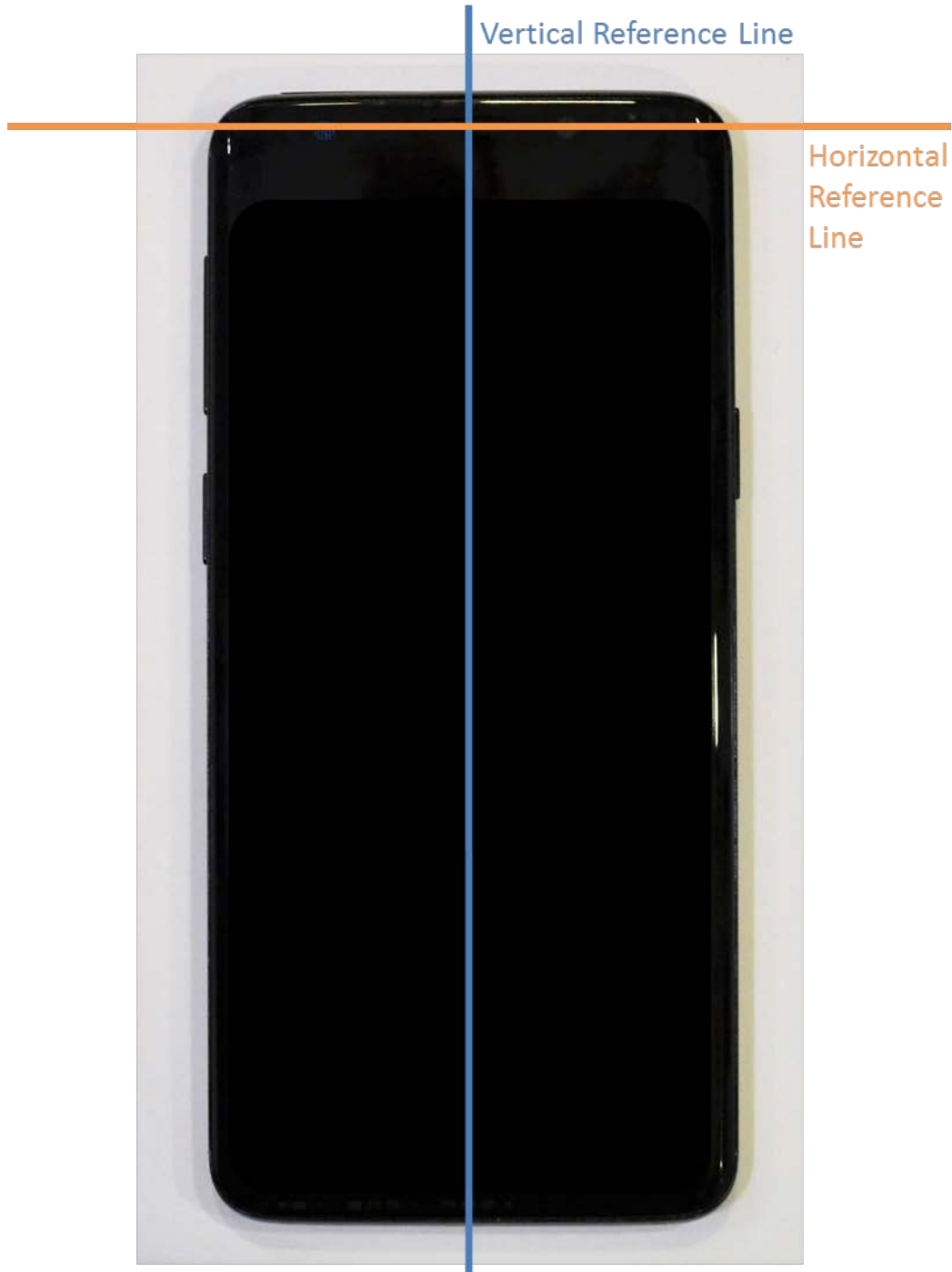
SAR Test Setup Photo 12 – Horizontal and Vertical Reference Lines
