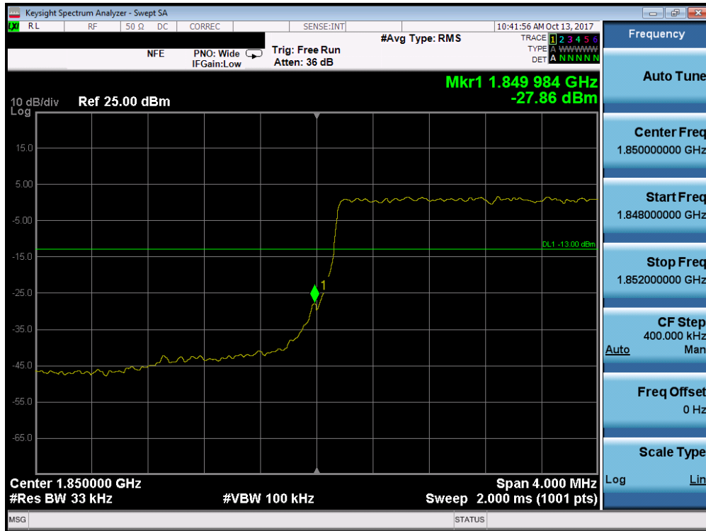
Plot 7-179. Lower Band Edge Plot (Band 2/25 - 3.0MHz QPSK - Full RB Configuration)
