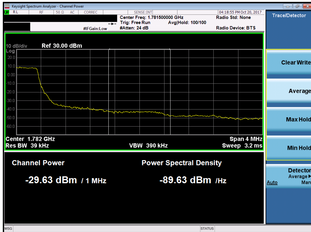
Plot 7-140. Upper Extended Band Edge Plot (Band 66 - 1.4MHz QPSK - Full RB Configuration)
