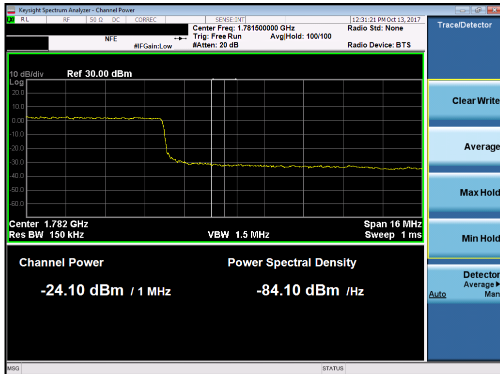
Plot 7-170. Upper Extended Band Edge Plot (Band 66 - 20.0MHz QPSK - Full RB Configuration)
