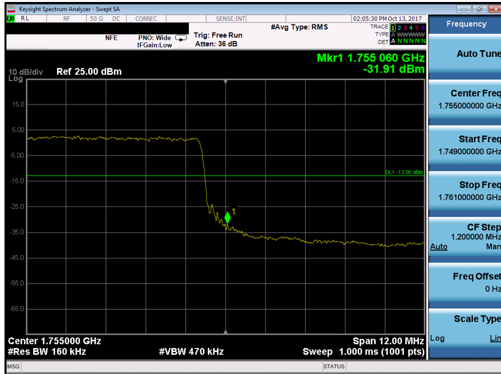
Plot 7-165. Upper Band Edge Plot (Band 4 – 15.0MHz QPSK - Full RB Configuration)
