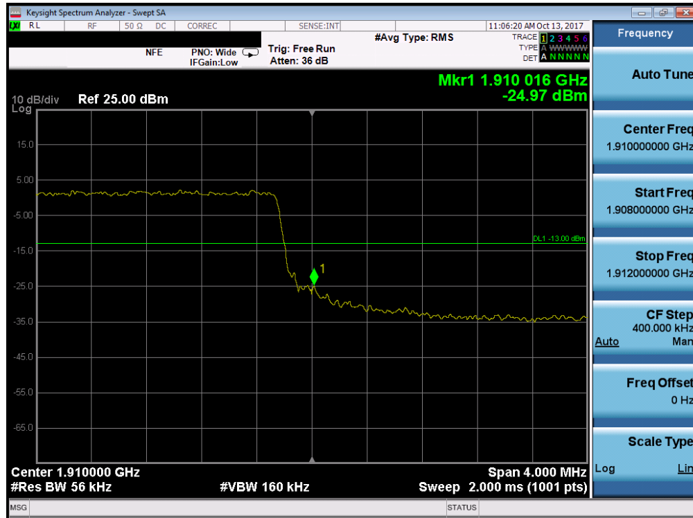
Plot 7-189. Upper Band Edge Plot (Band 2 – 5.0MHz QPSK - Full RB Configuration)
