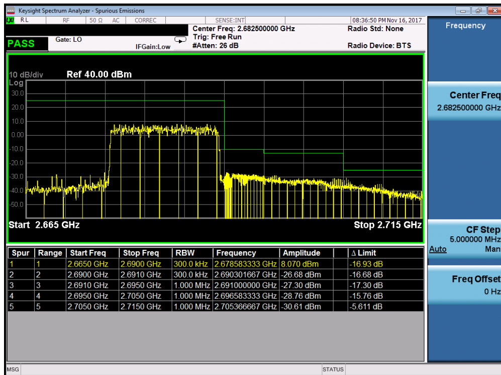
Plot 7-214. Upper ACP Plot (Band 41 - 15.0MHz QPSK - Full RB Configuration)
