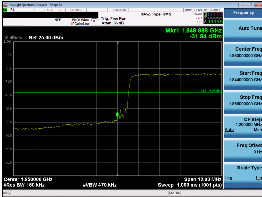
Plot 7-197. Lower Band Edge Plot (Band 2/25 - 15.0MHz QPSK - Full RB Configuration)
