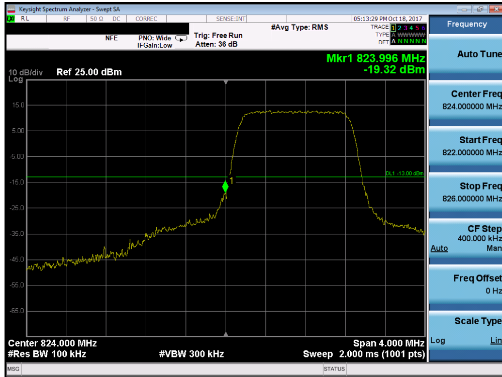
Plot 7-127. Lower Band Edge Plot (Band 5/26 - 1.4MHz QPSK - Full RB Configuration)
