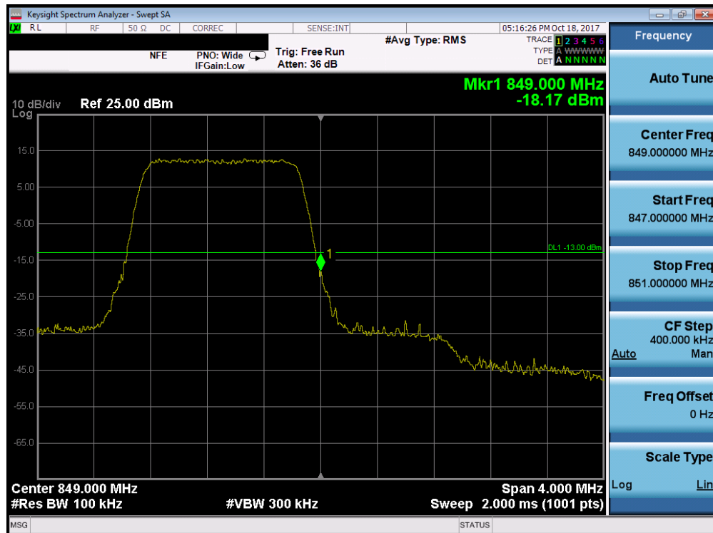
Plot 7-128. Upper Band Edge Plot (Band 5/26 - 1.4MHz QPSK - Full RB Configuration)
