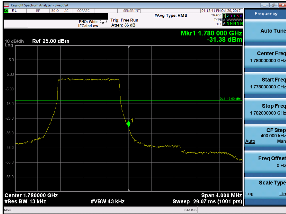
Plot 7-139. Upper Band Edge Plot (Band 66 - 1.4MHz QPSK - Full RB Configuration)
