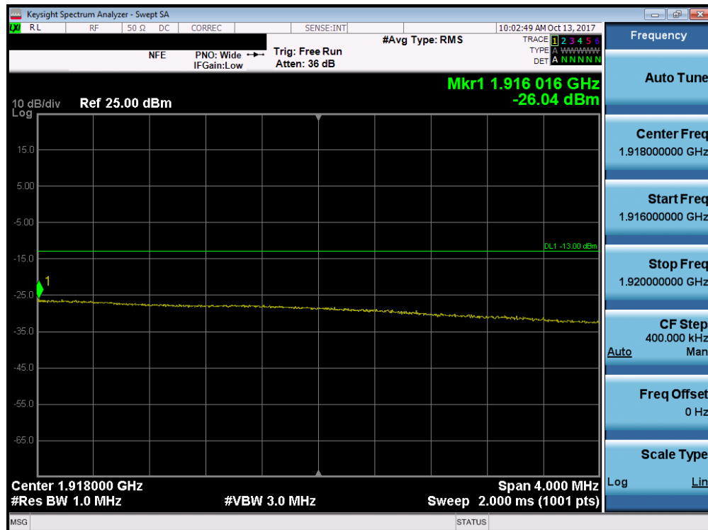
Plot 7-200. Upper Extended Band Edge Plot (Band 25 - 15.0MHz QPSK - Full RB Configuration)
