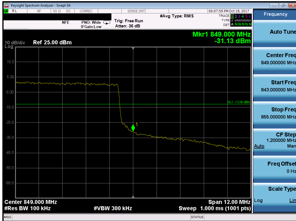
Plot 7-136. Upper Band Edge Plot (Band 26 - 15.0MHz QPSK - Full RB Configuration)
