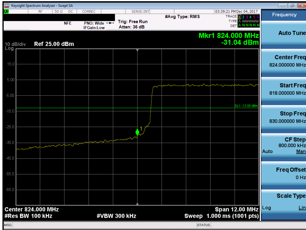
Plot 7-135. Lower Band Edge Plot (Band 26 - 15.0MHz QPSK - Full RB Configuration)
