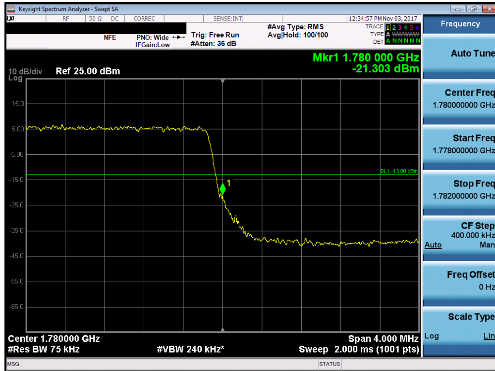
Plot 7-145. Upper Band Edge Plot (Band 66 - 3.0MHz QPSK - Full RB Configuration)
