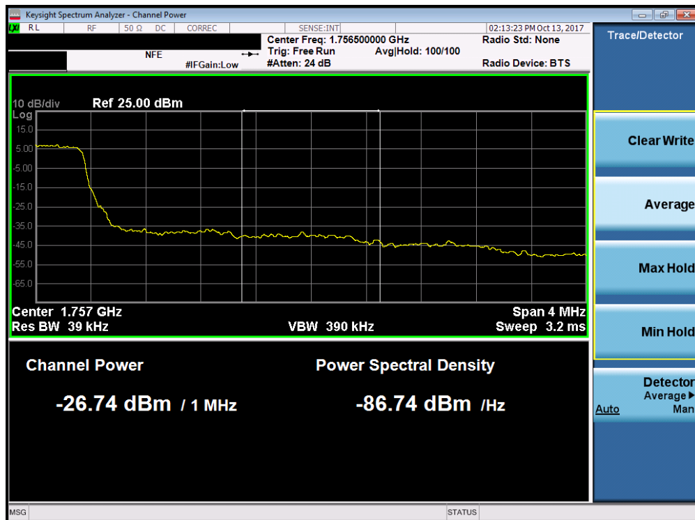
Plot 7-142. Upper Extended Band Edge Plot (Band 4 - 1.4MHz QPSK - Full RB Configuration)
