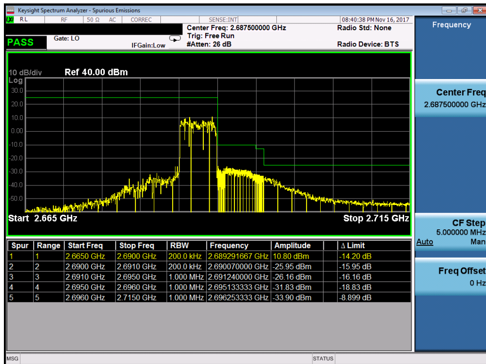
Plot 7-210. Upper ACP Plot (Band 41 - 5.0MHz QPSK - Full RB Configuration)
