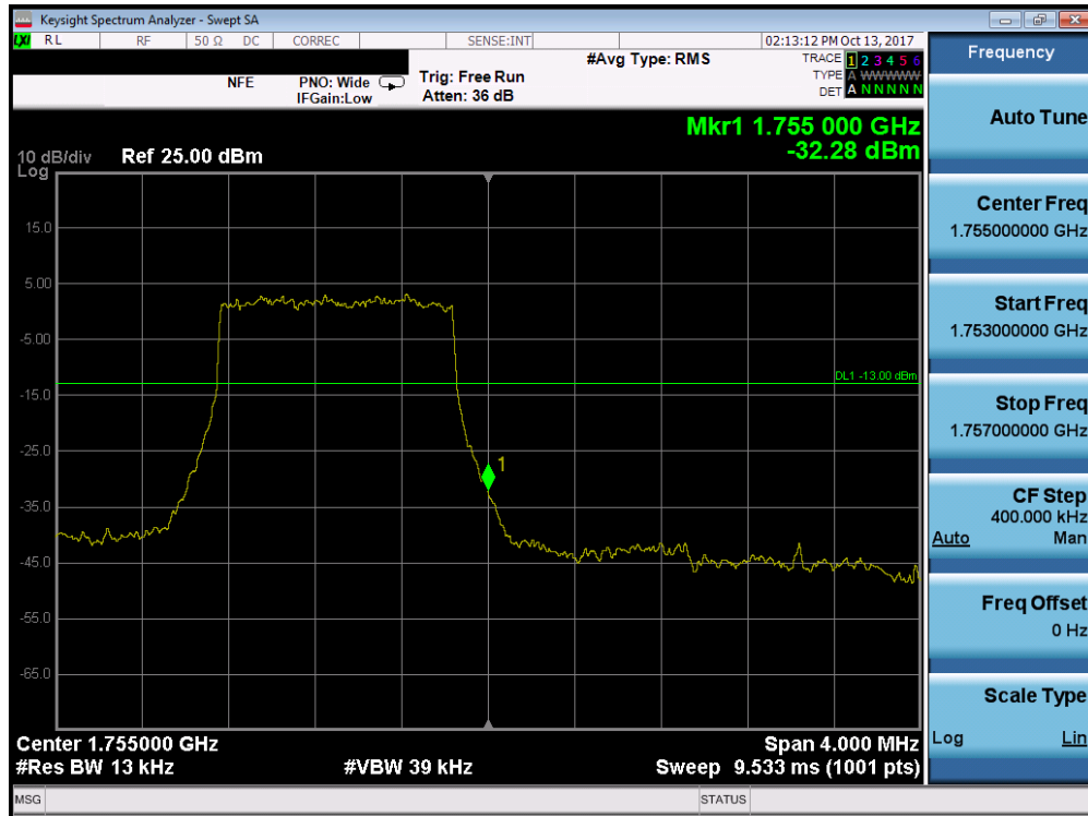
Plot 7-141. Upper Band Edge Plot (Band 4 - 1.4MHz QPSK - Full RB Configuration)
