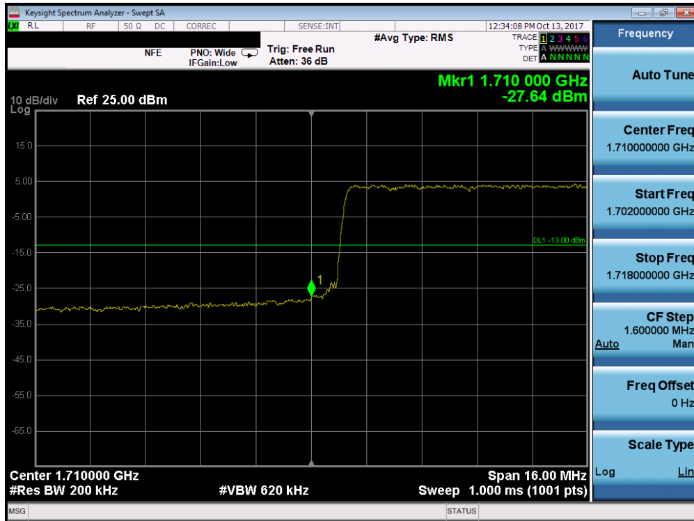
Plot 7-167. Lower Band Edge Plot (Band 4/66 - 20.0MHz QPSK - Full RB Configuration)
