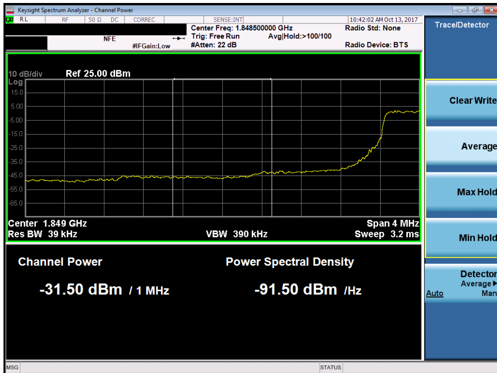
Plot 7-180. Lower Extended Band Edge Plot (Band 2/25 - 3.0MHz QPSK - Full RB Configuration)
