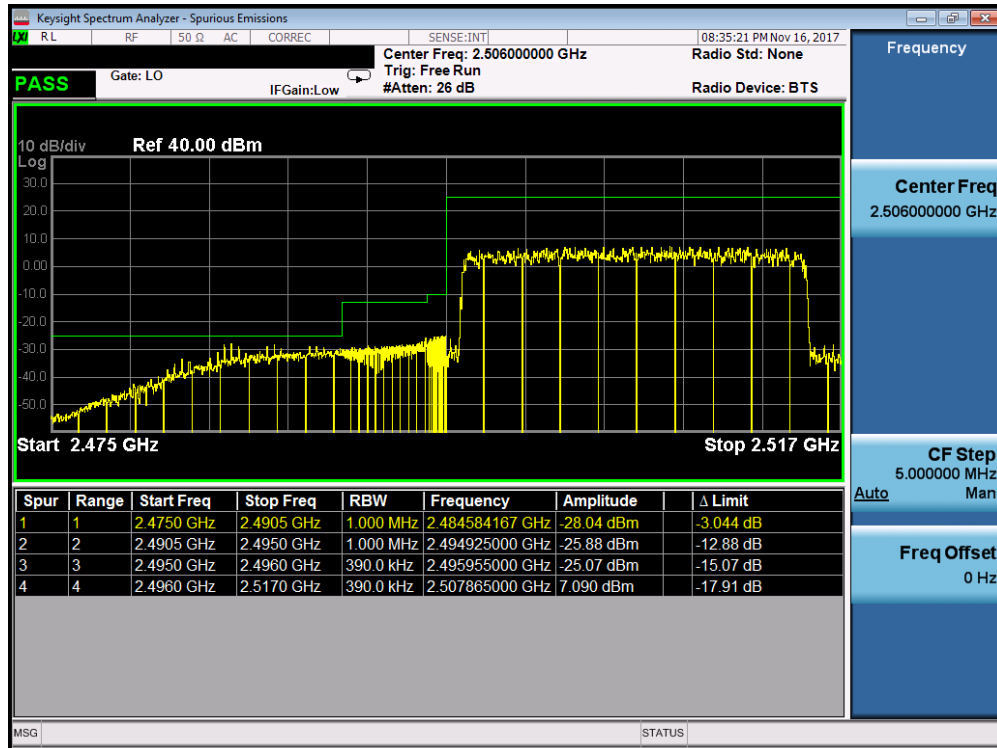
Plot 7-215. Lower ACP Plot (Band 41 - 20.0MHz QPSK - Full RB Configuration)
