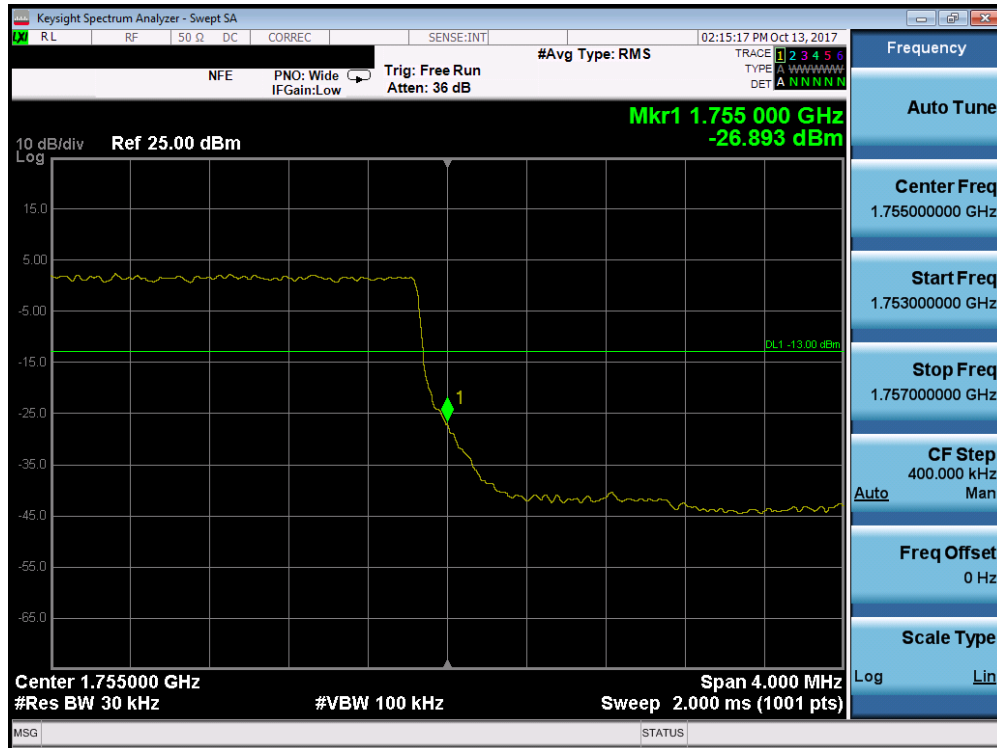
Plot 7-147. Upper Band Edge Plot (Band 4 – 3.0MHz QPSK - Full RB Configuration)
