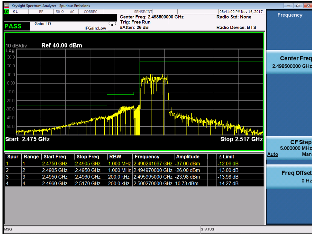
Plot 7-209. Lower ACP Plot (Band 41 - 5.0MHz QPSK - Full RB Configuration)
