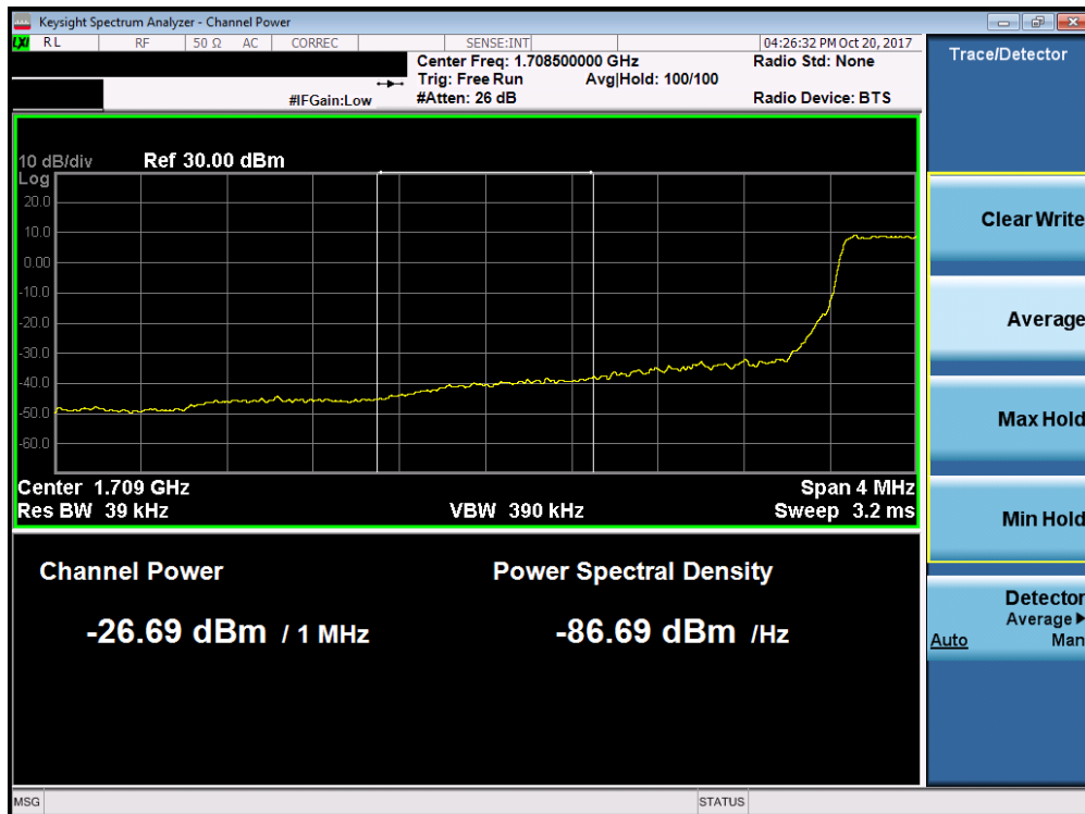
Plot 7-138. Lower Extended Band Edge Plot (Band 4/66 - 1.4MHz QPSK - Full RB Configuration)
