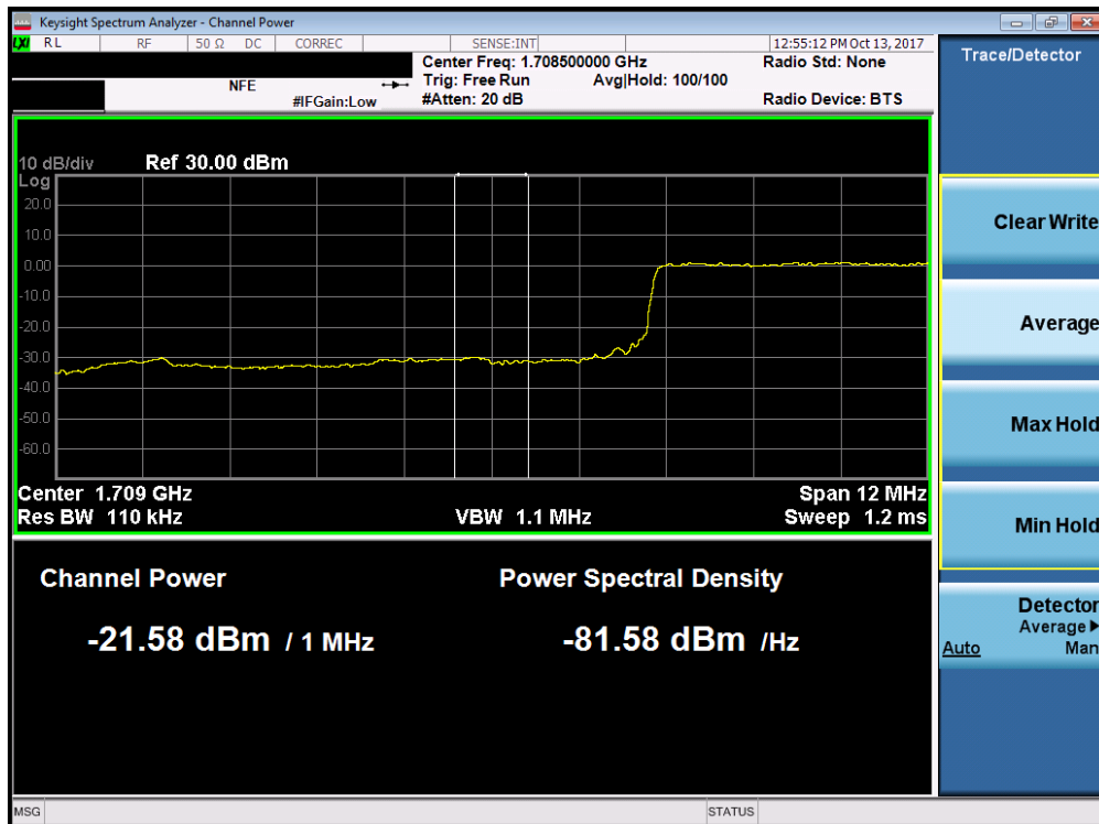
Plot 7-162. Lower Extended Band Edge Plot (Band 4/66 - 15.0MHz QPSK - Full RB Configuration)
