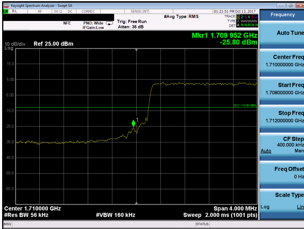
Plot 7-149. Lower Band Edge Plot (Band 4/66 - 5.0MHz QPSK - Full RB Configuration)
