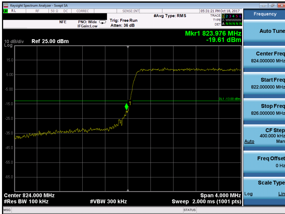
Plot 7-129. Lower Band Edge Plot (Band 5/26 - 3.0MHz QPSK - Full RB Configuration)
