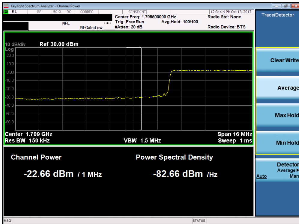
Plot 7-168. Lower Extended Band Edge Plot (Band 4/66 - 20.0MHz QPSK - Full RB Configuration)
