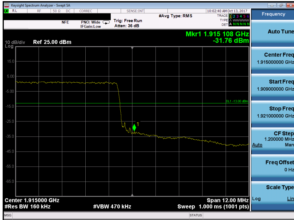
Plot 7-199. Upper Band Edge Plot (Band 25 - 15.0MHz QPSK - Full RB Configuration)
