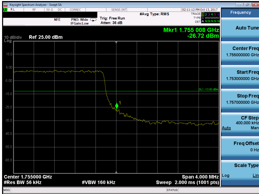
Plot 7-153. Upper Band Edge Plot (Band 4 – 5.0MHz QPSK - Full RB Configuration)
