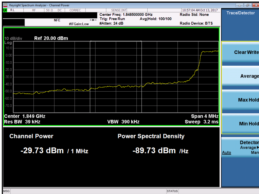
Plot 7-174. Lower Extended Band Edge Plot (Band 2/25 - 1.4MHz QPSK - Full RB Configuration)
