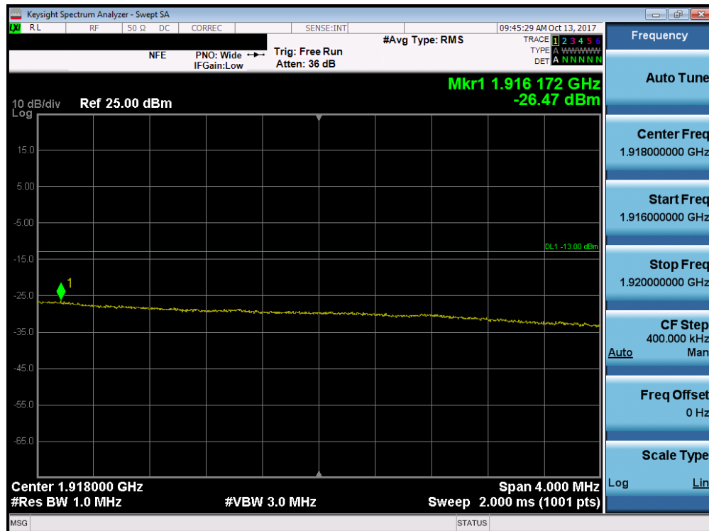
Plot 7-206. Upper Extended Band Edge Plot (Band 25 - 20.0MHz QPSK - Full RB Configuration)
