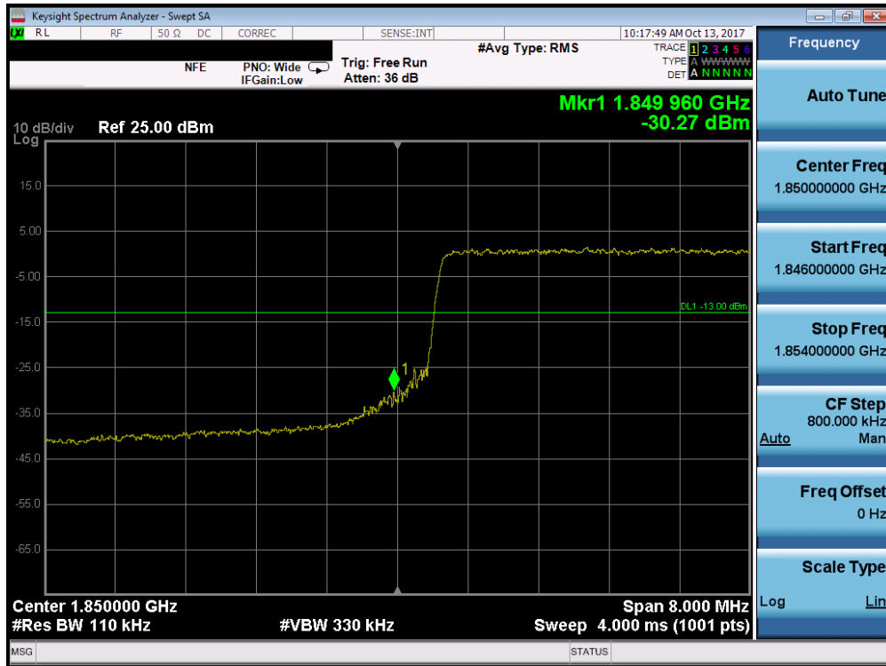
Plot 7-191. Lower Band Edge Plot (Band 2/25 - 10.0MHz QPSK - Full RB Configuration)
