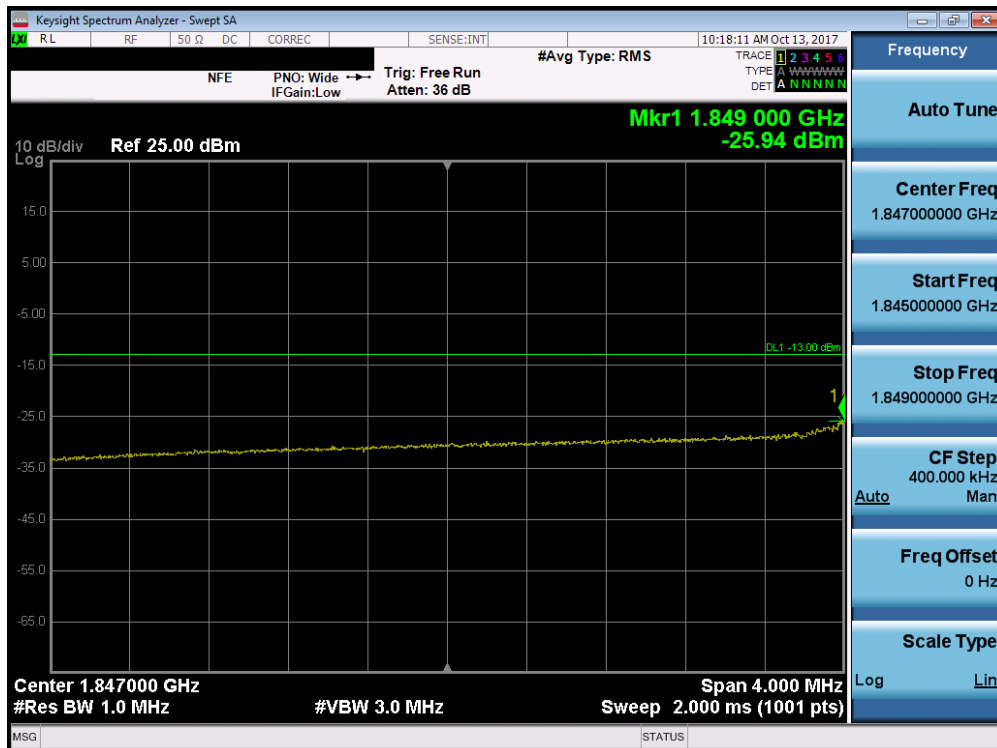
Plot 7-192. Lower Extended Band Edge Plot (Band 2/25 - 10.0MHz QPSK - Full RB Configuration)
