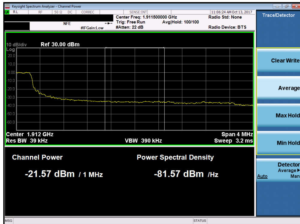
Plot 7-190. Upper Extended Band Edge Plot (Band 2 - 5.0MHz QPSK - Full RB Configuration)
