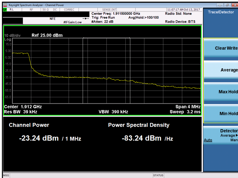
Plot 7-184. Upper Extended Band Edge Plot (Band 2 - 3.0MHz QPSK - Full RB Configuration)
