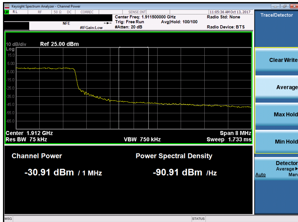
Plot 7-196. Upper Extended Band Edge Plot (Band 2 - 10.0MHz QPSK - Full RB Configuration)
