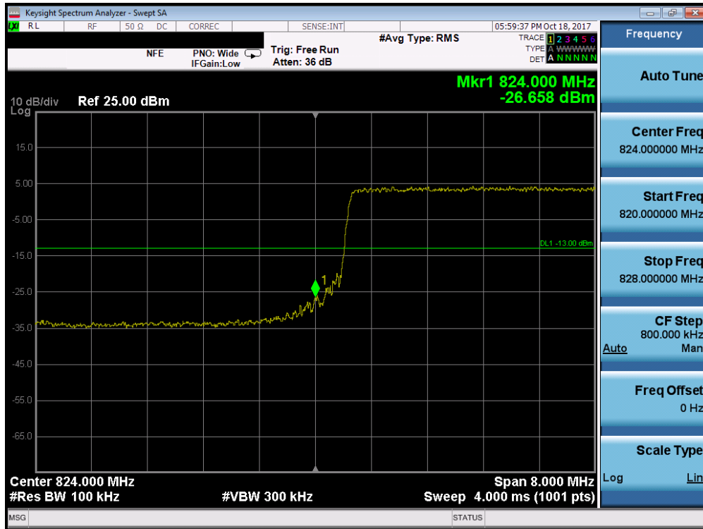
Plot 7-133. Lower Band Edge Plot (Band 5/26 - 10.0MHz QPSK - Full RB Configuration)
