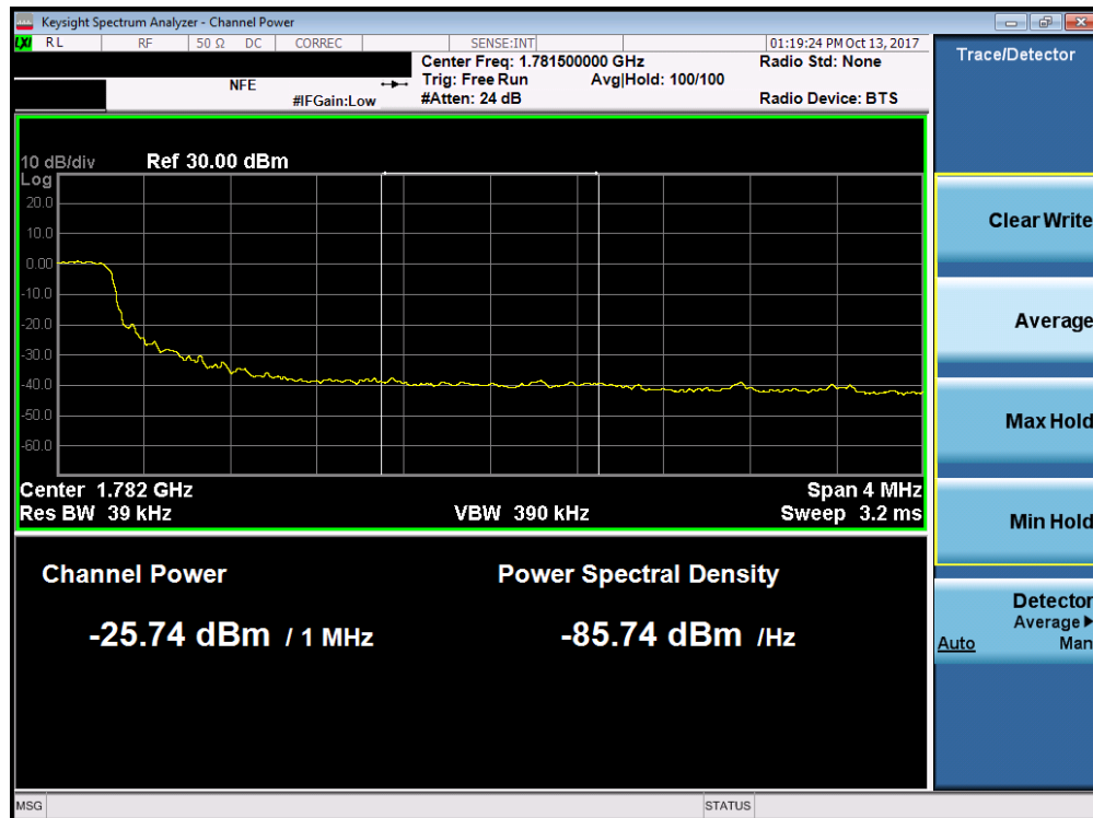
Plot 7-152. Upper Extended Band Edge Plot (Band 66 - 5.0MHz QPSK - Full RB Configuration)
