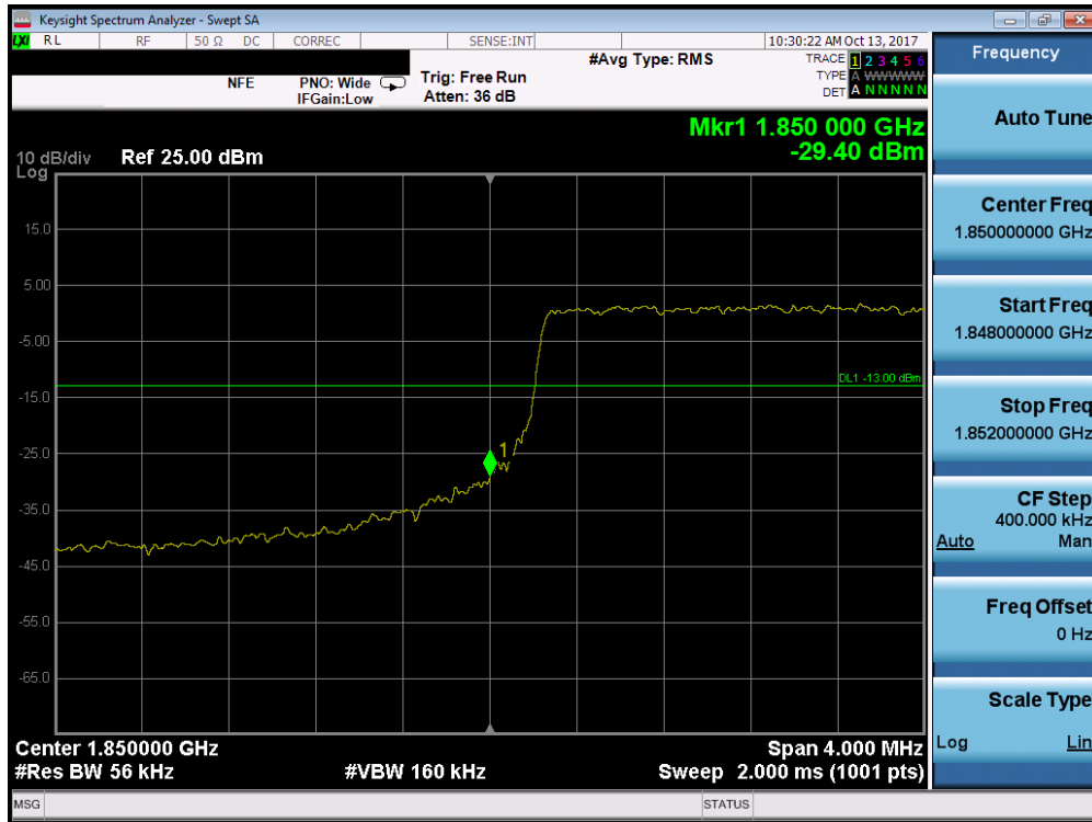
Plot 7-185. Lower Band Edge Plot (Band 2/25 - 5.0MHz QPSK - Full RB Configuration)
