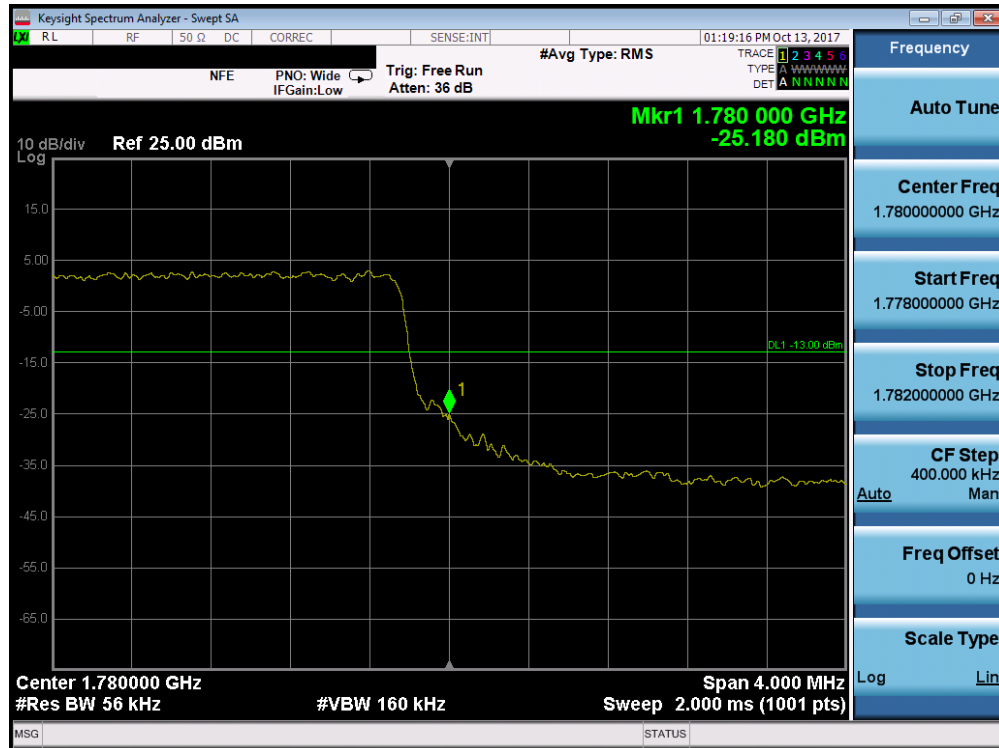
Plot 7-151. Upper Band Edge Plot (Band 66 - 5.0MHz QPSK - Full RB Configuration)
