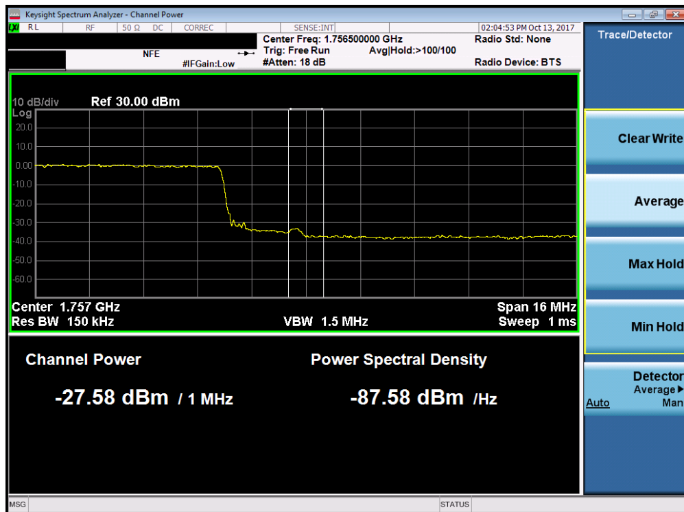
Plot 7-172. Upper Extended Band Edge Plot (Band 4 – 20.0MHz QPSK - Full RB Configuration)
