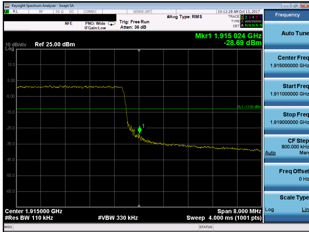
Plot 7-193. Upper Band Edge Plot (Band 25 - 10.0MHz QPSK - Full RB Configuration)
