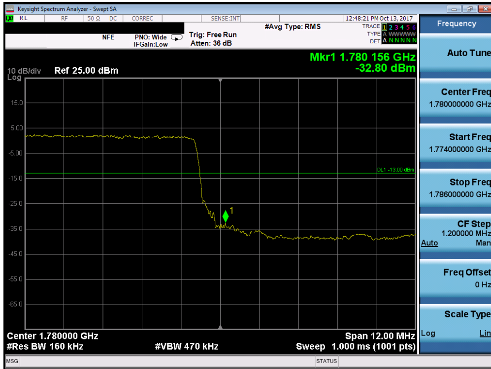
Plot 7-163. Upper Band Edge Plot (Band 66 - 15.0MHz QPSK - Full RB Configuration)
