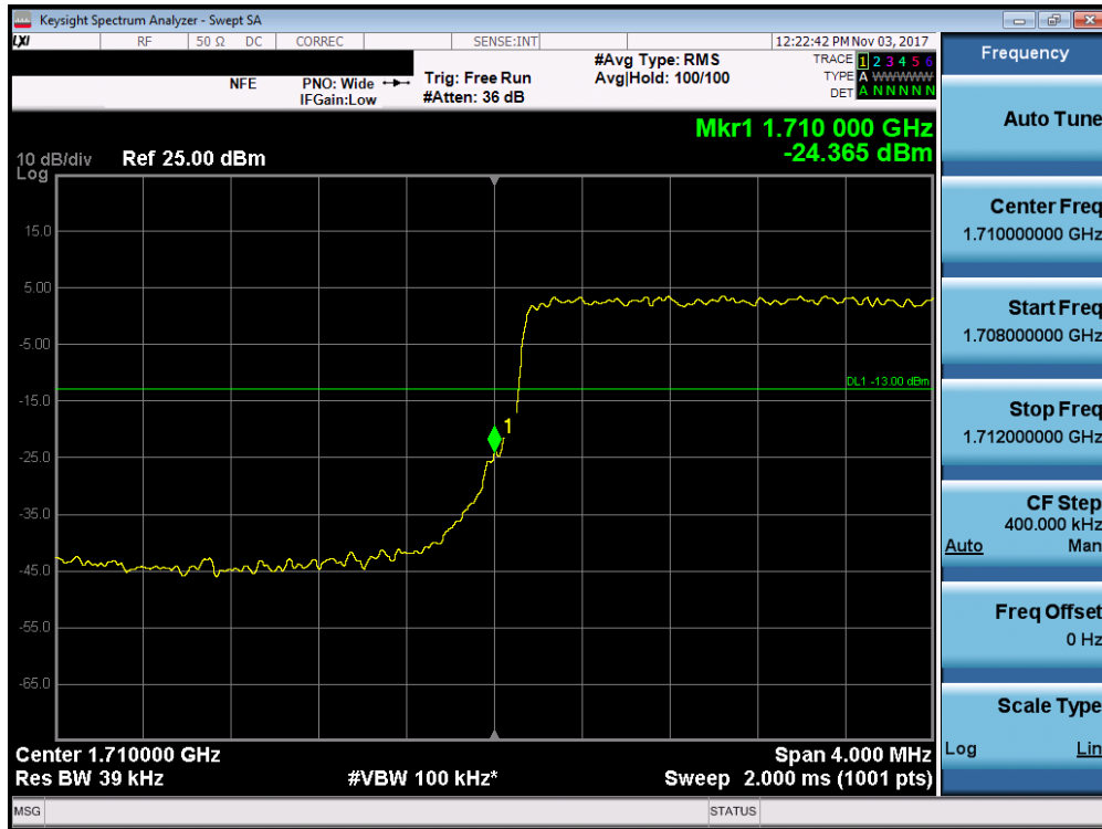
Plot 7-143. Lower Band Edge Plot (Band 4/66 - 3.0MHz QPSK - Full RB Configuration)
