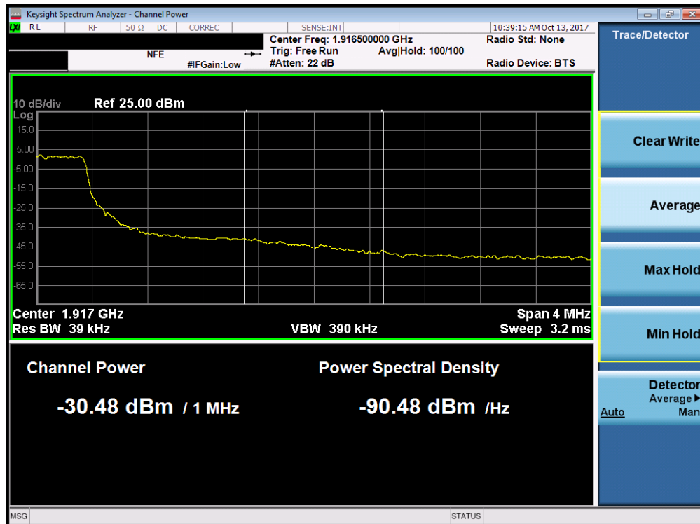
Plot 7-182. Upper Extended Band Edge Plot (Band 25 - 3.0MHz QPSK - Full RB Configuration)
