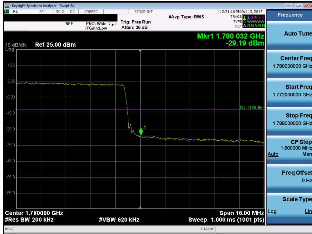
Plot 7-169. Upper Band Edge Plot (Band 66 - 20.0MHz QPSK - Full RB Configuration)
