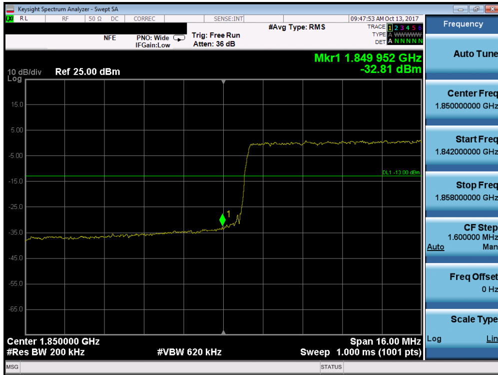
Plot 7-203. Lower Band Edge Plot (Band 2/25 - 20.0MHz QPSK - Full RB Configuration)
