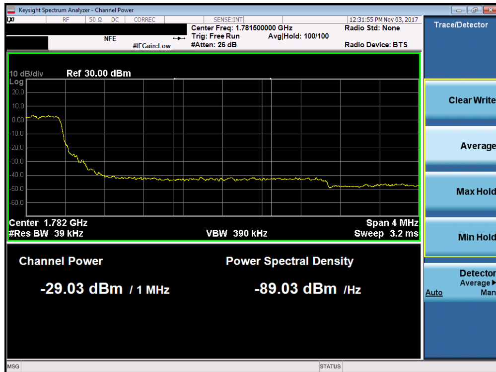
Plot 7-146. Upper Extended Band Edge Plot (Band 66 - 3.0MHz QPSK - Full RB Configuration)
