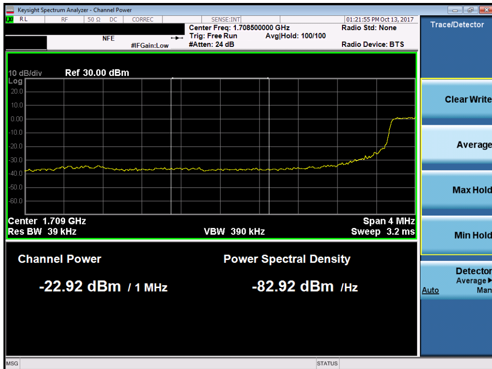
Plot 7-150. Lower Extended Band Edge Plot (Band 4/66 - 5.0MHz QPSK - Full RB Configuration)
