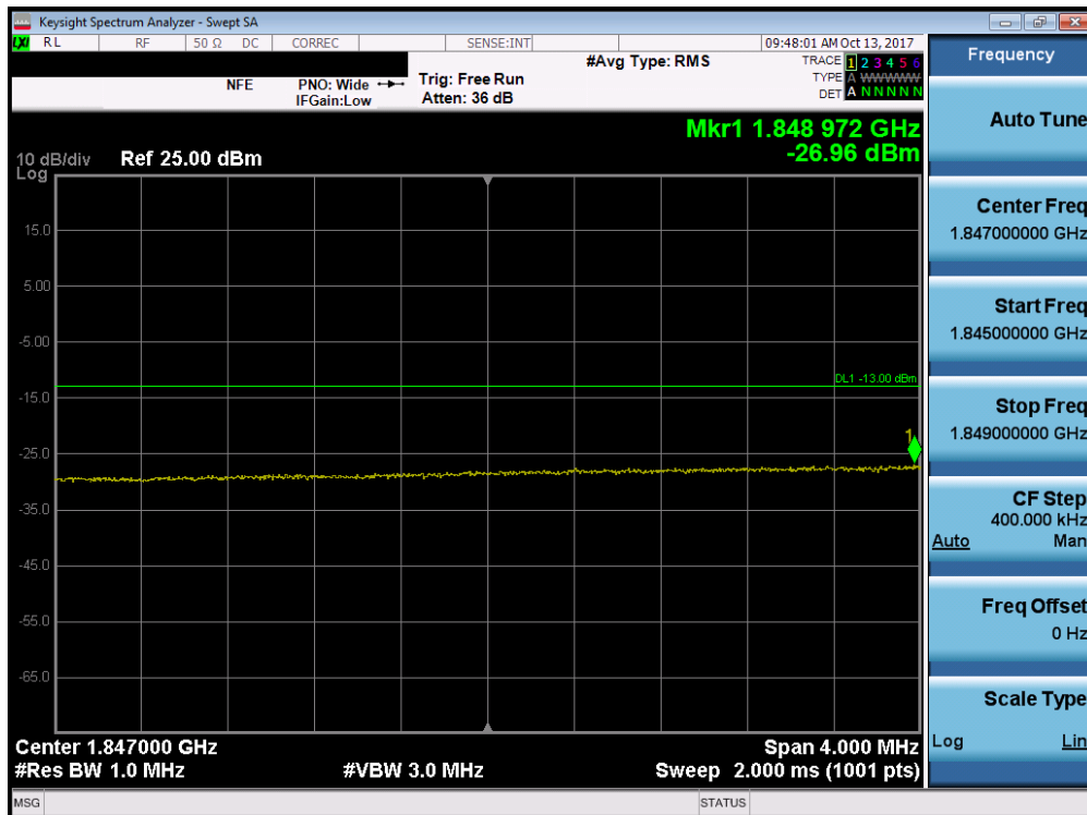
Plot 7-204. Lower Extended Band Edge Plot (Band 2/25 - 20.0MHz QPSK - Full RB Configuration)
