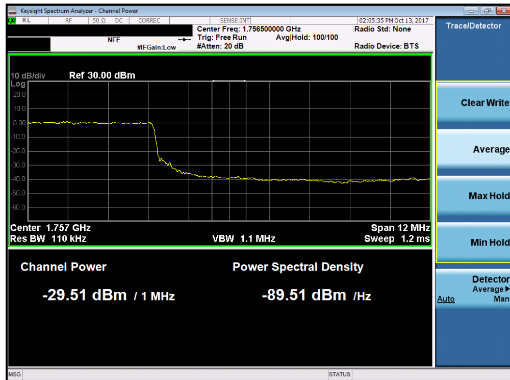
Plot 7-166. Upper Extended Band Edge Plot (Band 4 – 15.0MHz QPSK - Full RB Configuration)
