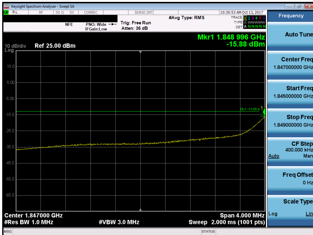
Plot 7-186. Lower Extended Band Edge Plot (Band 2/25 - 5.0MHz QPSK - Full RB Configuration)
