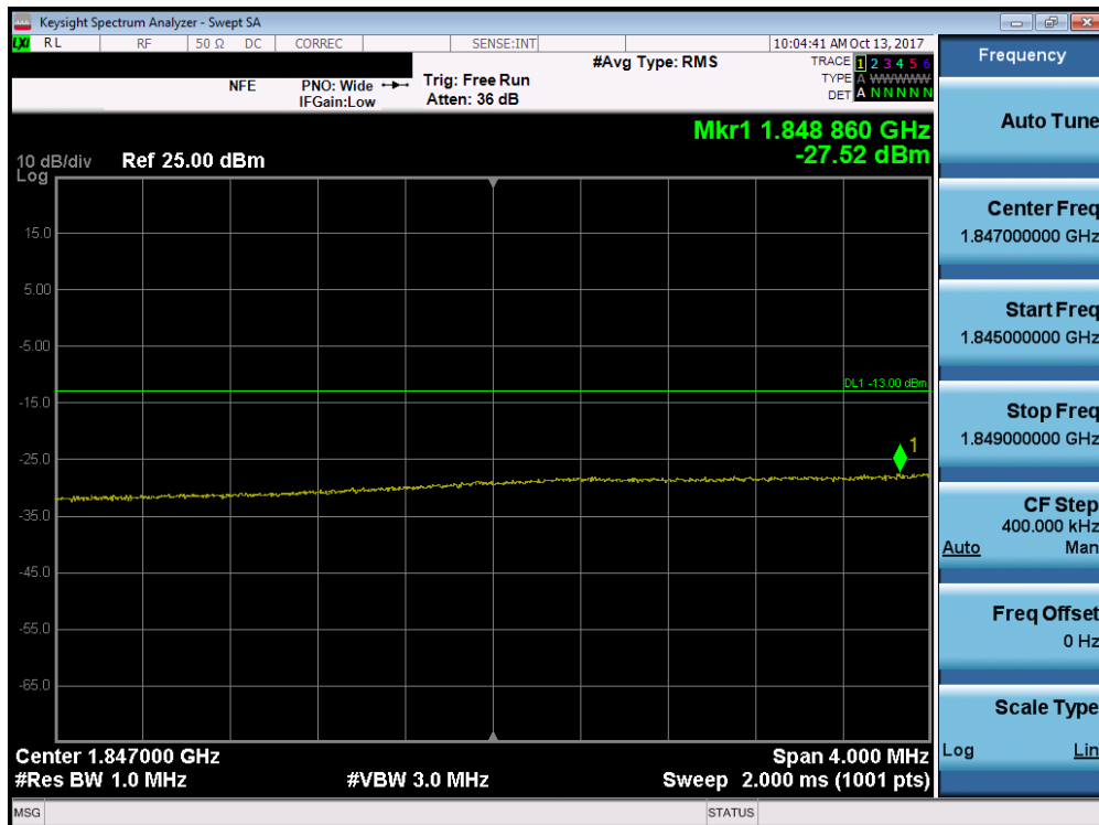
Plot 7-198. Lower Extended Band Edge Plot (Band 2/25 - 15.0MHz QPSK - Full RB Configuration)
