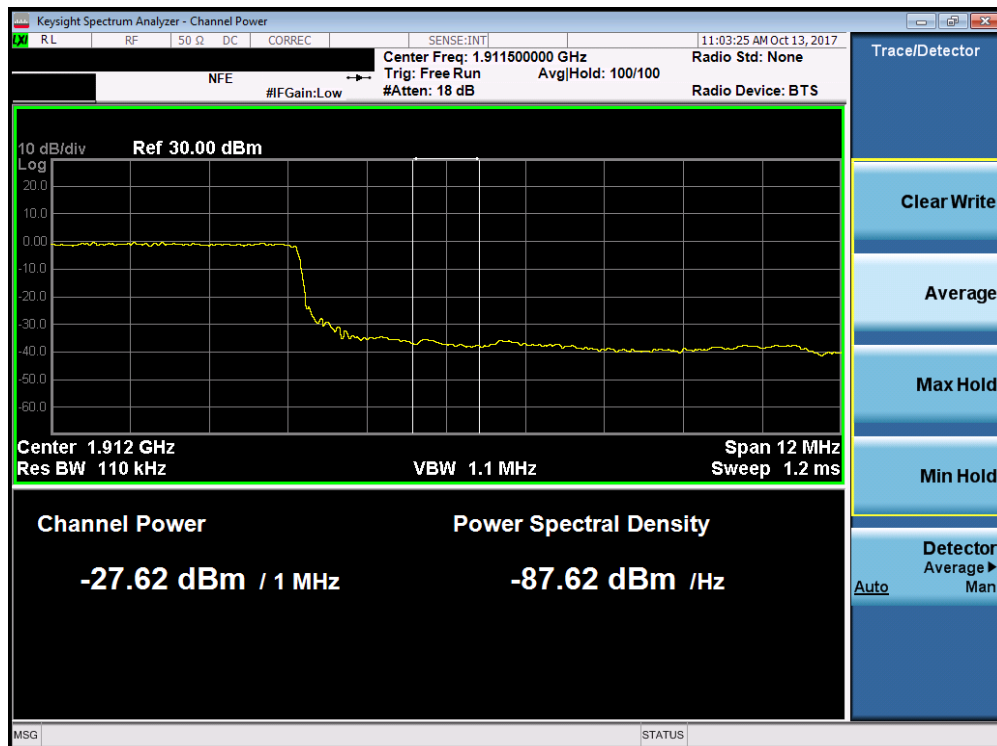
Plot 7-202. Upper Extended Band Edge Plot (Band 2 - 15.0MHz QPSK - Full RB Configuration)
