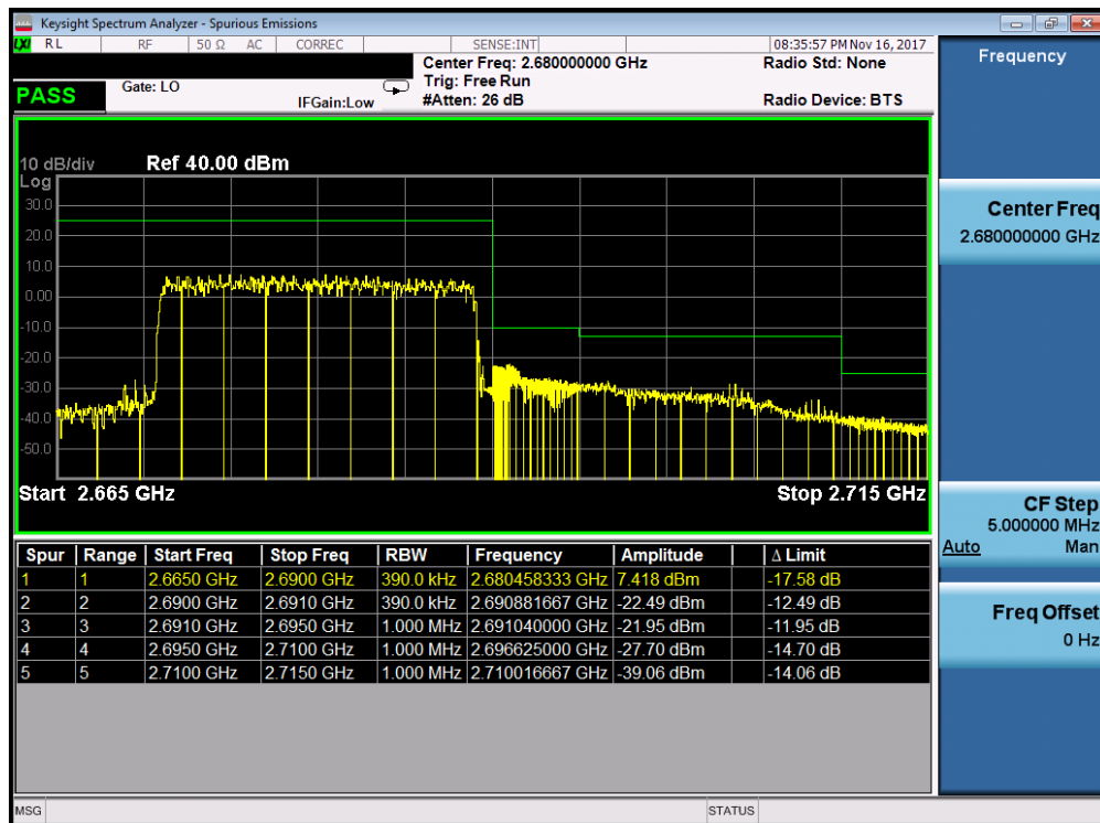
Plot 7-216. Upper ACP Plot (Band 41 - 20.0MHz QPSK - Full RB Configuration)
