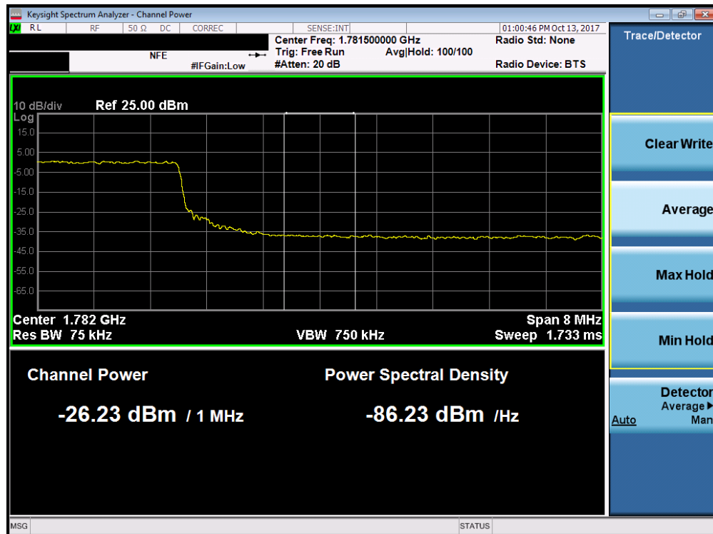
Plot 7-158. Upper Extended Band Edge Plot (Band 66 - 10.0MHz QPSK - Full RB Configuration)
