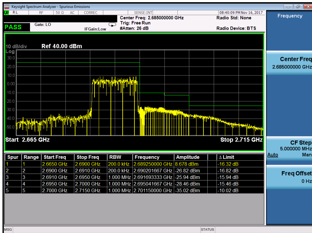
Plot 7-212. Upper ACP Plot (Band 41 - 10.0MHz QPSK - Full RB Configuration)
