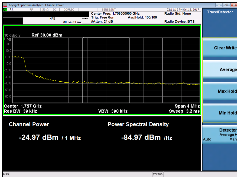
Plot 7-154. Upper Extended Band Edge Plot (Band 4 – 5.0MHz QPSK - Full RB Configuration)
