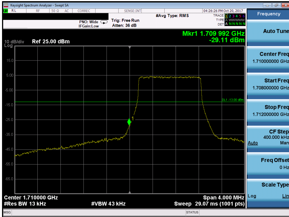
Plot 7-137. Lower Band Edge Plot (Band 4/66 - 1.4MHz QPSK - Full RB Configuration)
