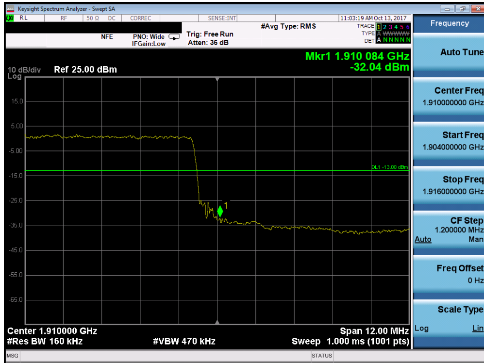
Plot 7-201. Upper Band Edge Plot (Band 2 – 15.0MHz QPSK - Full RB Configuration)
