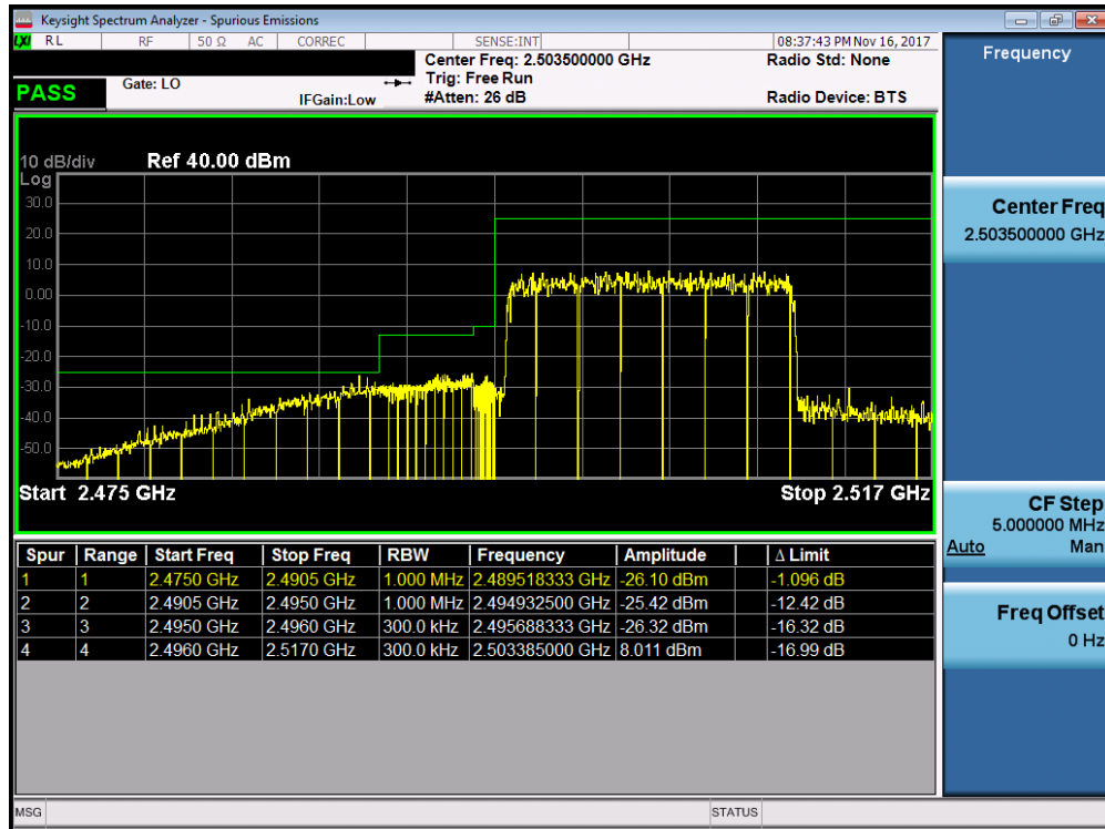
Plot 7-213. Lower ACP Plot (Band 41 - 15.0MHz QPSK - Full RB Configuration)
