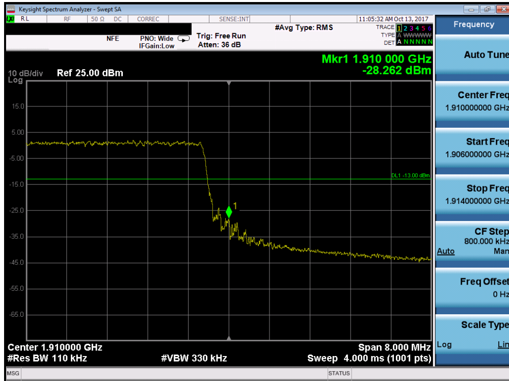
Plot 7-195. Upper Band Edge Plot (Band 2 – 10.0MHz QPSK - Full RB Configuration)
