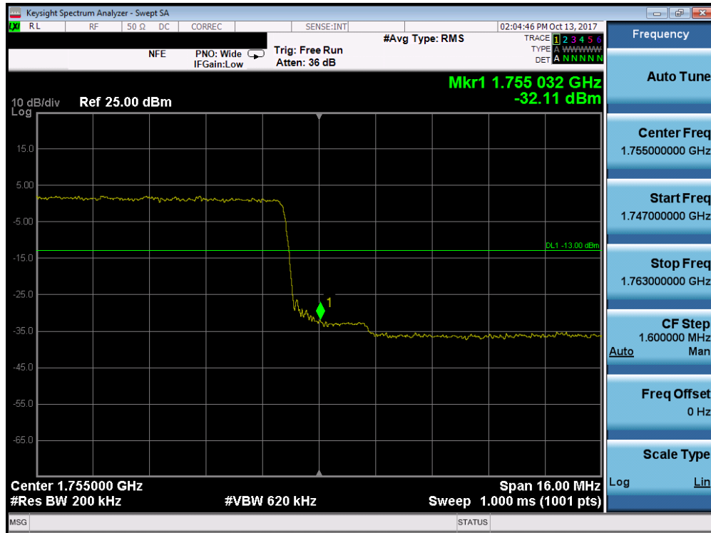
Plot 7-171. Upper Band Edge Plot (Band 4 – 20.0MHz QPSK - Full RB Configuration)
