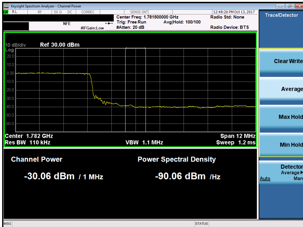
Plot 7-164. Upper Extended Band Edge Plot (Band 66 - 15.0MHz QPSK - Full RB Configuration)
