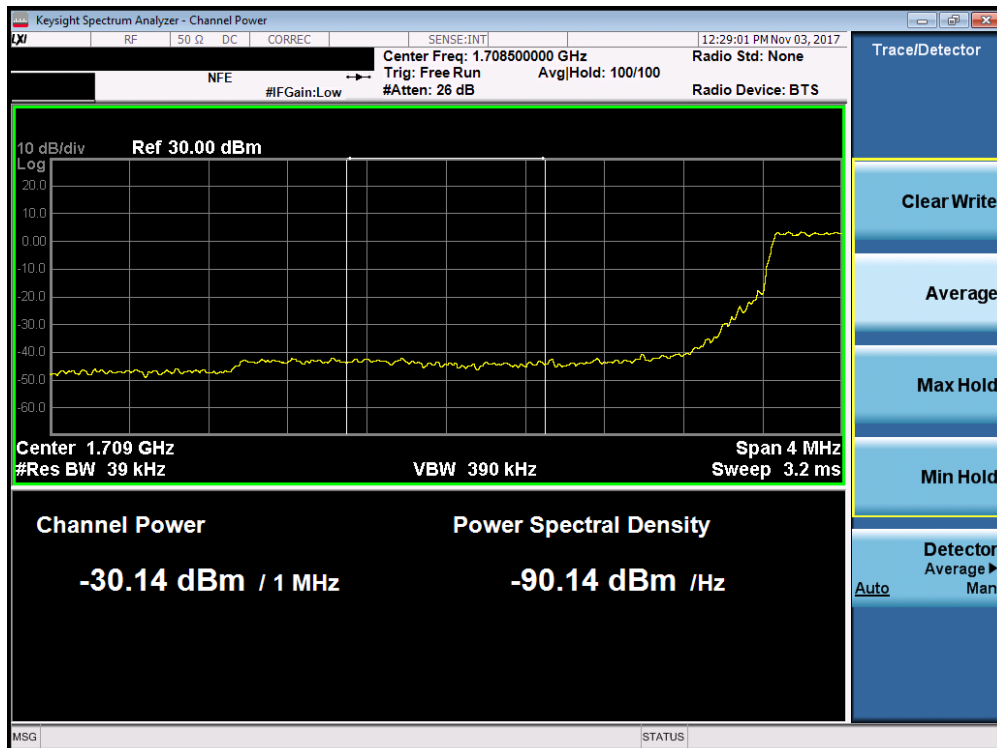
Plot 7-144. Lower Extended Band Edge Plot (Band 4/66 - 3.0MHz QPSK - Full RB Configuration)
