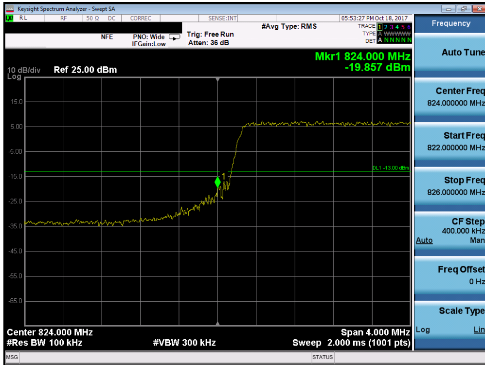
Plot 7-131. Lower Band Edge Plot (Band 5/26 - 5.0MHz QPSK - Full RB Configuration)
