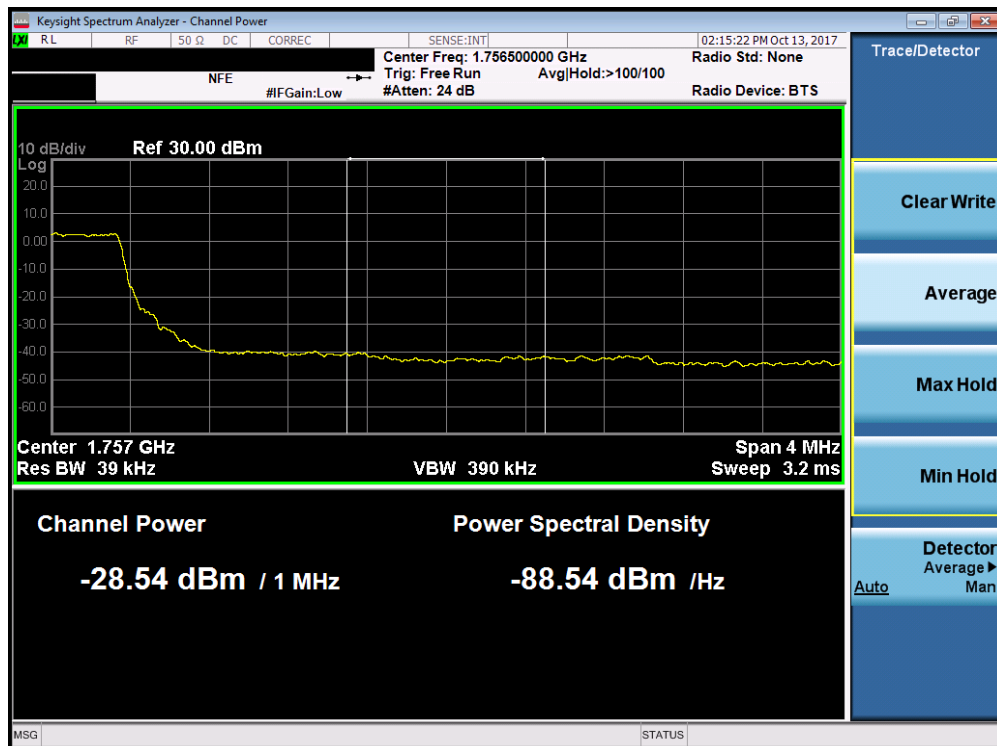
Plot 7-148. Upper Extended Band Edge Plot (Band 4 - 3.0MHz QPSK - Full RB Configuration)
