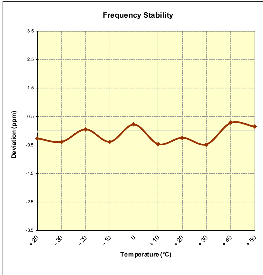
Figure 7-6. LTE Band 26 Frequency Stability Data (Ch. 26697)
