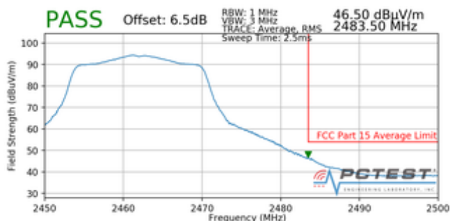
Plot 7-79. Radiated Restricted Upper Band Edge Measurement (Average)
