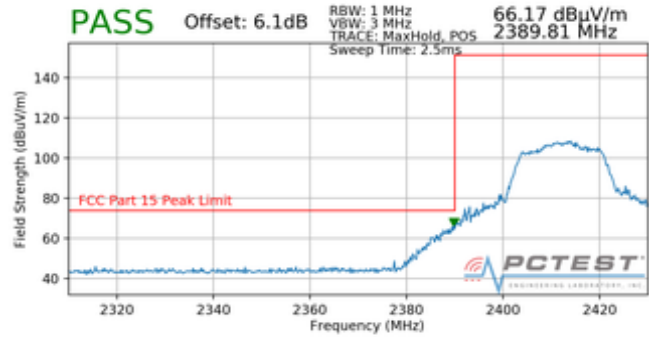
Plot 7-94. Radiated Restricted Lower Band Edge Measurement (Peak)
