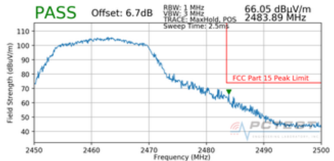
Plot 7-86. Radiated Restricted Upper Band Edge Measurement (Peak)
