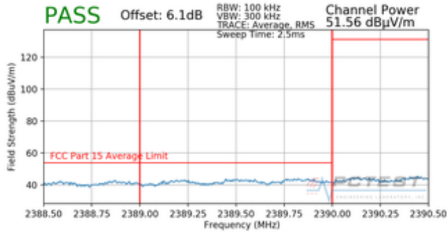
Plot 7-93. Radiated Restricted Lower Band Edge Measurement (Average)
