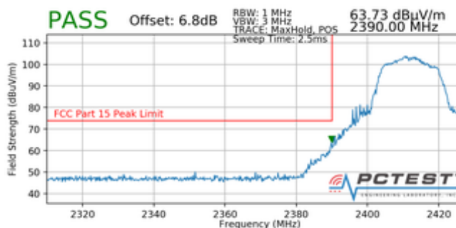
Plot 7-78. Radiated Restricted Lower Band Edge Measurement (Peak)
