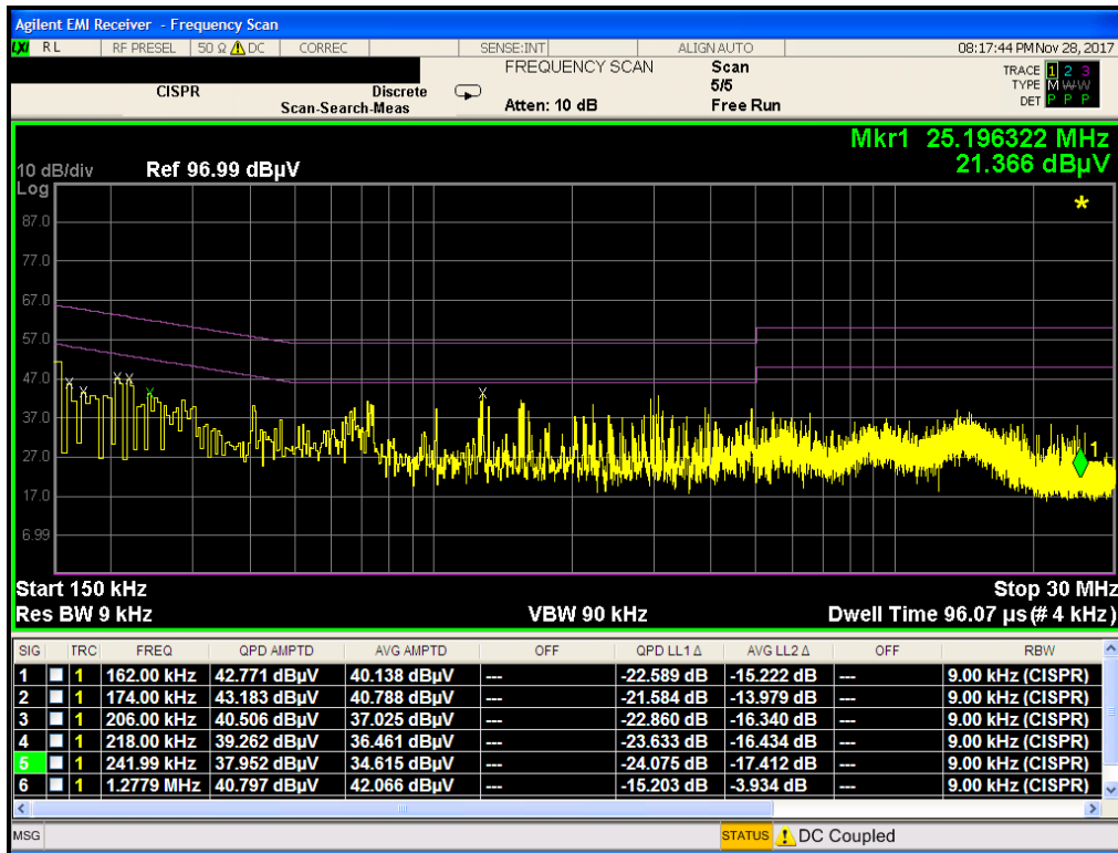
Plot 7-105. Line Conducted Plot with 802.11b (L1) (with WCP)
