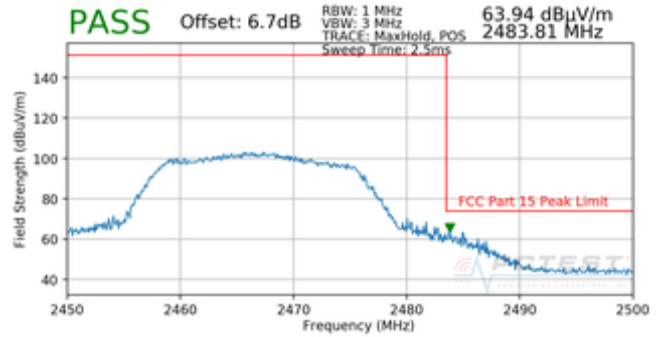
Plot 7-98. Radiated Restricted Band Edge Measurement with WCP (Peak)
