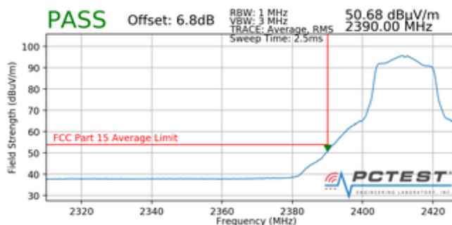
Plot 7-77. Radiated Restricted Lower Band Edge Measurement (Average)
