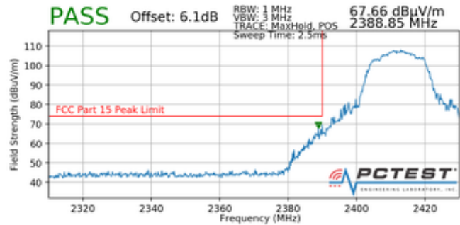
Plot 7-88. Radiated Restricted Band Edge Measurement with WCP (Peak)
