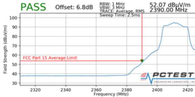
Plot 7-81. Radiated Restricted Band Edge Measurement with WCP (Average)
