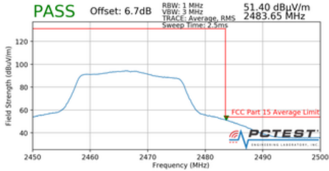
Plot 7-97. Radiated Restricted Band Edge Measurement with WCP (Average)
