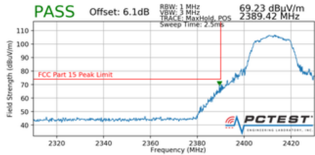
Plot 7-84. Radiated Restricted Lower Band Edge Measurement (Peak)
