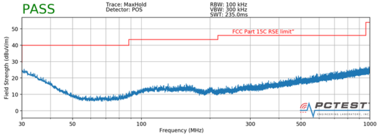
Plot 7-100. Radiated Spurious Plot below 1GHz (Pol. V)
