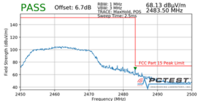
Plot 7-96. Radiated Restricted Upper Band Edge Measurement (Peak)
