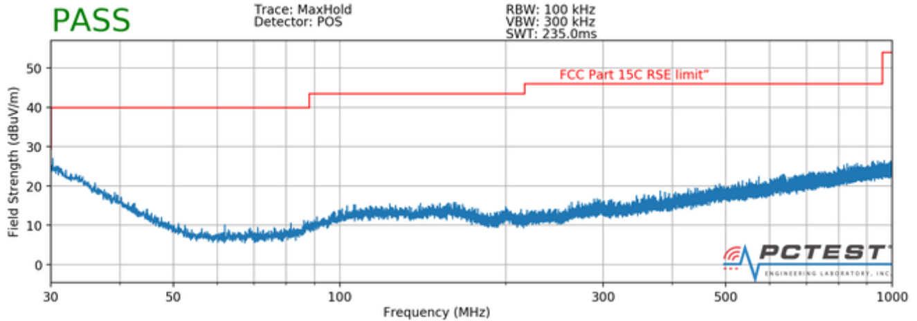
Plot 7-99. Radiated Spurious Plot below 1GHz (Pol. H)
