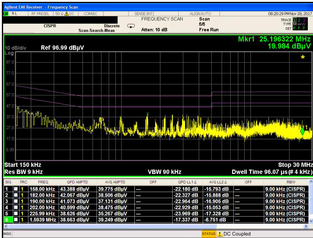
Plot 7-106. Line Conducted Plot with 802.11b (N) (with WCP)
