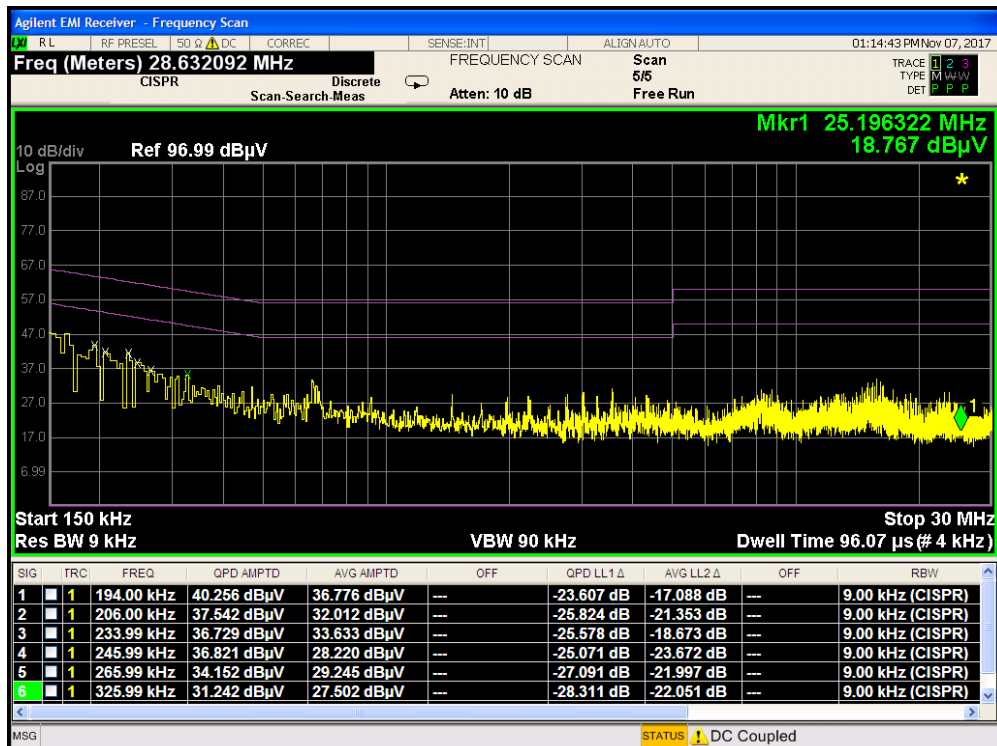
Plot 7-59. Line-Conducted Test Plot with WCP(N)
