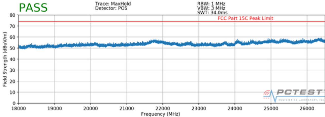
Plot 7-49. Radiated Spurious Plot above 18GHz (Pol. V)
