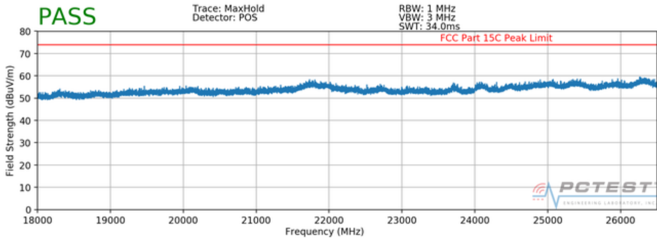
Plot 7-48. Radiated Spurious Plot above 18GHz (Pol. H)
