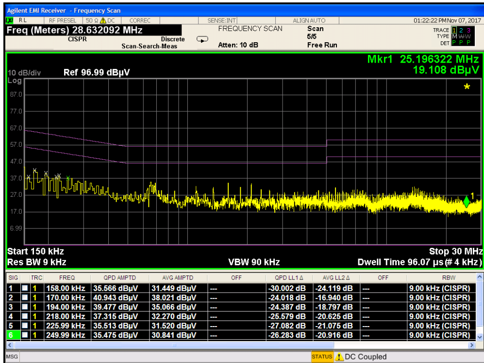
Plot 7-58. Line-Conducted Test Plot with WCP(L1)
