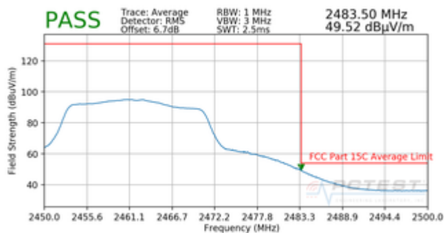
Plot 7-13. Radiated Restricted Band Edge Measurement with WCP (Average)
