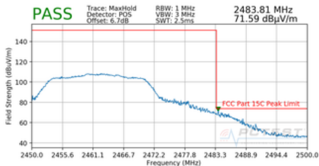
Plot 7-18. Radiated Restricted Upper Band Edge Measurement (Peak)
