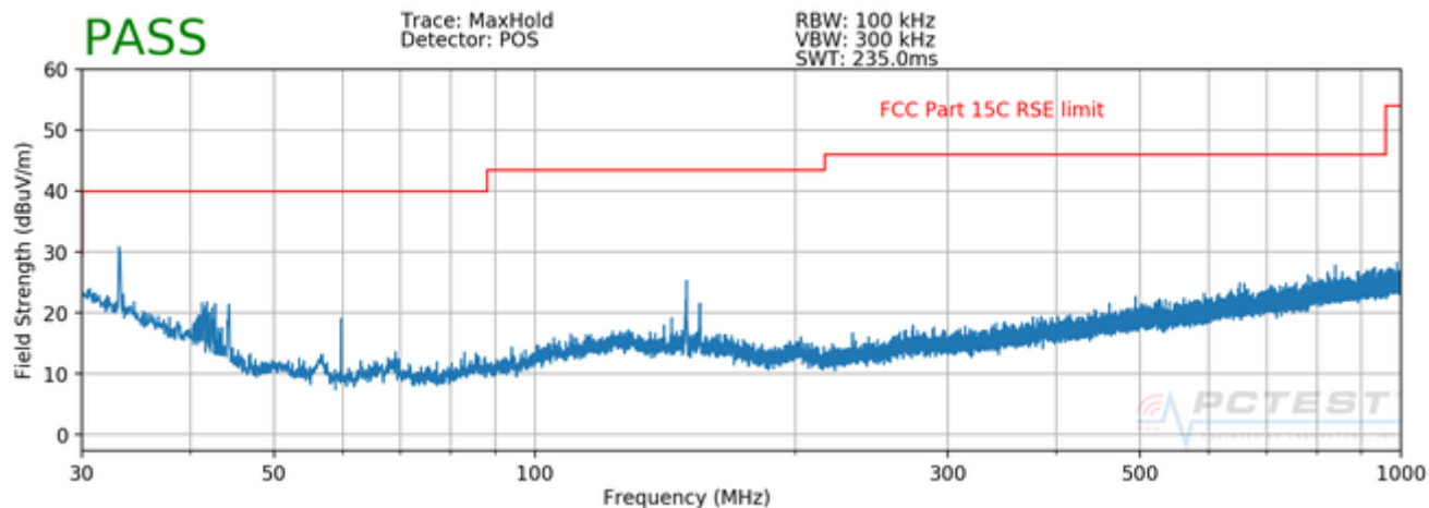
Plot 7-28. Radiated Spurious Plot below 1GHz (Pol. V)
