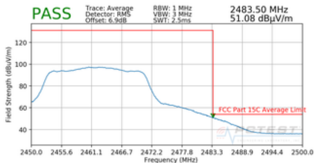
Plot 7-17. Radiated Restricted Upper Band Edge Measurement (Average)
