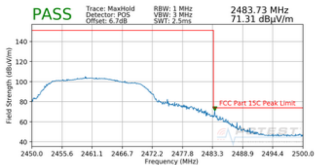
Plot 7-14. Radiated Restricted Band Edge Measurement with WCP (Peak)
