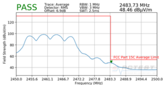
Plot 7-25. Radiated Restricted Band Edge Measurement with WCP (Average)
