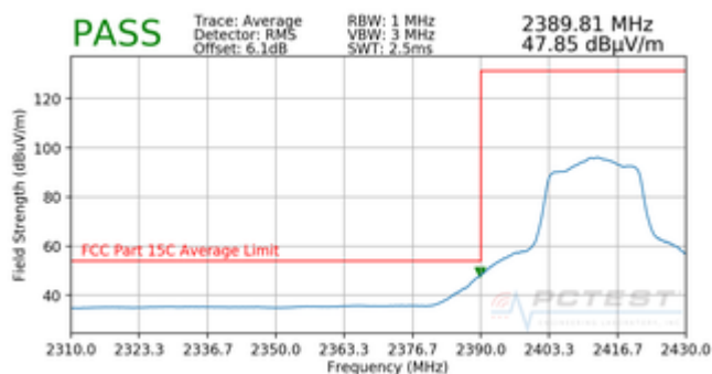
Plot 7-9. Radiated Restricted Lower Band Edge Measurement (Average)
