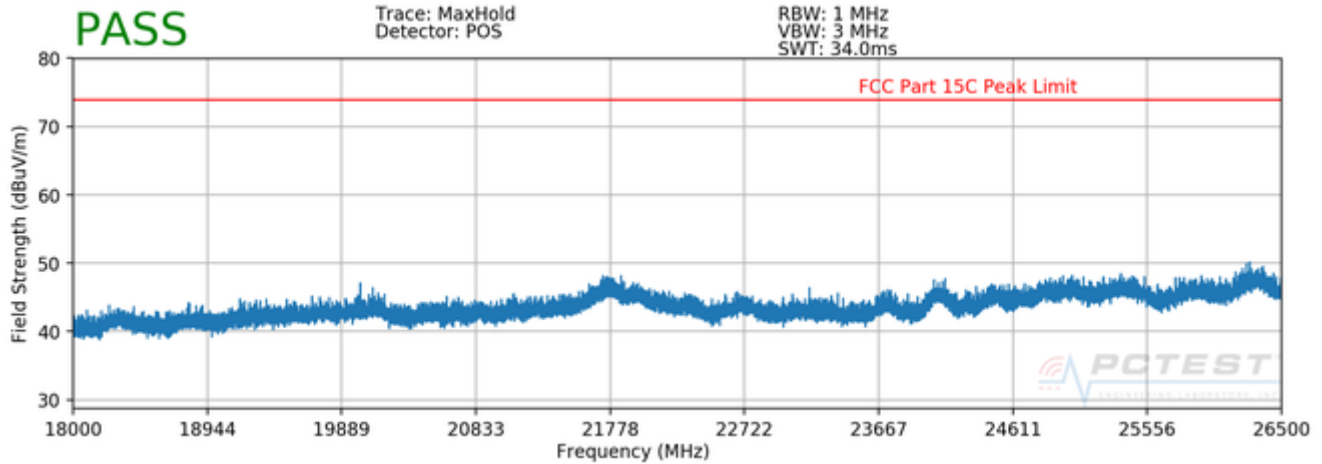
Plot 7-7. Radiated Spurious Plot above 18GHz (Pol. H)
