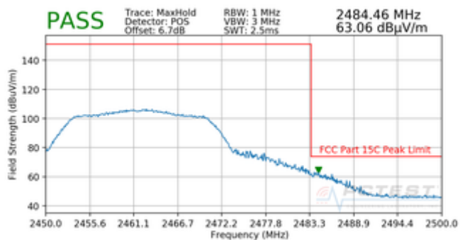
Plot 7-20. Radiated Restricted Band Edge Measurement with WCP (Peak)
