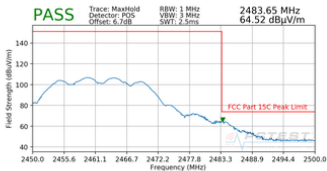
Plot 7-26. Radiated Restricted Band Edge Measurement with WCP (Peak)
