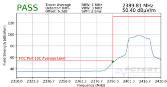
Plot 7-15. Radiated Restricted Lower Band Edge Measurement (Average)
