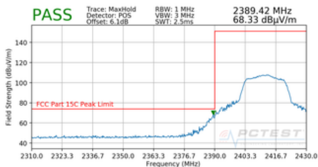
Plot 7-16. Radiated Restricted Lower Band Edge Measurement (Peak)
