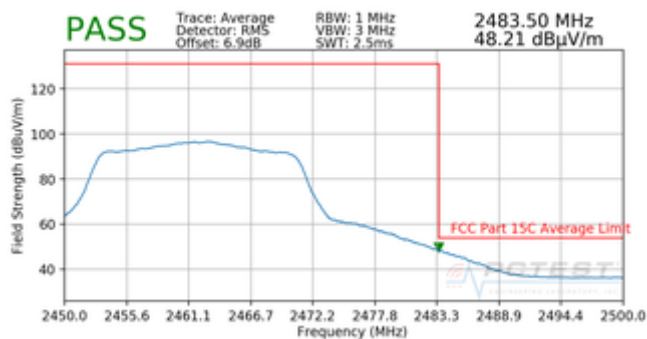
Plot 7-19. Radiated Restricted Band Edge Measurement with WCP (Average)
