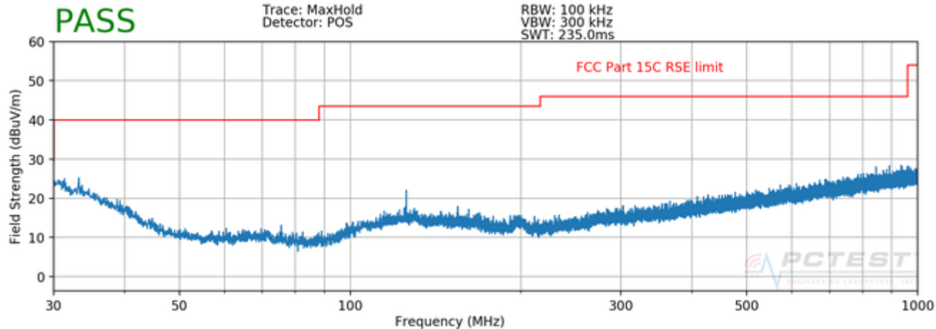
Plot 7-27. Radiated Spurious Plot below 1GHz (Pol. H)
