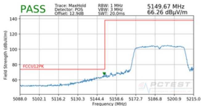
Plot 7-50. Radiated Lower Band Edge Plot (Peak – UNII Band 1)
