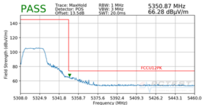
Plot 7-16. Radiated Upper Band Edge Plot (Peak – UNII Band 2A)
