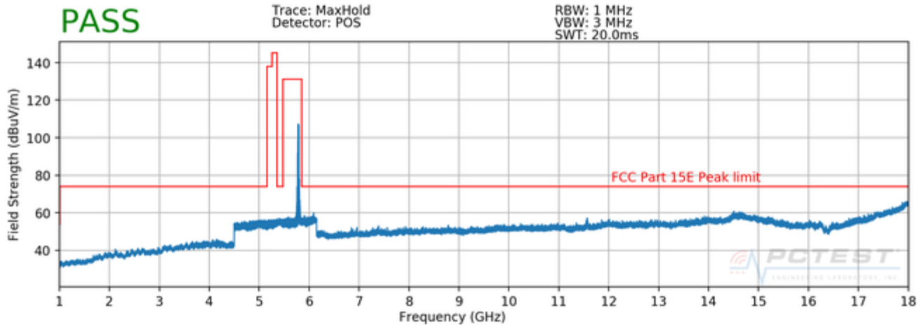
Plot 7-7. Radiated Spurious Plot above 1GHz (802.11a – U3 Ch. 157, Ant. Pol. H)
