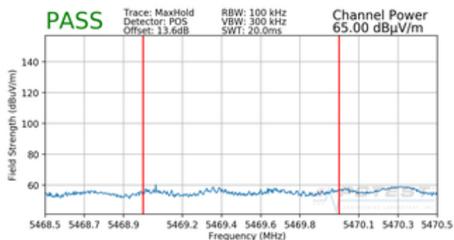
Plot 7-54. Radiated Lower Band Edge Plot (Peak – UNII Band 2C)
