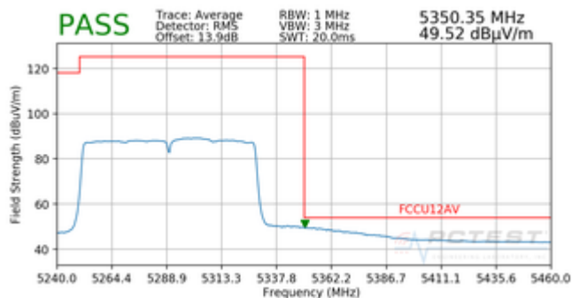
Plot 7-33. Radiated Upper Band Edge Plot (Average – UNII Band 2A)
