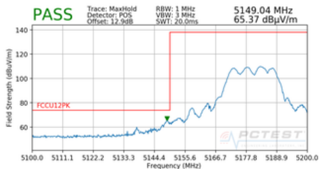
Plot 7-68. Radiated Lower Band Edge Plot (Peak – UNII Band 1)
