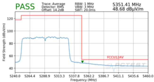
Plot 7-65. Radiated Band Edge Plot (Average – WCP)
