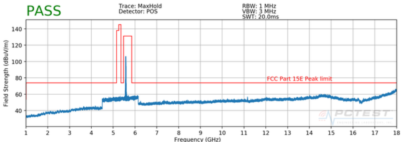
Plot 7-6. Radiated Spurious Plot above 1GHz (802.11a – U2C Ch. 116, Ant. Pol. V)
