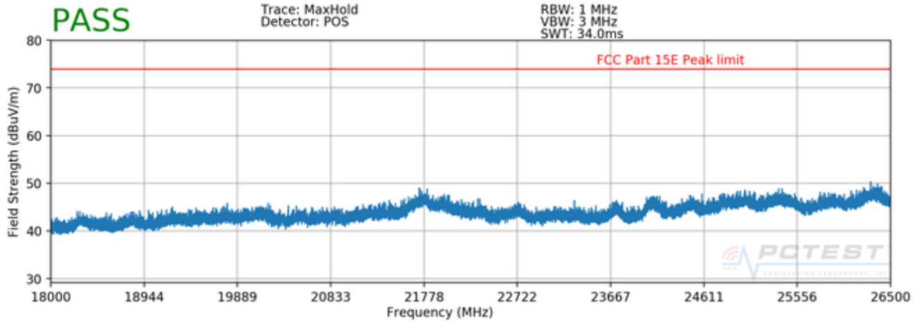
Plot 7-9. Radiated Spurious Plot 18GHz - 26.5GHz (802.11a – Ant. Pol. H)
