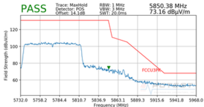
Plot 7-64. Radiated Upper Band Edge Plot (Peak – UNII Band 3)
