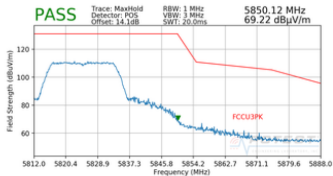
Plot 7-46. Radiated Upper Band Edge Plot (Peak – UNII Band 3)
