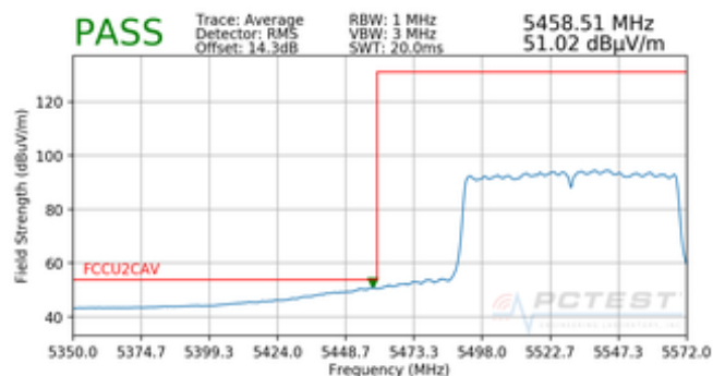
Plot 7-62. Radiated Lower Band Edge Plot (Average – UNII Band 2C)
