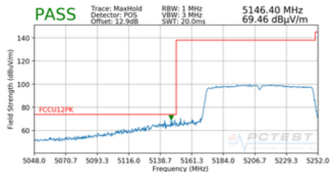
Plot 7-39. Radiated Band Edge Plot (Peak – WCP)
