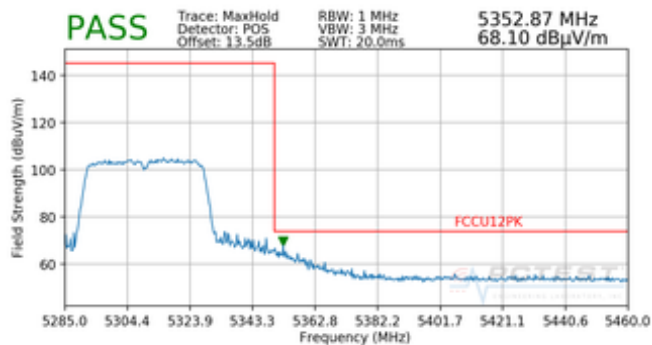
Plot 7-52. Radiated Upper Band Edge Plot (Peak – UNII Band 2A)
