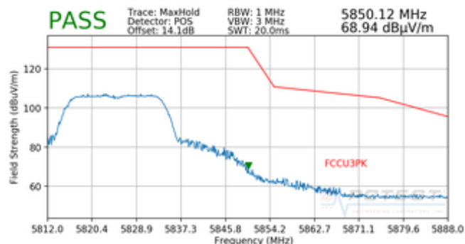
Plot 7-19. Radiated Upper Band Edge Plot (Peak – UNII Band 3)
