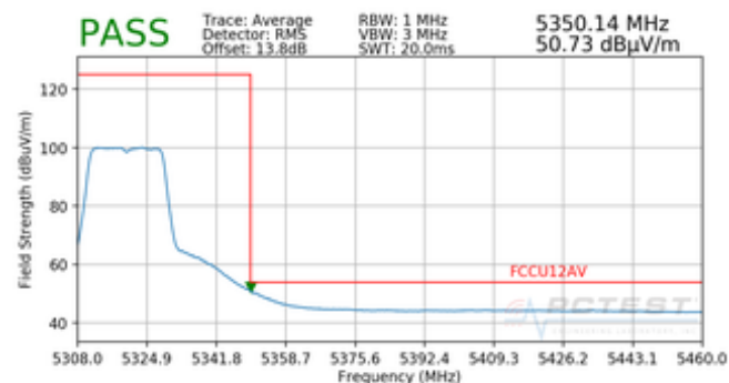
Plot 7-42. Radiated Upper Band Edge Plot (Average – UNII Band 2A)
