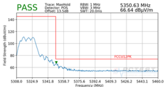
Plot 7-70. Radiated Upper Band Edge Plot (Peak – UNII Band 2A)
