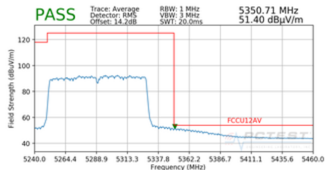
Plot 7-60. Radiated Upper Band Edge Plot (Average – UNII Band 2A)
