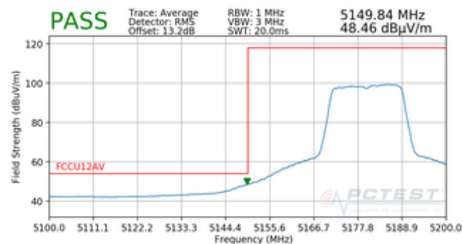
Plot 7-40. Radiated Lower Band Edge Plot (Average – UNII Band 1)
