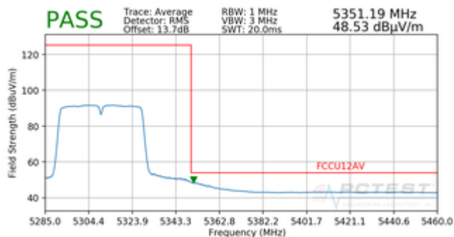
Plot 7-29. Radiated Band Edge Plot (Average – WCP)
