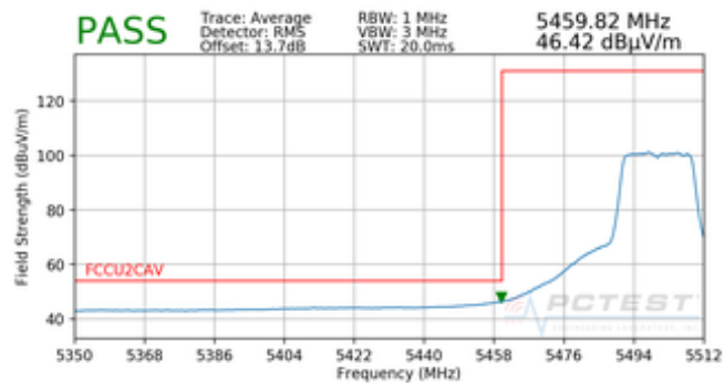
Plot 7-44. Radiated Lower Band Edge Plot (Average – UNII Band 2C)
