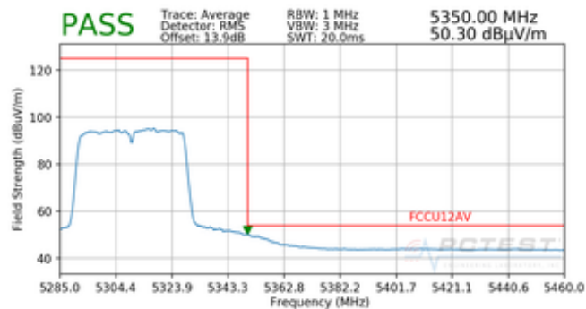
Plot 7-51. Radiated Upper Band Edge Plot (Average – UNII Band 2A)
