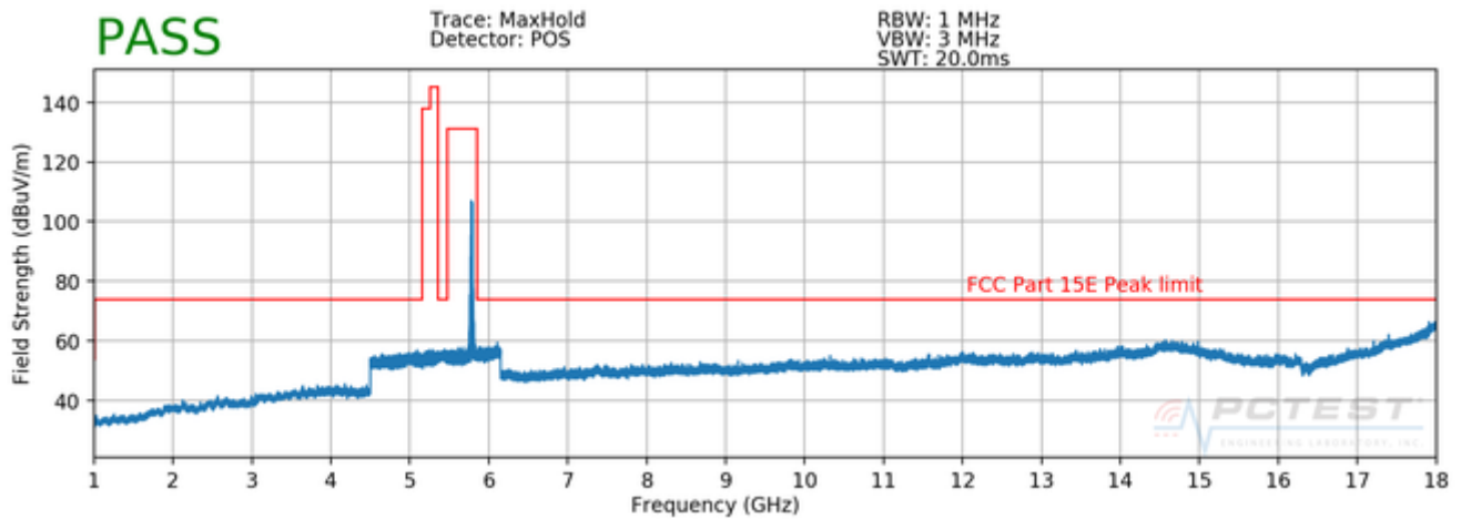
Plot 7-8. Radiated Spurious Plot above 1GHz (802.11a – U3 Ch. 157, Ant. Pol. V)
