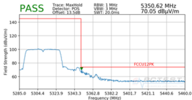
Plot 7-30. Radiated Band Edge Plot (Peak – WCP)
