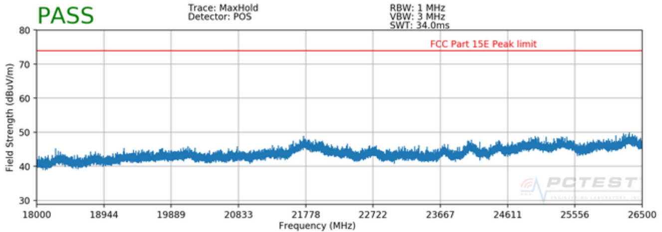
Plot 7-10. Radiated Spurious Plot above 18GHz - 26.5GHz (802.11a – Ant. Pol. V)
