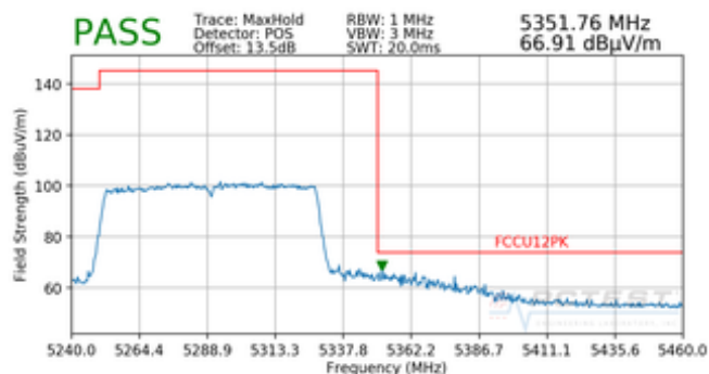
Plot 7-61. Radiated Upper Band Edge Plot (Peak – UNII Band 2A)
