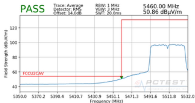
Plot 7-53. Radiated Lower Band Edge Plot (Average – UNII Band 2C)
