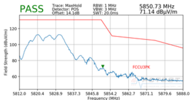
Plot 7-73. Radiated Upper Band Edge Plot (Peak – UNII Band 3)
