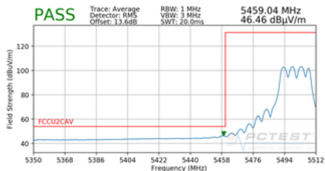
Plot 7-71. Radiated Lower Band Edge Plot (Average – UNII Band 2C)
