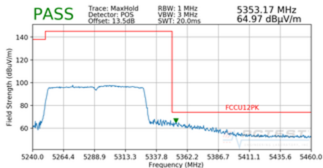
Plot 7-34. Radiated Upper Band Edge Plot (Peak – UNII Band 2A)
