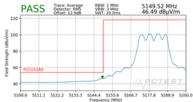
Plot 7-67. Radiated Lower Band Edge Plot (Average – UNII Band 1)
