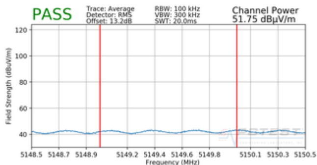
Plot 7-31. Radiated Lower Band Edge Plot (Average – UNII Band 1)
