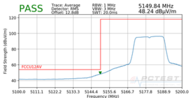
Plot 7-13. Radiated Lower Band Edge Plot (Average – UNII Band 1)
