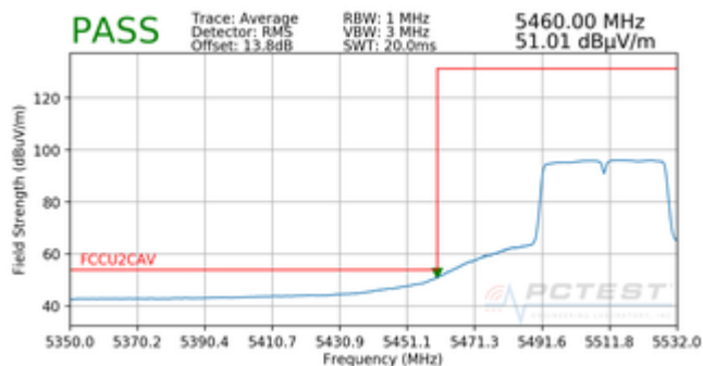
Plot 7-26. Radiated Lower Band Edge Plot (Average – UNII Band 2C)
