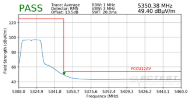
Plot 7-15. Radiated Upper Band Edge Plot (Average – UNII Band 2A)
