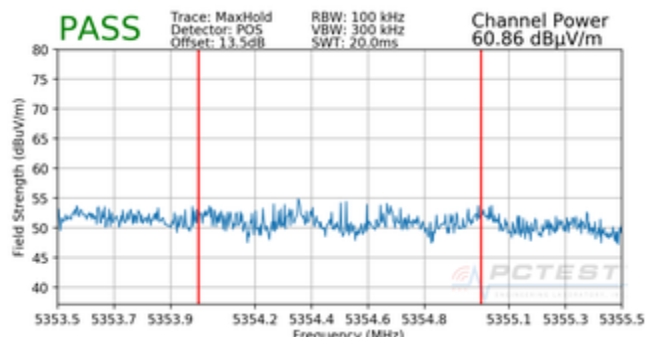
Plot 7-25. Radiated Upper Band Edge Plot (Peak – UNII Band 2A)
