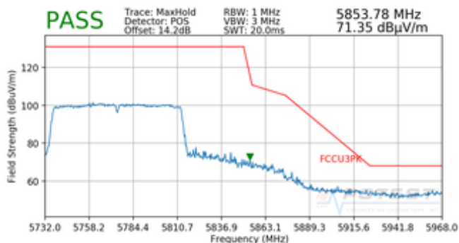
Plot 7-37. Radiated Upper Band Edge Plot (Peak – UNII Band 3)
