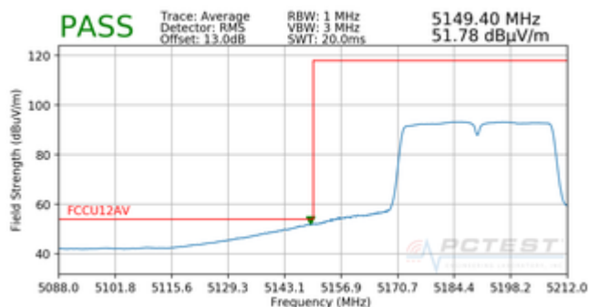
Plot 7-22. Radiated Lower Band Edge Plot (Average – UNII Band 1)
