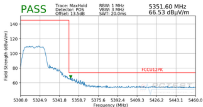
Plot 7-43. Radiated Upper Band Edge Plot (Peak – UNII Band 2A)
