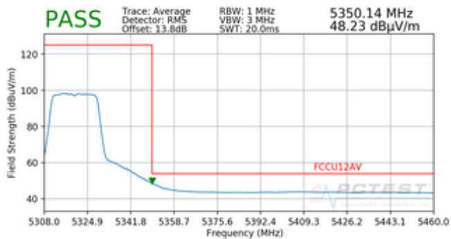
Plot 7-47. Radiated Band Edge Plot (Average – WCP)
