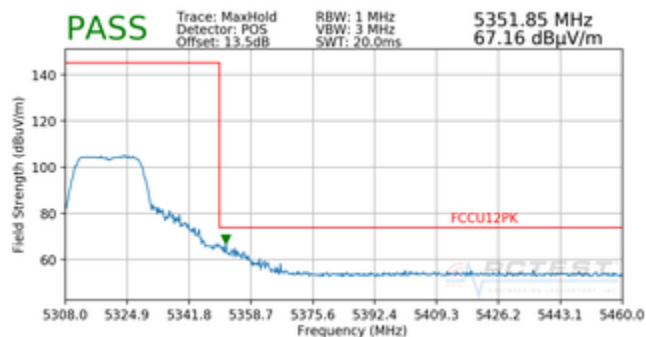
Plot 7-21. Radiated Band Edge Plot (Peak – WCP)
