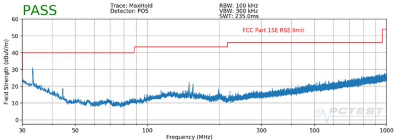
Plot 7-77. Radiated Spurious Plot below 1GHz (802.11a – U3 Ch. 157, Ant. Pol. V)
