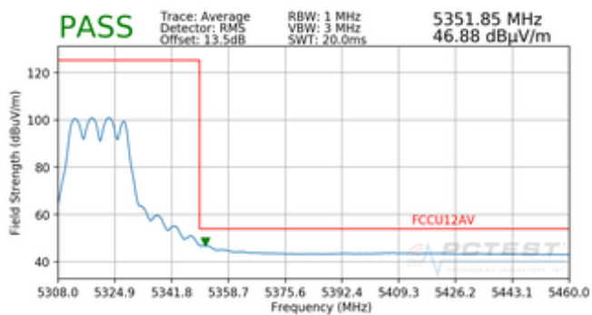
Plot 7-74. Radiated Band Edge Plot (Average – WCP)
