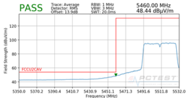
Plot 7-56. Radiated Band Edge Plot (Average – WCP)
