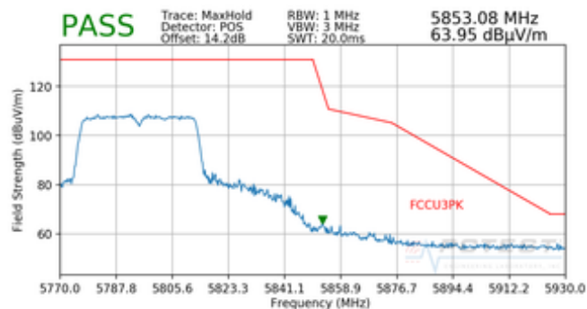
Plot 7-55. Radiated Upper Band Edge Plot (Peak – UNII Band 3)
