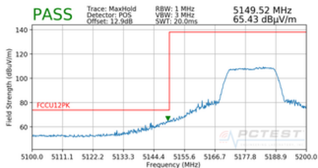
Plot 7-41. Radiated Lower Band Edge Plot (Peak – UNII Band 1)
