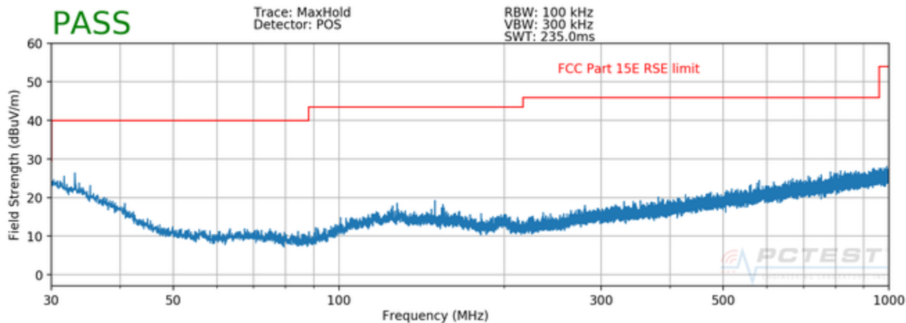
Plot 7-76. Radiated Spurious Plot below 1GHz (802.11a – U3 Ch. 157, Ant. Pol. H)
