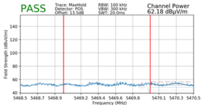
Plot 7-57. Radiated Band Edge Plot (Peak – WCP)
