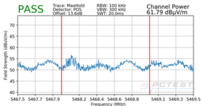
Plot 7-63. Radiated Lower Band Edge Plot (Peak – UNII Band 2C)
