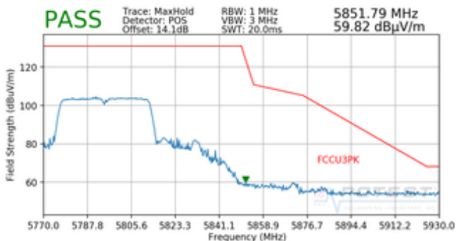
Plot 7-28. Radiated Upper Band Edge Plot (Peak – UNII Band 3)
