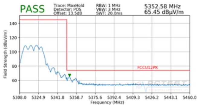
Plot 7-75. Radiated Band Edge Plot (Peak – WCP)
