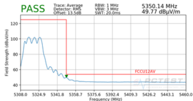
Plot 7-69. Radiated Upper Band Edge Plot (Average – UNII Band 2A)
