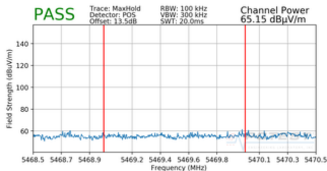
Plot 7-27. Radiated Lower Band Edge Plot (Peak – UNII Band 2C)
