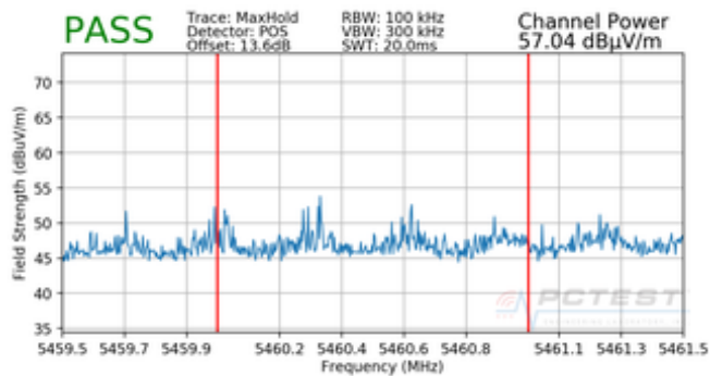
Plot 7-45. Radiated Lower Band Edge Plot (Peak – UNII Band 2C)
