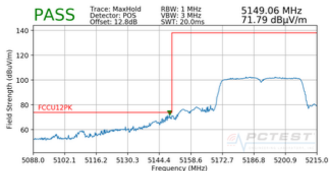
Plot 7-23. Radiated Lower Band Edge Plot (Peak – UNII Band 1)
