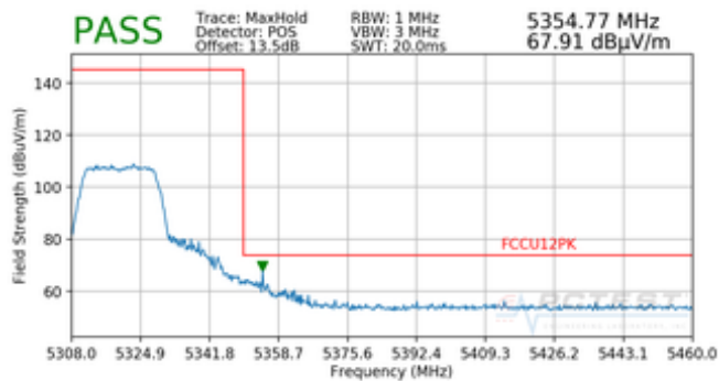
Plot 7-48. Radiated Band Edge Plot (Peak – WCP)
