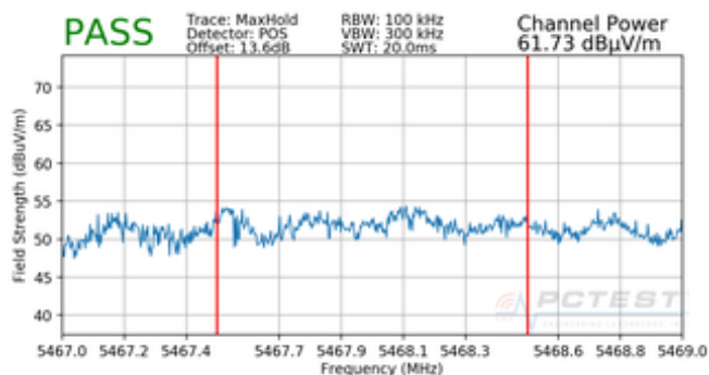
Plot 7-72. Radiated Lower Band Edge Plot (Peak – UNII Band 2C)
