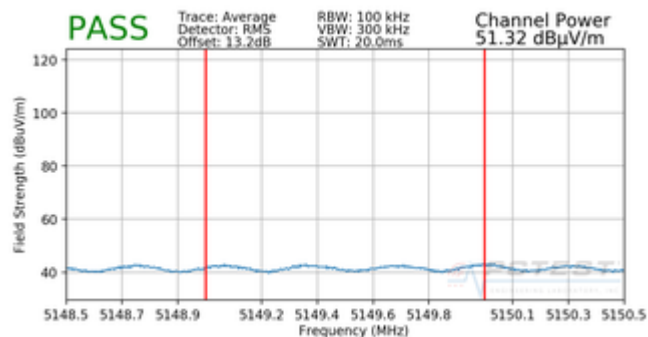
Plot 7-38. Radiated Band Edge Plot (Average – WCP)
