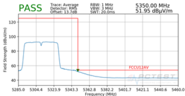
Plot 7-24. Radiated Upper Band Edge Plot (Average – UNII Band 2A)
