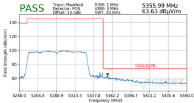
Plot 7-66. Radiated Band Edge Plot (Peak – WCP)
