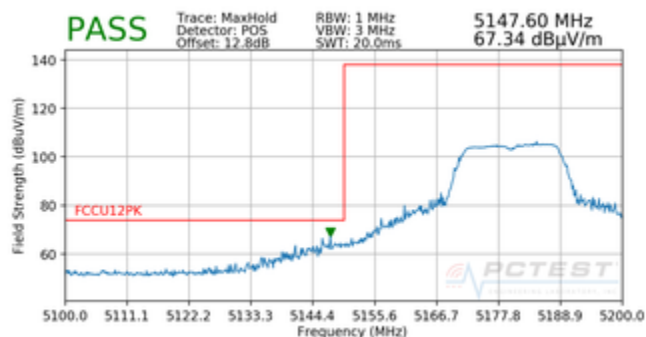
Plot 7-14. Radiated Lower Band Edge Plot (Peak – UNII Band 1)
