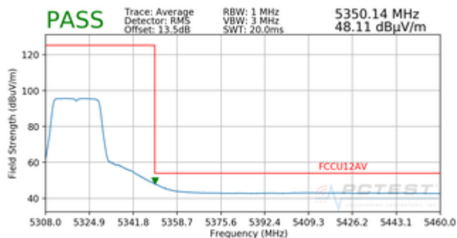
Plot 7-20. Radiated Band Edge Plot (Average – WCP)
