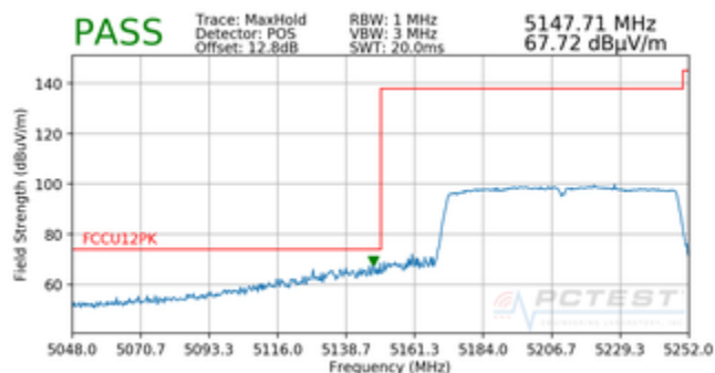
Plot 7-32. Radiated Lower Band Edge Plot (Peak – UNII Band 1)
