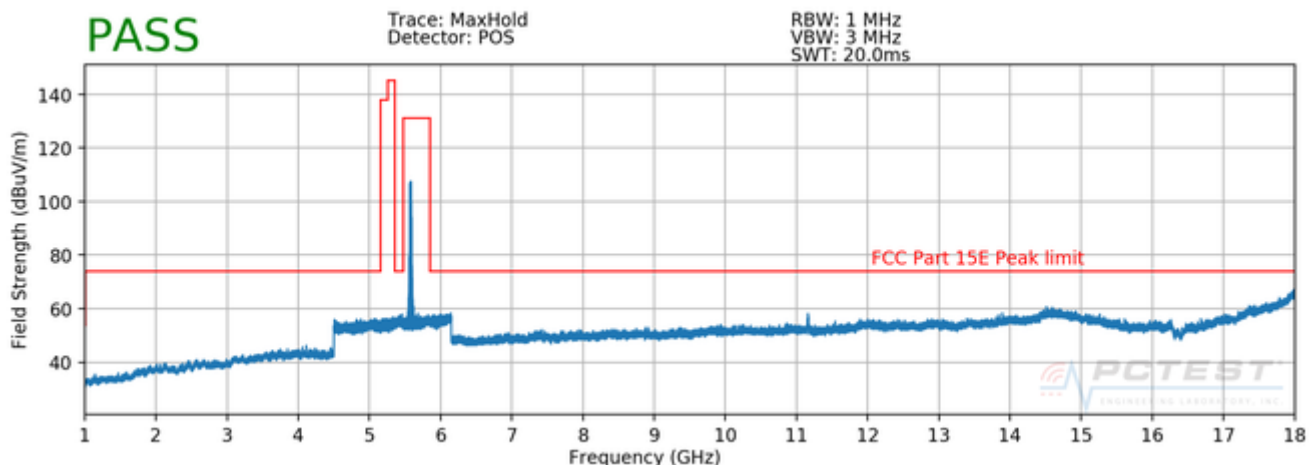
Plot 7-5. Radiated Spurious Plot above 1GHz (802.11a – U2C Ch. 116, Ant. Pol. H)
