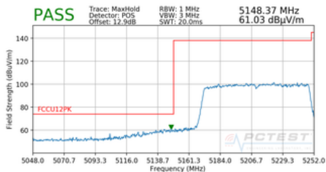
Plot 7-59. Radiated Lower Band Edge Plot (Peak – UNII Band 1)
