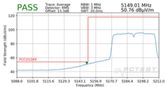
Plot 7-49. Radiated Lower Band Edge Plot (Average – UNII Band 1)
