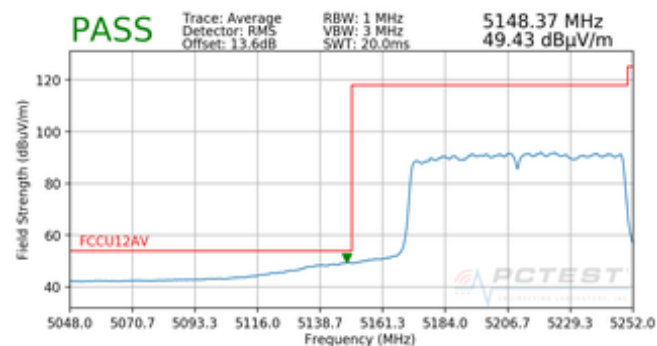
Plot 7-58. Radiated Lower Band Edge Plot (Average – UNII Band 1)
