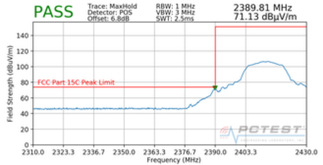
Plot 7-82. Radiated Restricted Band Edge Measurement with WCP (Peak)
