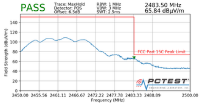
Plot 7-94. Radiated Restricted Band Edge Measurement with WCP (Peak)
