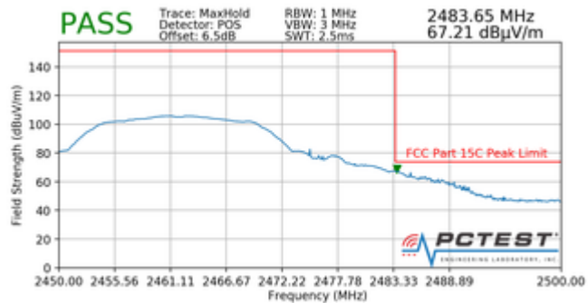
Plot 7-86. Radiated Restricted Upper Band Edge Measurement (Peak)
