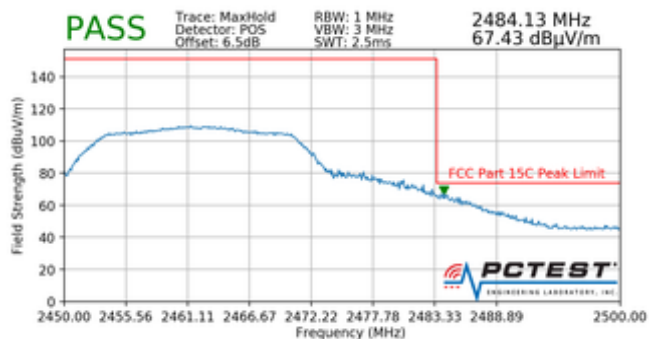
Plot 7-98. Radiated Restricted Upper Band Edge Measurement (Peak)
