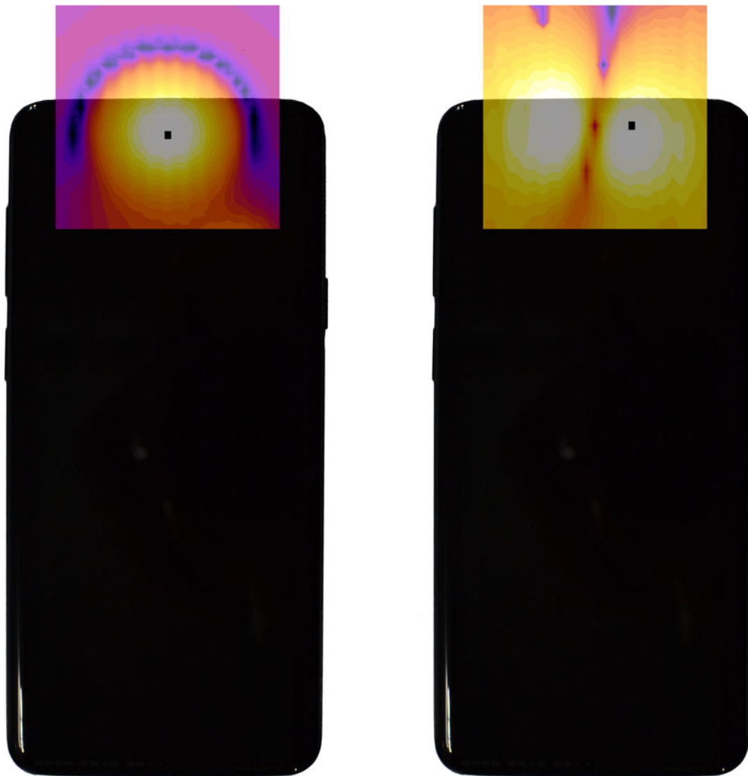
Figure 14-3 T-Coil Scan Overlay Magnetic Field Distributions
