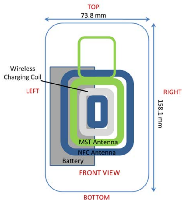
Figure F-2 NFC Antenna Locations
