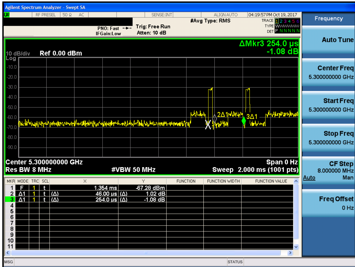
Figure 5-1. Band 2A Channel Loading
