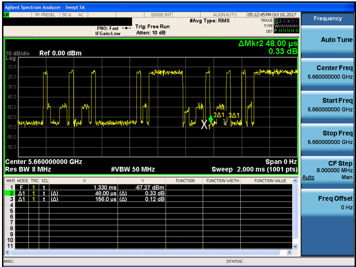
Figure 5-2. Band 2C Channel loading
