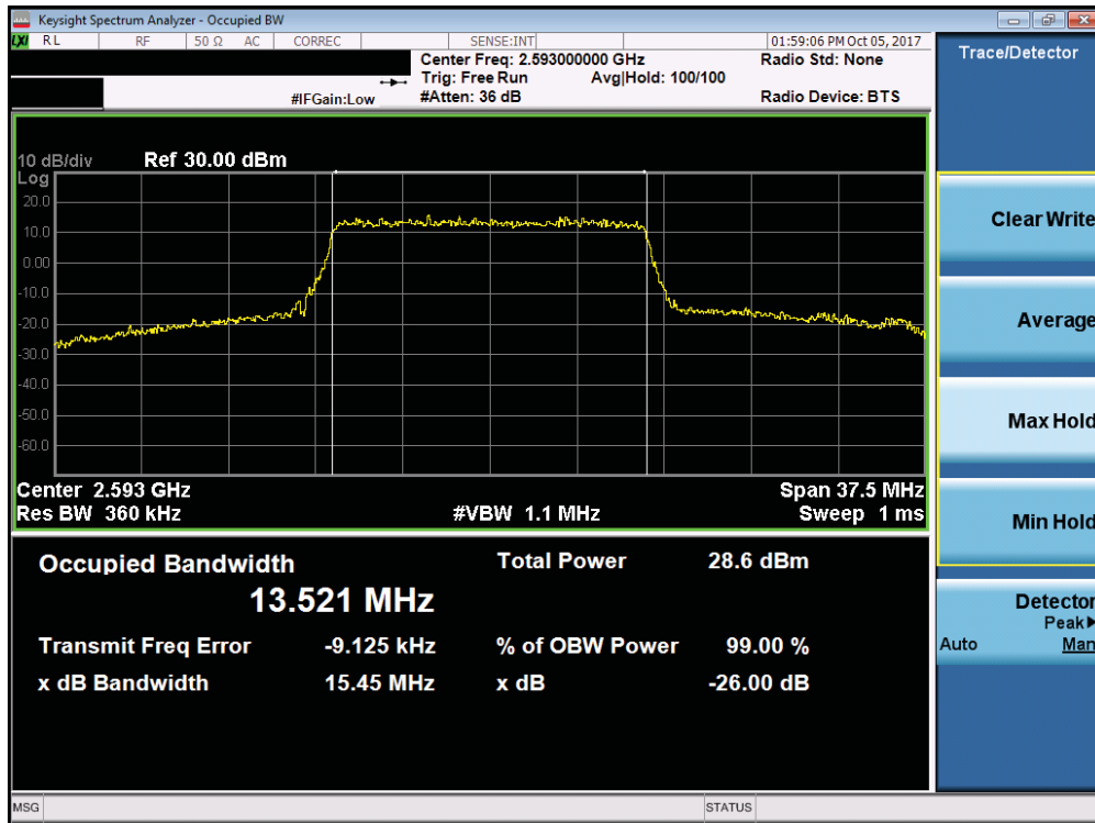
Plot 7-90. Occupied Bandwidth Plot (Band 38/41 - 15.0MHz 64-QAM - Full RB Configuration)
