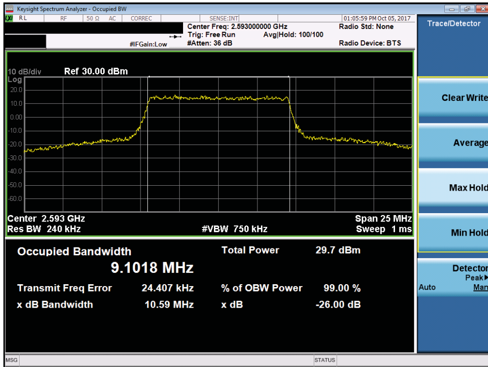
Plot 7-86. Occupied Bandwidth Plot (Band 38/41 - 10.0MHz 16-QAM - Full RB Configuration)
