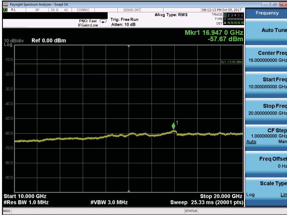
Plot 7-117. Conducted Spurious Plot (Band 66/4 - 10.0MHz QPSK - RB Size 1, RB Offset 0 - Low Channel)
