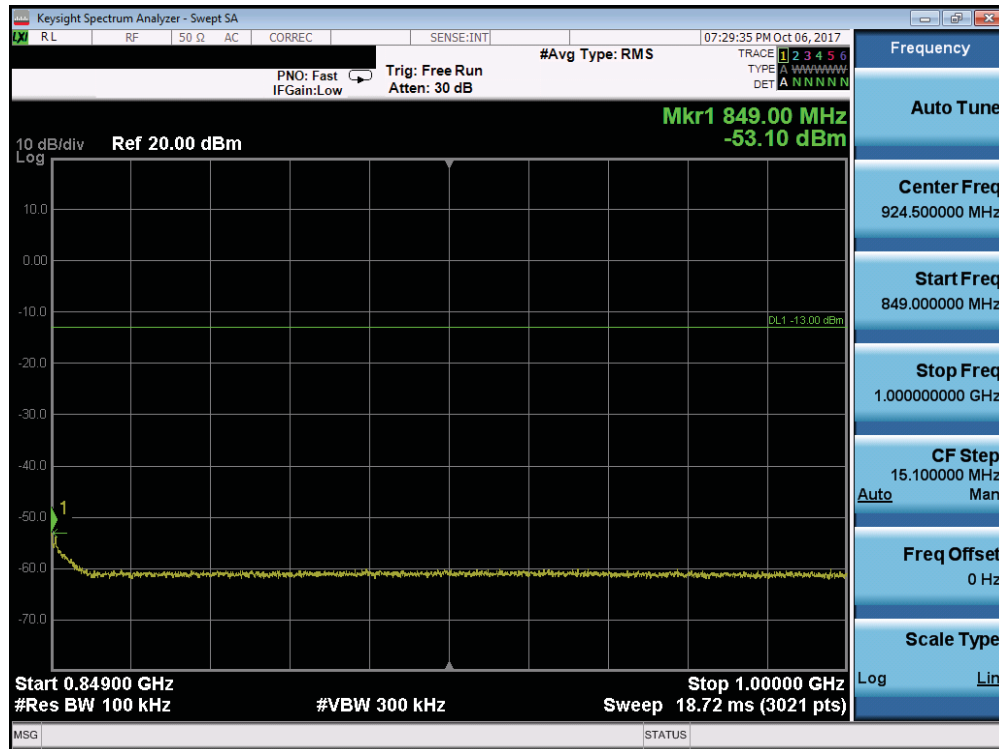
Plot 7-110. Conducted Spurious Plot (Band 5/26 - 10.0MHz QPSK - RB Size 1, RB Offset 0 - Mid Channel)
