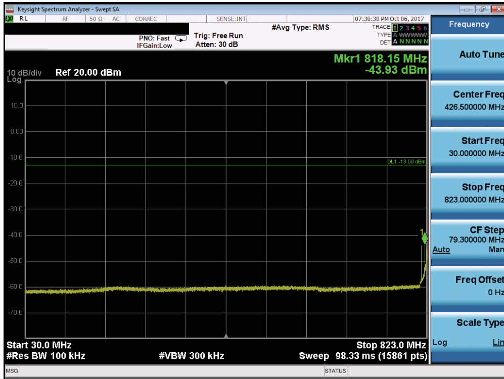
Plot 7-106. Conducted Spurious Plot (Band 5/26 - 10.0MHz QPSK - RB Size 1, RB Offset 0 - Low Channel)
