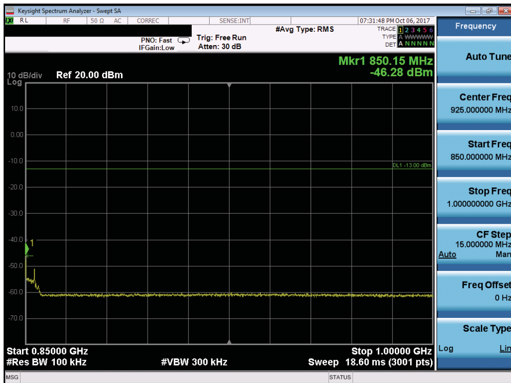
Plot 7-113. Conducted Spurious Plot (Band 5/26 - 10.0MHz QPSK - RB Size 1, RB Offset 0 - High Channel)
