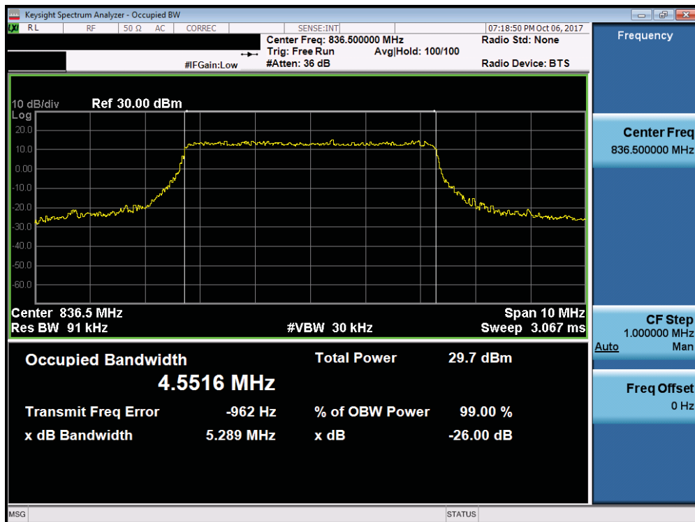
Plot 7-26. Occupied Bandwidth Plot (Band 5/26 – 5MHz 16-QAM - Full RB Configuration)
