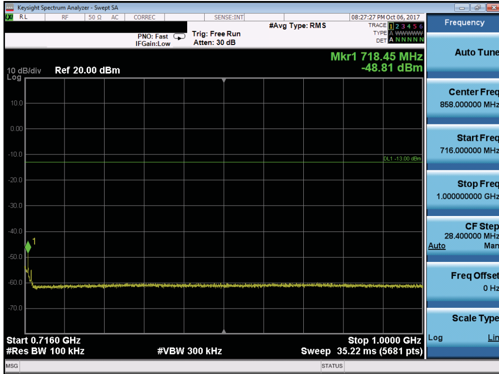
Plot 7-98. Conducted Spurious Plot (Band 12/17 - 10.0MHz QPSK - RB Size 1, RB Offset 0 - Mid Channel)
