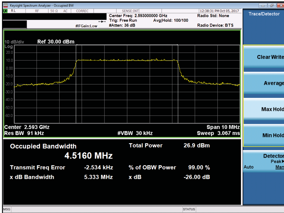
Plot 7-84. Occupied Bandwidth Plot (Band 38/41 - 5.0MHz 64-QAM - Full RB Configuration)
