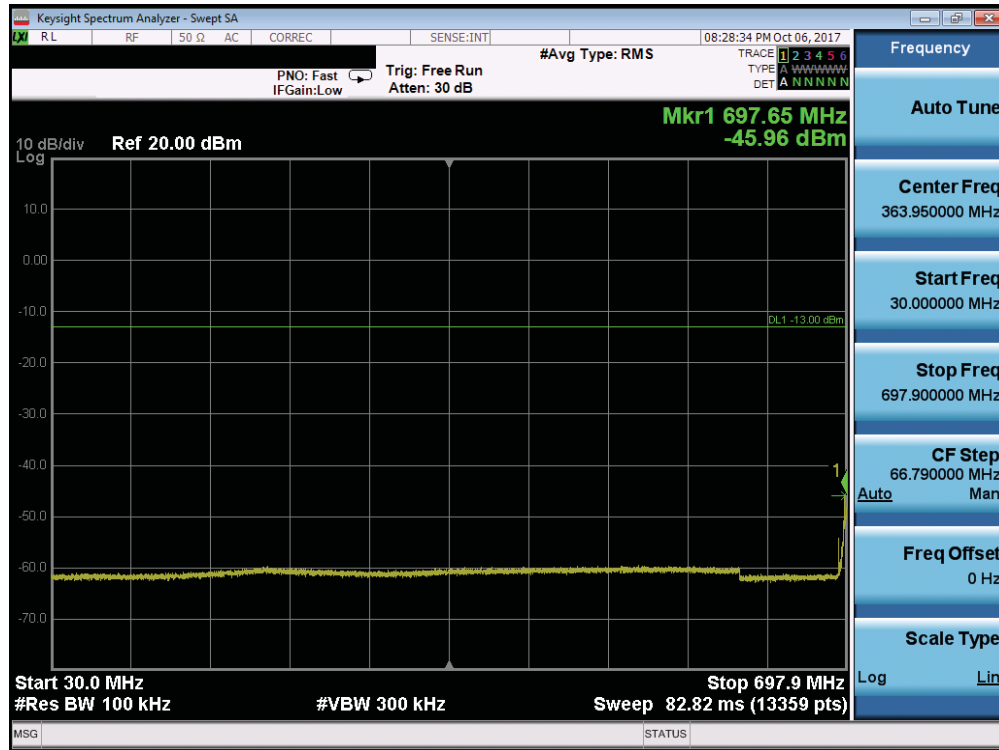
Plot 7-94. Conducted Spurious Plot (Band 12/17 - 10.0MHz QPSK - RB Size 1, RB Offset 0 - Low Channel)
