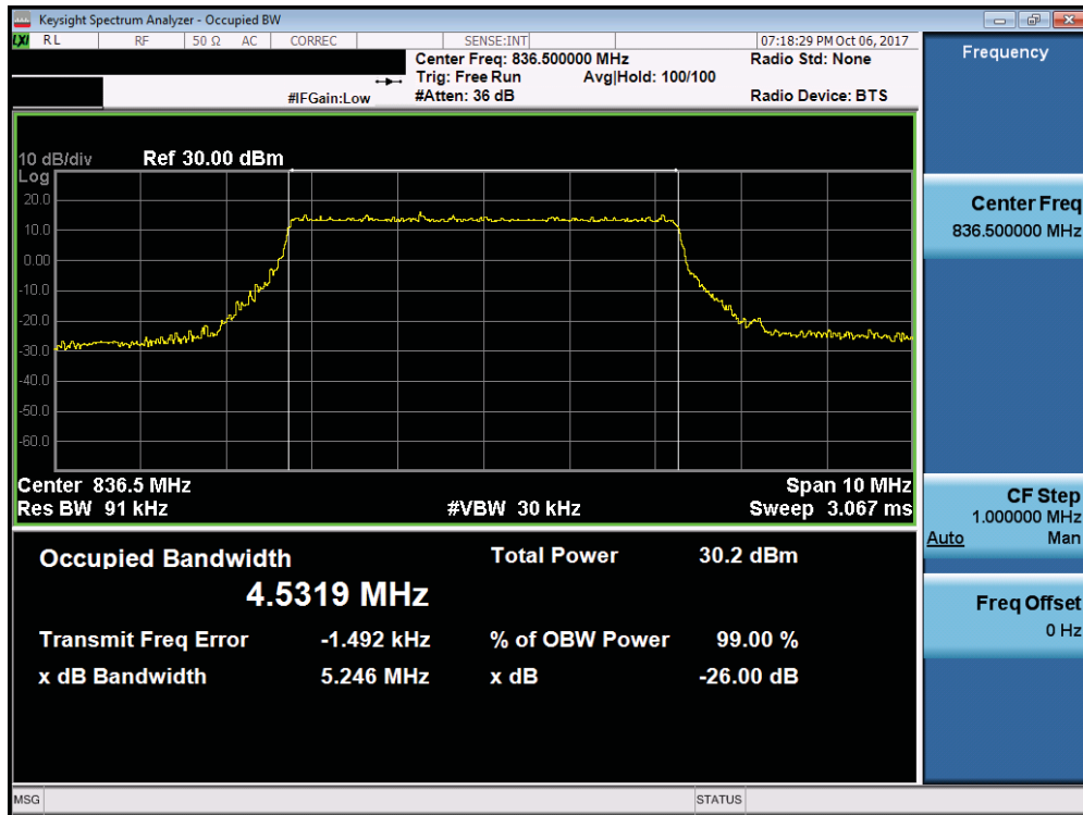
Plot 7-25. Occupied Bandwidth Plot (Band 5/26 – 5MHz QPSK - Full RB Configuration)
