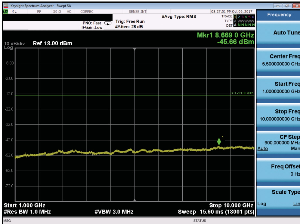
Plot 7-99. Conducted Spurious Plot (Band 12/17 - 10.0MHz QPSK - RB Size 1, RB Offset 0 - Mid Channel)
