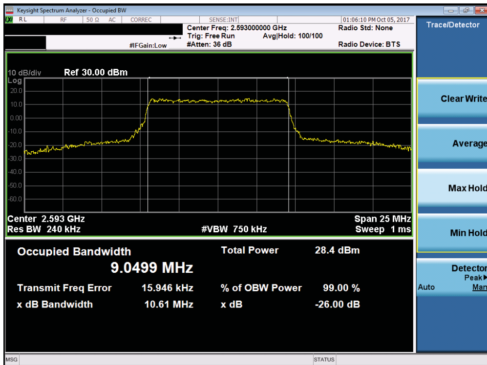
Plot 7-87. Occupied Bandwidth Plot (Band 38/41 - 10.0MHz 64-QAM - Full RB Configuration)
