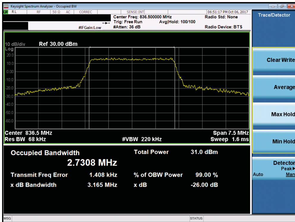
Plot 7-23. Occupied Bandwidth Plot (Band 5/26 – 3MHz 16-QAM - Full RB Configuration)
