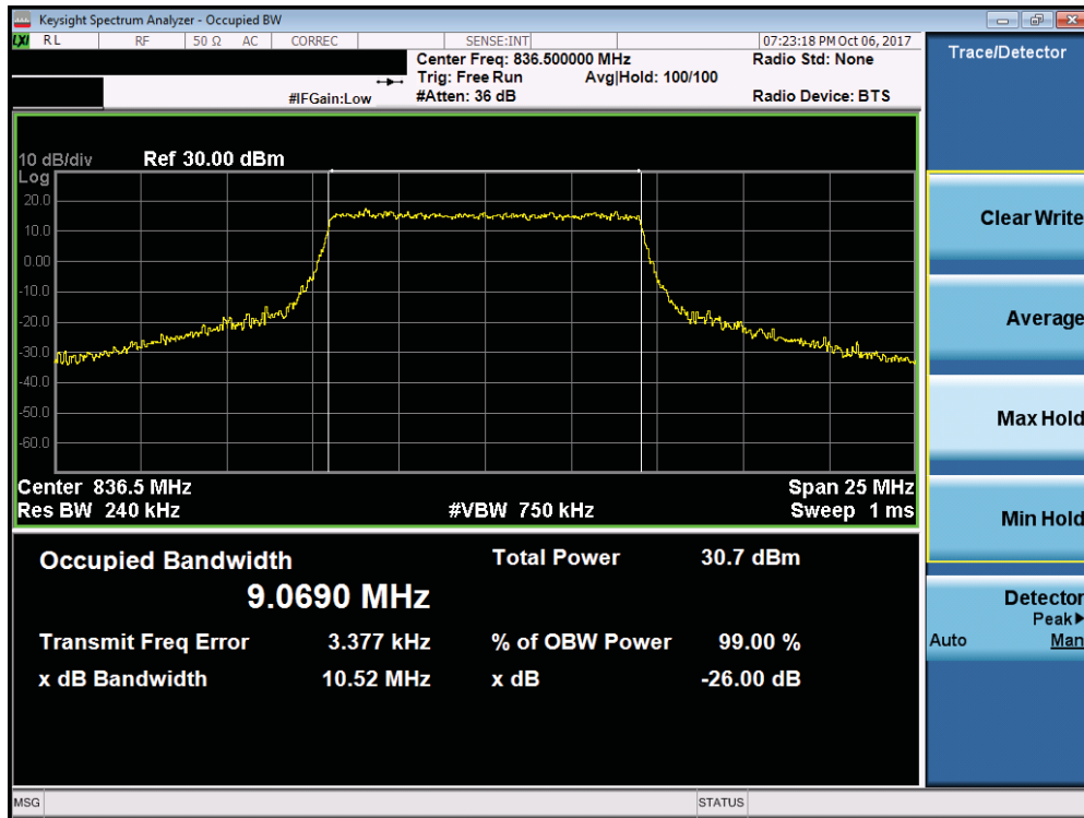
Plot 7-29. Occupied Bandwidth Plot (Band 5/26 – 10MHz 16-QAM - Full RB Configuration)
