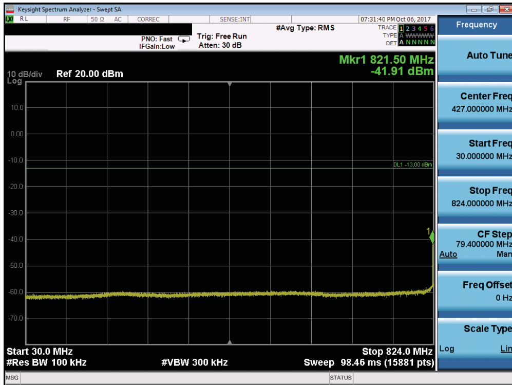
Plot 7-112. Conducted Spurious Plot (Band 5/26 - 10.0MHz QPSK - RB Size 1, RB Offset 0 - High Channel)
