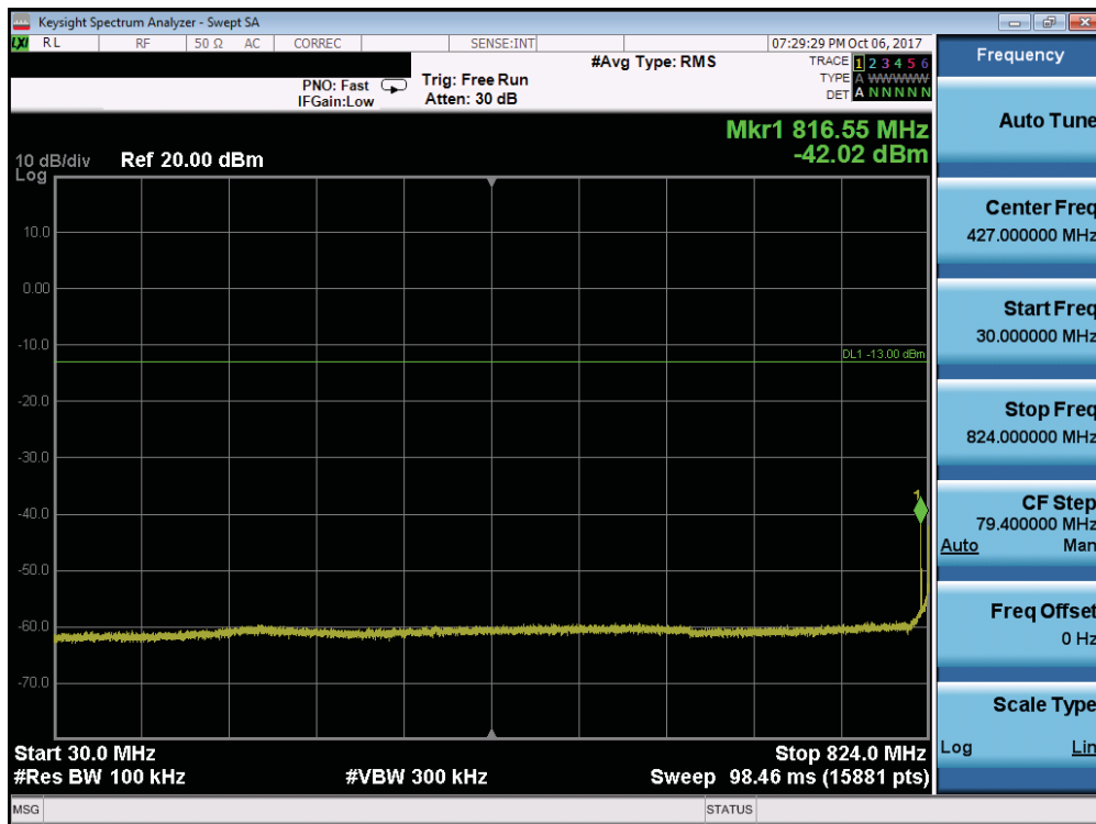
Plot 7-109. Conducted Spurious Plot (Band 5/26 - 10.0MHz QPSK - RB Size 1, RB Offset 0 - Mid Channel)
