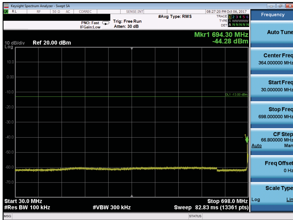
Plot 7-97. Conducted Spurious Plot (Band 12/17 - 10.0MHz QPSK - RB Size 1, RB Offset 0 - Mid Channel)
