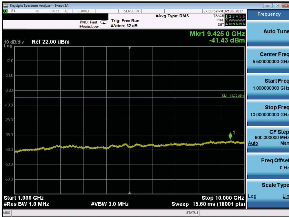
Plot 7-108. Conducted Spurious Plot (Band 5/26 - 10.0MHz QPSK - RB Size 1, RB Offset 0 - Low Channel)
