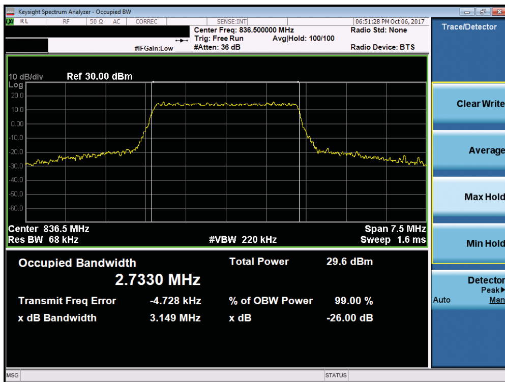
Plot 7-24. Occupied Bandwidth Plot (Band 5/26 – 3MHz 64-QAM - Full RB Configuration)
