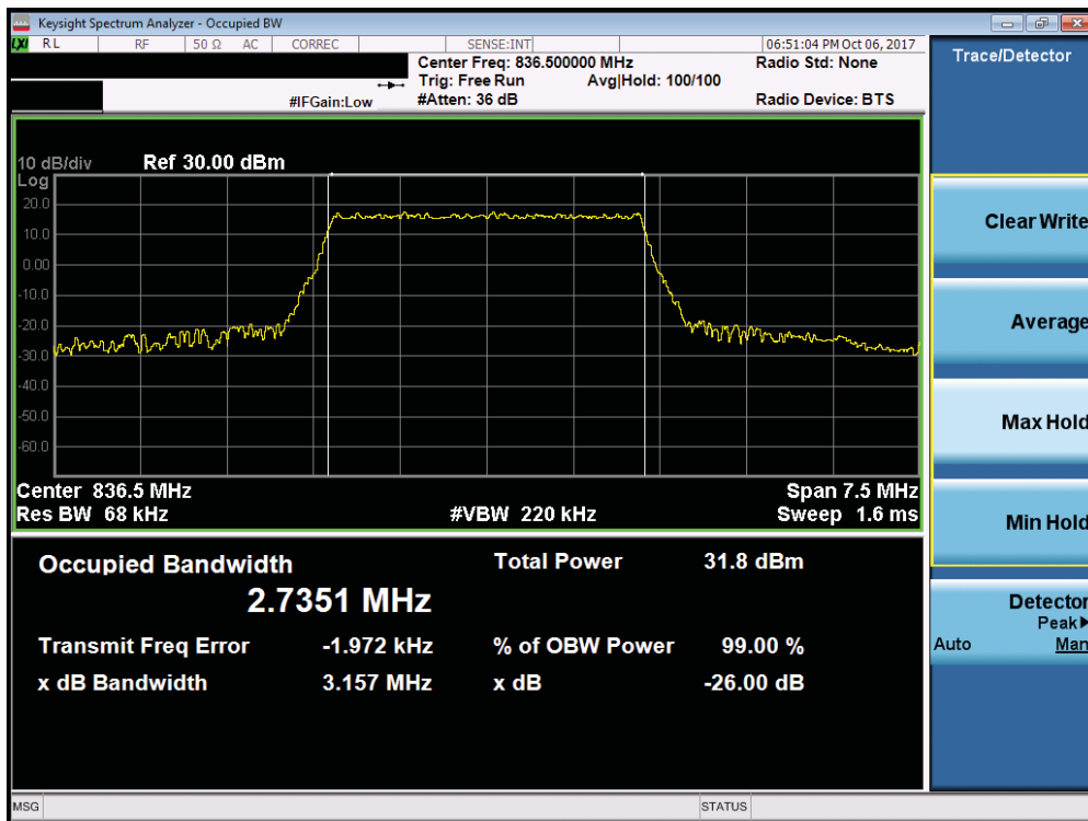
Plot 7-22. Occupied Bandwidth Plot (Band 5/26 – 3MHz QPSK - Full RB Configuration)
