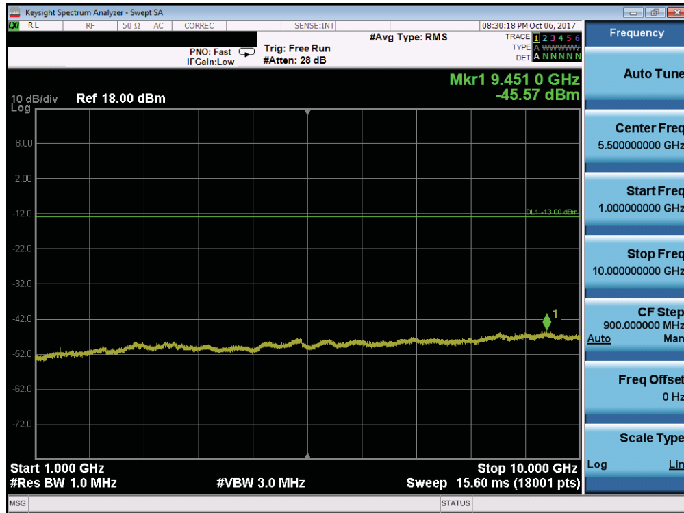
Plot 7-102. Conducted Spurious Plot (Band 12/17 - 10.0MHz QPSK - RB Size 1, RB Offset 0 - High Channel)
