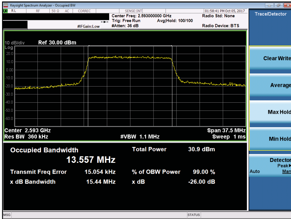
Plot 7-88. Occupied Bandwidth Plot (Band 38/41 - 15.0MHz QPSK - Full RB Configuration)
