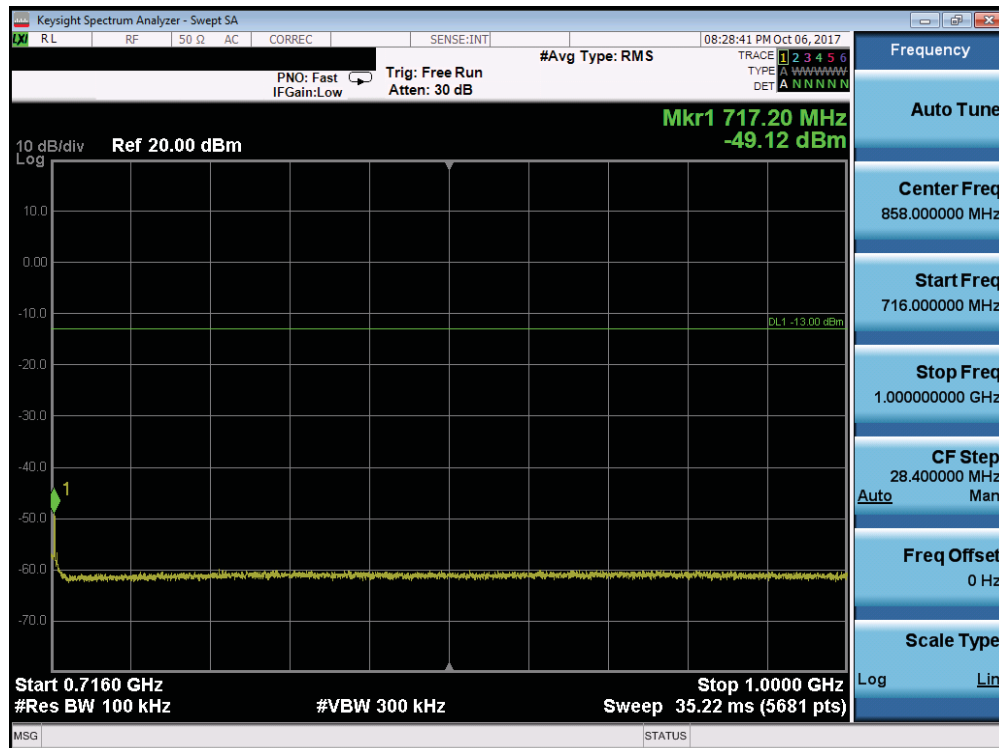
Plot 7-95. Conducted Spurious Plot (Band 12/17 - 10.0MHz QPSK - RB Size 1, RB Offset 0 - Low Channel)
