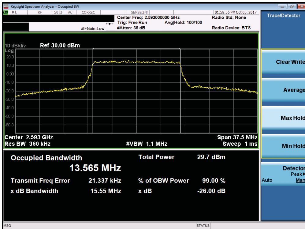
Plot 7-89. Occupied Bandwidth Plot (Band 38/41 - 15.0MHz 16-QAM - Full RB Configuration)
