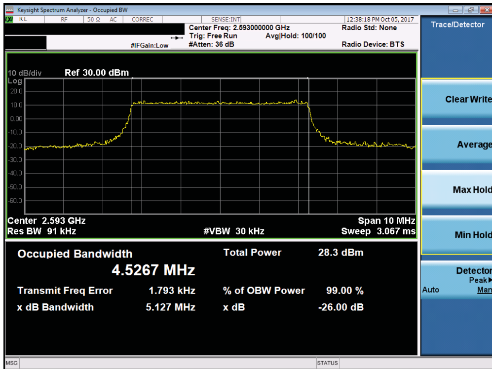
Plot 7-83. Occupied Bandwidth Plot (Band 38/41 - 5.0MHz 16-QAM - Full RB Configuration)
