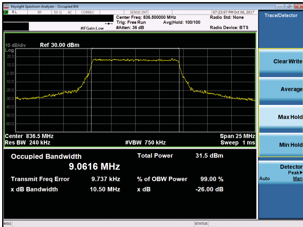
Plot 7-28. Occupied Bandwidth Plot (Band 5/26 – 10MHz QPSK - Full RB Configuration)
