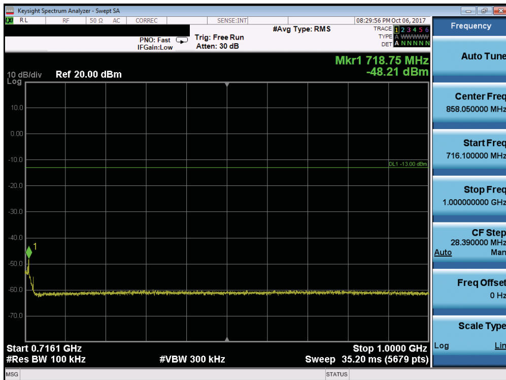
Plot 7-101. Conducted Spurious Plot (Band 12/17 - 10.0MHz QPSK - RB Size 1, RB Offset 0 - High Channel)
