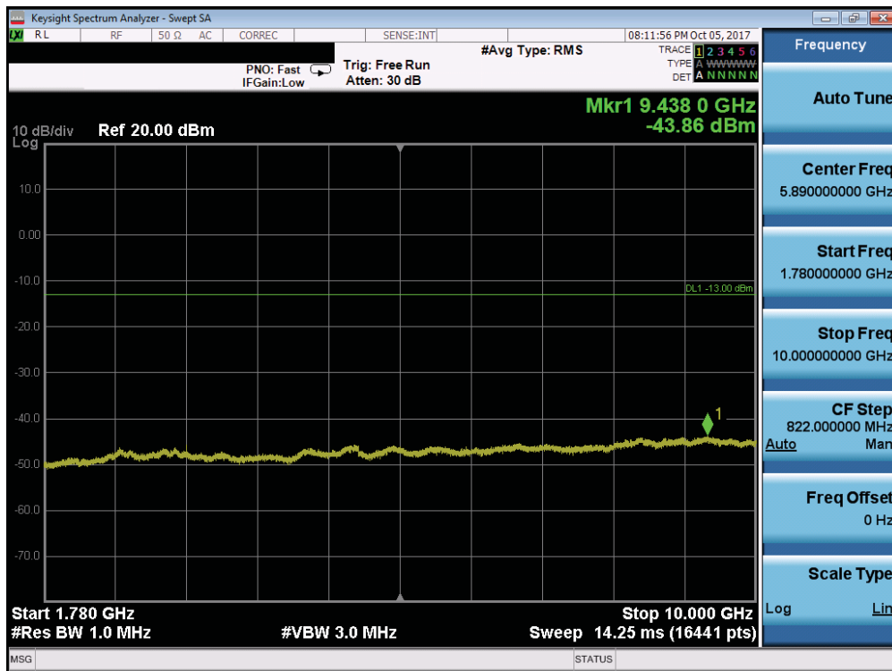
Plot 7-116. Conducted Spurious Plot (Band 66/4 - 10.0MHz QPSK - RB Size 1, RB Offset 0 - Low Channel)
