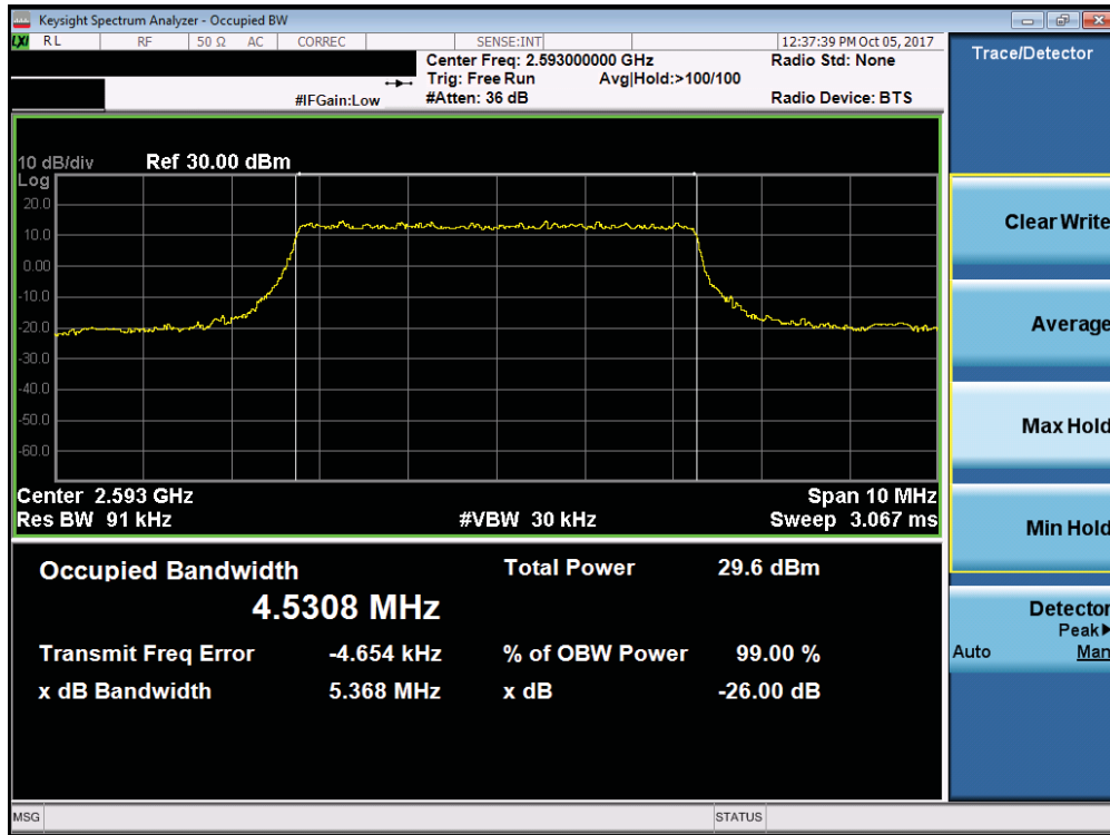
Plot 7-82. Occupied Bandwidth Plot (Band 38/41 - 5.0MHz QPSK - Full RB Configuration)
