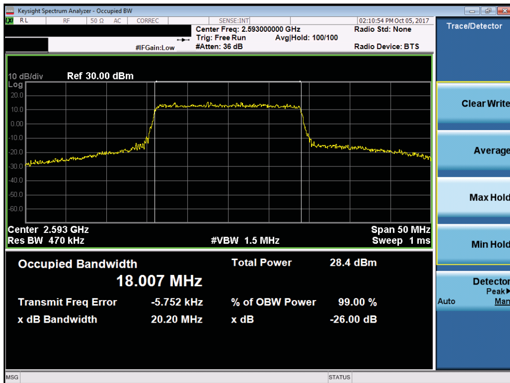
Plot 7-93. Occupied Bandwidth Plot (Band 38/41 - 20.0MHz 64-QAM - Full RB Configuration)
