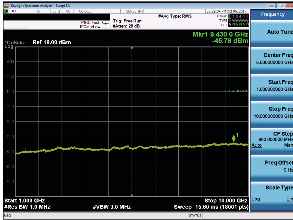
Plot 7-96. Conducted Spurious Plot (Band 12/17 - 10.0MHz QPSK - RB Size 1, RB Offset 0 - Low Channel)
