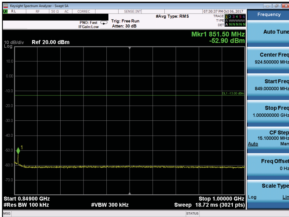
Plot 7-107. Conducted Spurious Plot (Band 5/26 - 10.0MHz QPSK - RB Size 1, RB Offset 0 - Low Channel)
