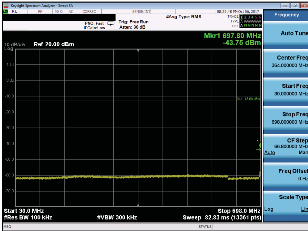
Plot 7-100. Conducted Spurious Plot (Band 12/17 - 10.0MHz QPSK - RB Size 1, RB Offset 0 - High Channel)
