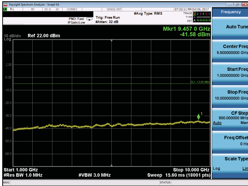
Plot 7-114. Conducted Spurious Plot (Band 5/26 - 10.0MHz QPSK - RB Size 1, RB Offset 0 - High Channel)
