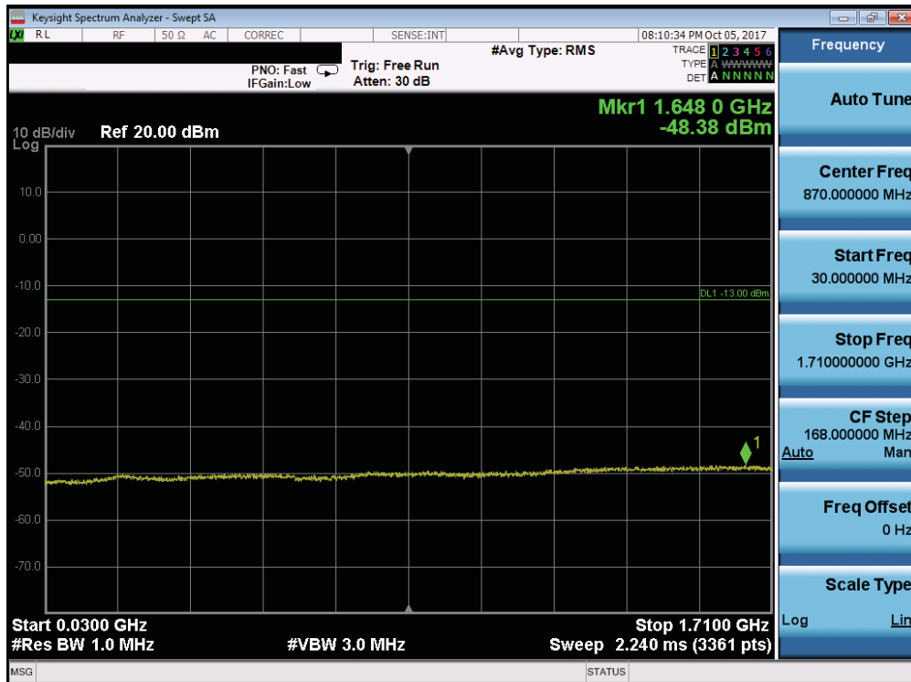
Plot 7-118. Conducted Spurious Plot (Band 66/4 - 10.0MHz QPSK - RB Size 1, RB Offset 0 - Mid Channel)
