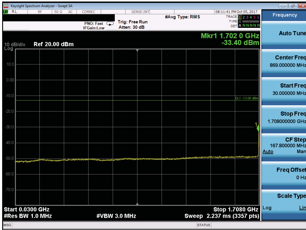
Plot 7-115. Conducted Spurious Plot (Band 66/4 - 10.0MHz QPSK - RB Size 1, RB Offset 0 - Low Channel)
