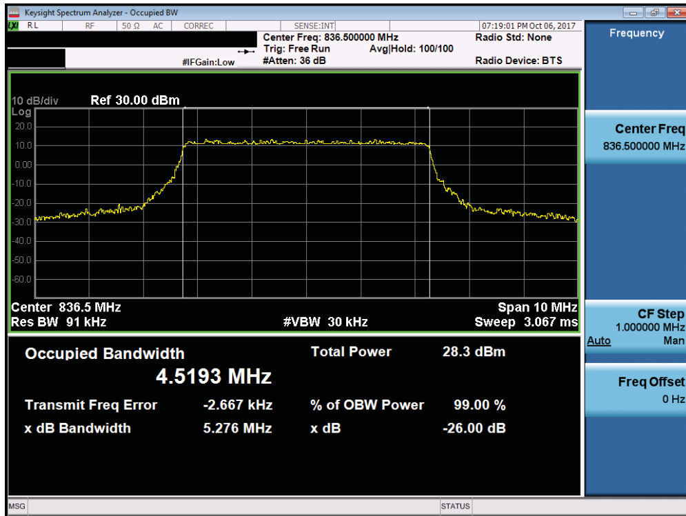
Plot 7-27. Occupied Bandwidth Plot (Band 5/26 – 5MHz 64-QAM - Full RB Configuration)
