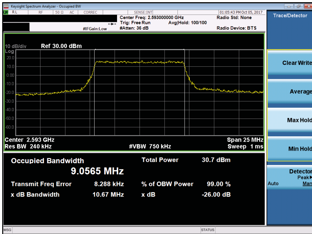
Plot 7-85. Occupied Bandwidth Plot (Band 38/41 - 10.0MHz QPSK - Full RB Configuration)
