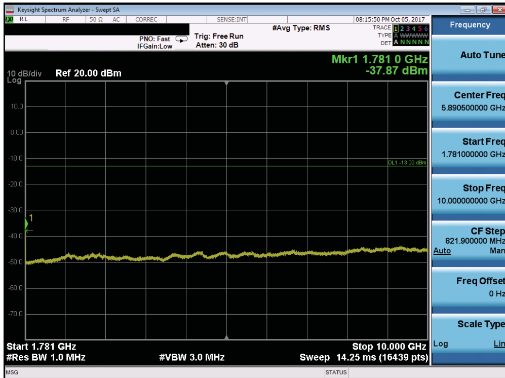
Plot 7-122. Conducted Spurious Plot (Band 66/4 - 10.0MHz QPSK - RB Size 1, RB Offset 0 - High Channel)
