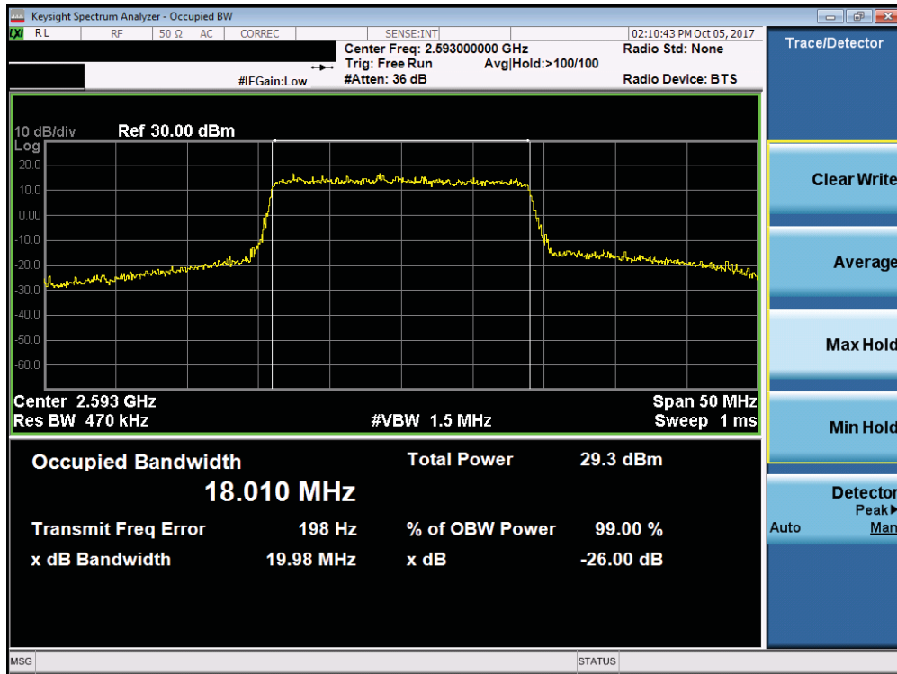
Plot 7-92. Occupied Bandwidth Plot (Band 38/41 - 20.0MHz 16-QAM - Full RB Configuration)
