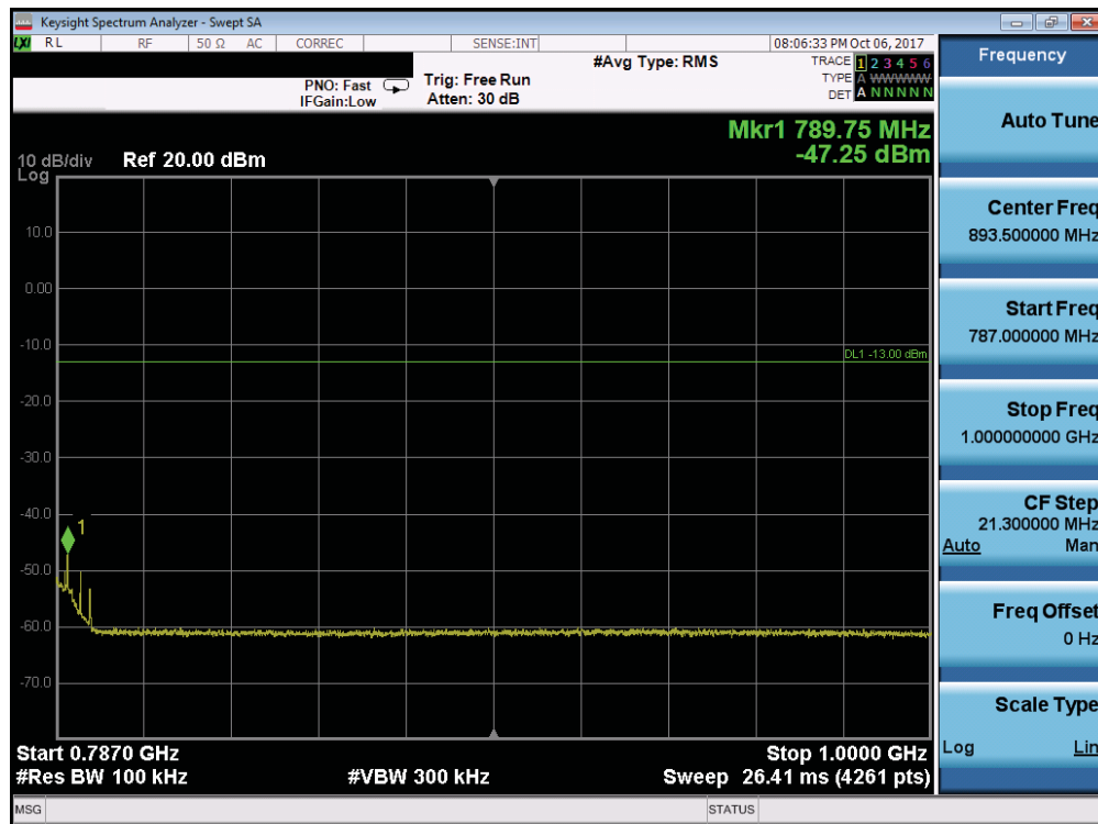
Plot 7-104. Conducted Spurious Plot (Band 13 - 10.0MHz QPSK - RB Size 1, RB Offset 0)
