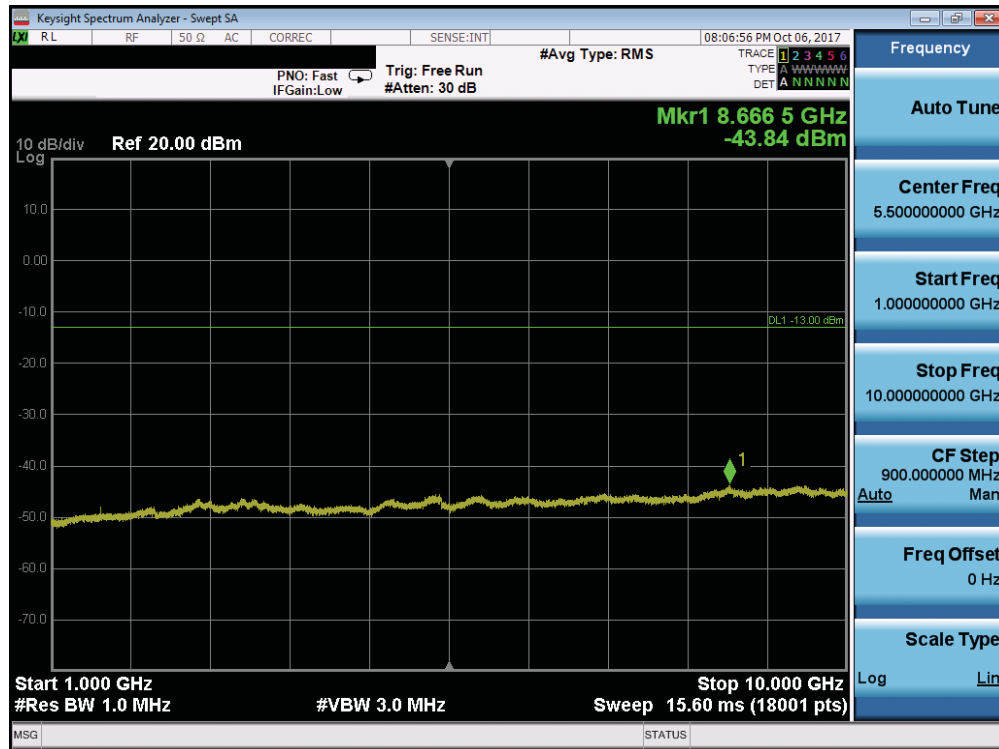
Plot 7-105. Conducted Spurious Plot (Band 13 - 10.0MHz QPSK - RB Size 1, RB Offset 0)
