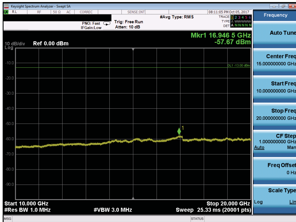
Plot 7-120. Conducted Spurious Plot (Band 66/4 - 10.0MHz QPSK - RB Size 1, RB Offset 0 - Mid Channel)
