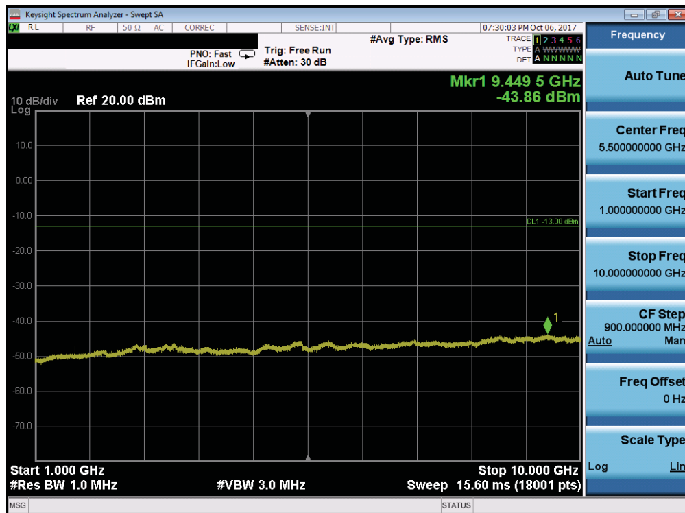
Plot 7-111. Conducted Spurious Plot (Band 5/26 - 10.0MHz QPSK - RB Size 1, RB Offset 0 - Mid Channel)
