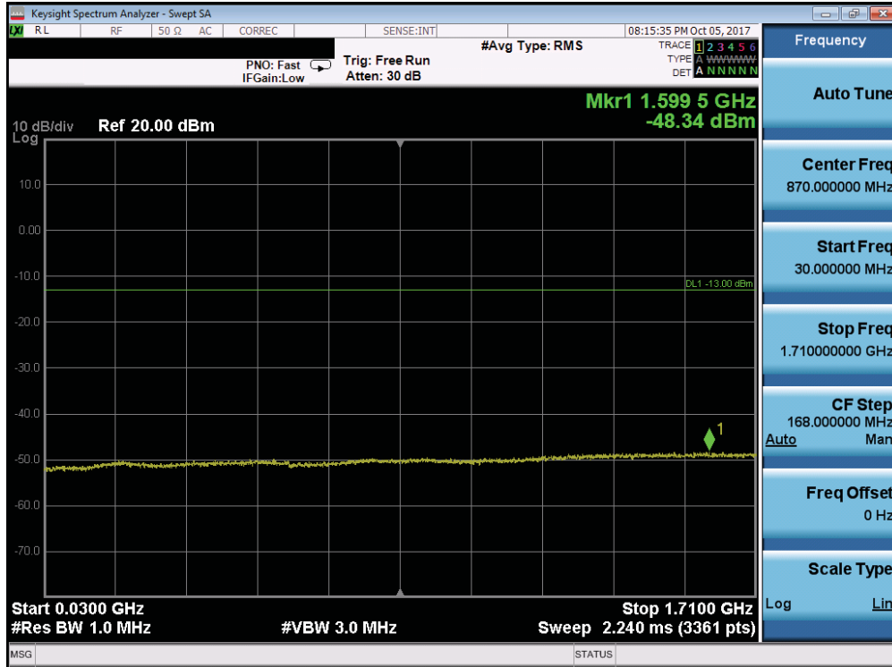
Plot 7-121. Conducted Spurious Plot (Band 66/4 - 10.0MHz QPSK - RB Size 1, RB Offset 0 - High Channel)
