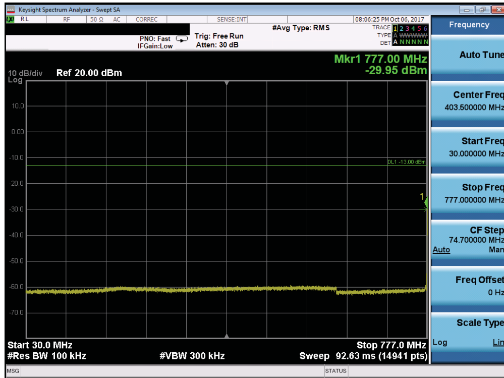
Plot 7-103. Conducted Spurious Plot (Band 13 - 10.0MHz QPSK - RB Size 1, RB Offset 0)
