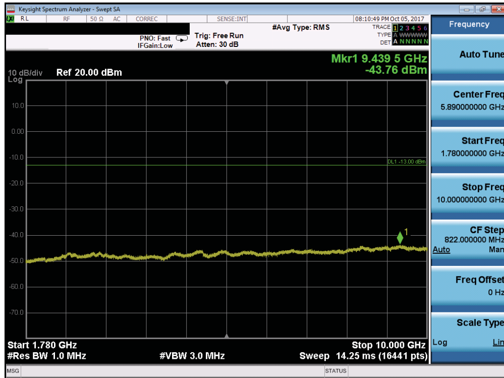
Plot 7-119. Conducted Spurious Plot (Band 66/4 - 10.0MHz QPSK - RB Size 1, RB Offset 0 - Mid Channel)
