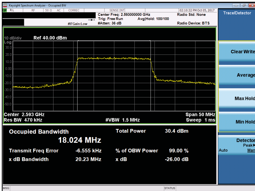
Plot 7-91. Occupied Bandwidth Plot (Band 38/41 - 20.0MHz QPSK - Full RB Configuration)
