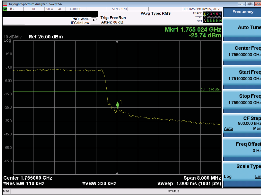
Plot 7-199. Upper Band Edge Plot (Band 4 - 10.0MHz QPSK - Full RB Configuration)
