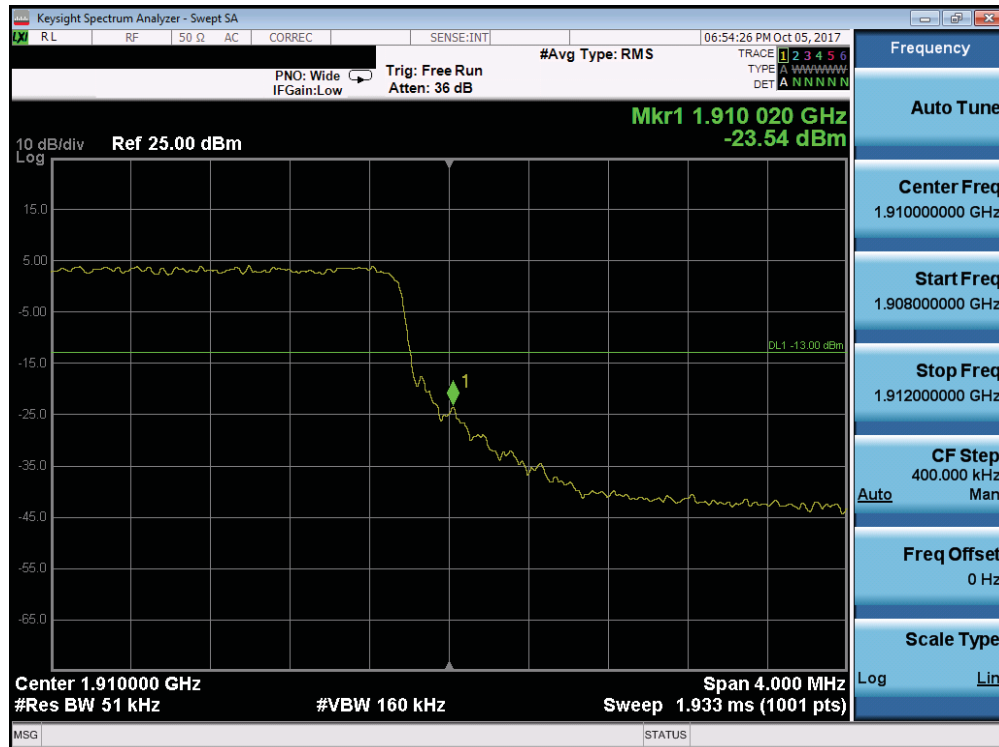
Plot 7-229. Upper Band Edge Plot (Band 2 - 5.0MHz QPSK - Full RB Configuration)
