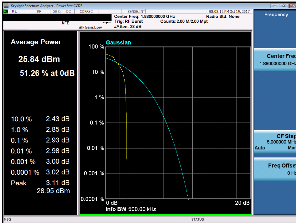
Plot 7-72. Peak-Average Ratio Plot (PCS EGPRS Mode)
