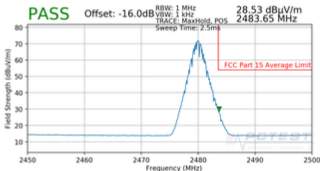
Plot 7-52. Radiated Restricted Upper Band Edge Measurement with WCP (Average)
