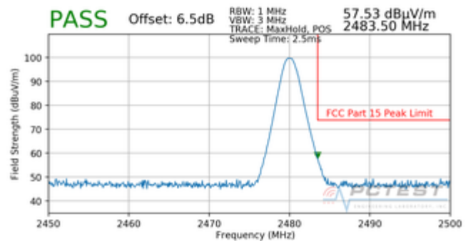
Plot 7-53. Radiated Restricted Upper Band Edge Measurement with WCP (Peak)
