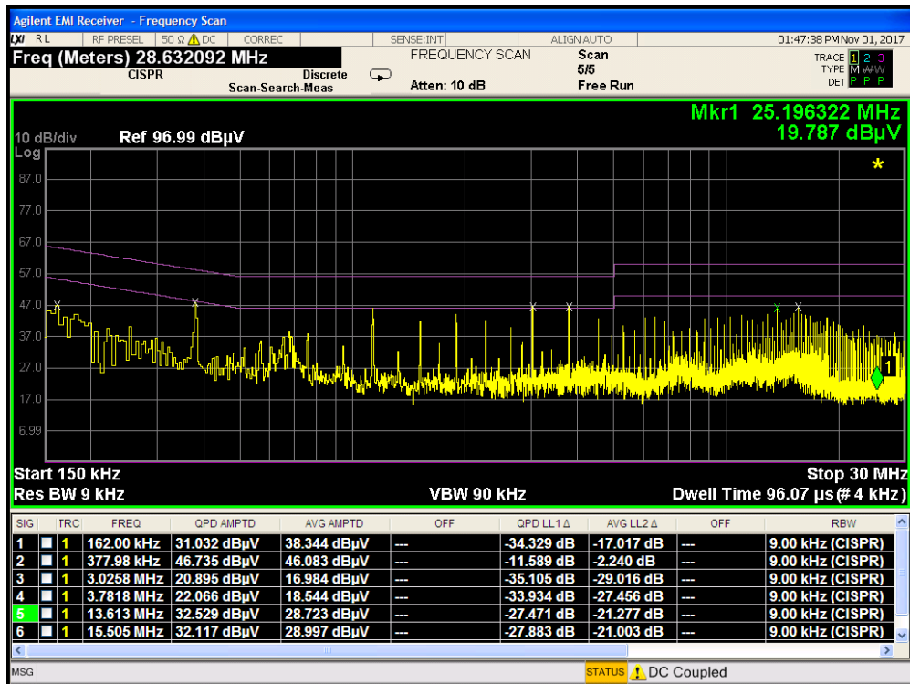
Plot 7-59. Line-Conducted Test Plot with Wireless Charging Pad (N)
