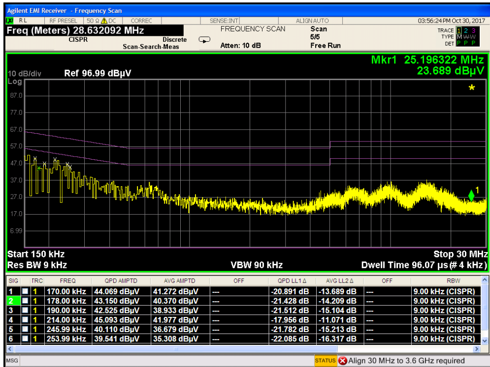
Plot 7-56. Line-Conducted Test Plot with Travel Adapter (L1)
