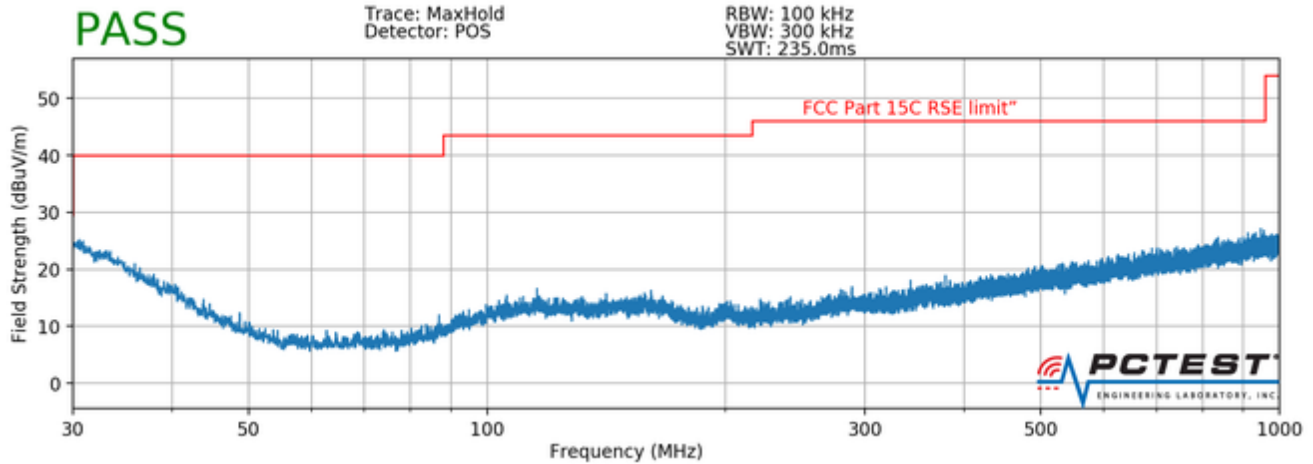
Plot 7-55. Radiated Spurious Plot below 1GHz (Pol. V)
