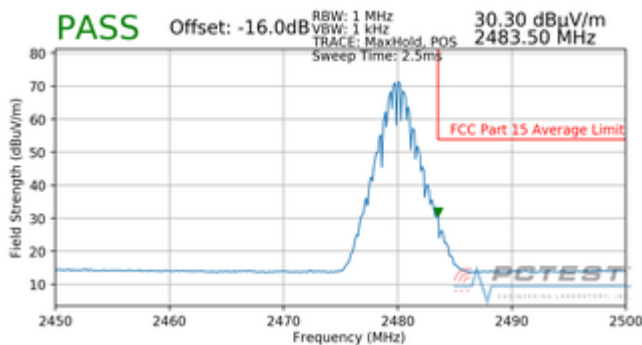
Plot 7-50. Radiated Restricted Upper Band Edge Measurement (Average)
