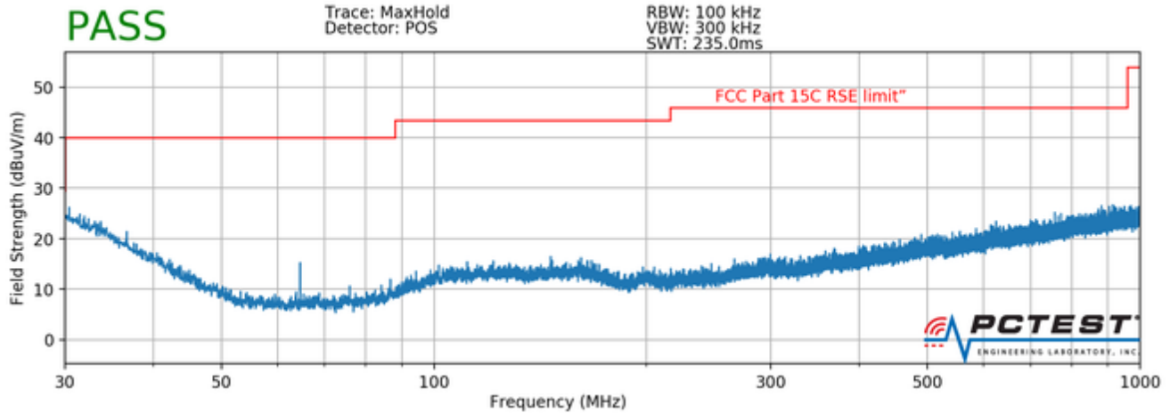
Plot 7-54. Radiated Spurious Plot below 1GHz (Pol. H)
