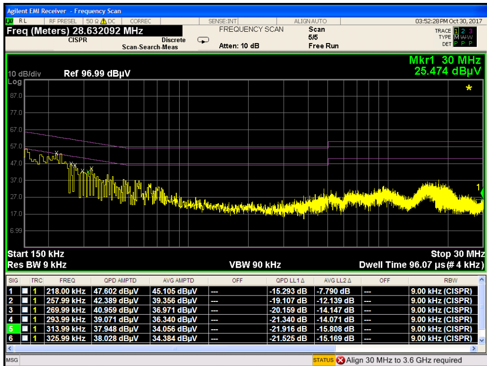
Plot 7-57. Line-Conducted Test Plot with Travel Adapter (N)
