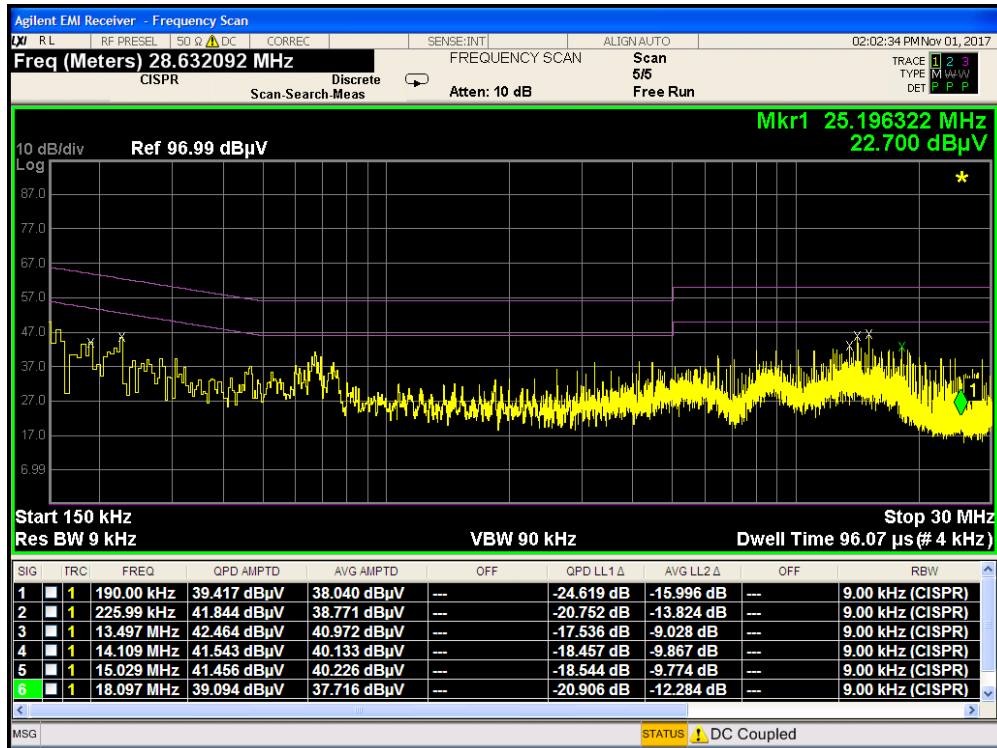
Plot 7-58. Line-Conducted Test Plot with Wireless Charging Pad (L1)
