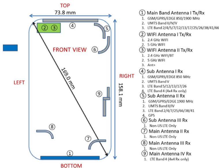
Figure F-1 DUT Antenna Locations
