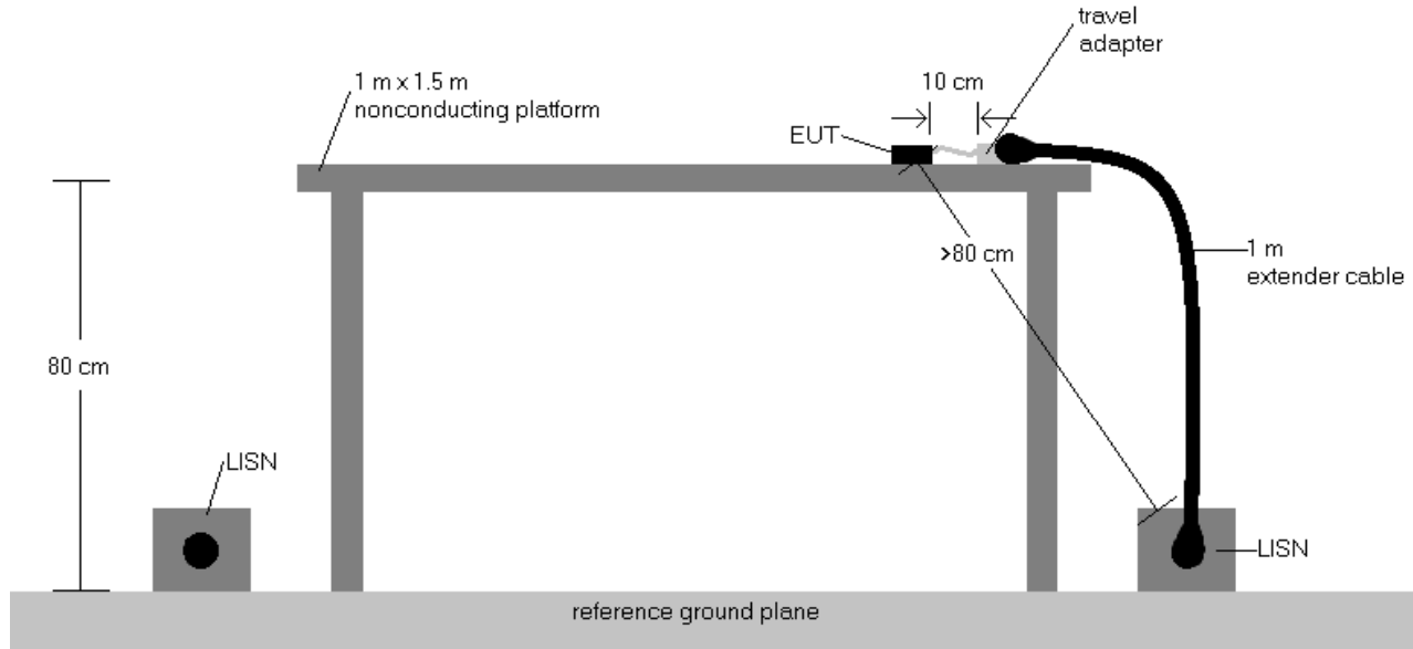
Figure 7-7. Test Instrument & Measurement Setup
