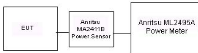
Figure 7-3. Test Instrument & Measurement Setup
