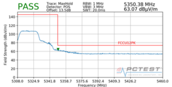
Plot 7-229. Radiated Upper Band Edge Plot (Peak – UNII Band 2A)
