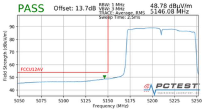
Plot 7-224. Radiated Band Edge Plot (Average – WCP)
