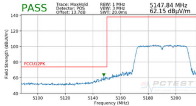
Plot 7-270. Radiated Band Edge Plot (Peak – WCP)
