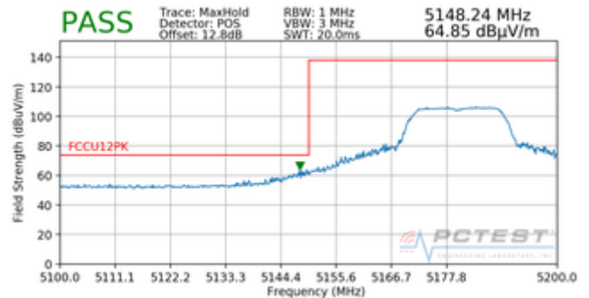
Plot 7-227. Radiated Lower Band Edge Plot (Peak – UNII Band 1)
