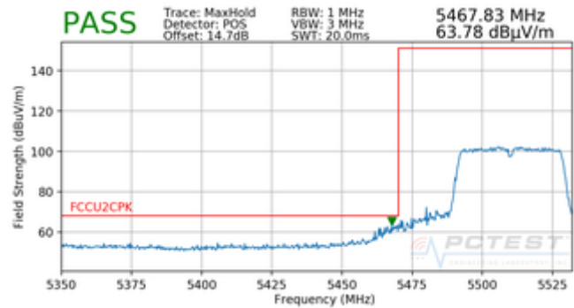
Plot 7-267. Radiated Lower Band Edge Plot (Peak – UNII Band 2C)
