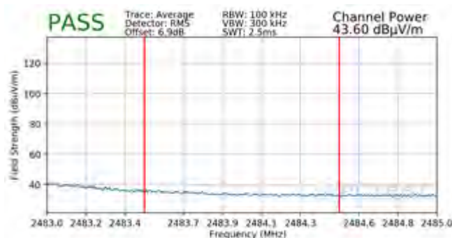
Plot 7-227. Radiated Restricted Upper Band Edge Measurement MIMO (Average – 242 Tones)
