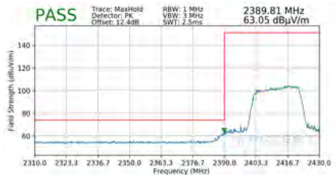
Plot 7-178. Radiated Restricted Band Edge Measurement SISO ANT1 with WCP (Peak – 242 Tones)
