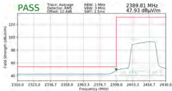
Plot 7-177. Radiated Restricted Band Edge Measurement SISO ANT1 with WCP (Average – 242 Tones)
