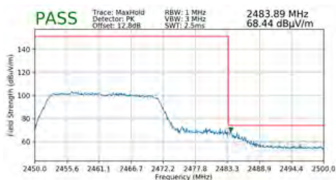
Plot 7-230. Radiated Restricted Band Edge Measurement MIMO with WCP (Peak – 242 Tones)
