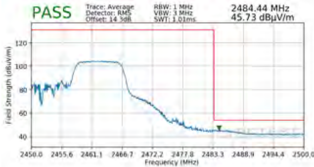
Plot 7-157. Radiated Restricted Upper Band Edge Measurement SISO ANT1 (Average – 106 Tones)
