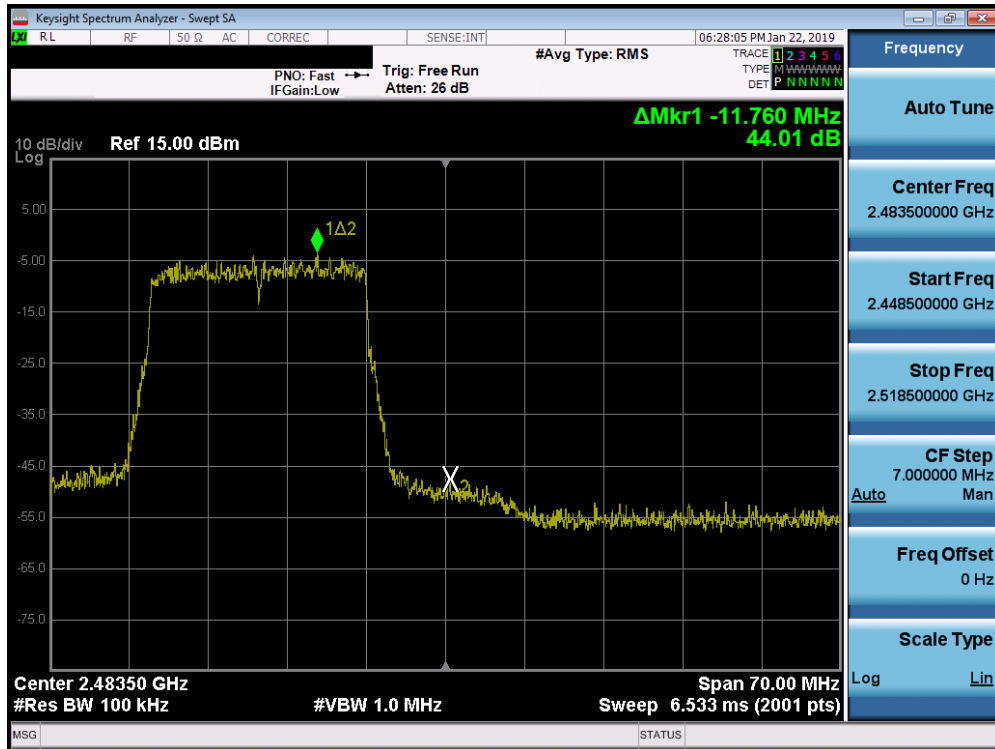
Plot 7-63. Band Edge Plot SISO ANT1 (802.11ax OFDMA - 242 Tones - Ch. 12)
