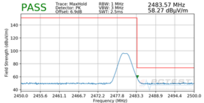
Plot 7-54. Radiated Restricted Upper Band Edge Measurement with WCP (Peak)
