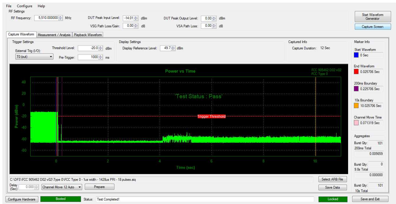
Figure 5-4. Band 2C Move Time and Aggregate Time
